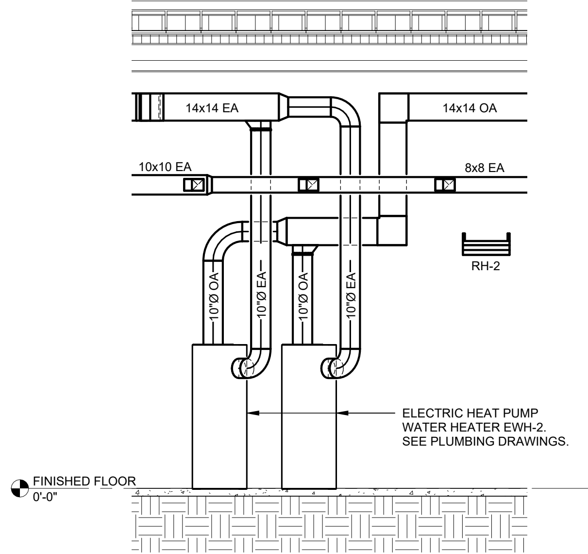
2 WATER HEATER DUCTWORK ELEVATION SCALE: 1/4" = 1'-0"
