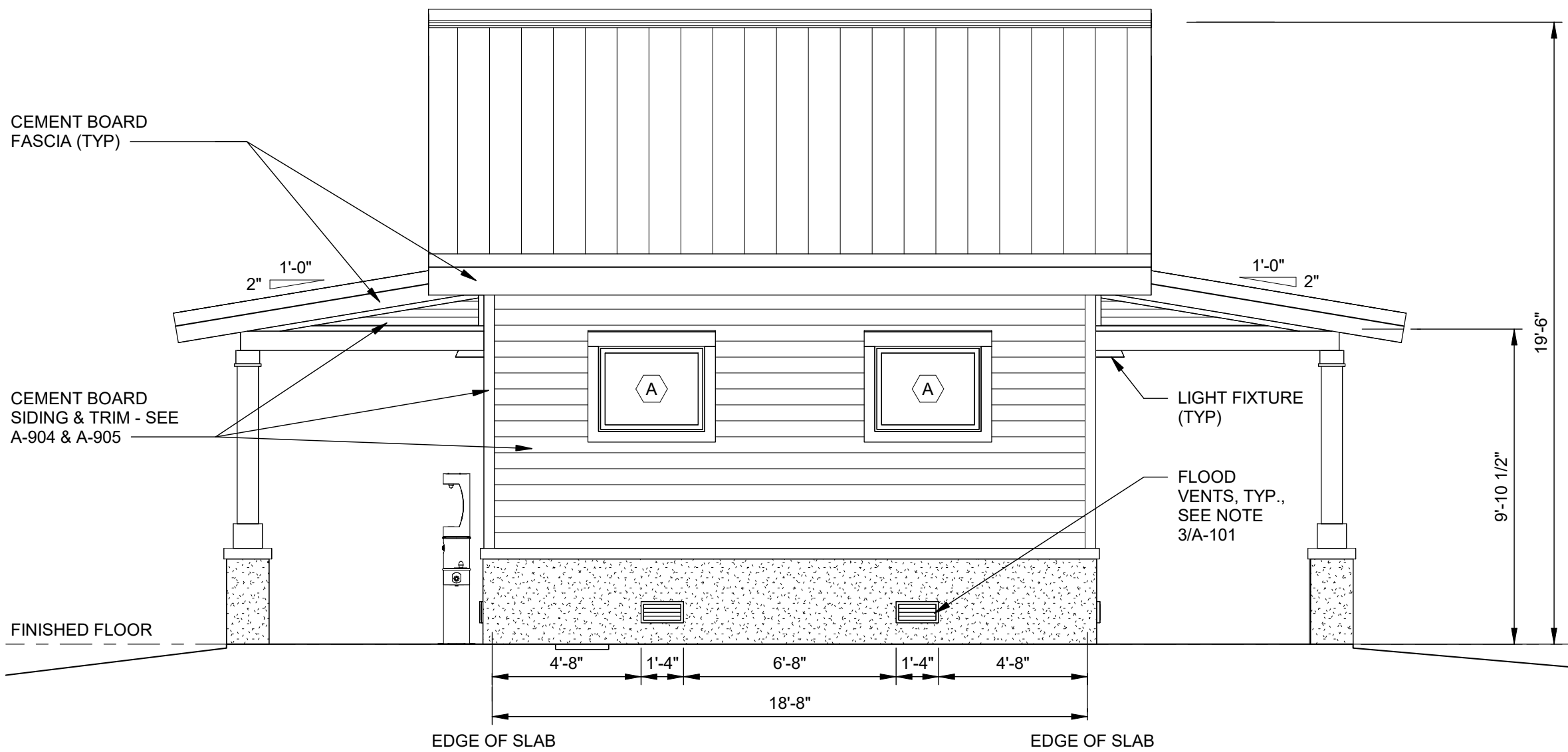
1 A-102 BUILDING 100 - WEST ELEVATION SCALE: 1/4" = 1'-0"
