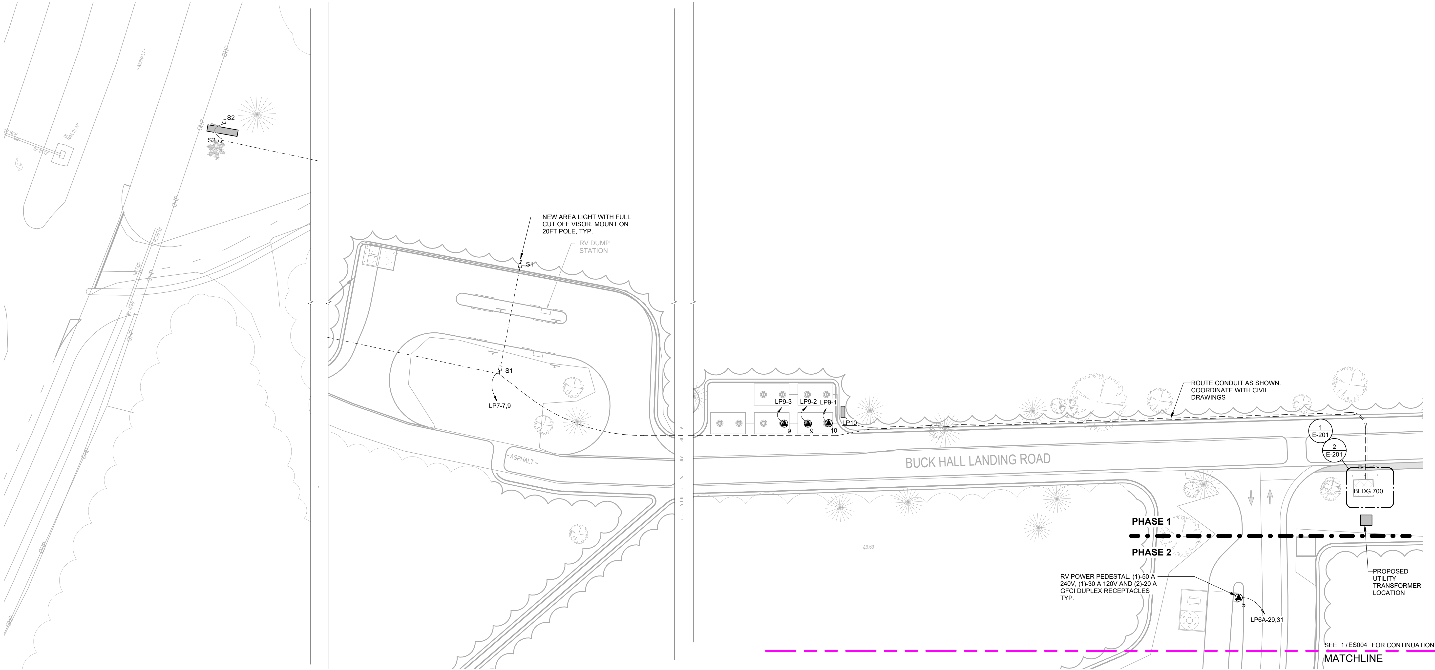
ELECTRICAL SITE PLAN - SHEET 5 ES005 SCALE: 1" = 30'-0"
