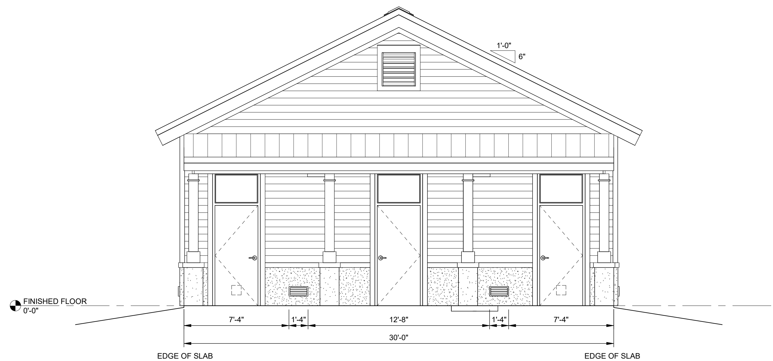
2 BUILDINGS 300/600 ELEVATION A-302 SCALE: 1/4" = 1'-0"
