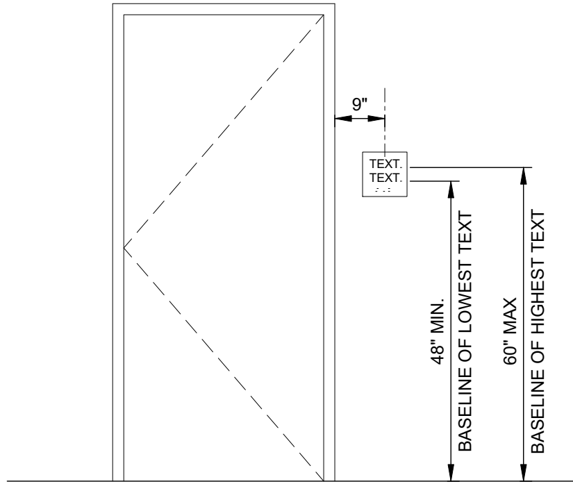
5 SIGN LOCATION DETAIL G-002 SCALE: 1/2" = 1'-0"
