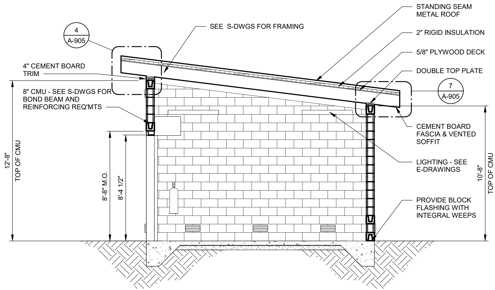
8 BUILDING 400 - SECTION SCALE: 1/4" = 1'-0"
