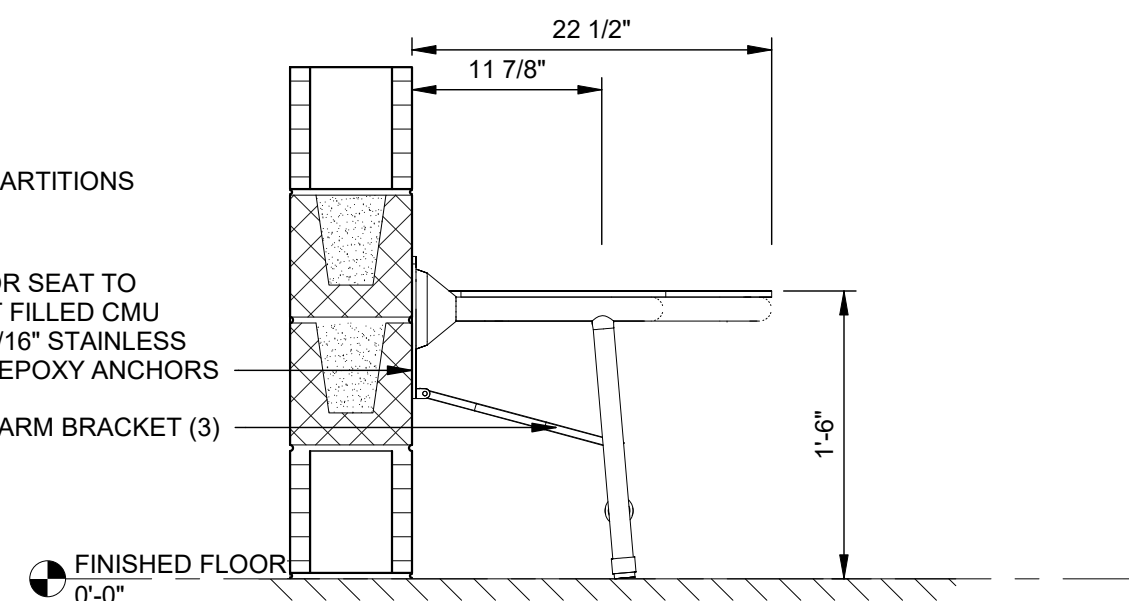
7 FOLDING SHOWER SEAT W/ LEGS A-902 SCALE: 1" = 1'-0"
