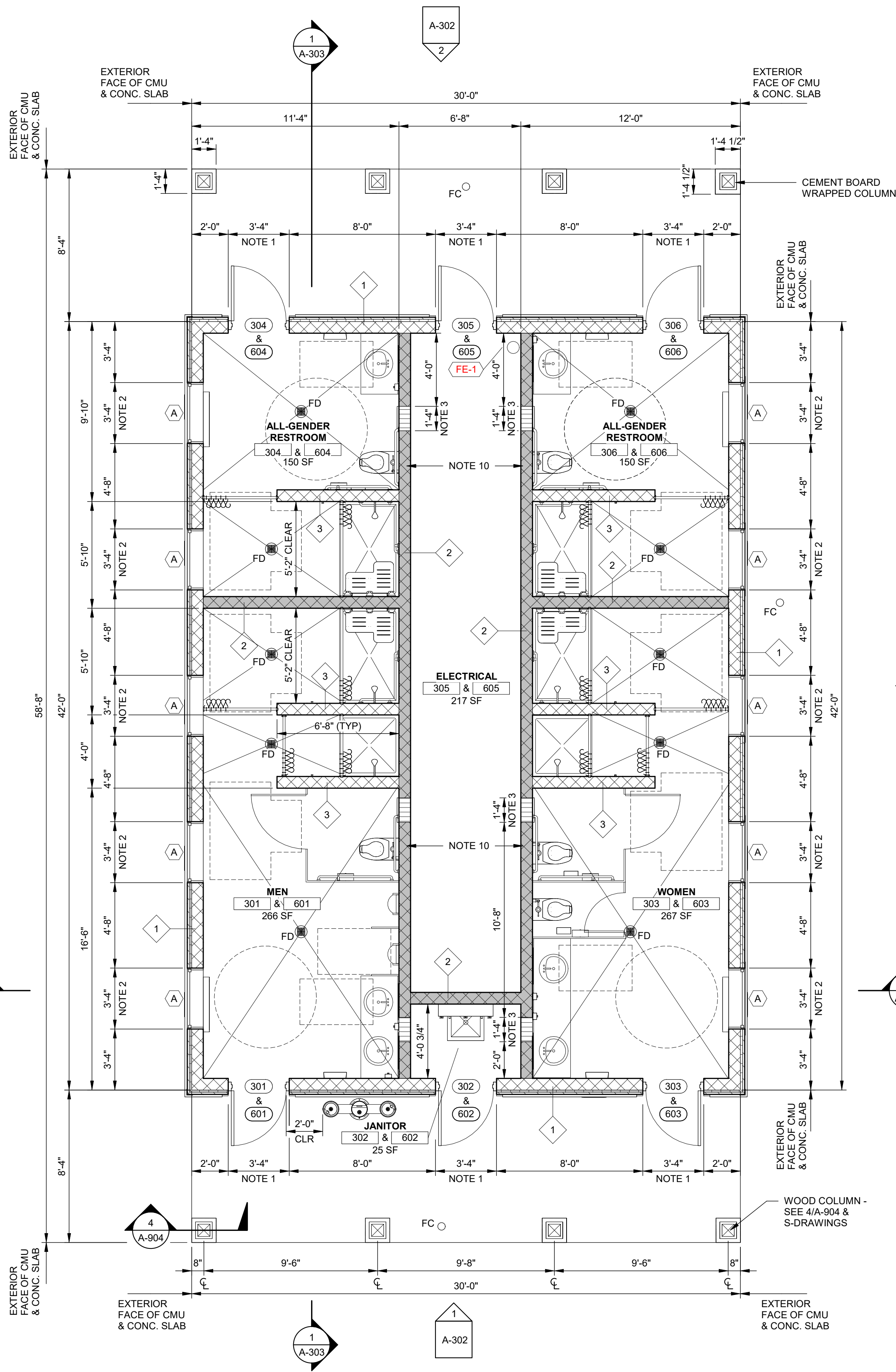
1 BUILDINGS 300/600 - FLOOR PLAN SCALE: 1/4" = 1'-0"
