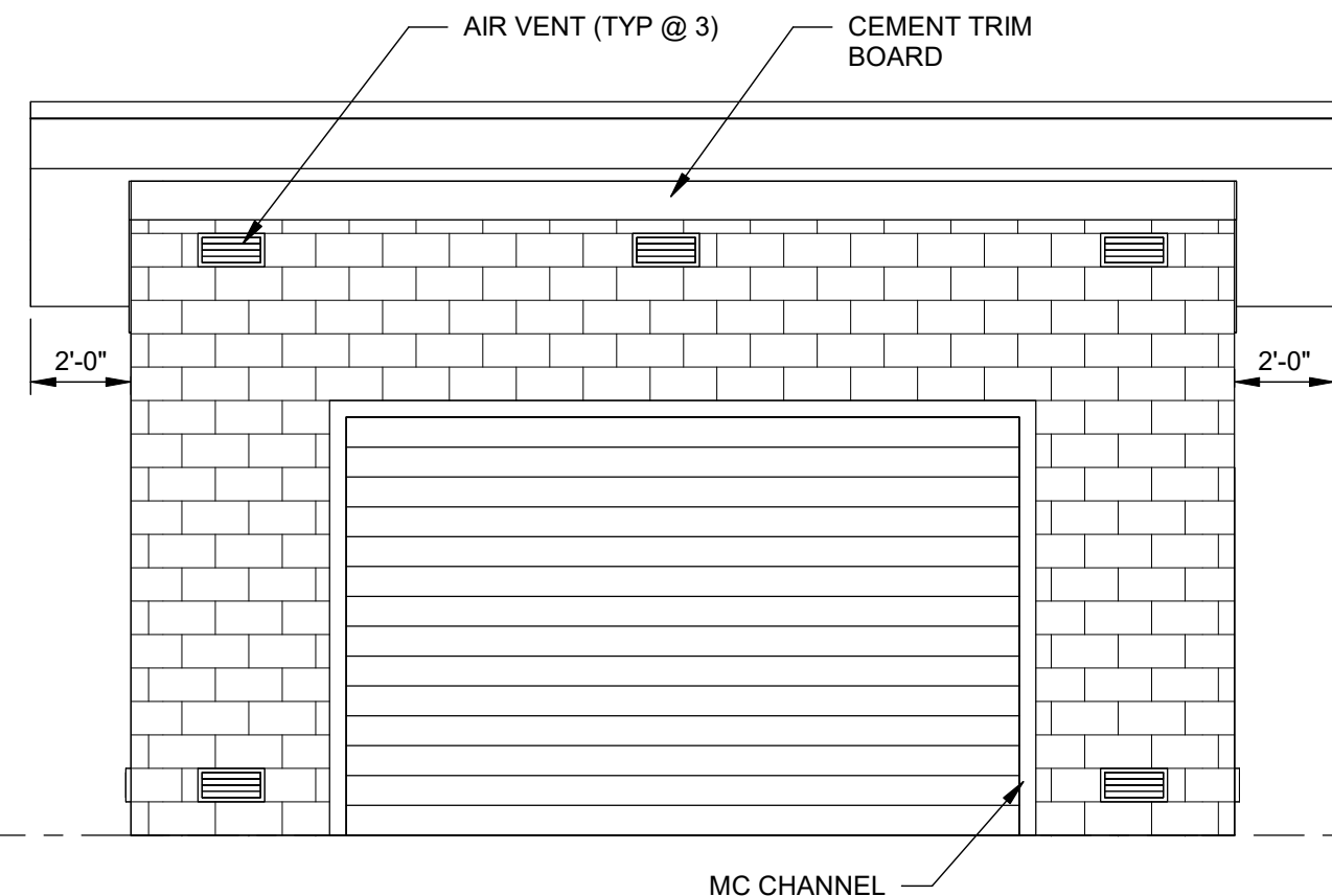
5 BUILDING 400 - EAST ELEVATION SCALE: 1/4" = 1'-0"
