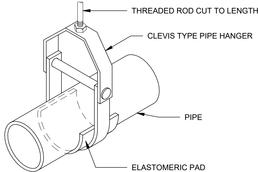
DETAIL - CLEVIS TYPE PIPE SUPPORT FOR NONMETALLIC PIPE NO SCALE
