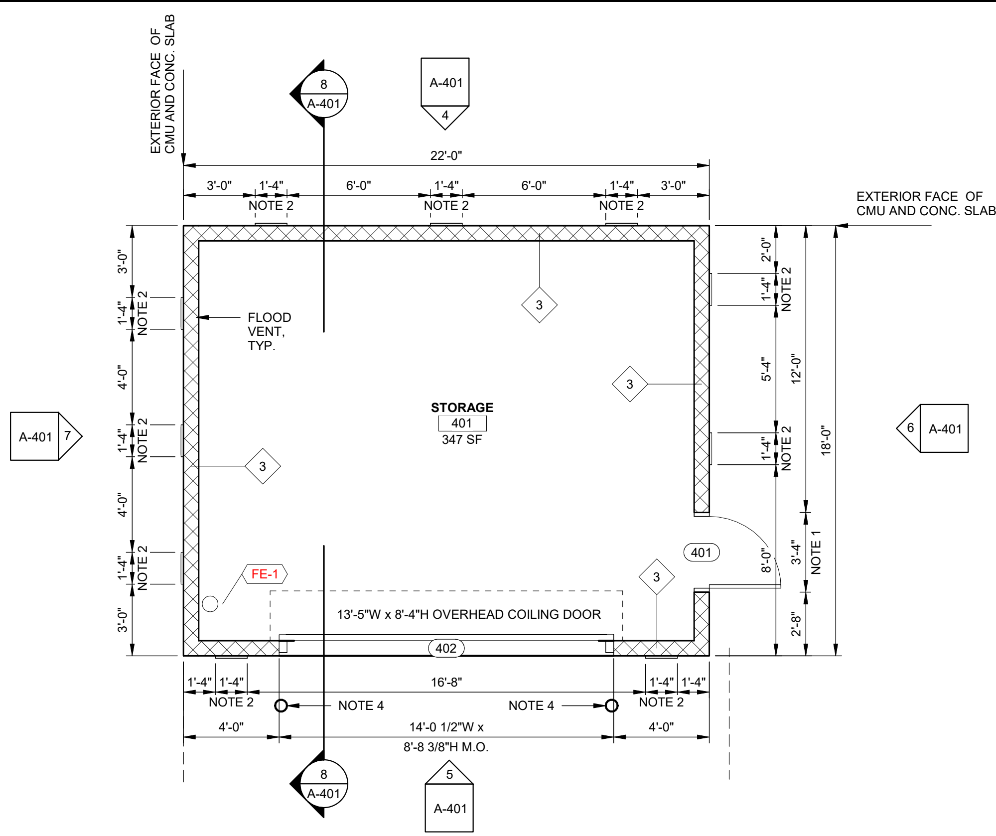
1 BUILDING 400 - FLOOR PLAN SCALE: 1/4" = 1'-0"
