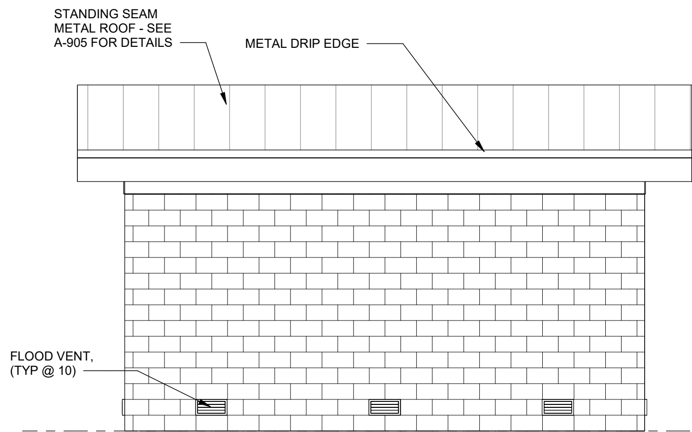
4 BUILDING 400 - WEST ELEVATION SCALE: 1/4" = 1'-0"
