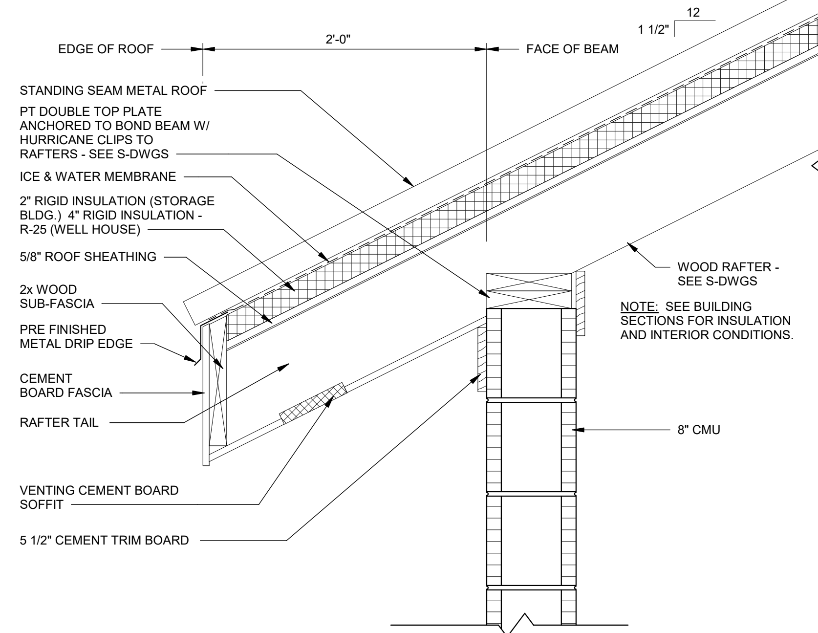
7 BUILDINGS 200, 400 & 700 - EAVE DETAIL A-905 SCALE: 1 1/2" = 1'-0"
