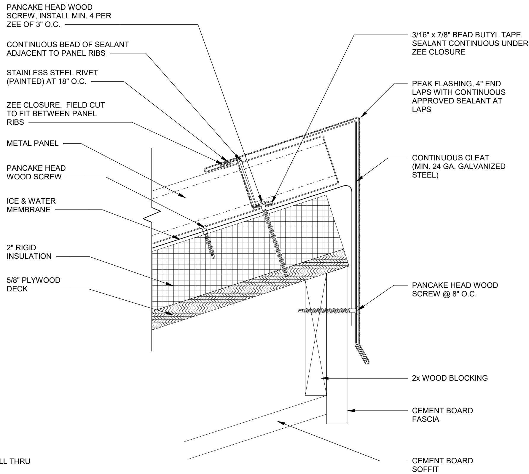
4 BUILDINGS 200, 400 & 700 - HIGH EAVE A-905 SCALE: 6" = 1'-0"
