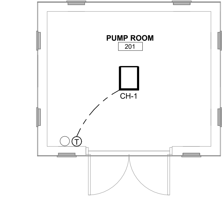
1 M-201 BUILDING 200/700 HVAC PLAN SCALE: 1/4" = 1'-0"
