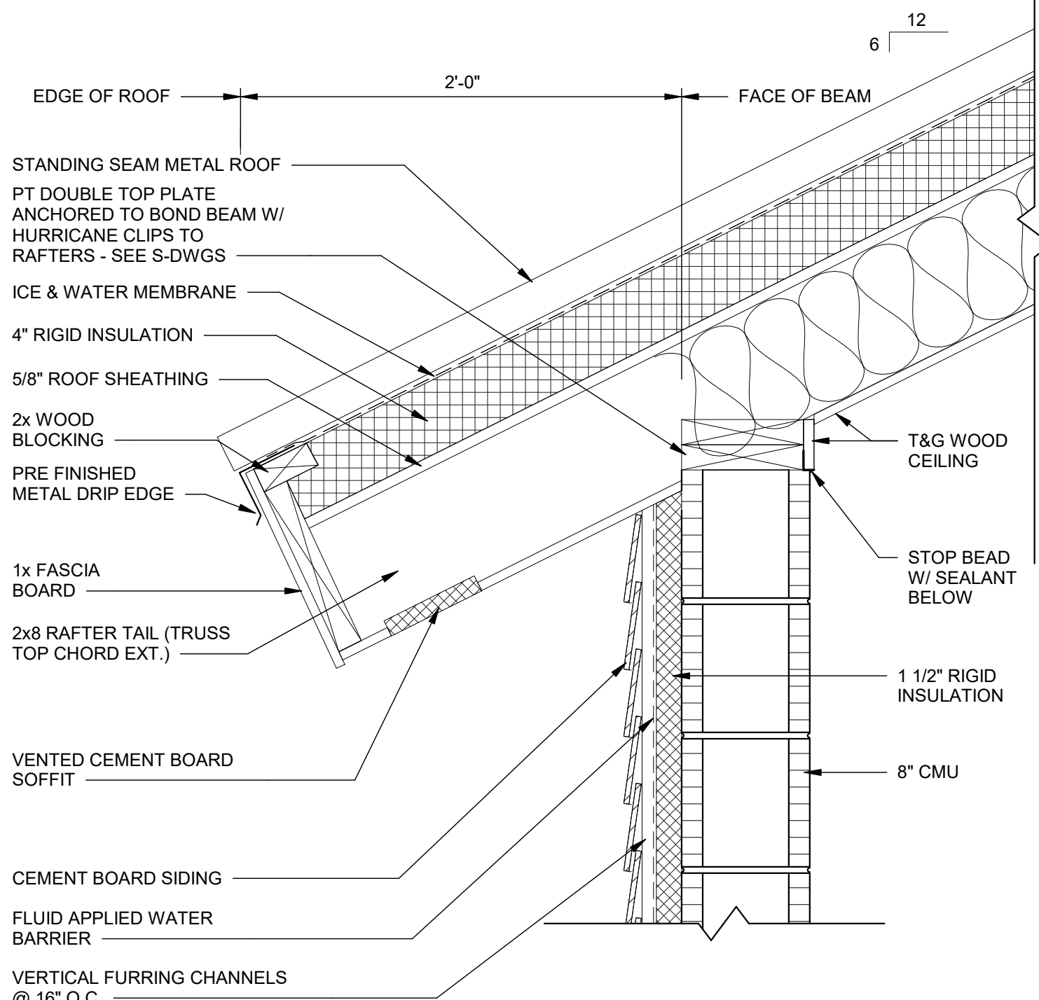
6 BUILDINGS 100, 300 & 600 - EAVE DETAIL A-905 SCALE: 1 1/2" = 1'-0"
