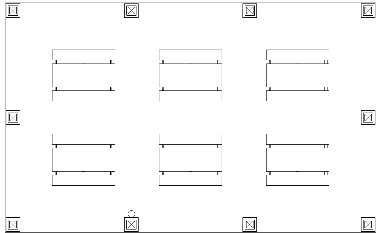
5 BUILDING 500 - FINISH PLAN A-902 SCALE: 3/16" = 1'-0"
