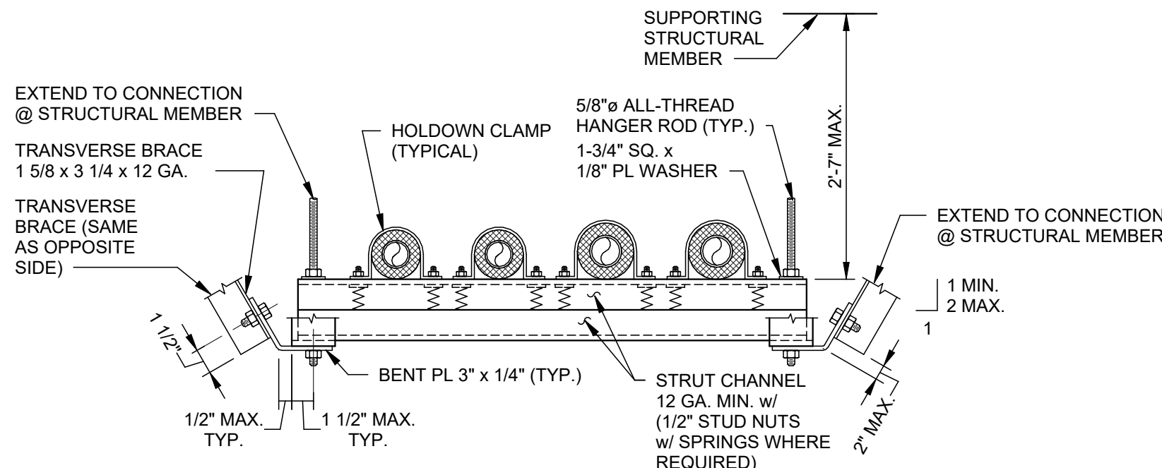
DETAIL - PIPE HANGER TRAPEZE NO SCALE
