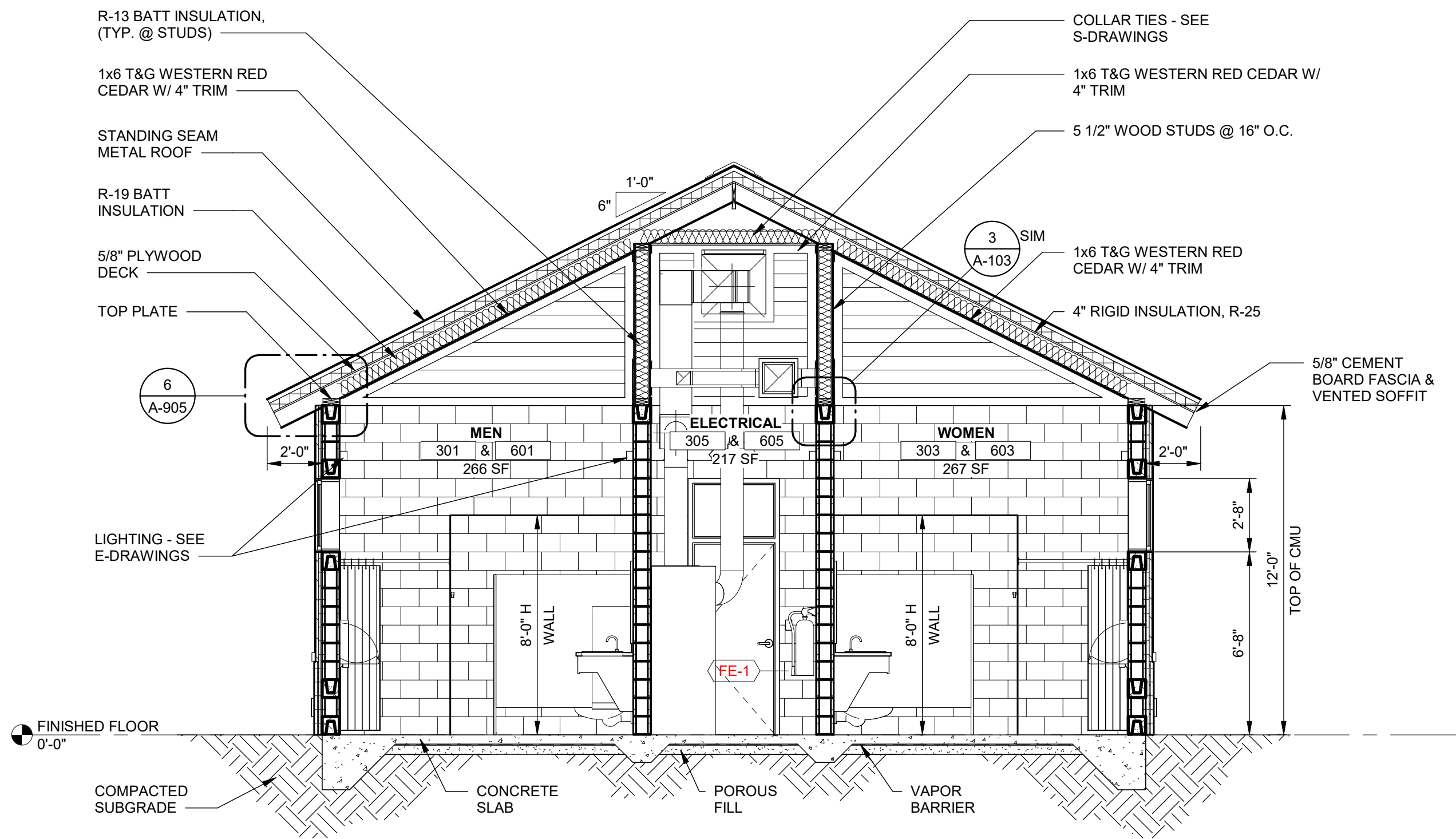
2 BUILDINGS 300/600 - TRANSVERSE SECTION A-303 SCALE: 1/4" = 1'-0"
