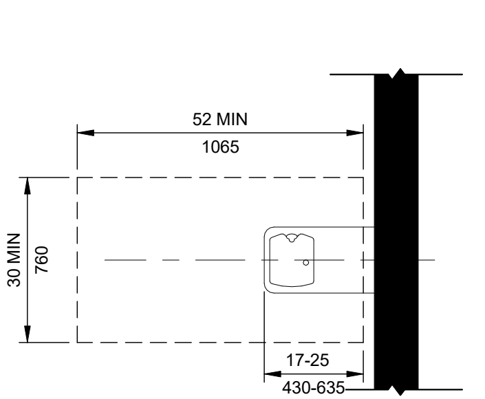
FIGURE 602.2.1(A) CLEAR FLOOR SPACE AT WHEELCHAIR DRINKING FOUNTAINS
