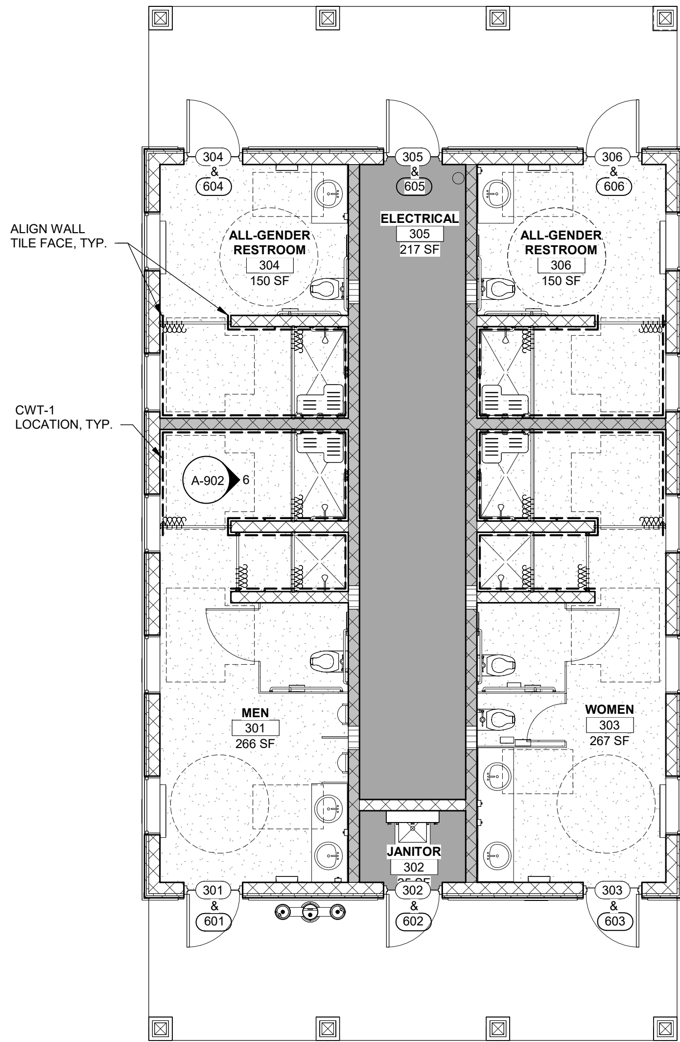
4 BUILDINGS 300/600 - FINISH PLAN A-902 SCALE: 3/16" = 1'-0"
