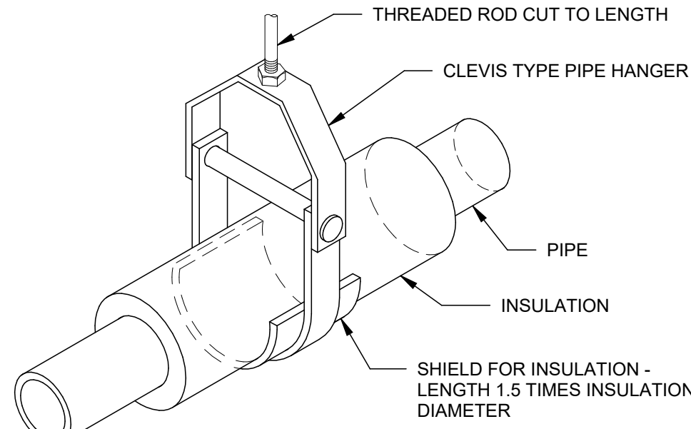
DETAIL - CLEVIS TYPE PIPE SUPPORT FOR INSULATED PIPE NO SCALE
