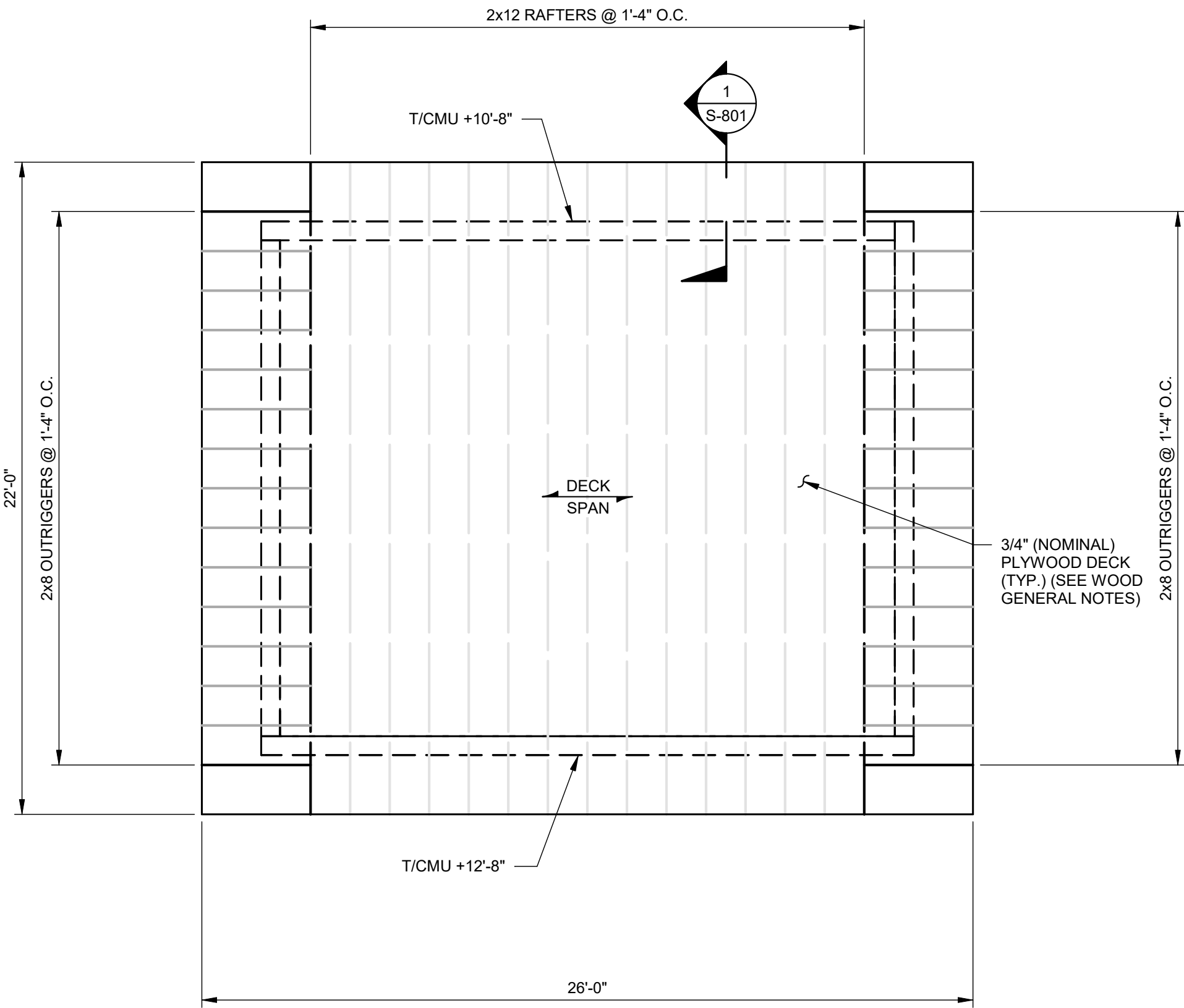
2 S-401 BUILDING 400 - FRAMING PLAN SCALE: 1/4" = 1'-0"
