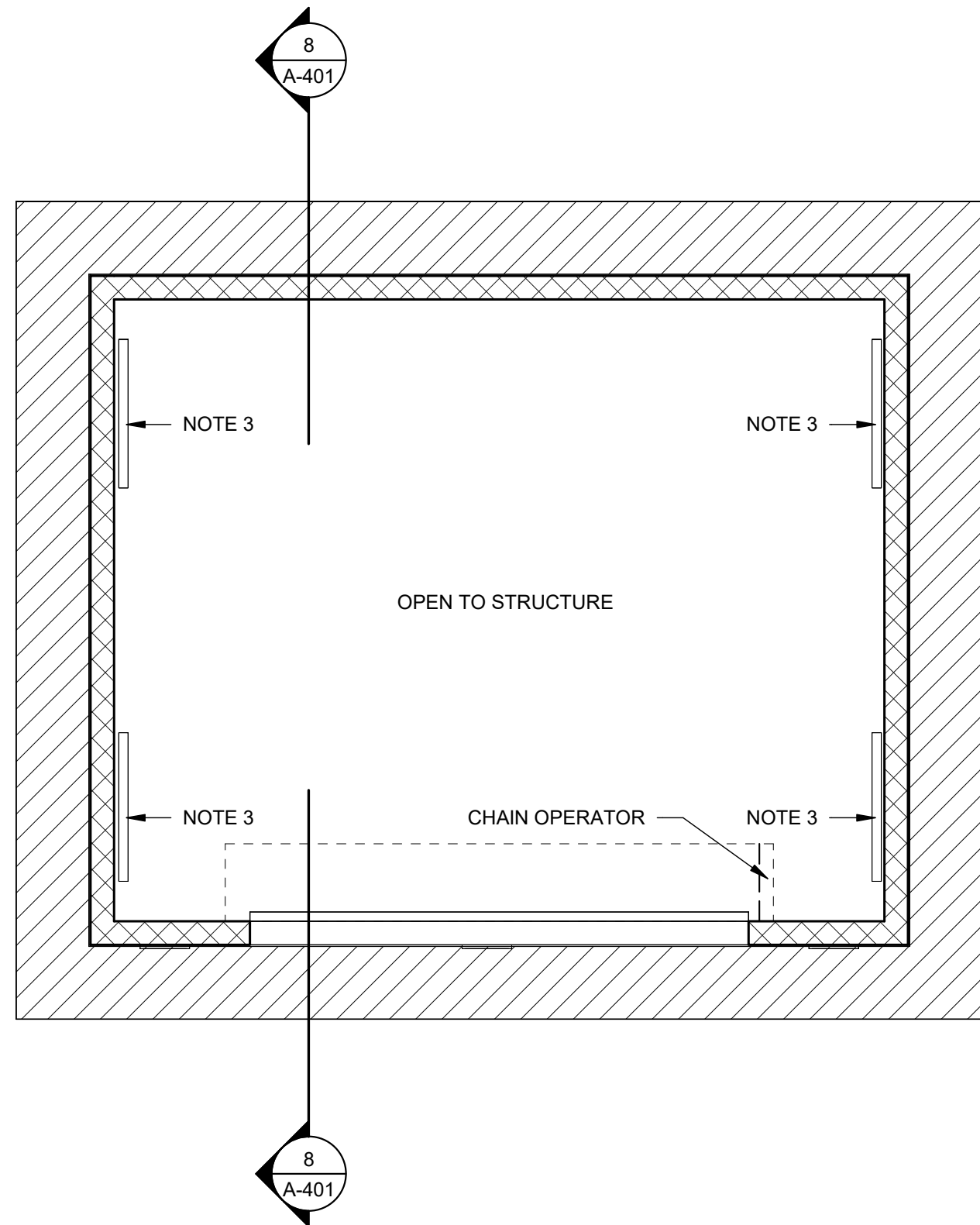
2 BUILDING 400 - REFLECTED CEILING PLAN SCALE: 1/4" = 1'-0"
