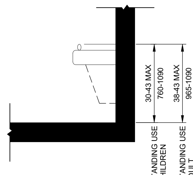
FIGURE 602.3.2 STANDING USE DRINKING FOUNTAIN SPOUT HEIGHT AND LOCATION
