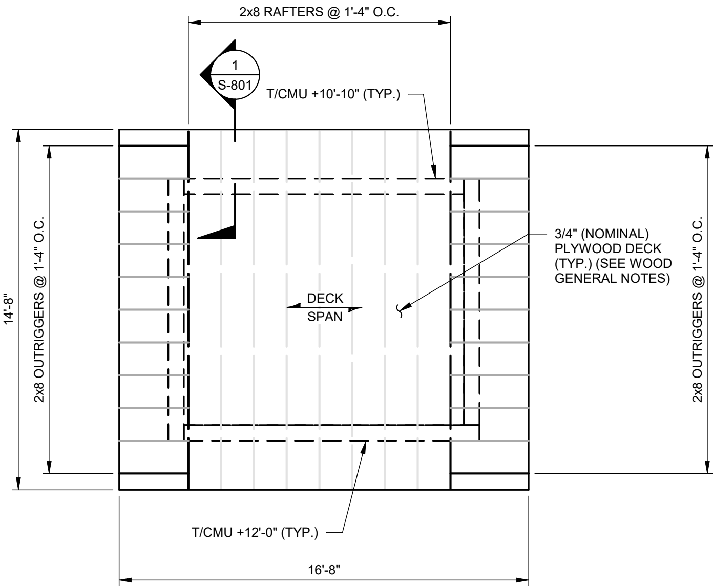
2 BUILDING 200/700 - FRAMING PLAN S-201 SCALE: 1/4" = 1'-0"
