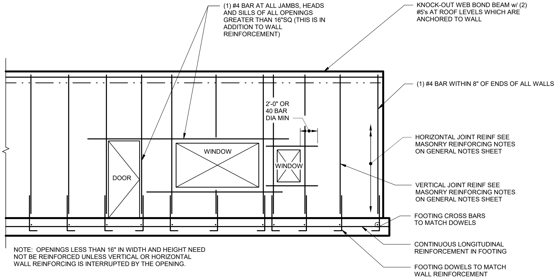
DETAIL SCALE: 3/16" = 1'-0"
