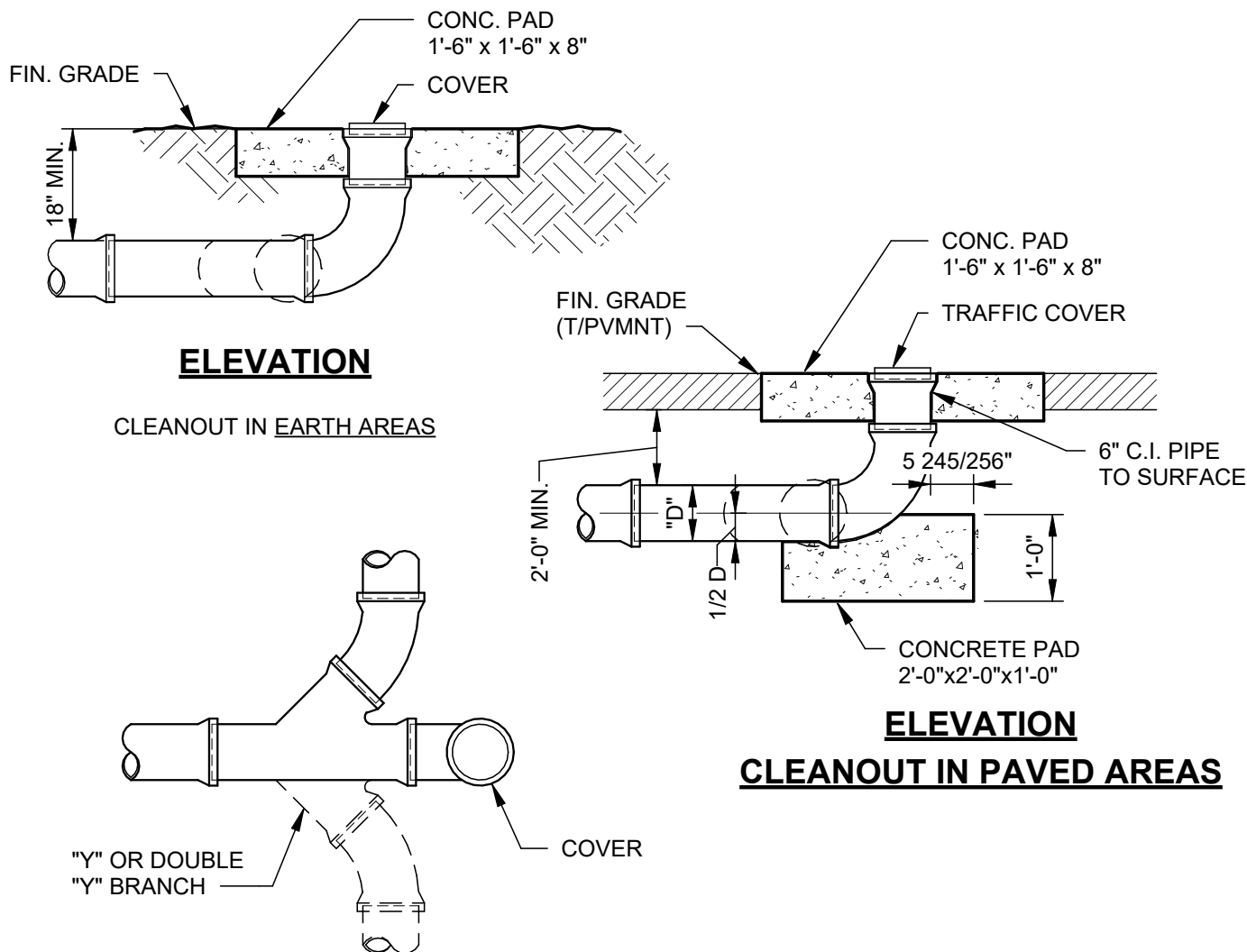
GROUND CLEANOUT DETAILS NO SCALE
