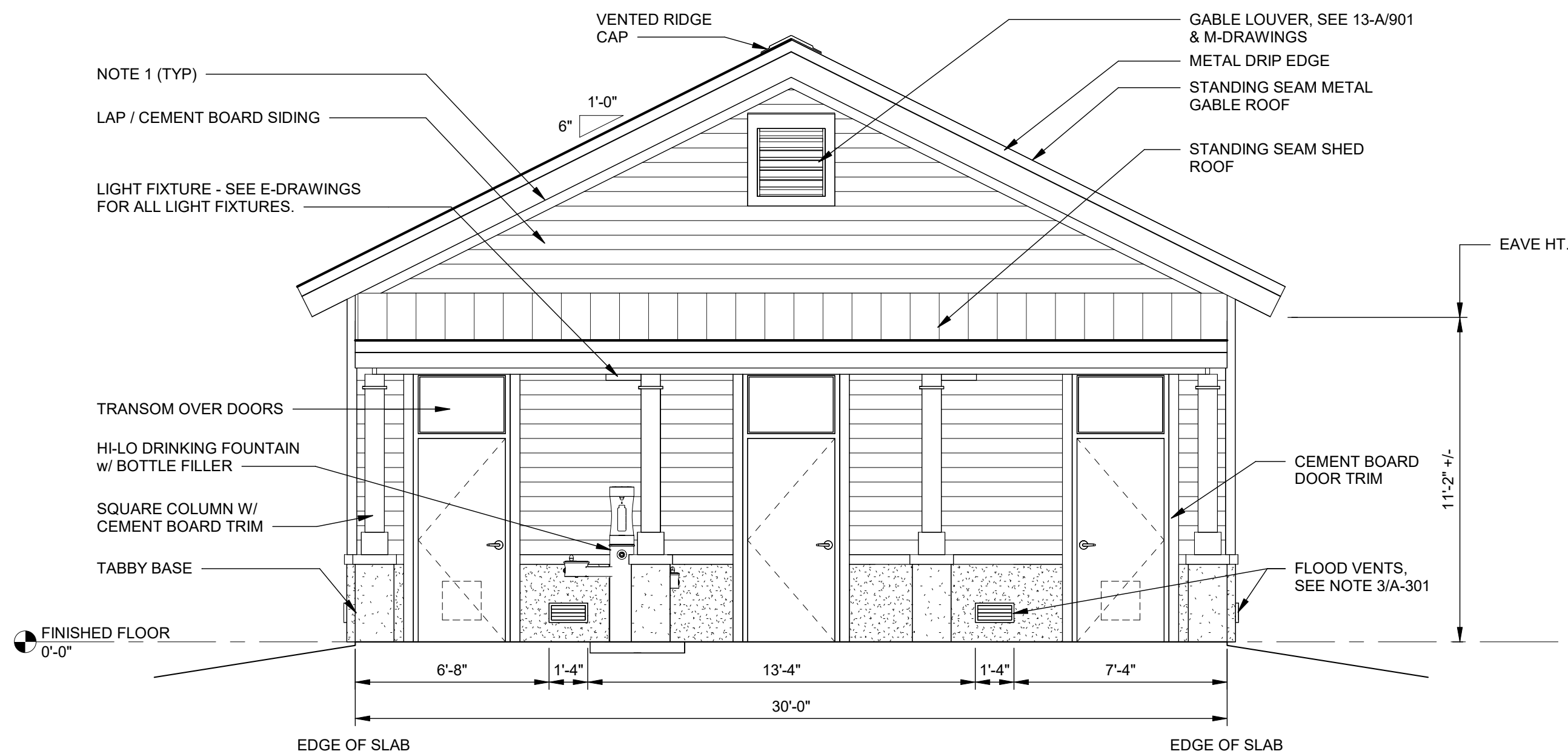
1 BUILDINGS 300/600 ELEVATION A-302 SCALE: 1/4" = 1'-0"
