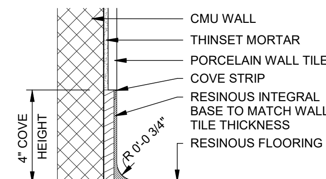
8 WALL BASE DETAIL @ WALL TILE A-902 SCALE: 3" = 1'-0"
