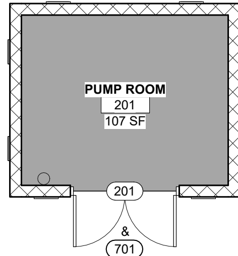
2 BUILDINGS 200/700 - FINISH PLAN A-902 SCALE: 3/16" = 1'-0"
