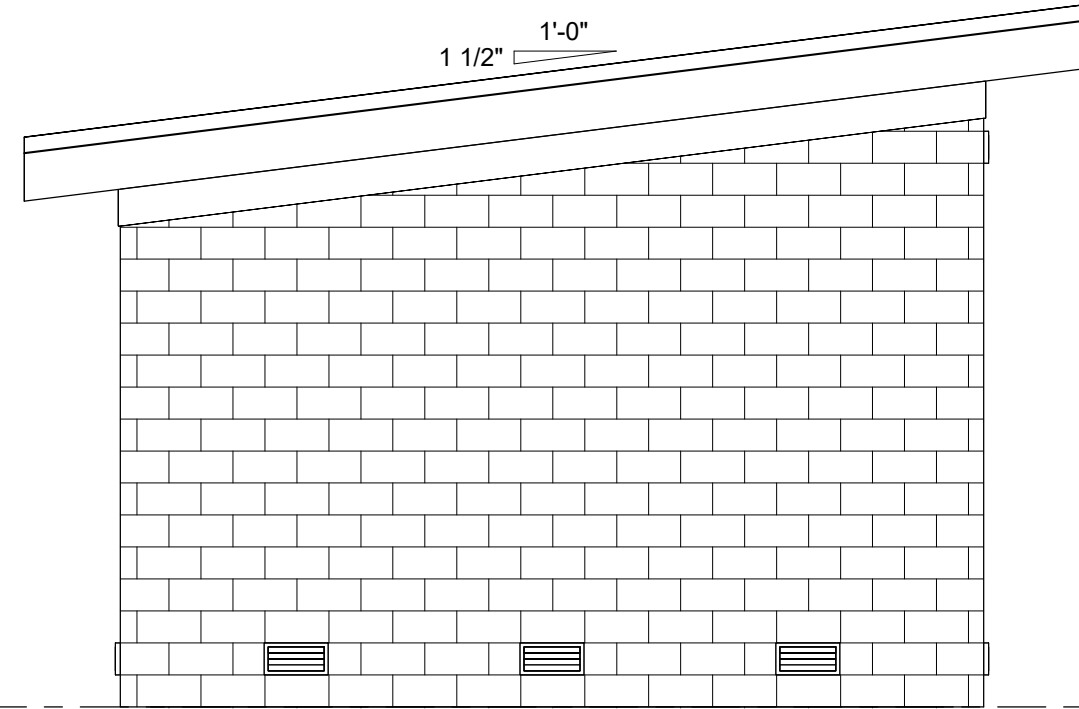
7 BUILDING 400 - SOUTH ELEVATION SCALE: 1/4" = 1'-0"
