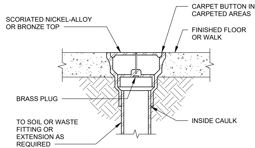
DETAIL - FLOOR CLEANOUT NO SCALE
