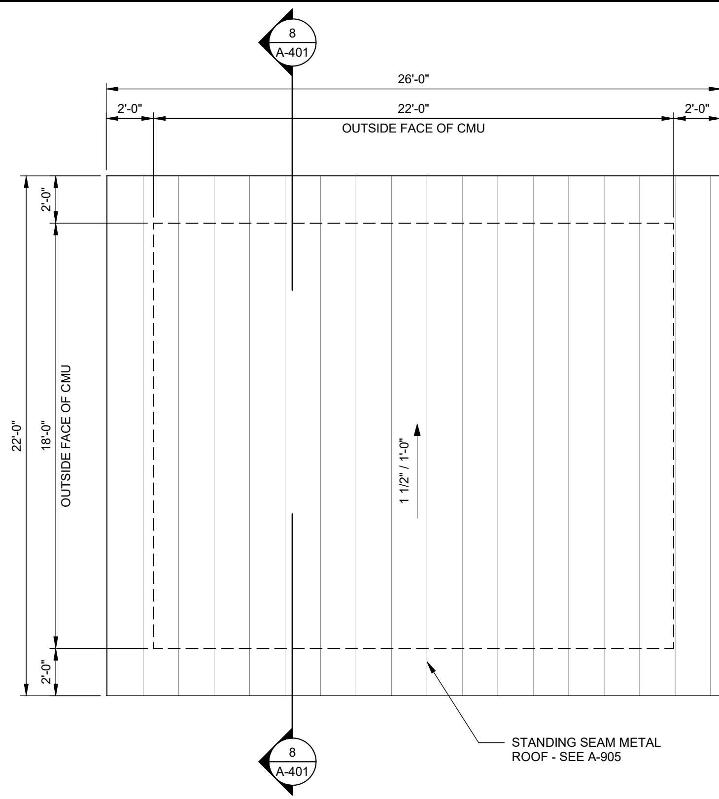
3 BUILDING 400 - ROOF PLAN SCALE: 1/4" = 1'-0"
