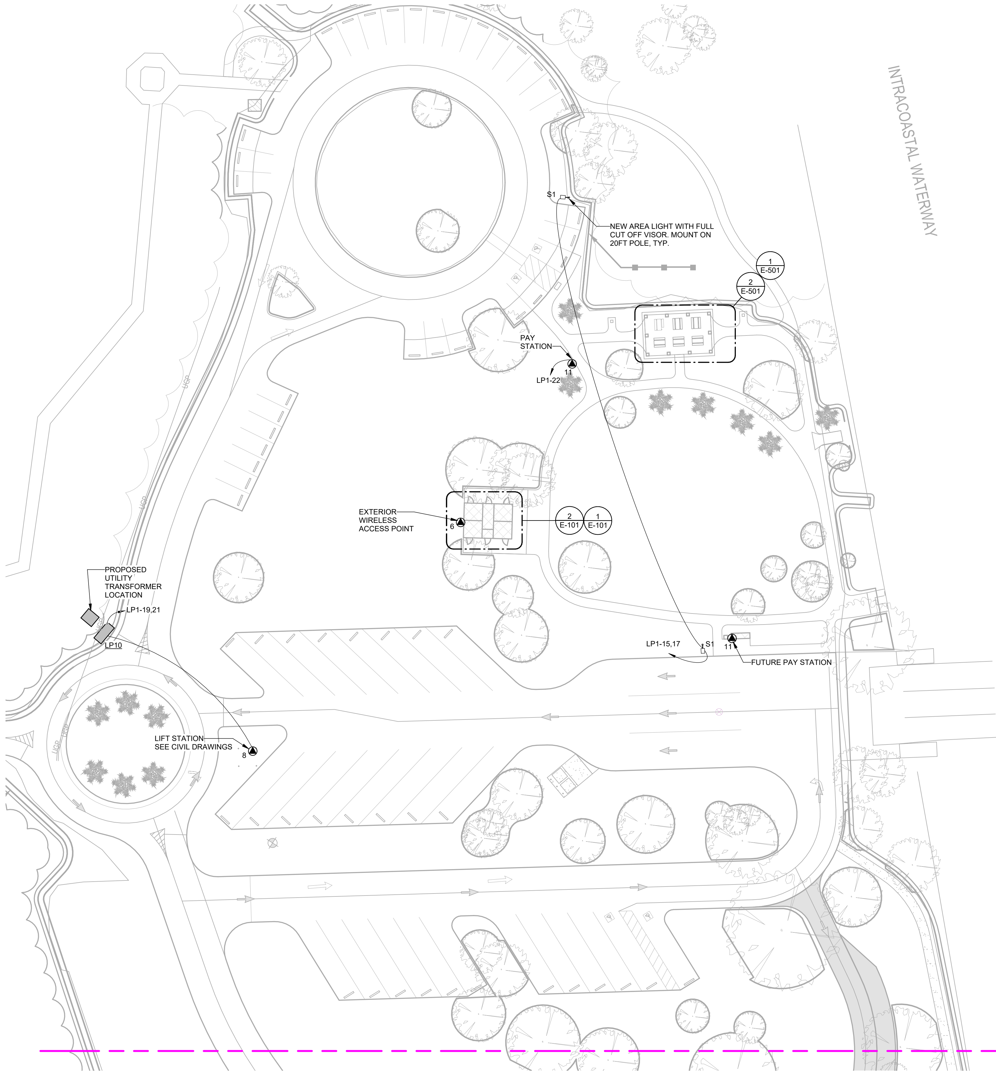
ELECTRICAL SITE PLAN - SHEET 1 SCALE: 1" = 30'-0"
