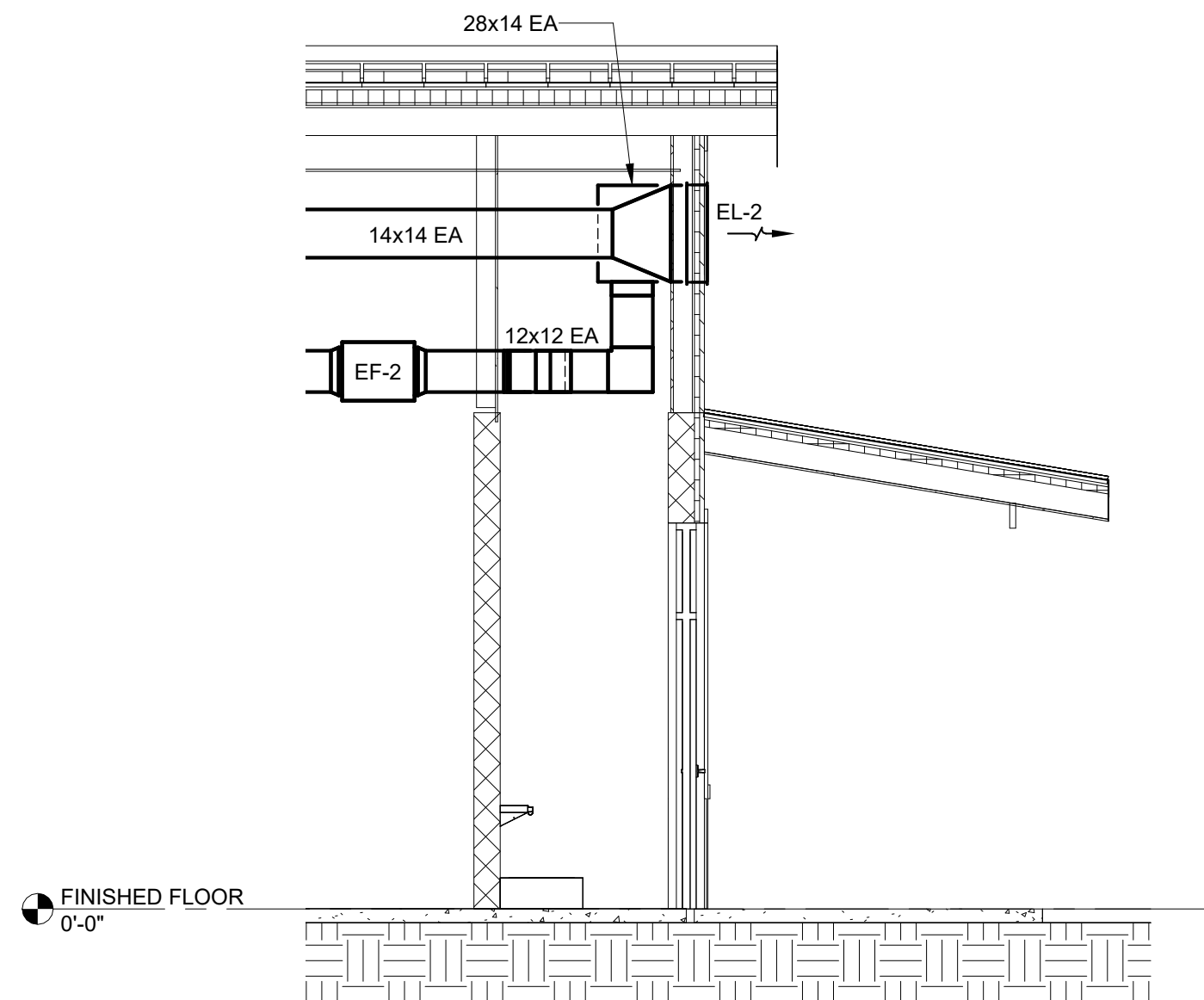
3 EXHAUST LOUVER DUCTWORK ELEVATION SCALE: 1/4" = 1'-0"
