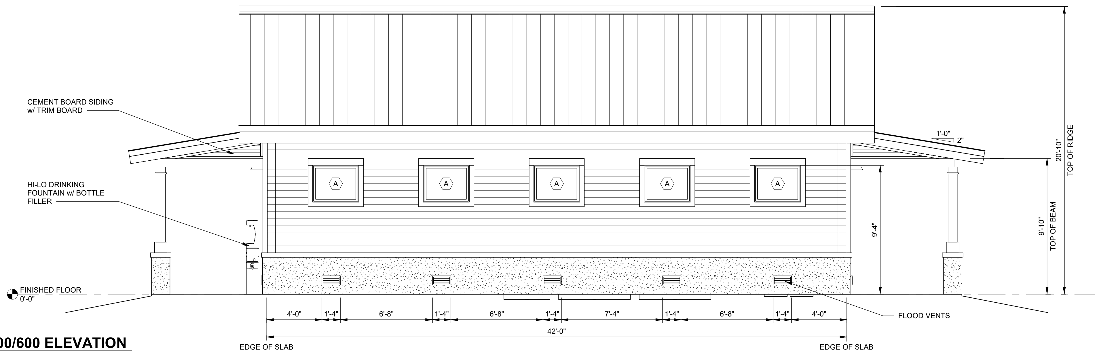
3 BUILDINGS 300/600 ELEVATION A-302 SCALE: 1/4" = 1'-0"
