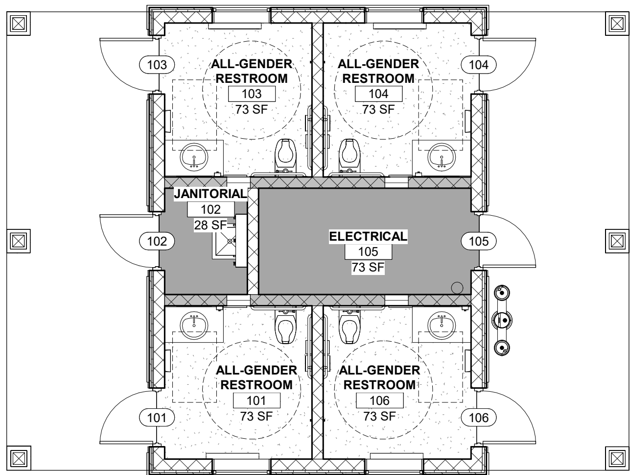
1 BUILDING 100 - FINISH PLAN A-902 SCALE: 3/16" = 1'-0"
