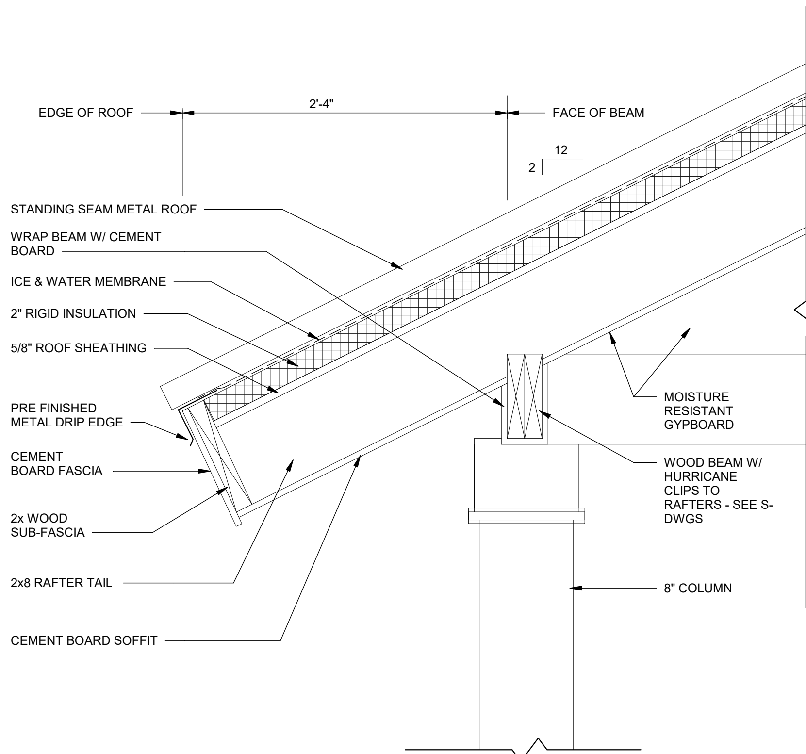
5 BUILDINGS 100, 300, 500 & 600 - EAVE DETAIL @ PORCH A-905 SCALE: 1 1/2" = 1'-0"
