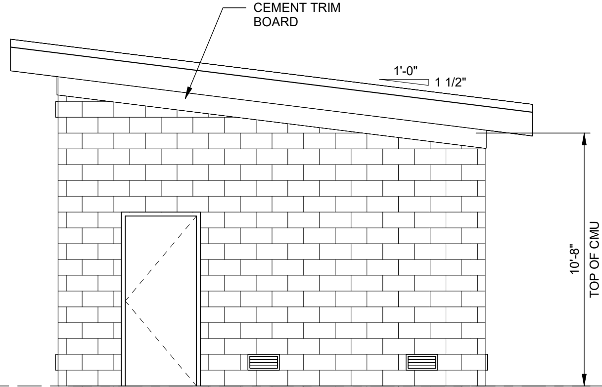
6 BUILDING 400 - NORTH ELEVATION SCALE: 1/4" = 1'-0"
