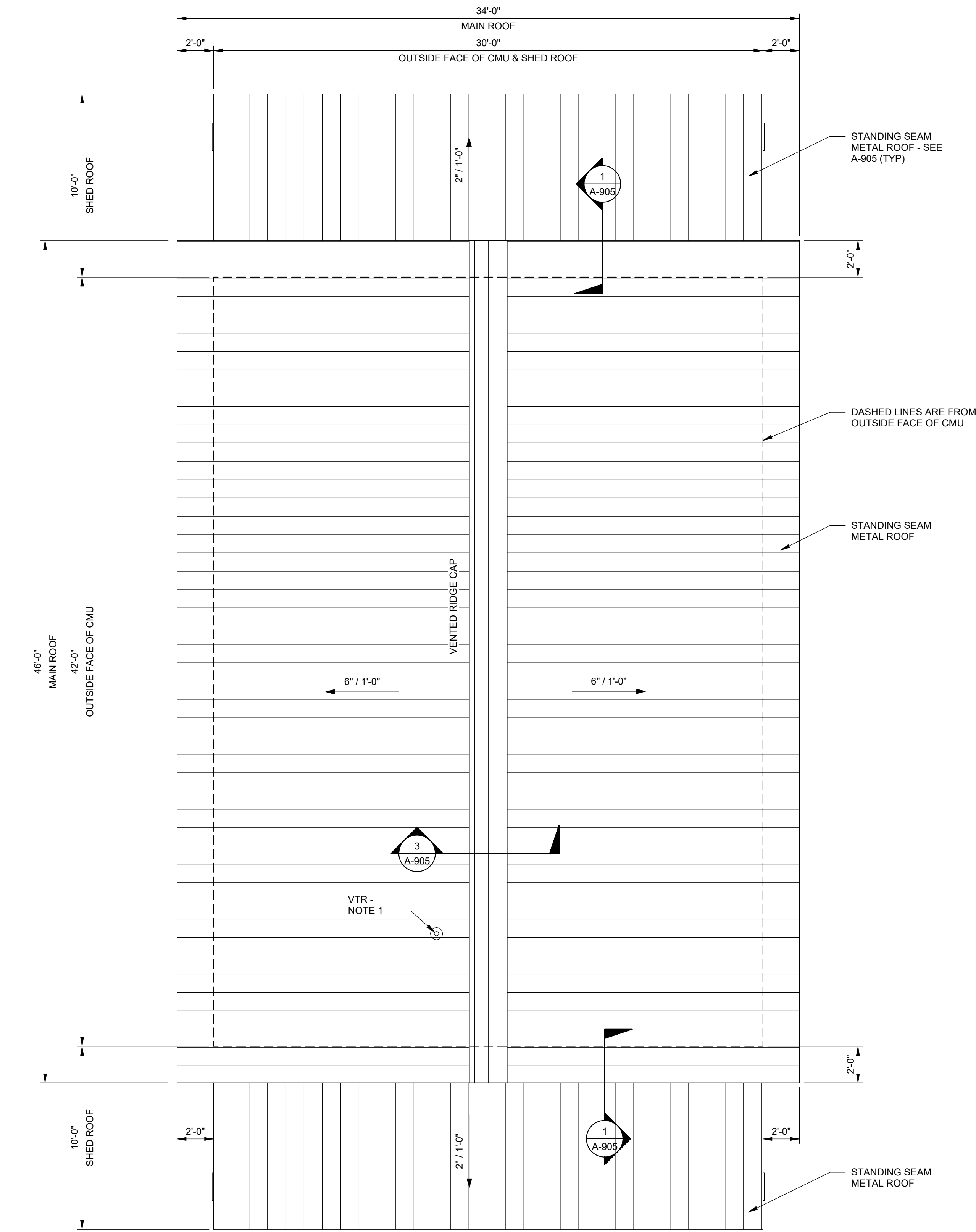
BUILDINGS 300/600 - ROOF PLAN SCALE: 1/4" = 1'-0"
