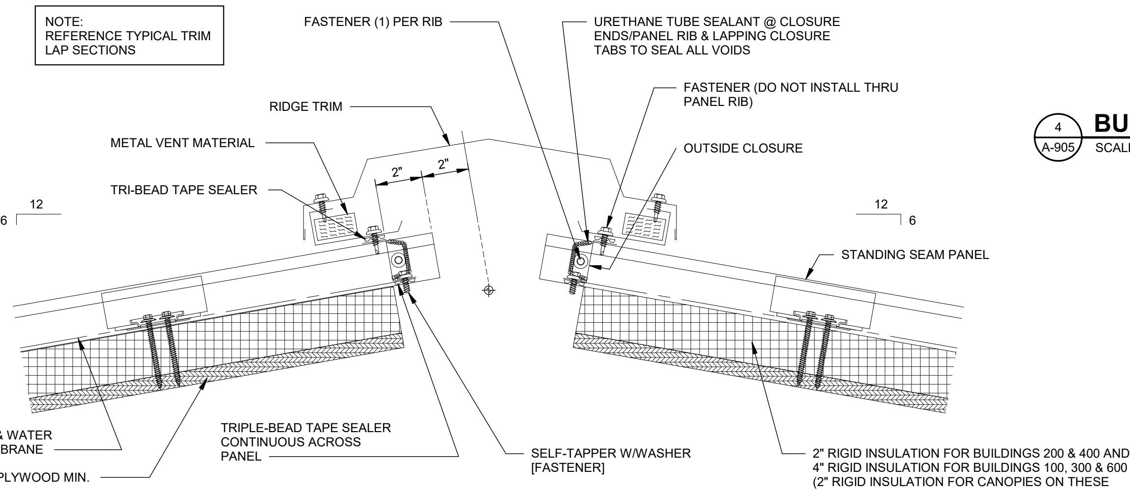
3 LOW FLOATING RIDGE A-905 SCALE: 3" = 1'-0"
