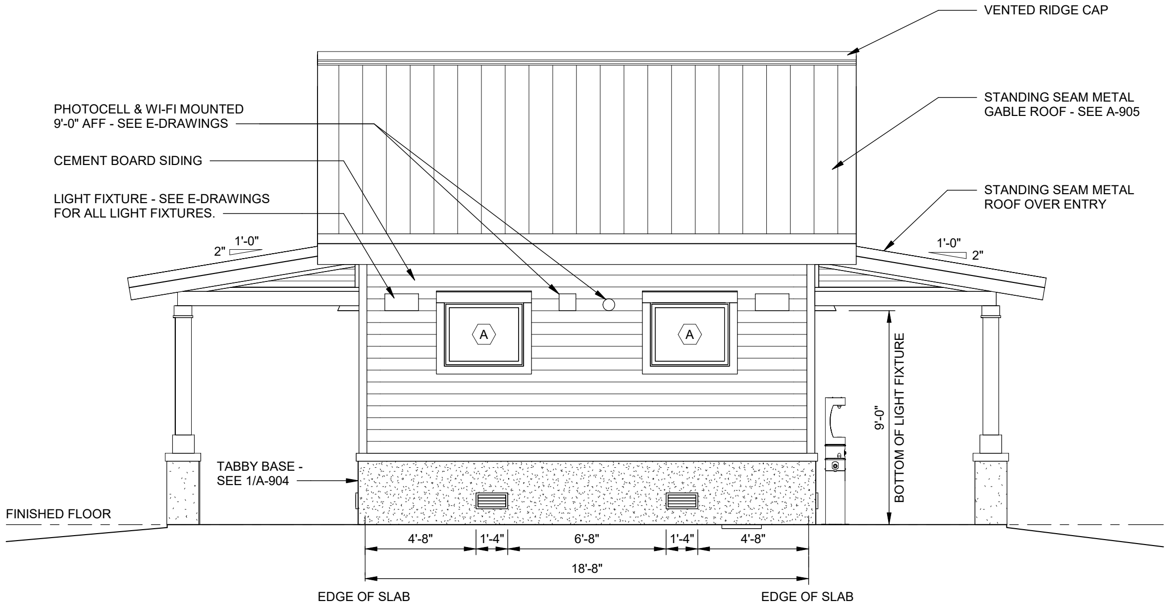
2 A-102 BUILDING 100 - EAST ELEVATION SCALE: 1/4" = 1'-0"
