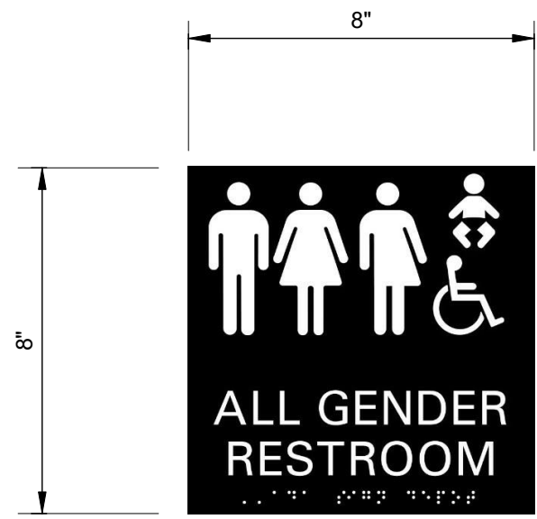
3 ALL GENDER RESTROOM SIGN G-002 SCALE: 3" = 1'-0"
