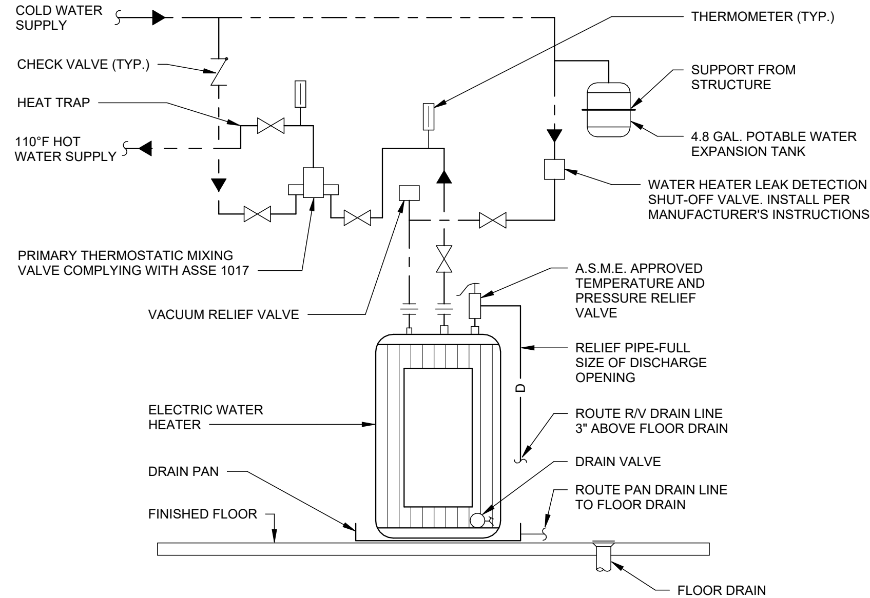
ELECTRIC WATER HEATER SCHEMATIC NO SCALE
