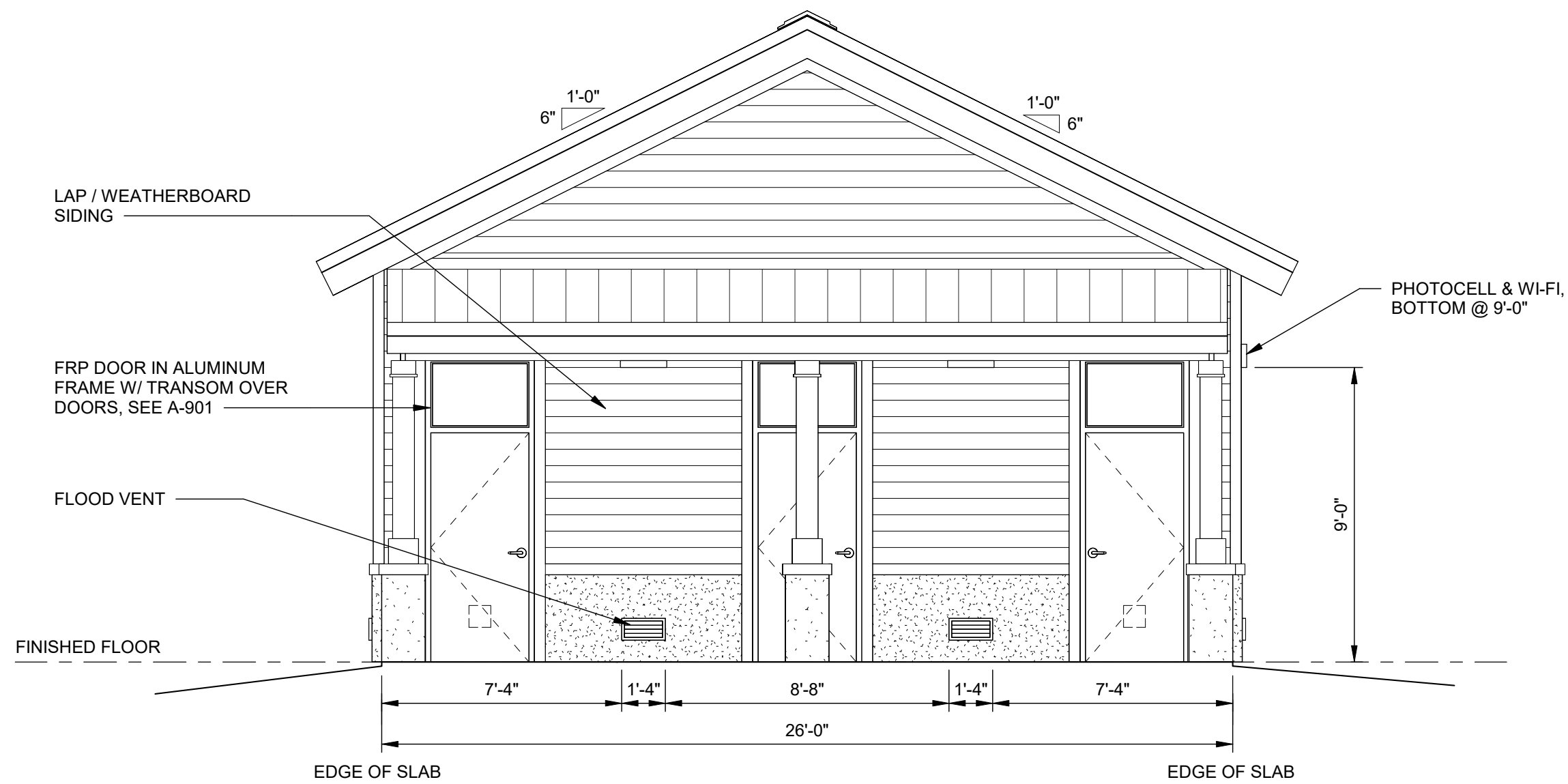
4 A-102 BUILDING 100 - SOUTH ELEVATION SCALE: 1/4" = 1'-0"
