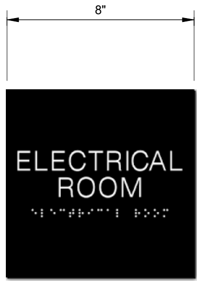
4 ELECTRICAL ROOM SIGN G-002 SCALE: 3" = 1'-0"
