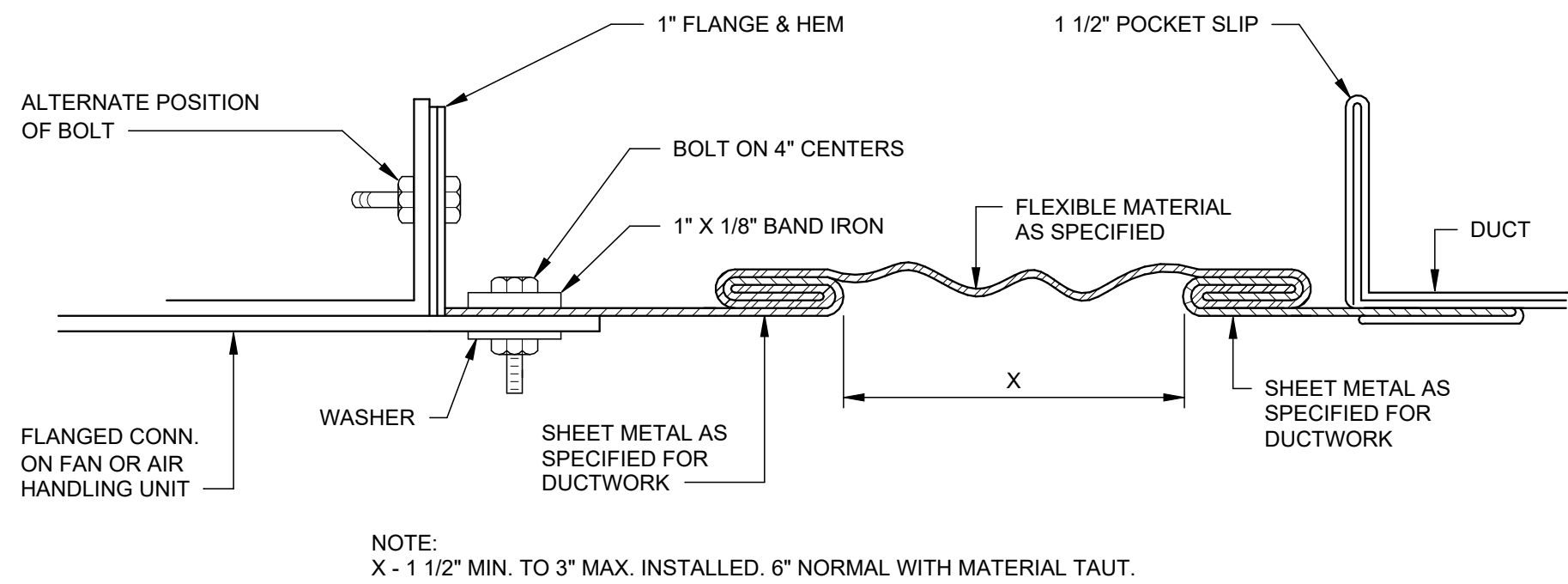
RECTANGULAR FLEXIBLE CONNECTION DETAIL NO SCALE
