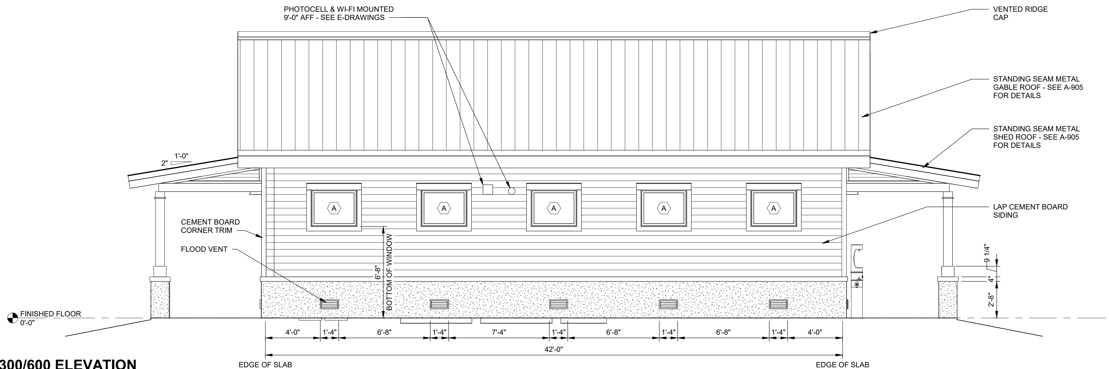
4 BUILDINGS 300/600 ELEVATION A-302 SCALE: 1/4" = 1'-0"
