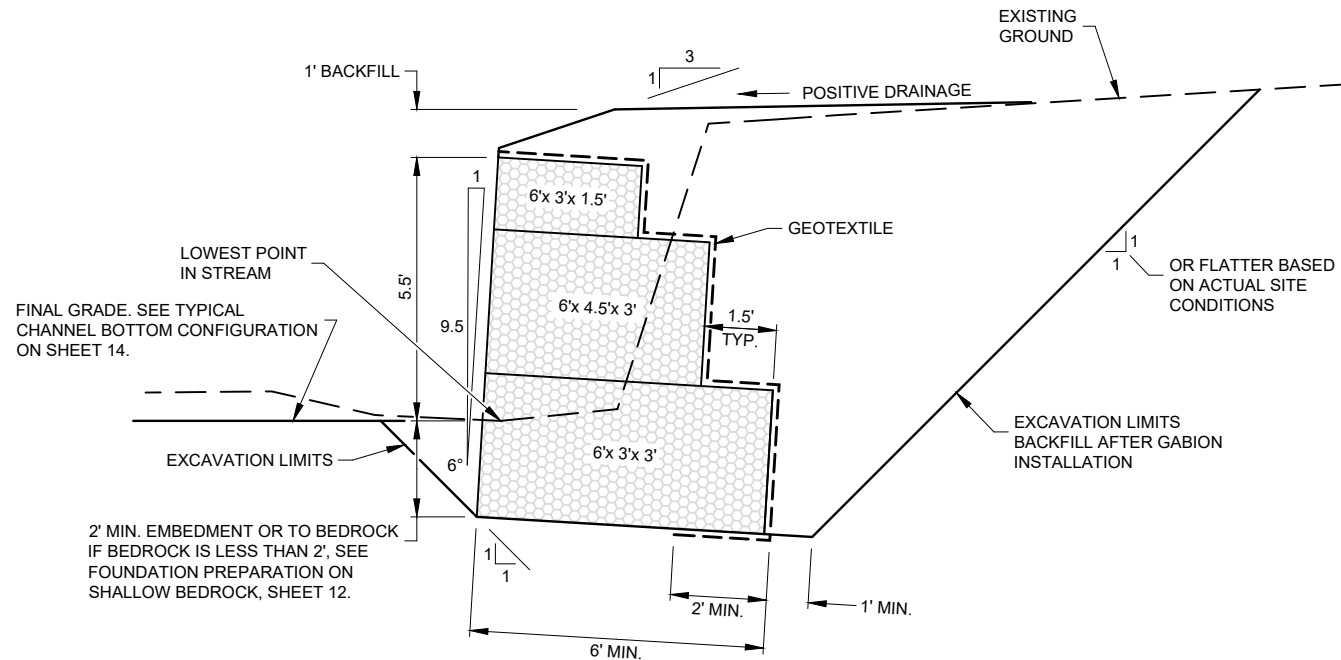
SECTION - 7.5' HIGH GABION WALL
