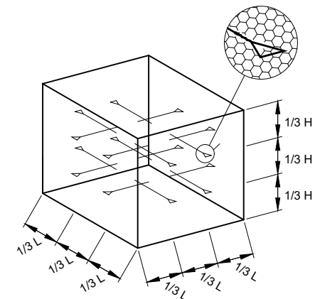
INTERIOR SUPPORT DETAIL
