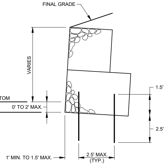
SECTION - GABIONS WITH REBAR SPACING
