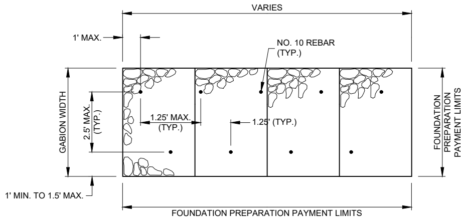
PLAN - GABIONS WITH REBAR/DRILLHOLE PATTERN
