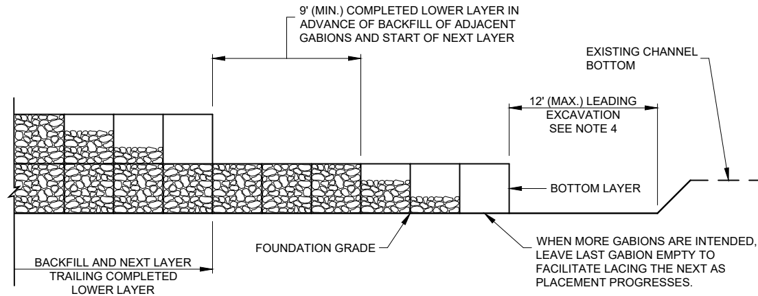
PROFILE - GABION PLACEMENT/FILLING SEQUENCE
