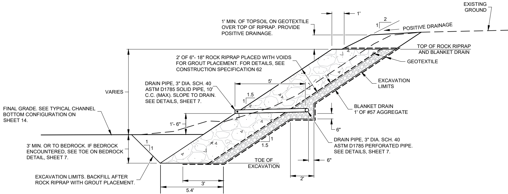
SECTION - GROUTED ROCK RIPRAP
