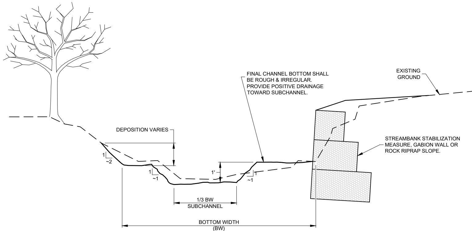
CHANNEL BOTTOM CONFIGURATION SEE SITE PLAN
