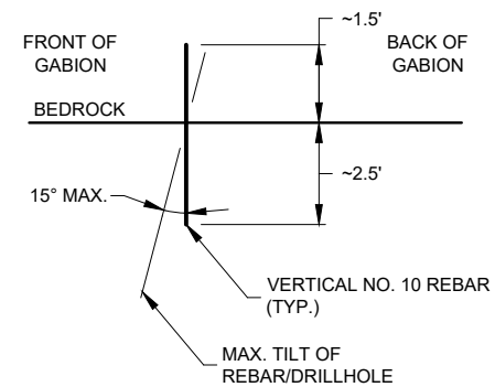
MAXIMUM ANGLE OF REBAR/DRILLHOLE PATTERN
