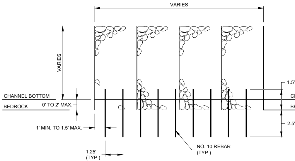
PROFILE - GABIONS WITH REBAR SPACING
