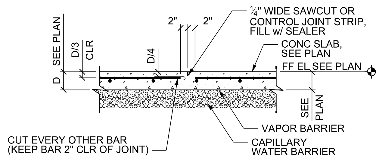
SLAB CONTRACTION JOINT (CJ)
