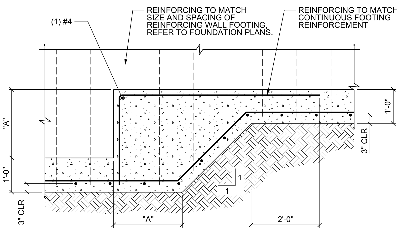
STEP FOOTING
