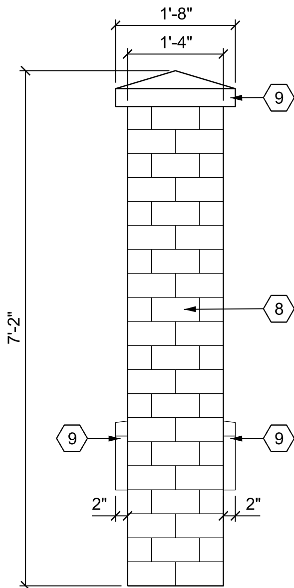
SIDE ELEVATION NOT TO SCALE
