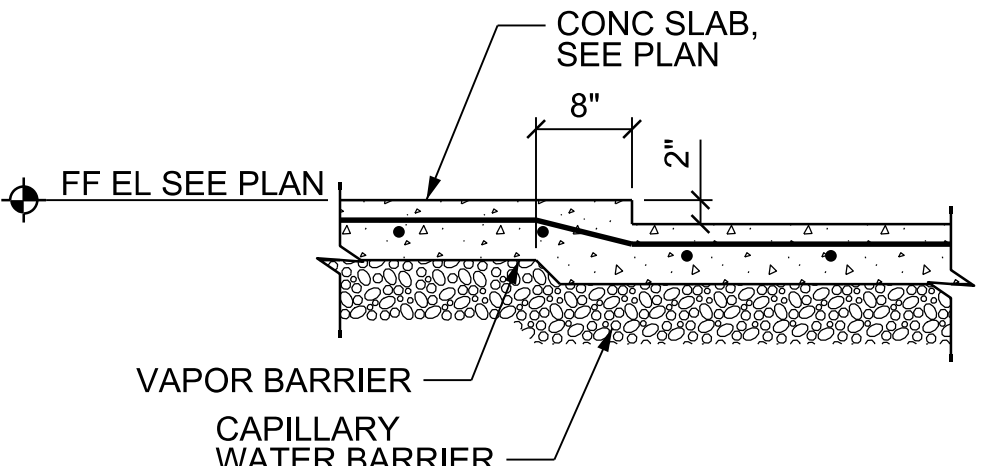
RECESSED SLAB
