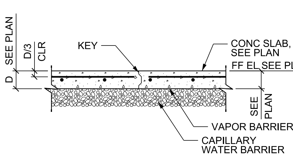
SLAB CONSTRUCTION JOINT (CONST. JT.)
