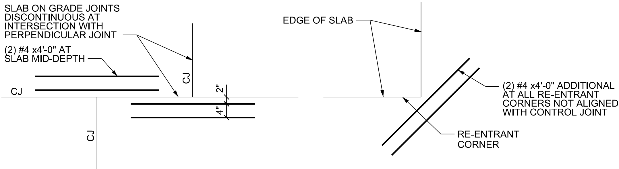
JOINT INTERSECTION DETAIL
