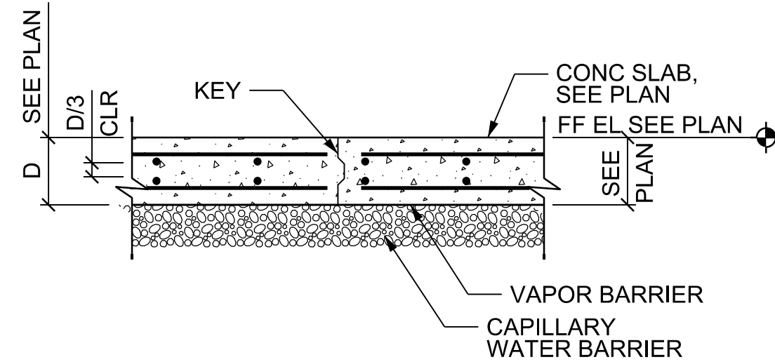
8" SLAB CONSTRUCTION JOINT (CONST JT)
