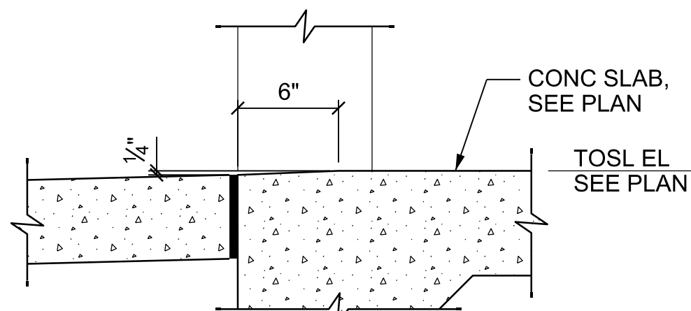
AT ROLLUP DOOR
