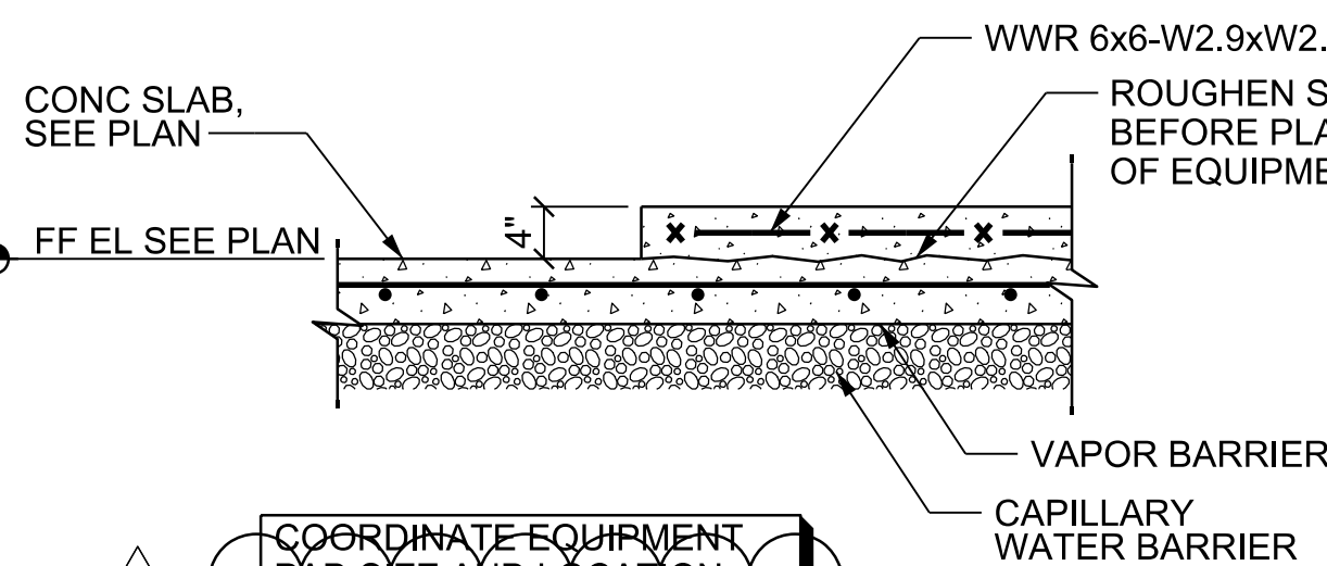
EQUIPMENT PAD/CURB DETAIL
