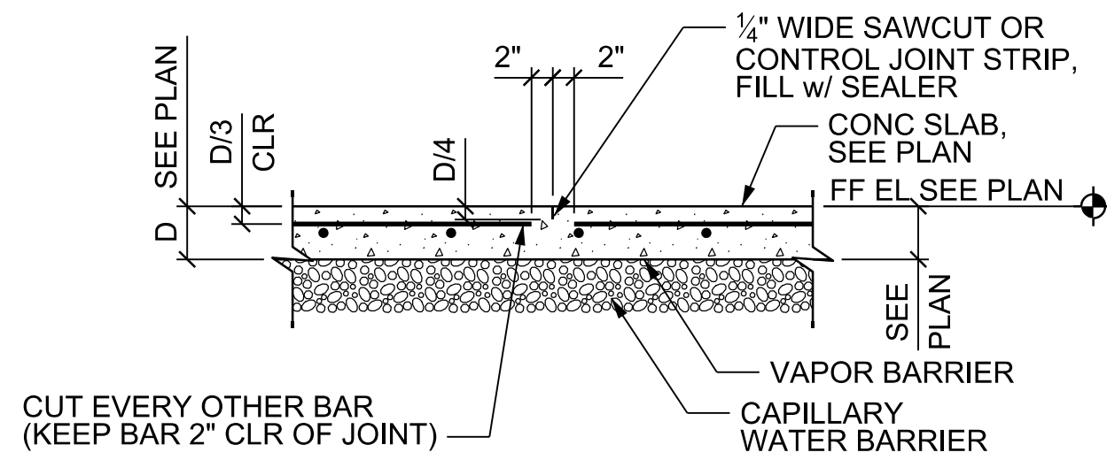
5" SLAB CONTRACTION JOINT (CJ)
