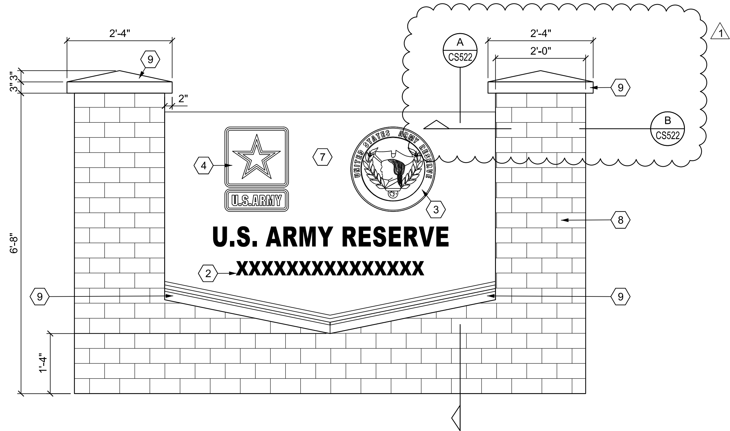
FRONT AND BACK ELEVATION NOT TO SCALE
