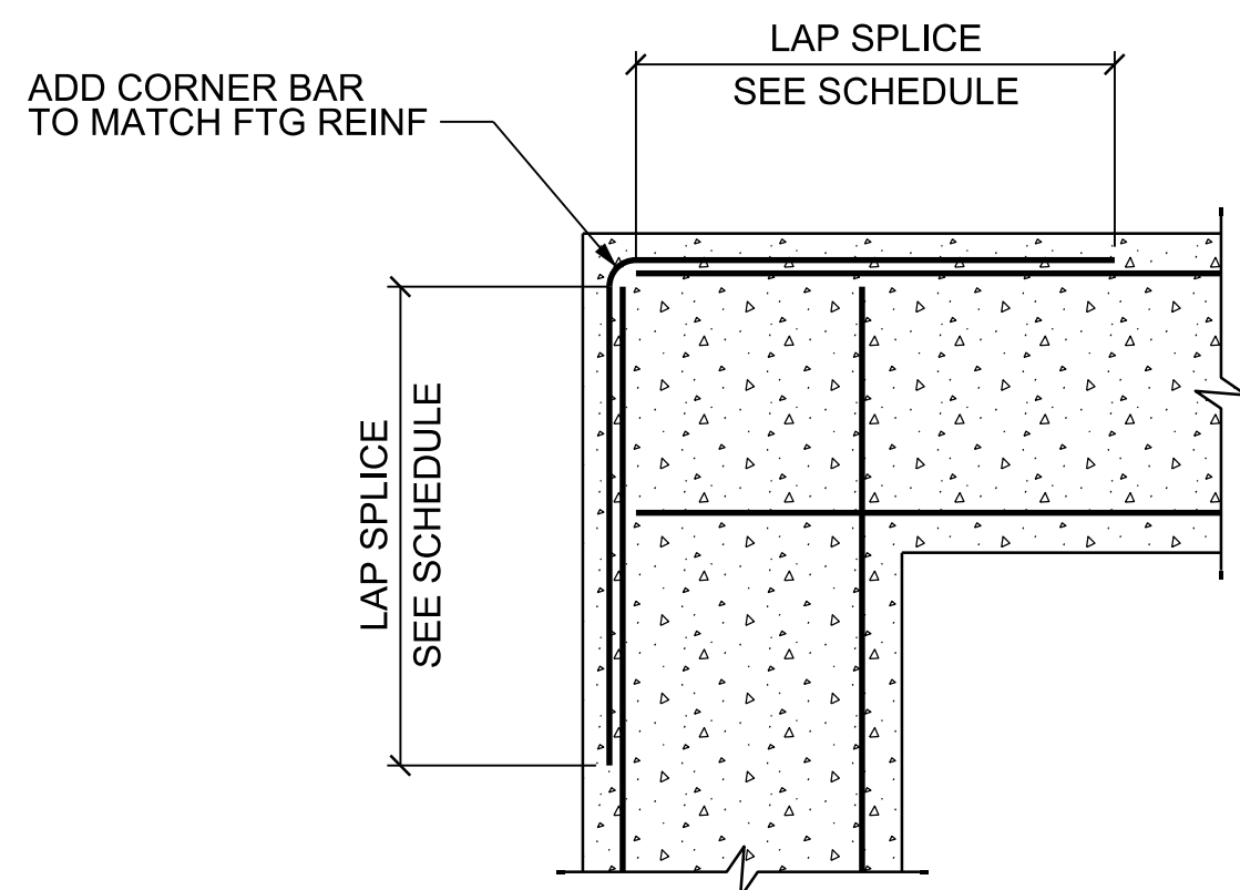
PLAN AT CORNER
