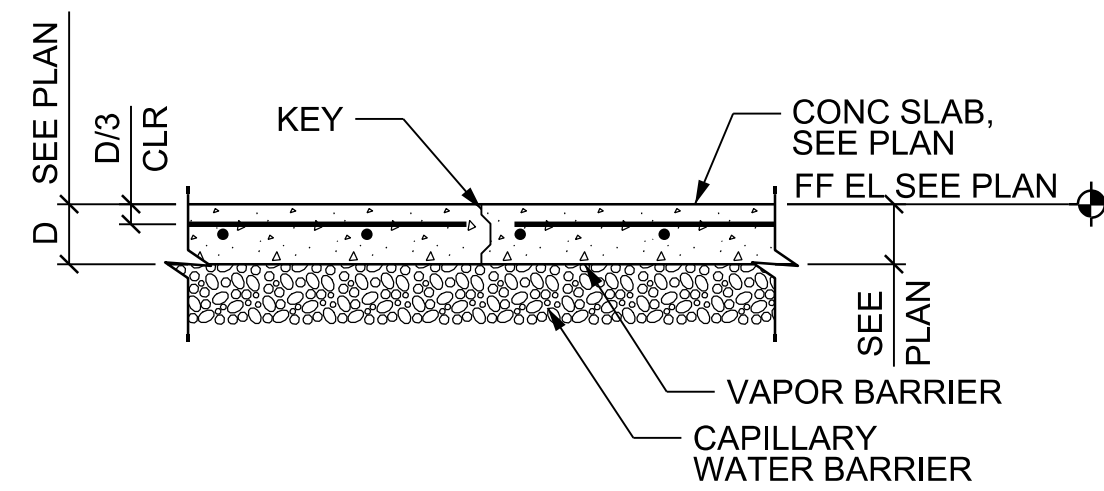
5" SLAB CONSTRUCTION JOINT (CONST JT)
