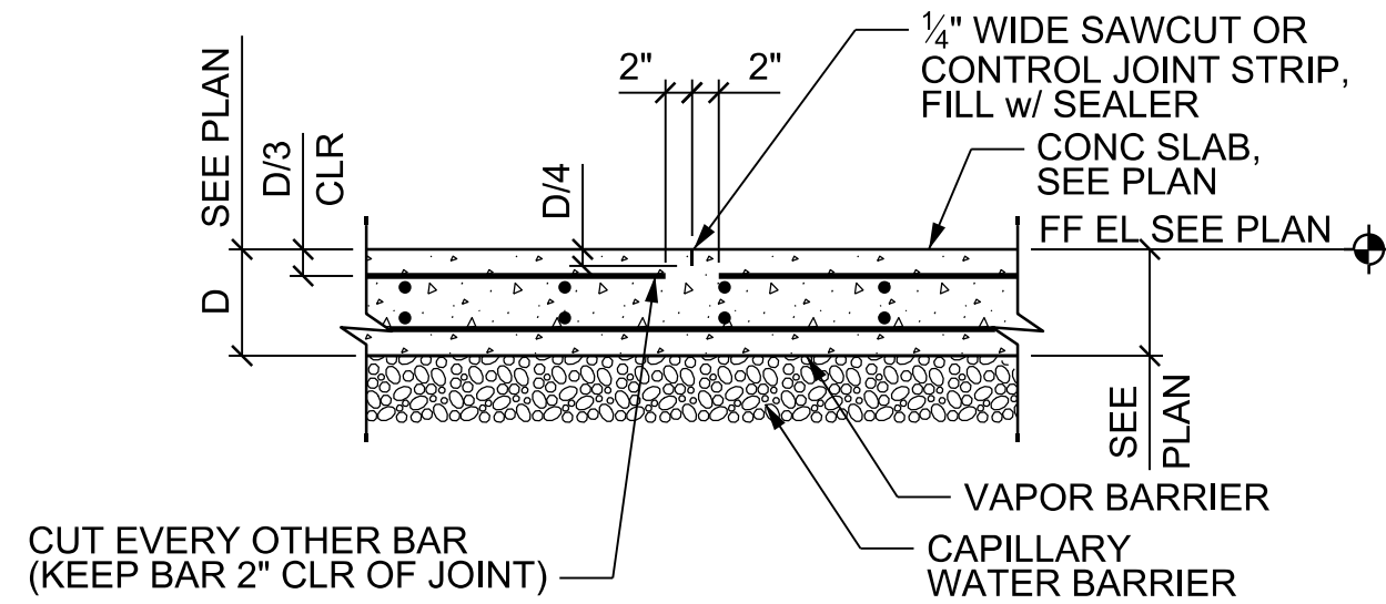
8" SLAB CONTRACTION JOINT (CJ)
