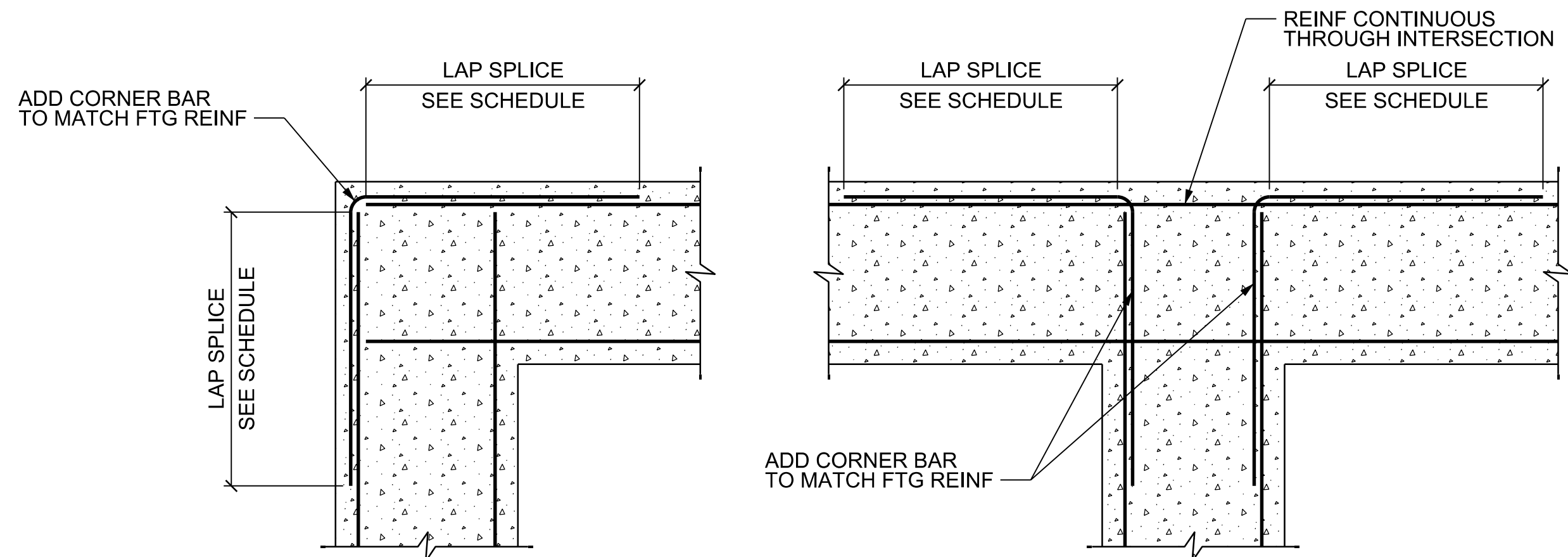
PLAN AT CORNER
