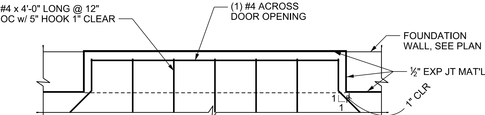
ADDITIONAL SLAB REINFORCING AT DOORWAY
