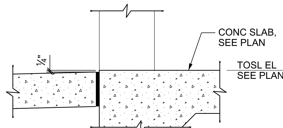
AT PERSONNEL DOOR
