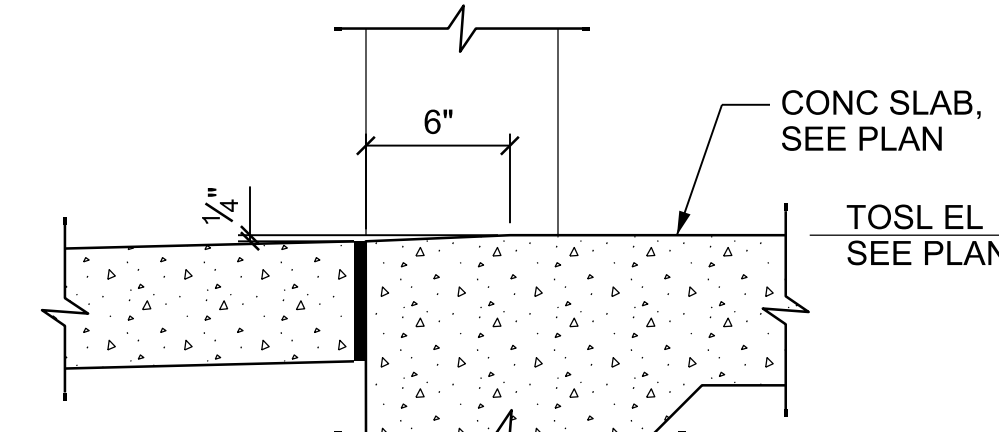
AT ROLLUP DOOR
