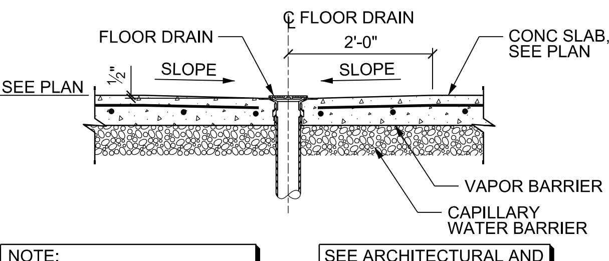
FLOOR DRAIN
