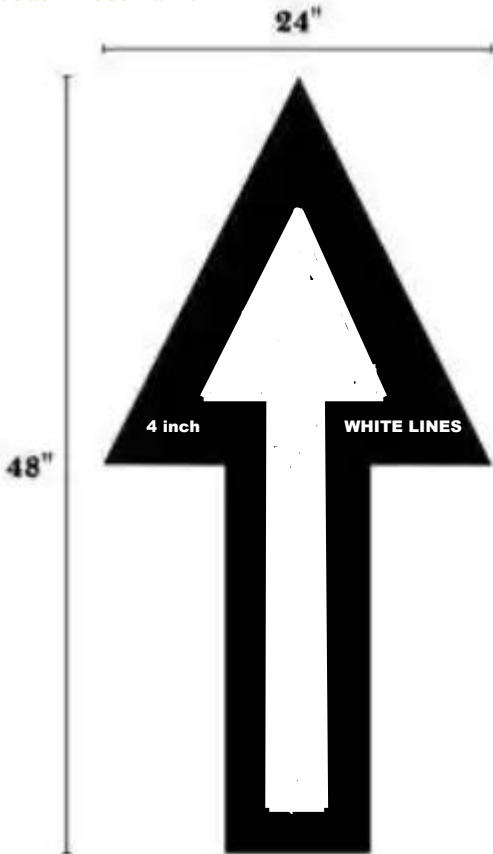
TRAFFIC FLOW ARROW
