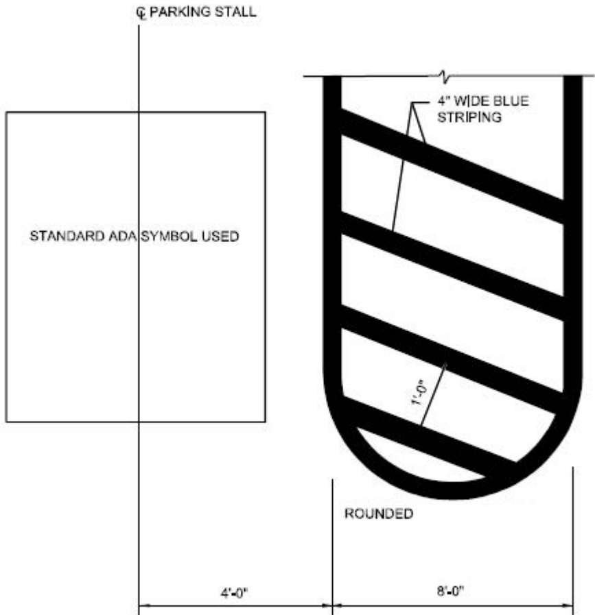
HANDICAPPED PARKING DETAIL N.T.S.
