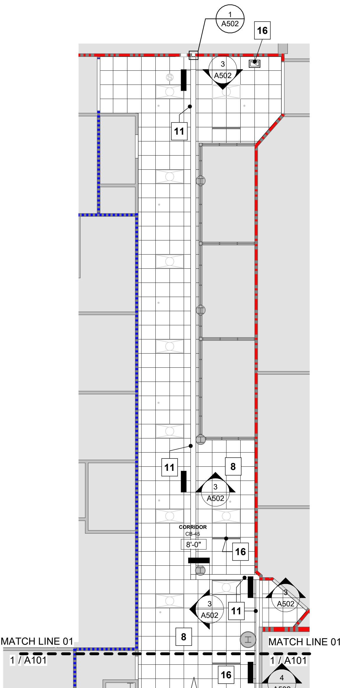
2 BASEMENT RCP CORRIDOR CB-45 1/8" = 1'-0"
