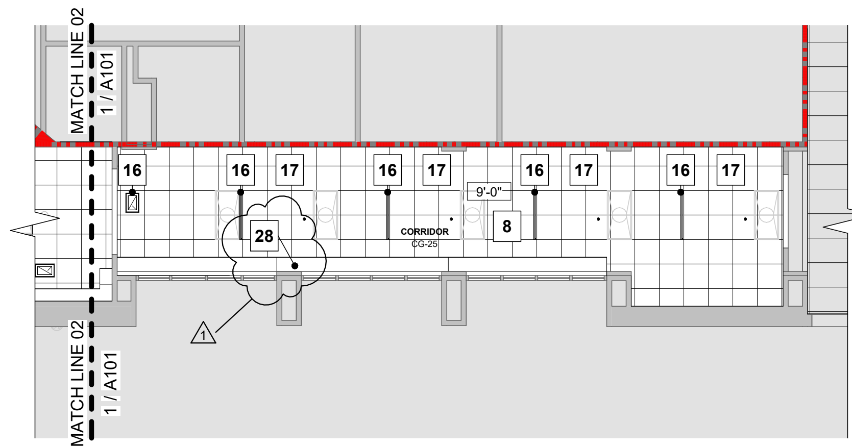
3 BASEMENT RCP CORRIDOR CG-25 1/8" = 1'-0"
