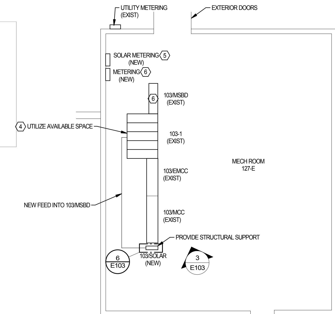
2 FIRST FLOOR - SERVICE RM 127-E SCALE: 1/8\"/>
