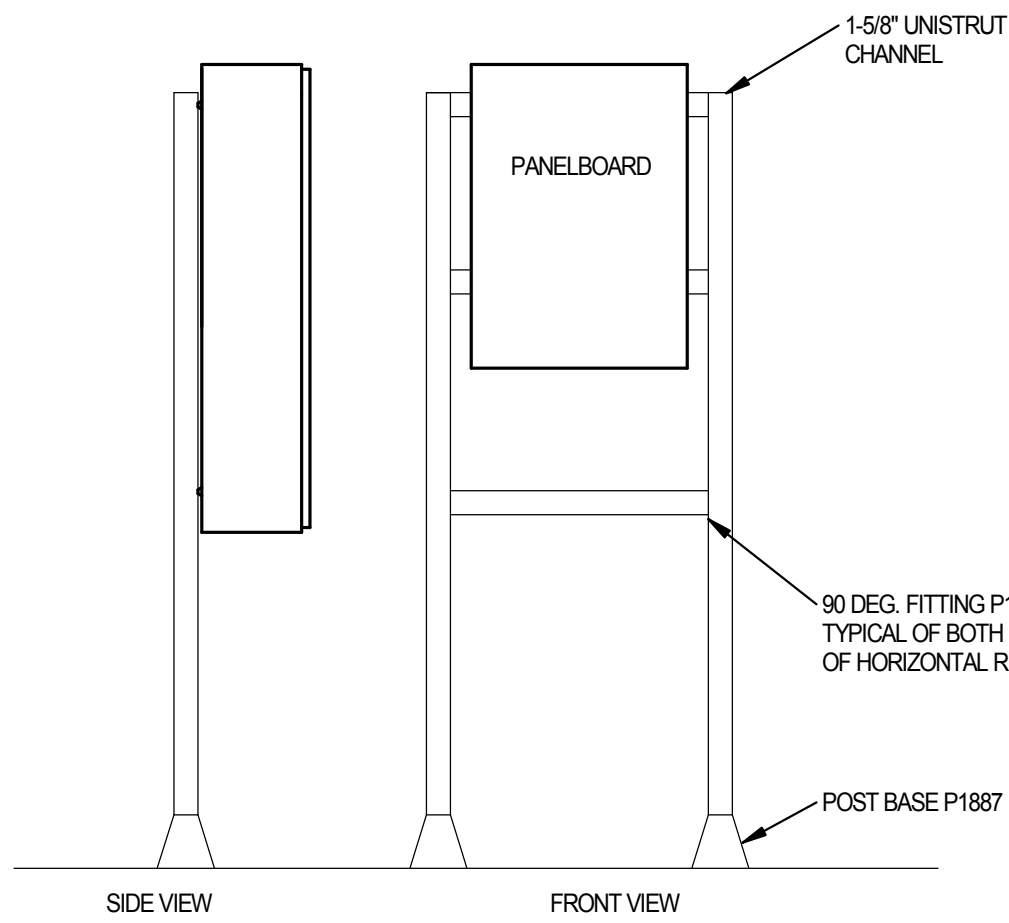
6 FREE STANDING PANEL SCALE: NONE
