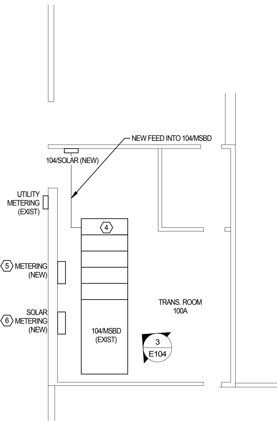
FIRST FLOOR - TRANSFORMER RM 100A
