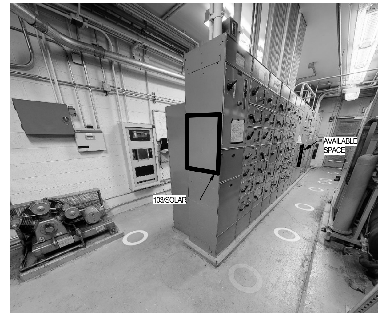
3 BUILDING 103 MAIN ELEC RM 127-E SCALE: NONE
