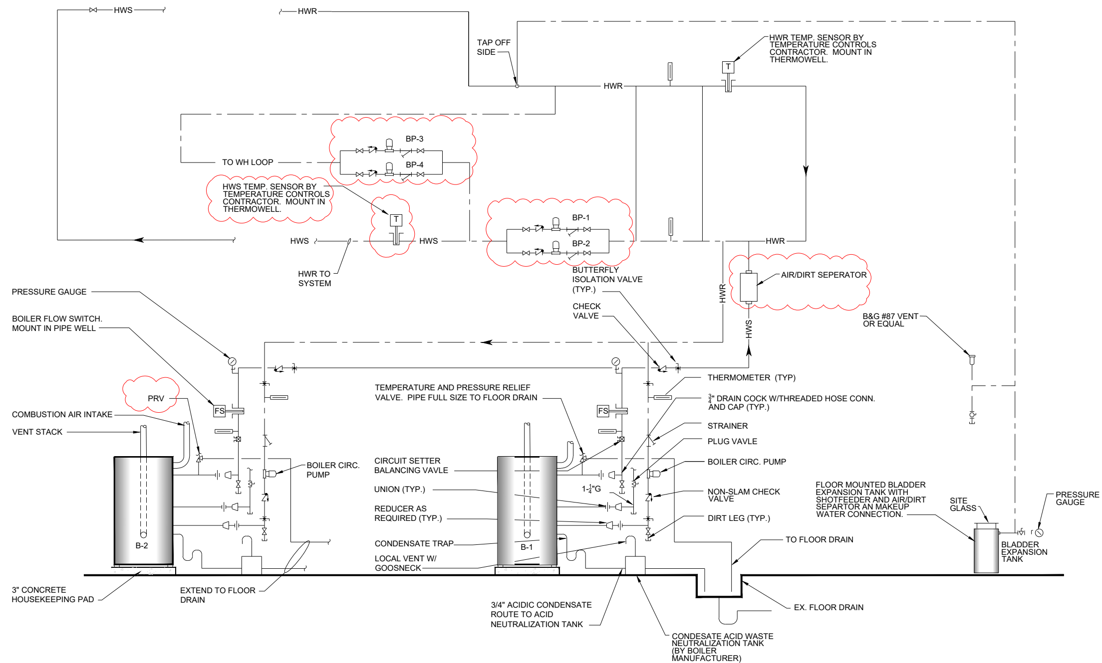
1 HEATING PLANT PIPING DIAGRAM 6 SCALE: N.T.S.
