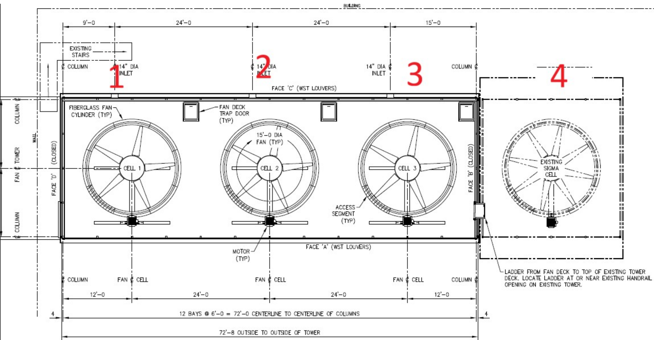
TOWER SCHEMATIC PLAN VIEW (SEE DRAWING 18-21823 FOR ENDWALL ELEVATION VIEW)
