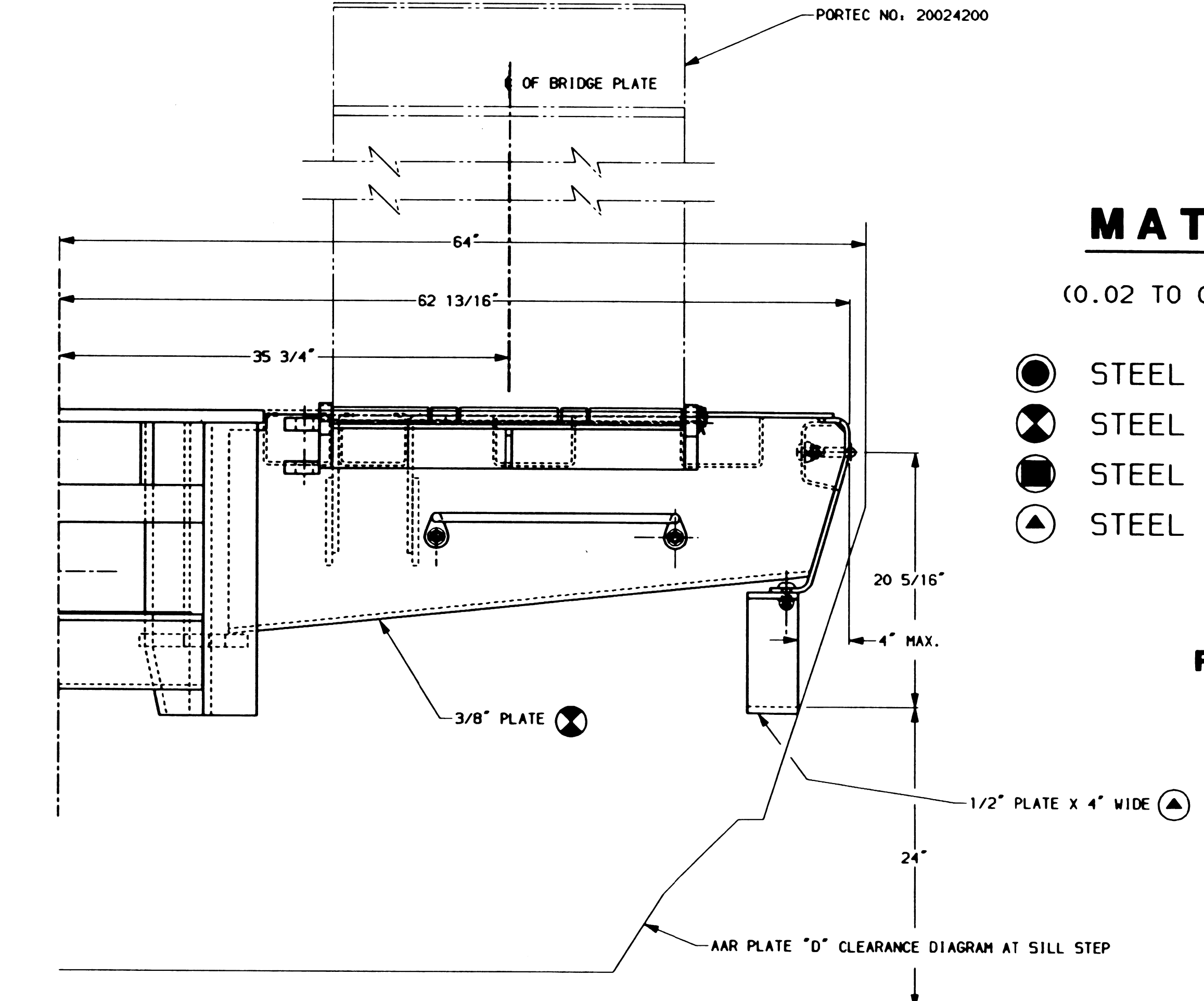
VIEW - "A - A"
