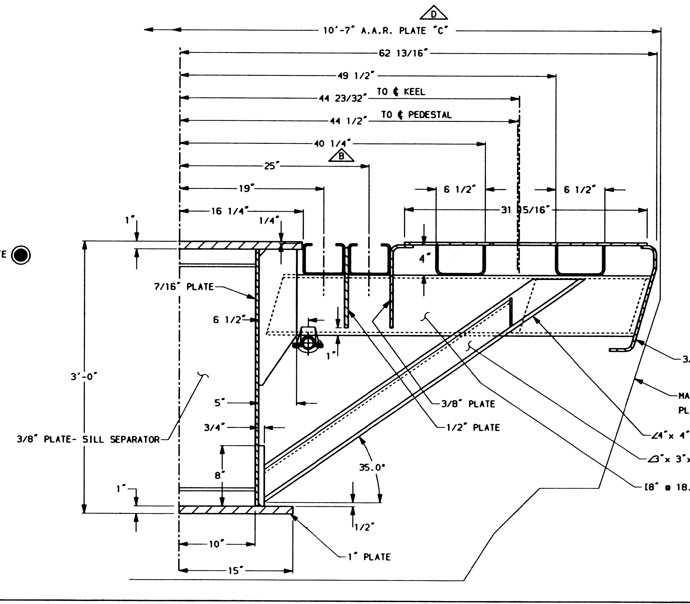
SECTION - "Z - Z"
