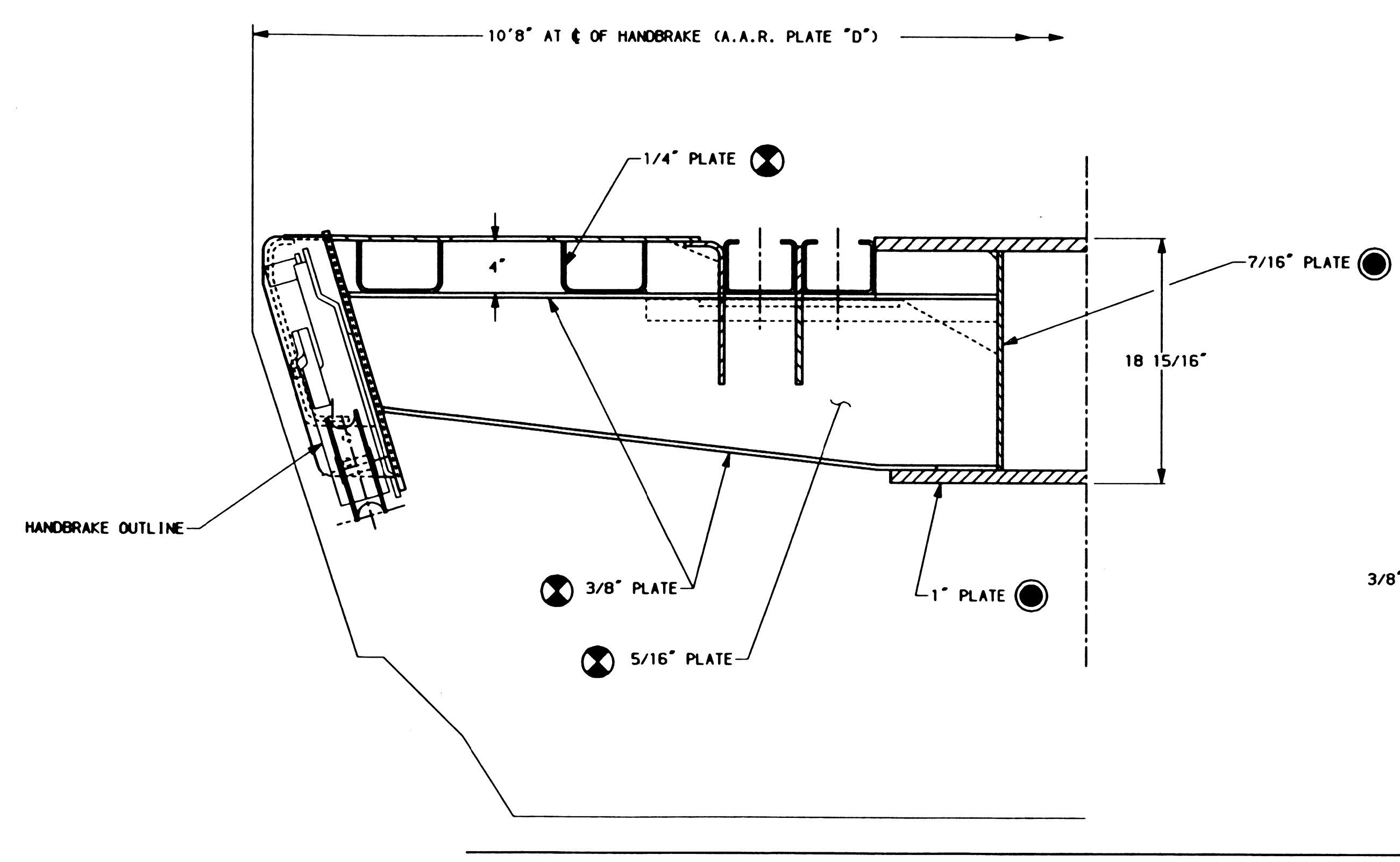
SECTION - "Y - Y"
