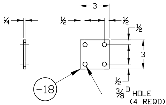
DETAIL A (REAR BRACKET)
