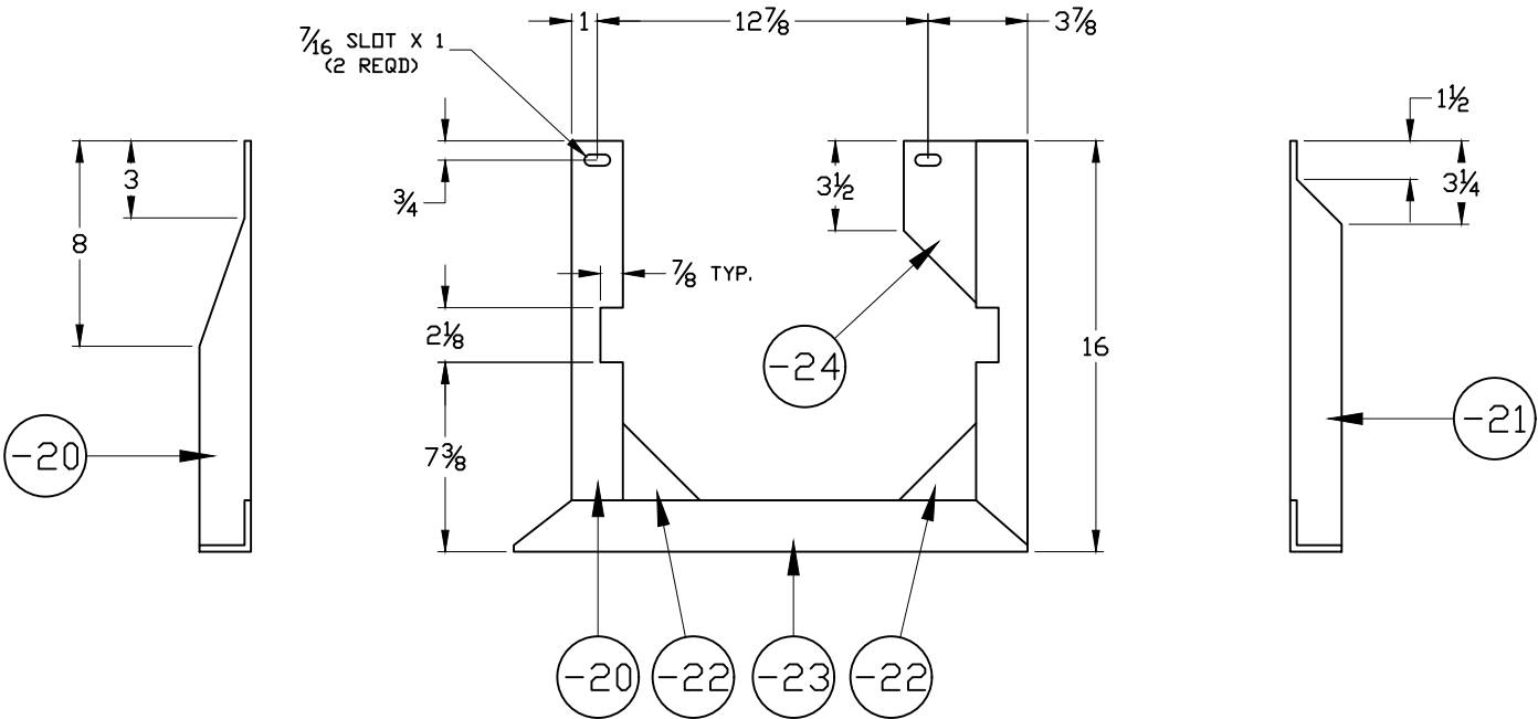
END VIEW
