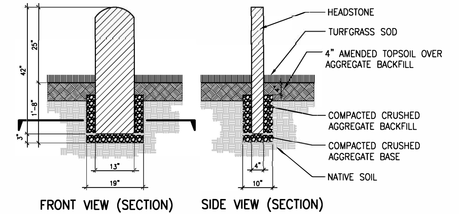
1 UPRIGHT HEADSTONE INSTALLATION (BASE BID) SCALE: N.T.S. PLAN/SECTION/CROSS-SECTION
