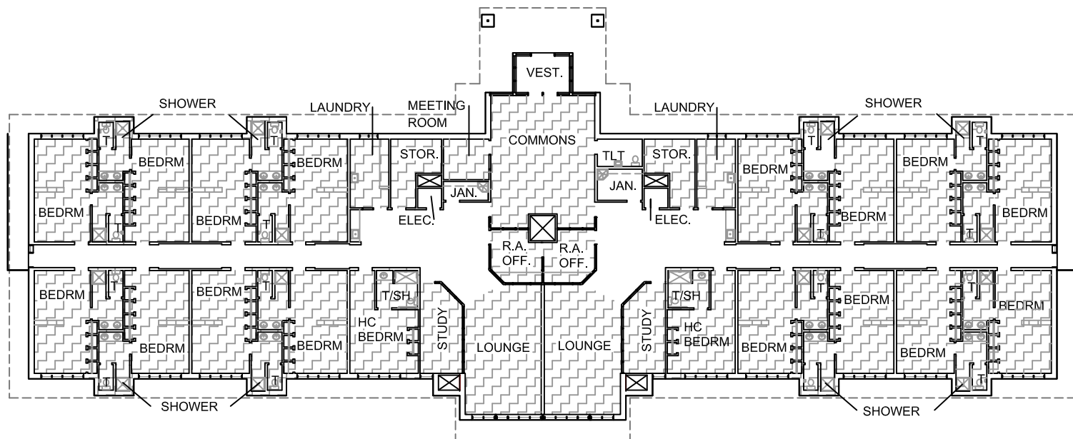
FIRST FLOOR
