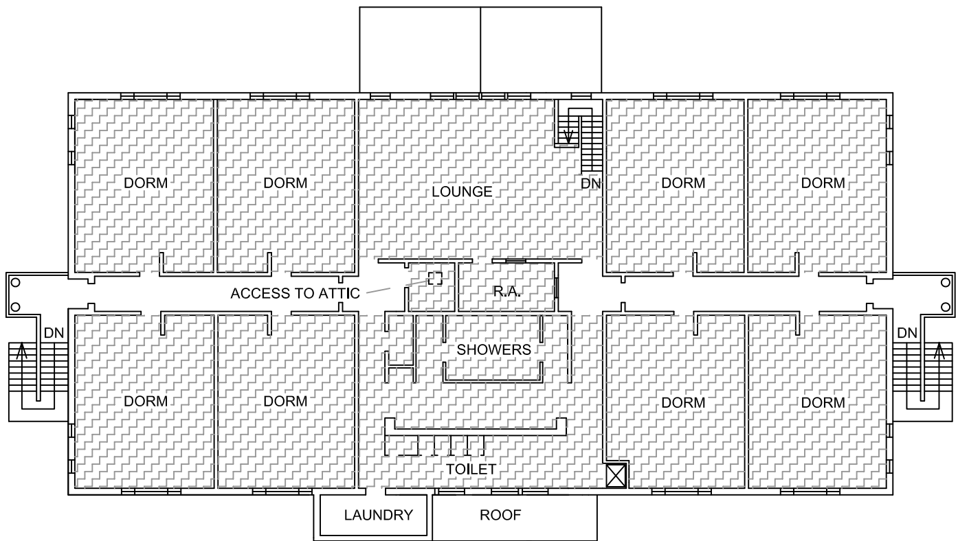
SECOND FLOOR
