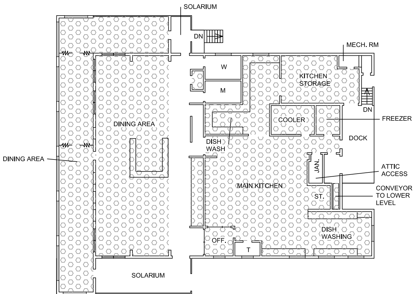
UPPER LEVEL
