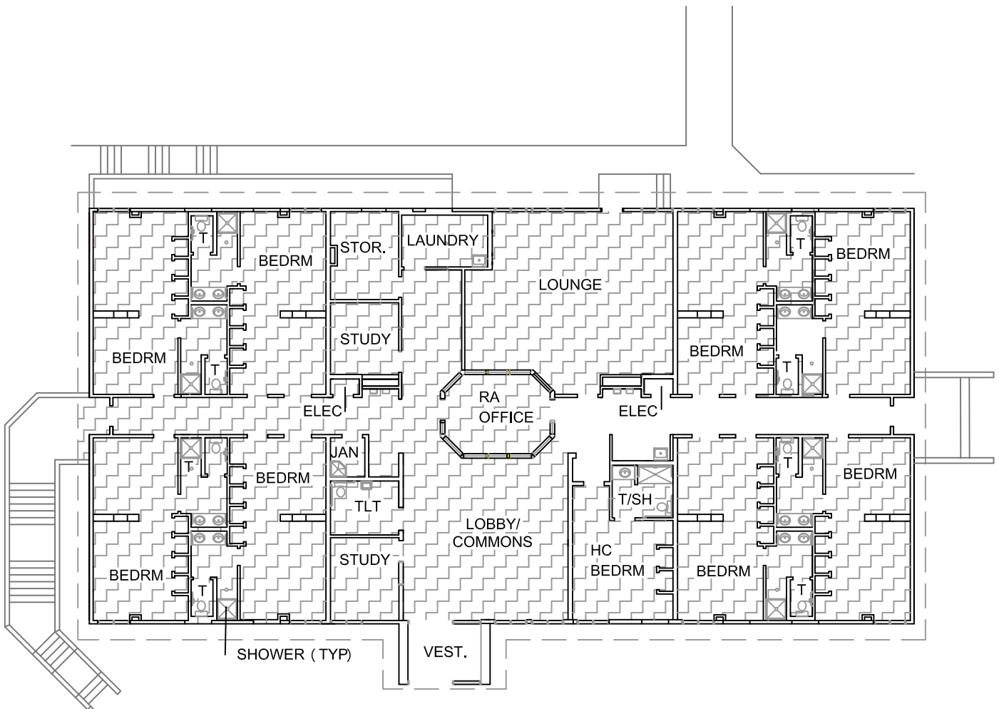
FIRST FLOOR
