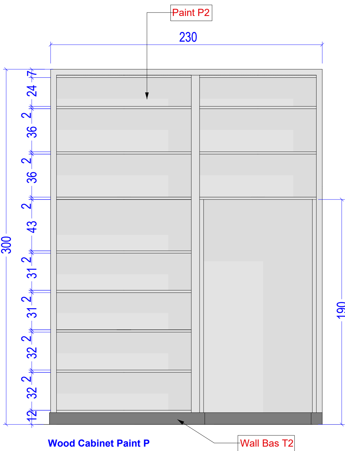
ELEVATION INTERIEUR
