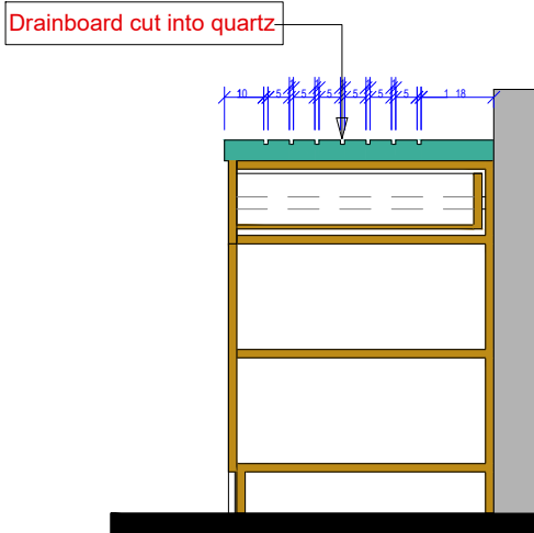
COUPE -BB-
