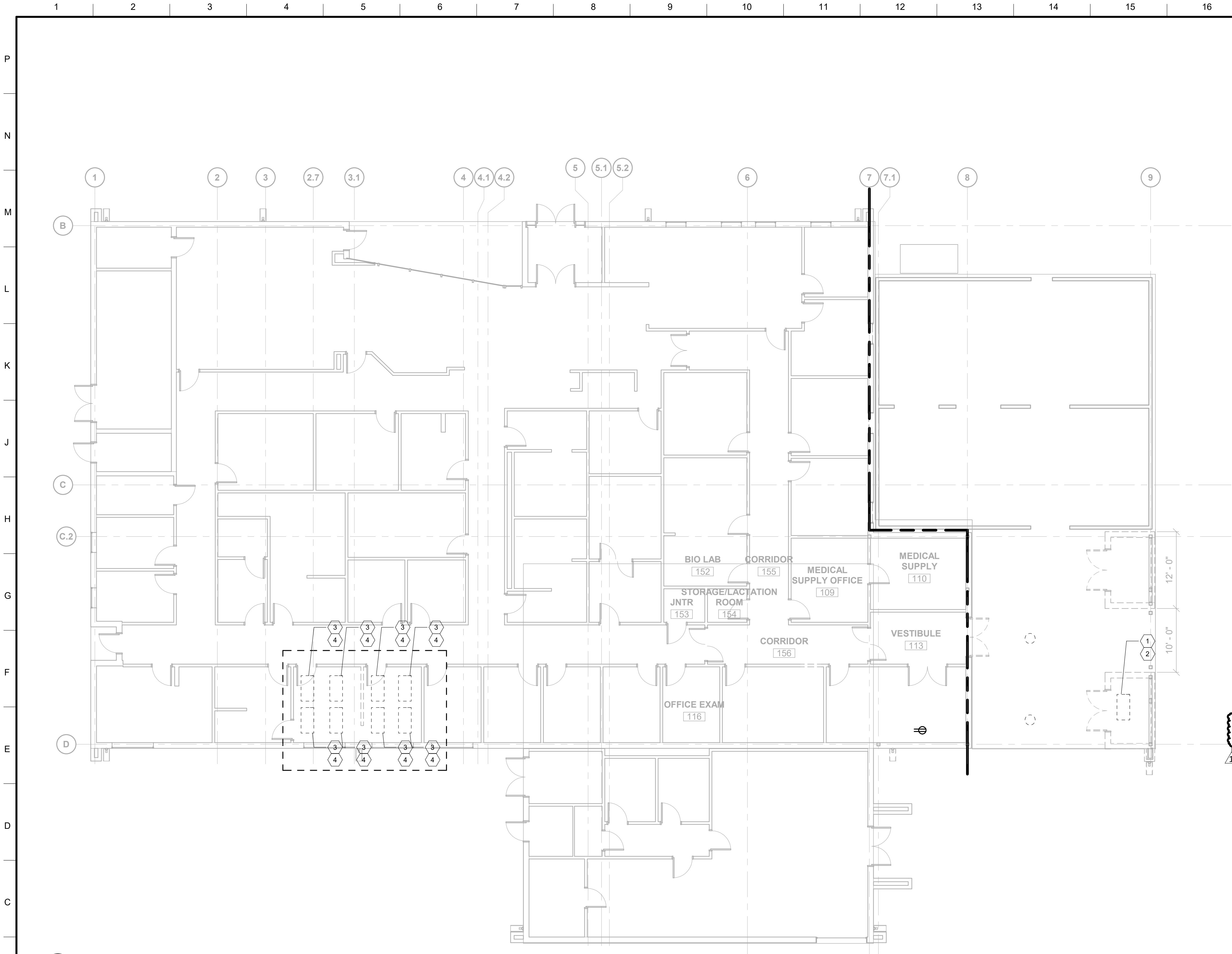
B1 LEVEL 1 - ELECTRICAL DEMOLITION SCALE: 1/8" = 1'-0"
