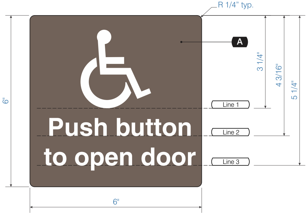
1 N8 FRONT 1/2" = 1"
