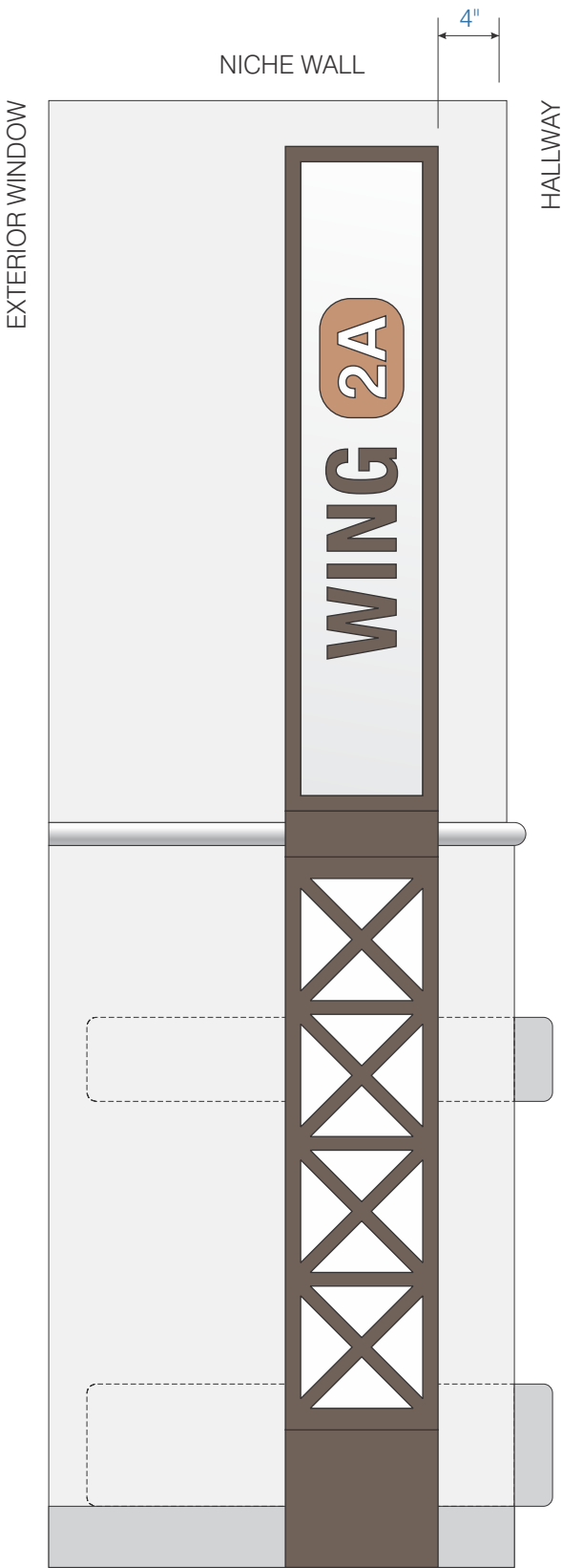
9 EAST NICHE WALL ELEVATION, TYP. W4 1" = 1'-0"
