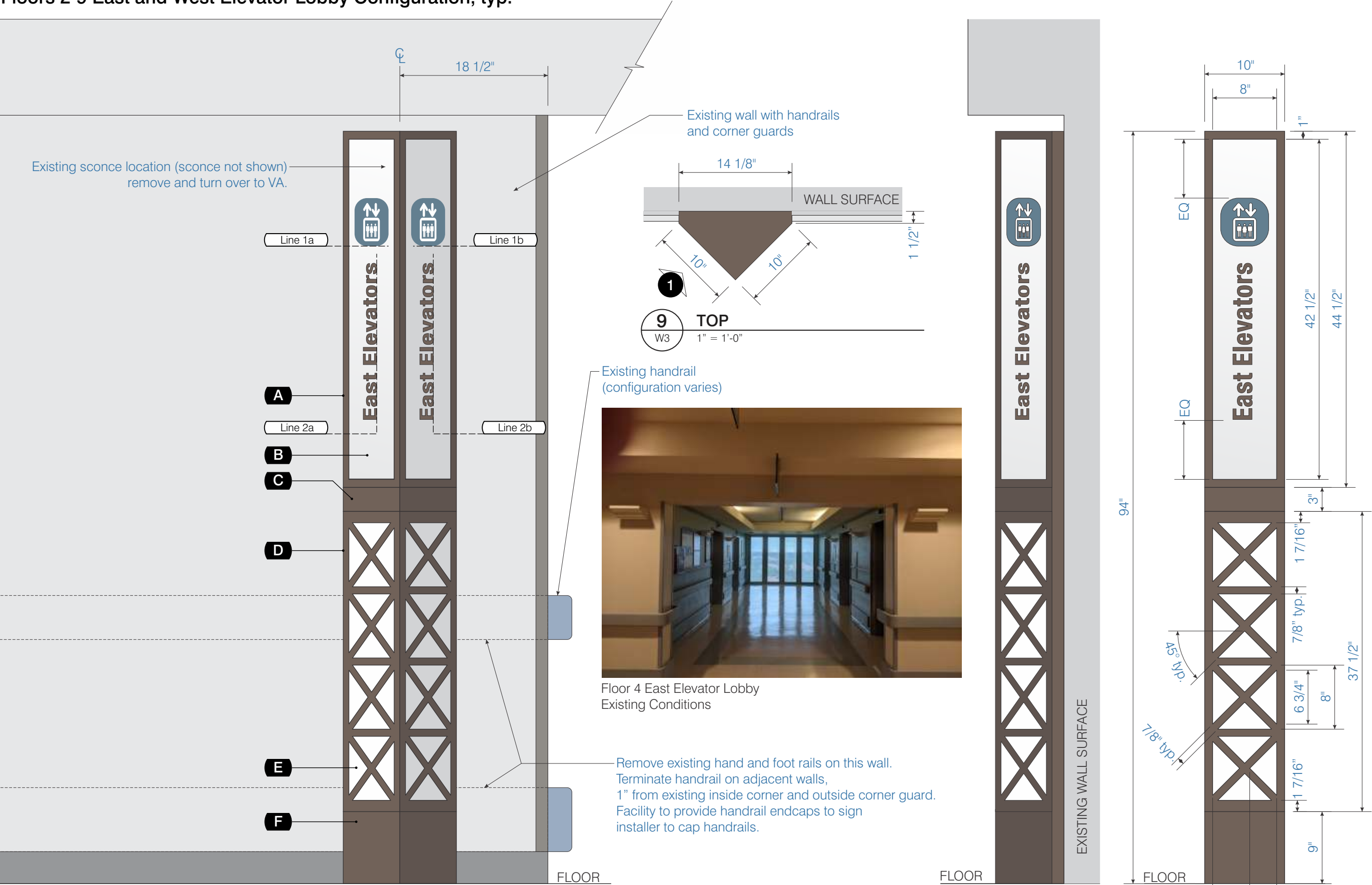
10 FRONT W3 1" = 1'-0"
