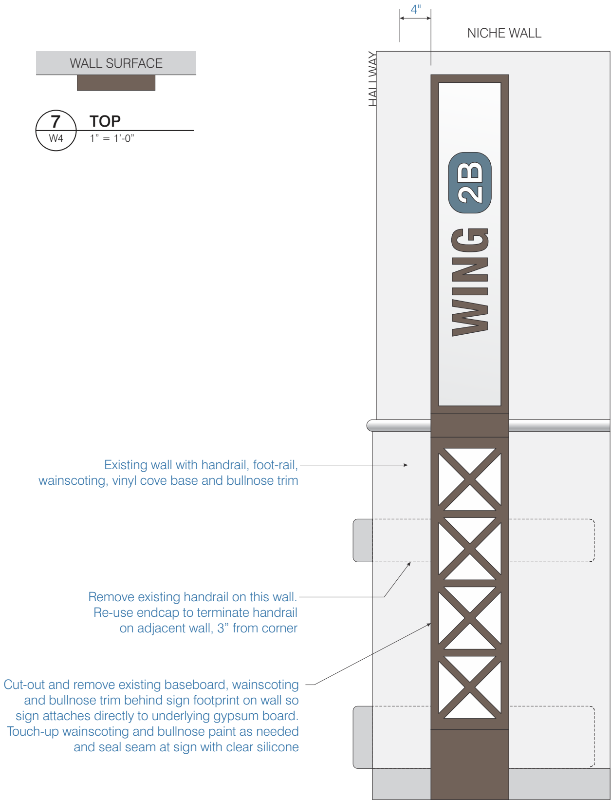
8 WEST NICHE WALL ELEVATION, TYP. W4 1" = 1'-0"
