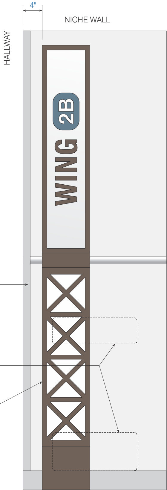
8 WEST NICHE WALL ELEVATION, TYP. W4 1" = 1'-0"
