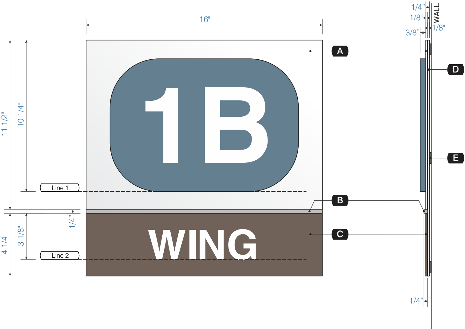
2 FRONT i1 1/4" = 1"
