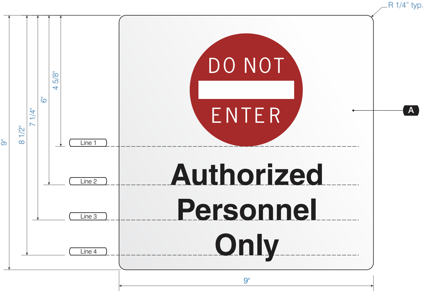
1 FRONT R4 1/2" = 1"
