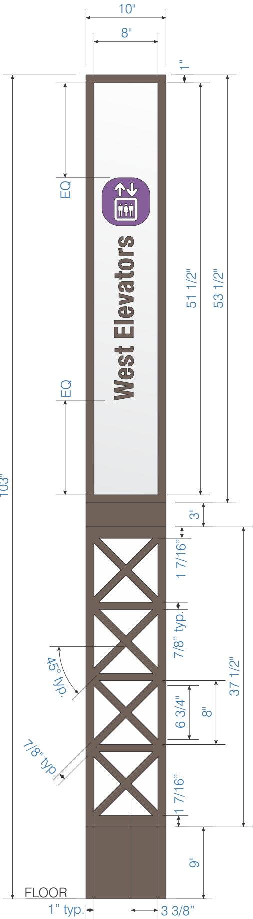
8 ELEVATION 1 W3 1" = 1'-0"
