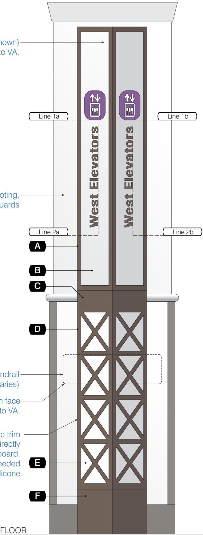
6 FRONT W3 1" = 1'-0"
