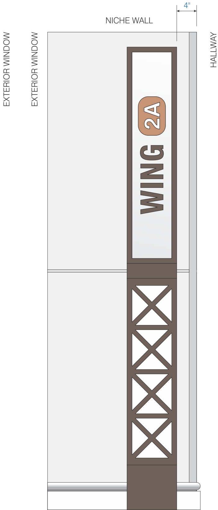
13 W4 EAST NICHE WALL ELEVATION, TYP. 1" = 1'-0"
