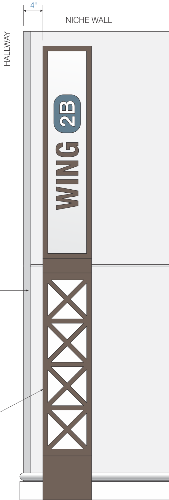
12 W4 WEST NICHE WALL ELEVATION, TYP. 1" = 1'-0"
