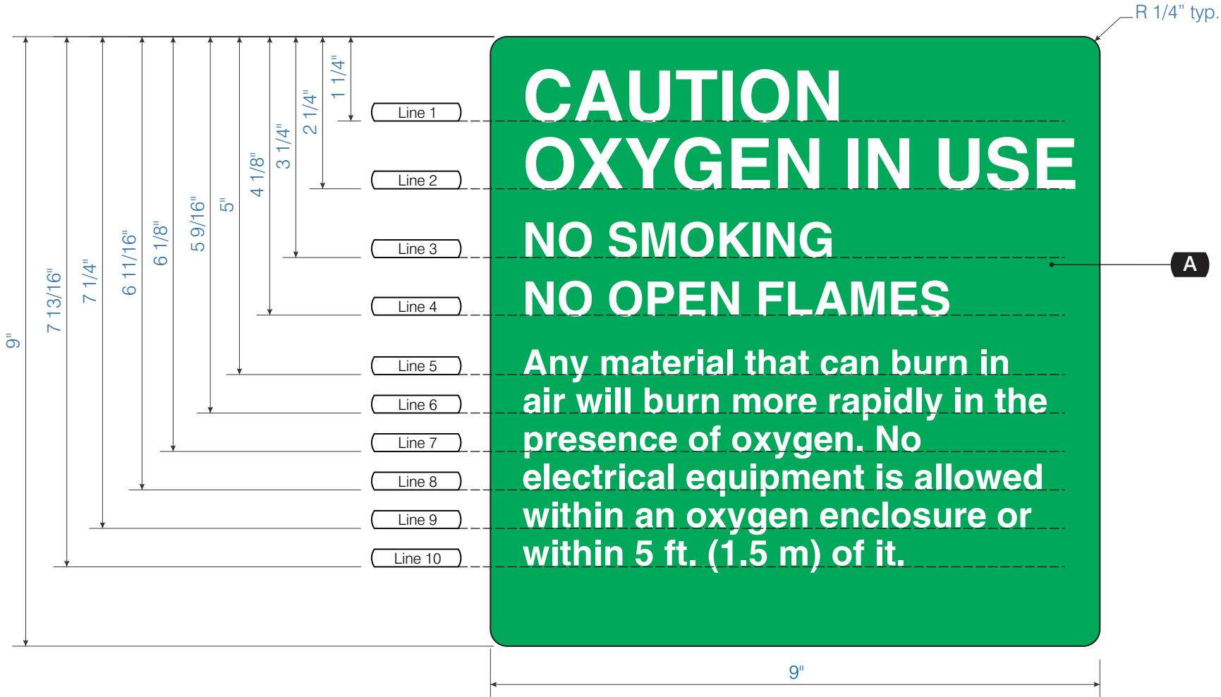
1 FRONT R3 1/2" = 1"
