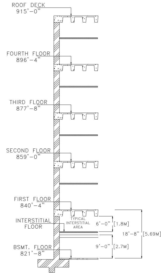
TYPICAL ELEVATION NOT TO SCALE
