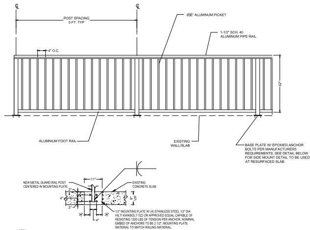
5 METAL GUARD RAIL NTS
