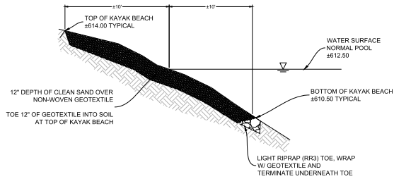
8 SAND BEACH KAYAK LAUNCH NTS
