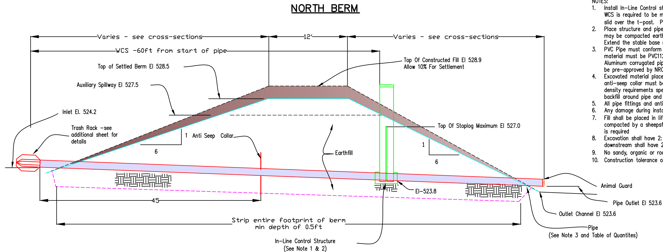
TYPICAL BERM CROSS SECTION
