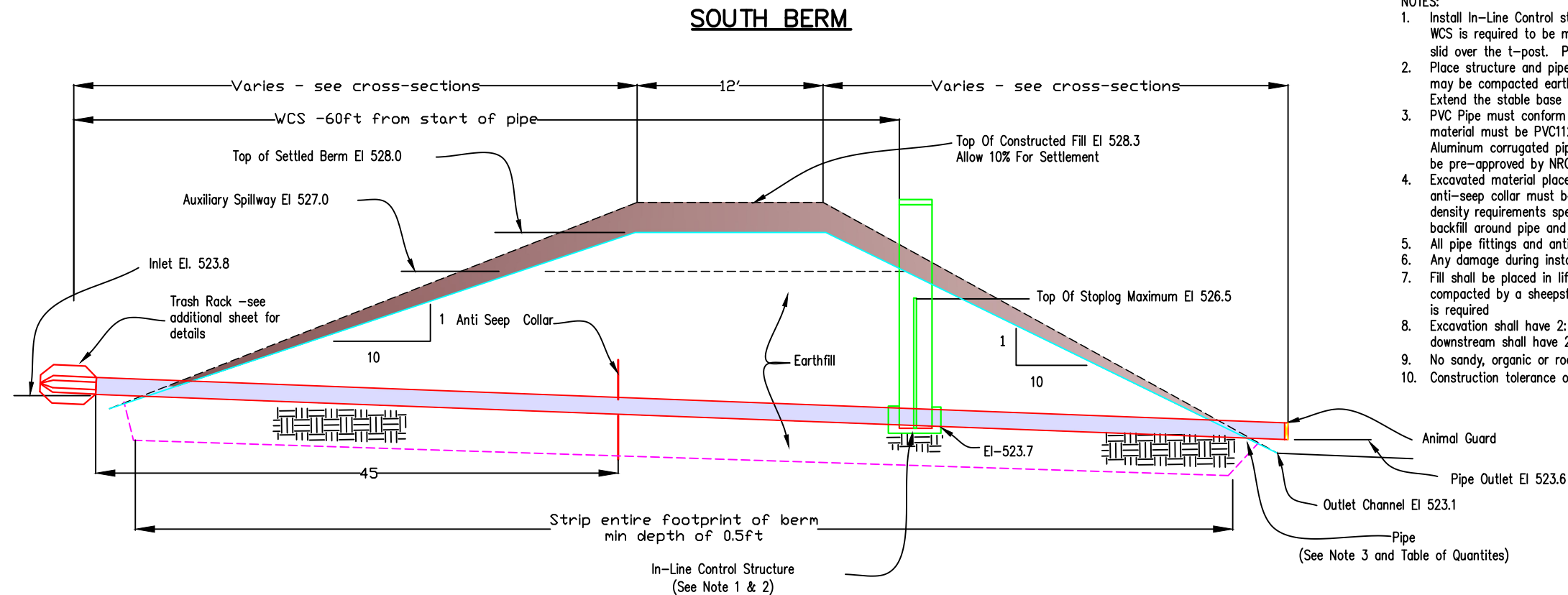
TYPICAL BERM CROSS SECTION
