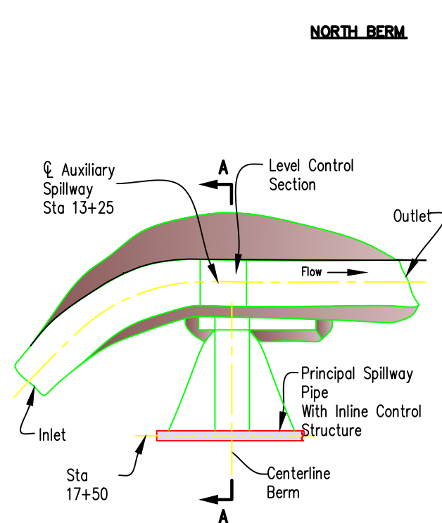
AUXILIARY SPILLWAY PLAN
