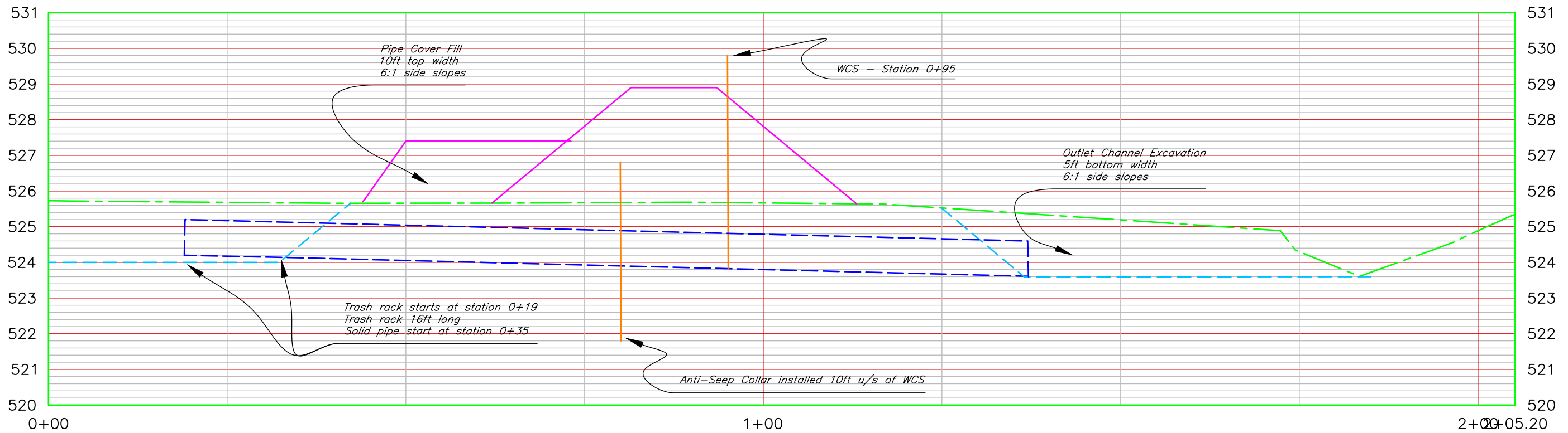
Pipe North PROFILE
