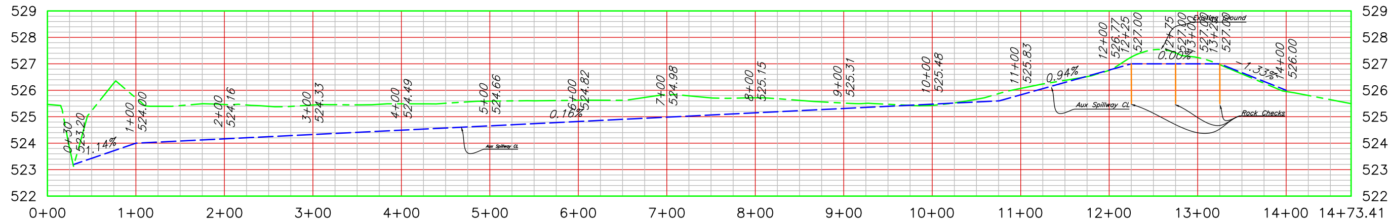
Alignment – Aux Spillway PROFILE
