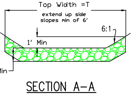
Rock Check sectional view
