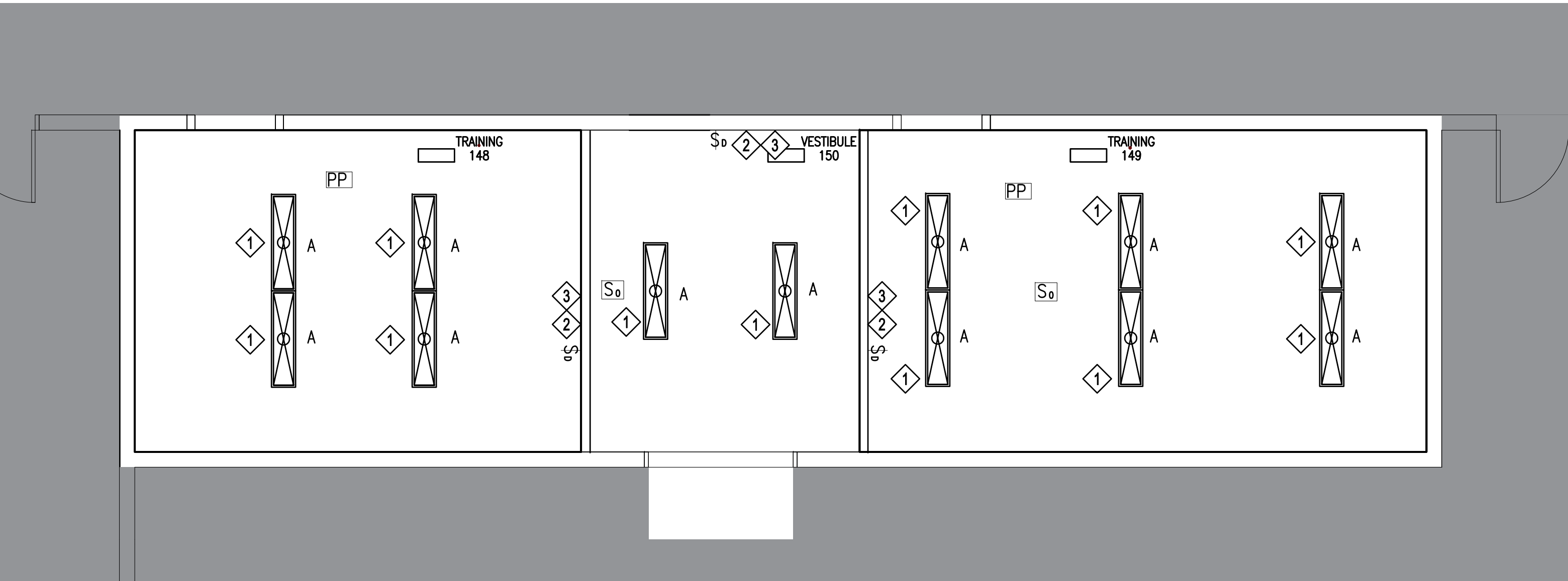
A1 B4845 - ROOM 148,149 & 150 LIGHTING NEW WORK PLAN SCALE: 1/4"=1'-0"
