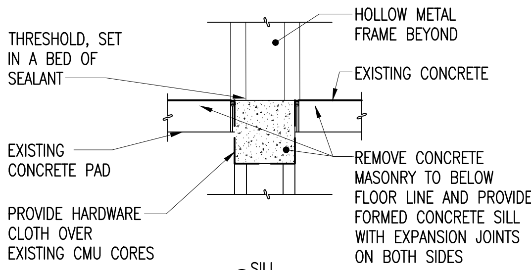
A SILL
