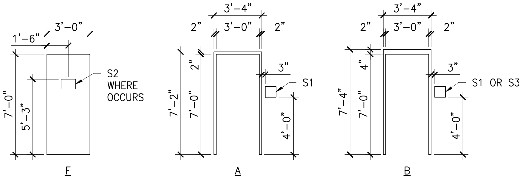
C1 DOOR & STEEL FRAME DIMENSIONS SCALE: 1/4"=1'-0"
