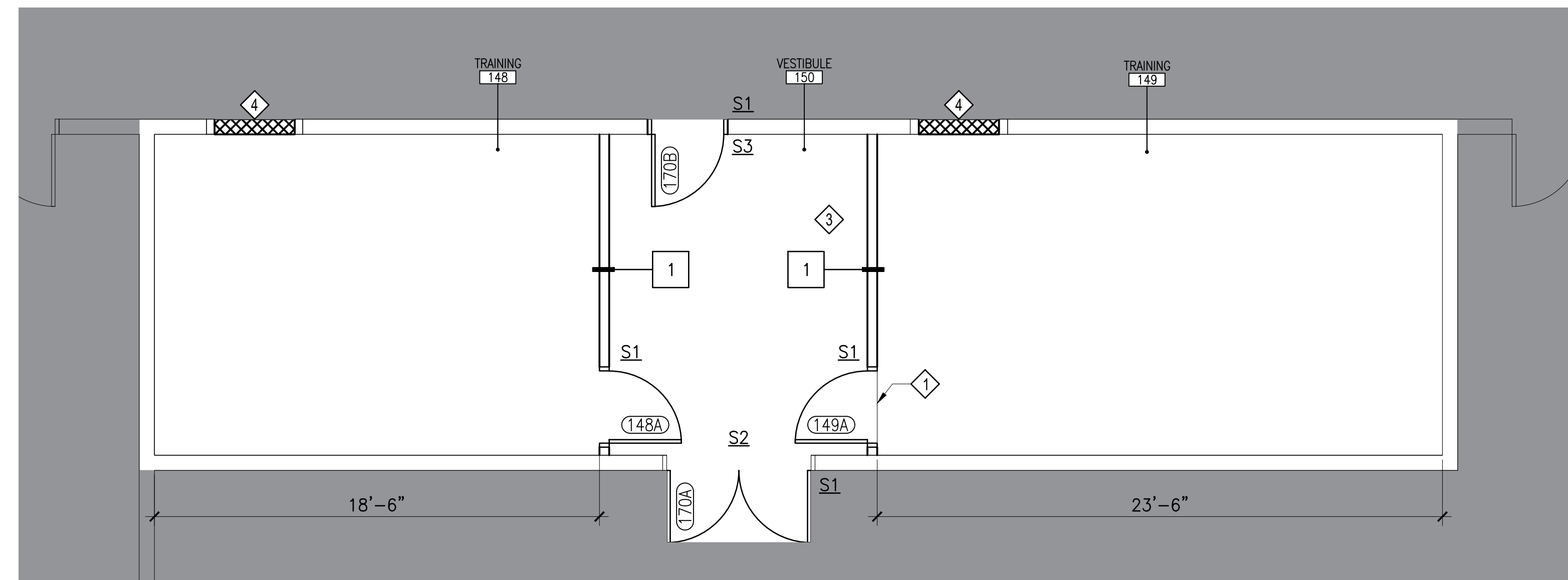
A1 B4845 FLOOR PLAN - CONSTRUCTION SCALE: 1/4"=1'-0"
