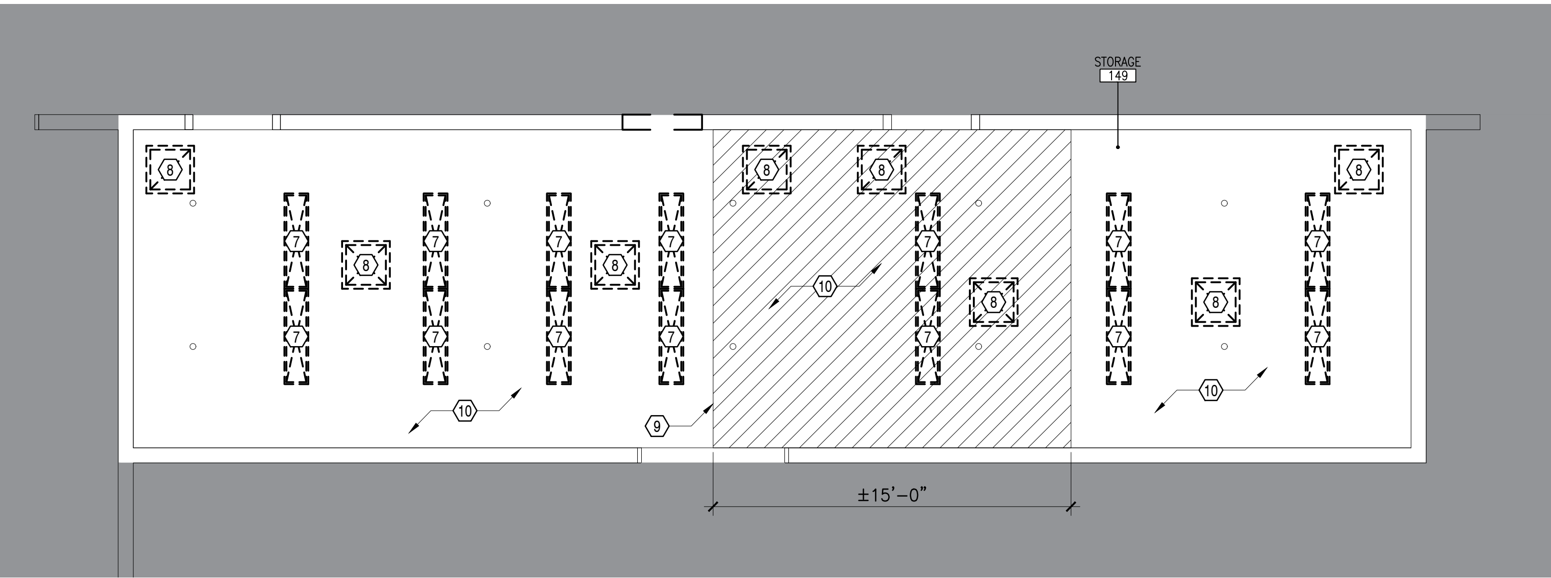
C1 B4845 REFLECTED CEILING PLAN - DEMOLITION SCALE: 1/4"=1'-0"
