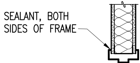
A HEAD
