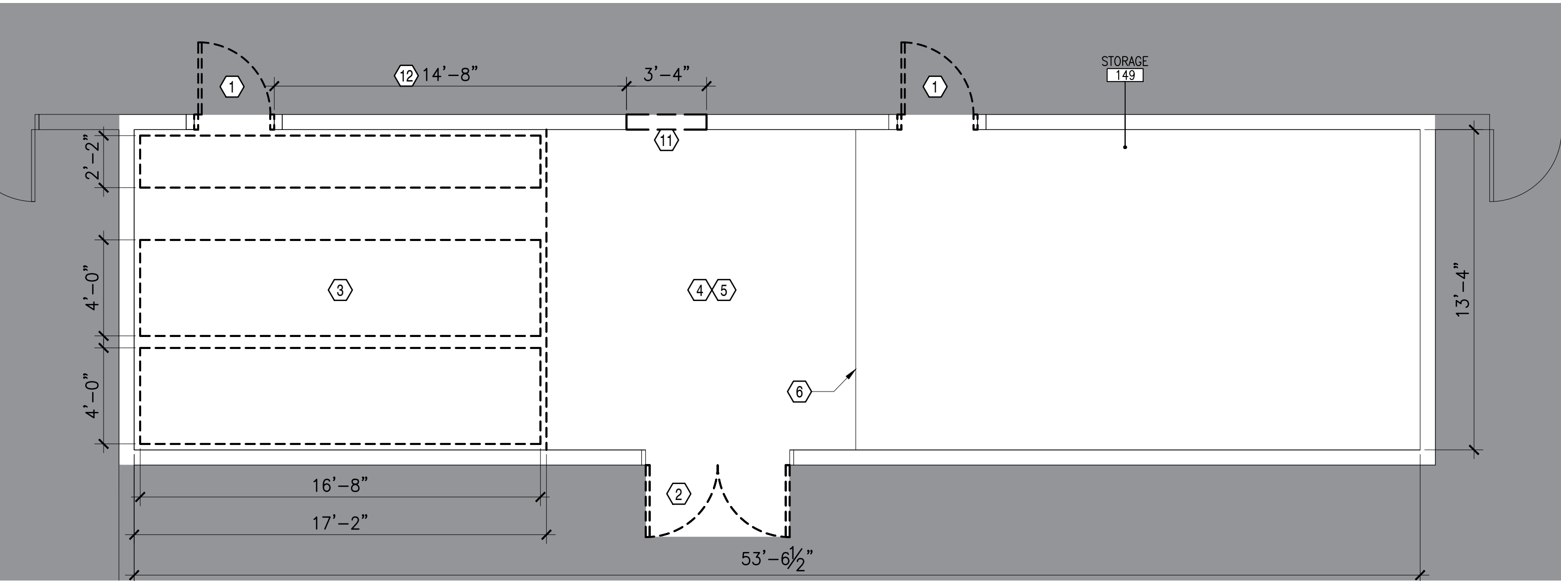
A1 B4845 FLOOR PLAN - DEMOLITION SCALE: 1/4"=1'-0"
