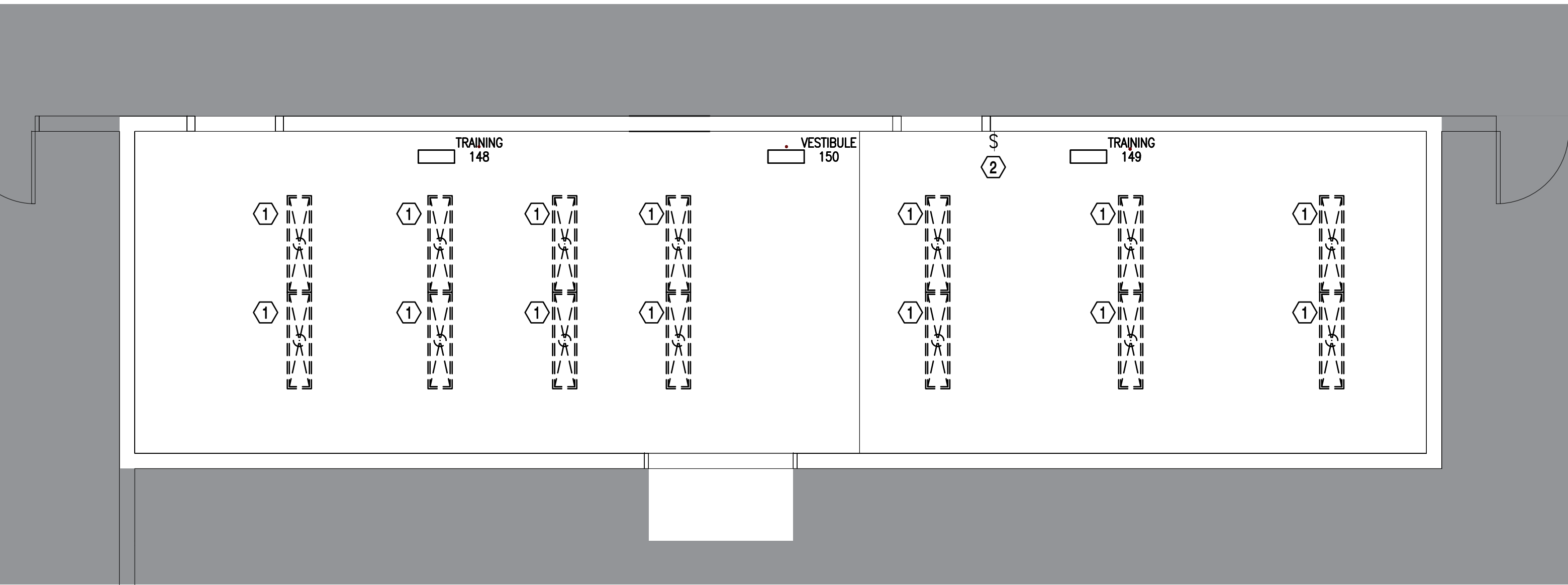
C1 B4845 - ROOM 148, 149 & 150 LIGHTING DEMO PLAN SCALE: 1/4"=1'-0"
