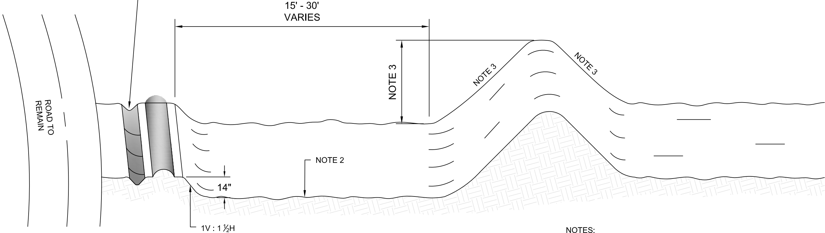
ISOMETRIC VIEW
