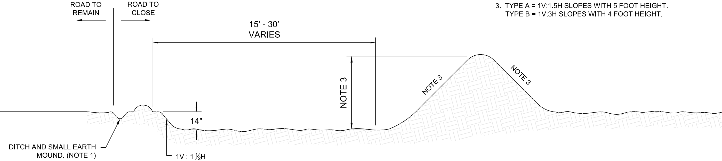
PROFILE VIEW
