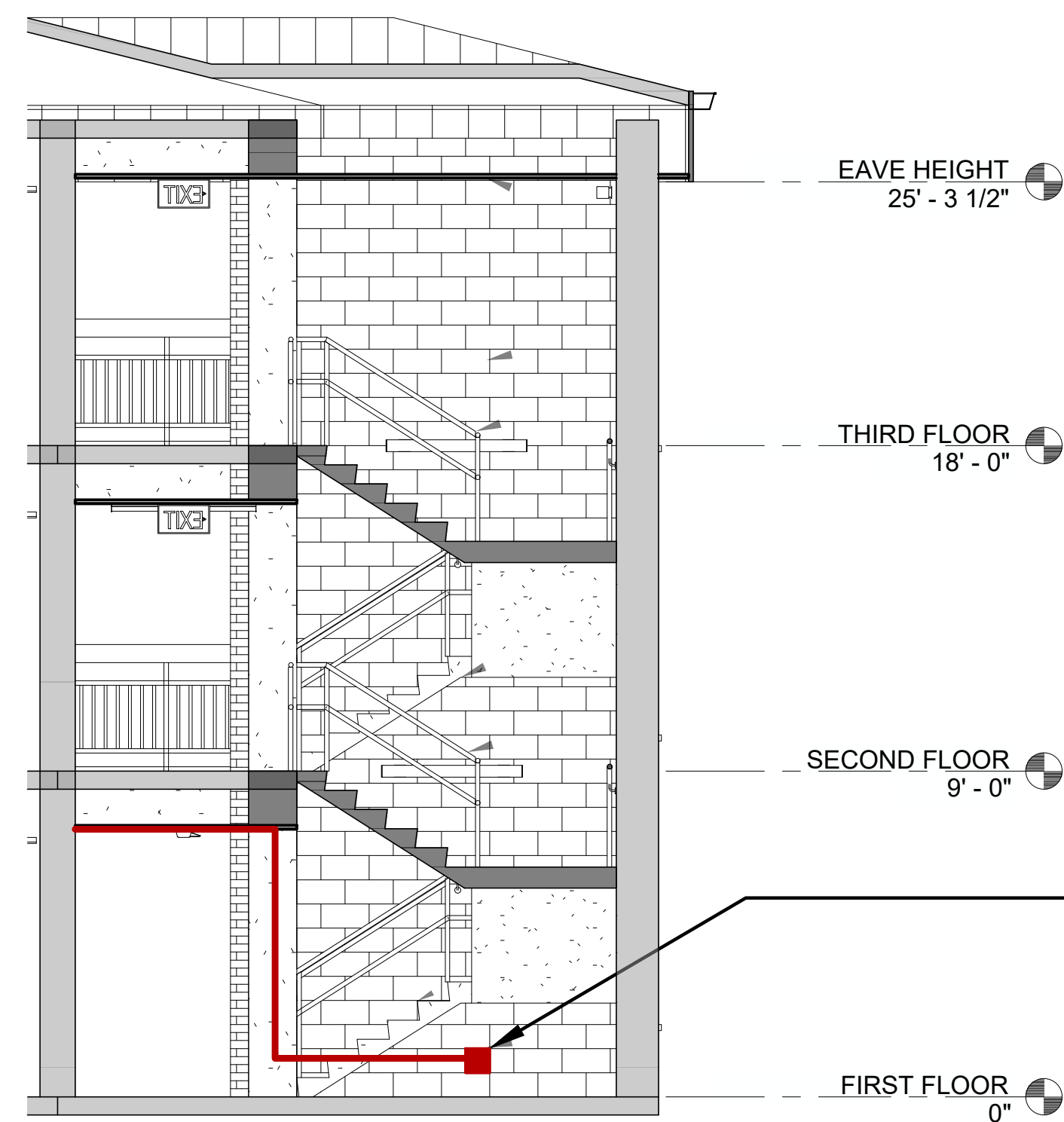
4 ENLARGED STAIR SECTION -TYPICAL AE403 1/4" - 1'-0"
