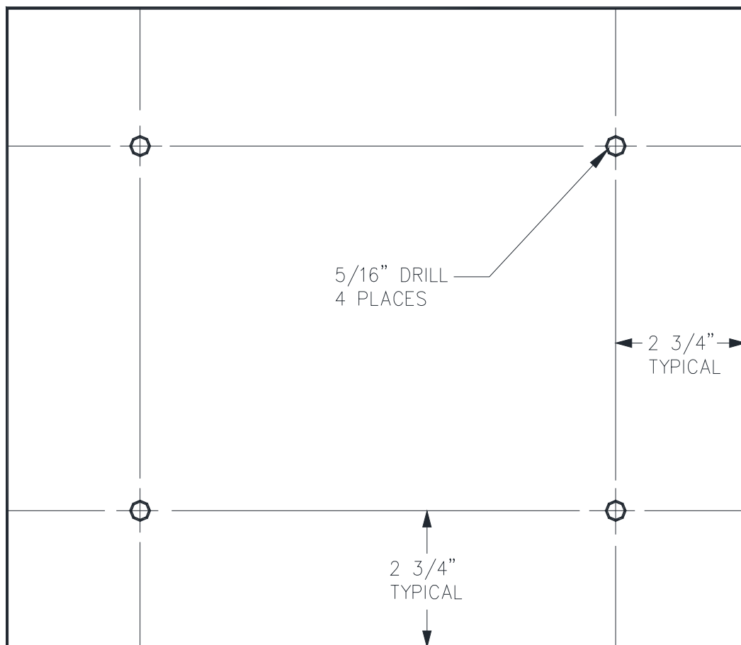
BASE INSERT (5) DETAIL "A"
