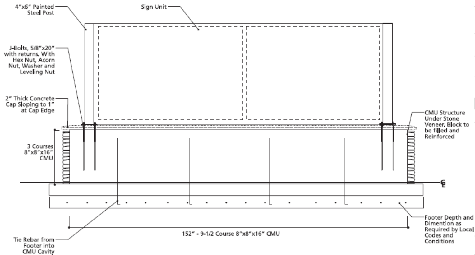
1 - 1.0A Sign Front Elevation
