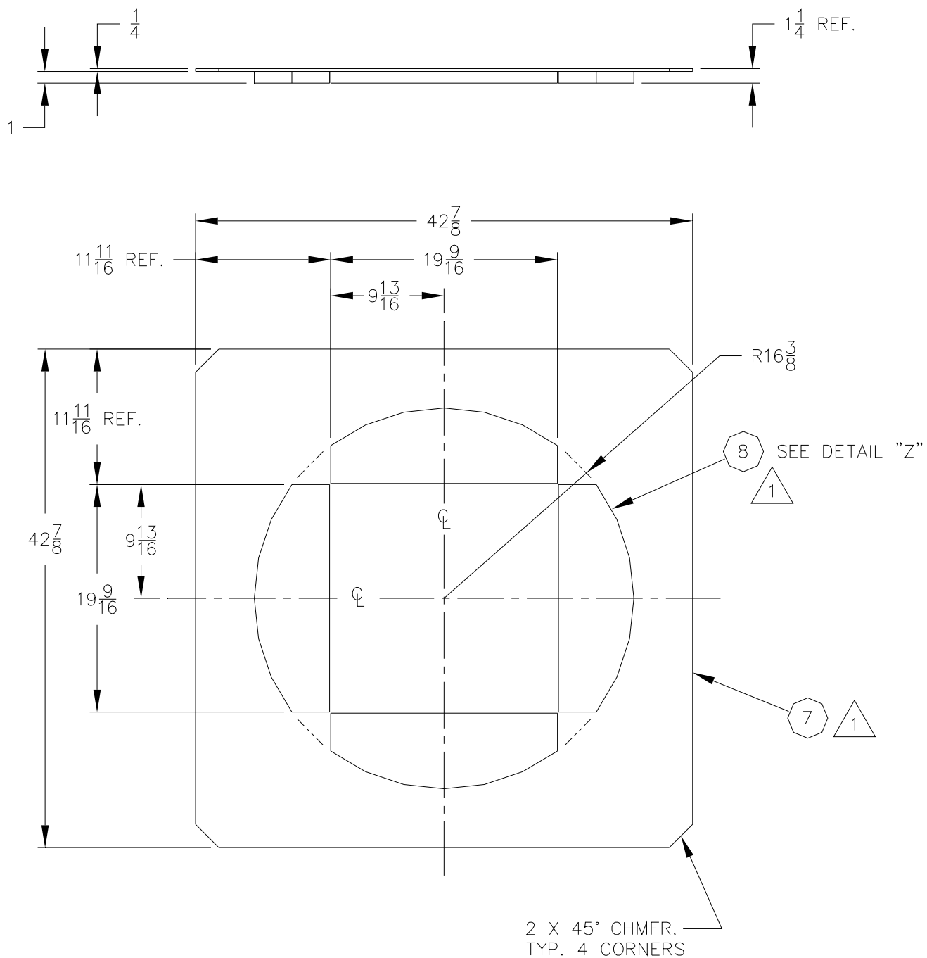
DETAIL "B"
