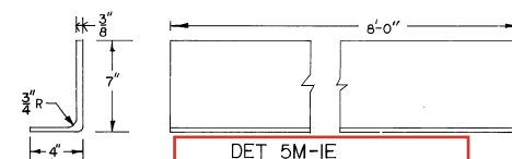
DET 5M-IE DMGT1/GTM204 SCALE: 3'-0" (INSTL DET SHTS 3J & 3K) CUT TO SUIT AT INSTALL
