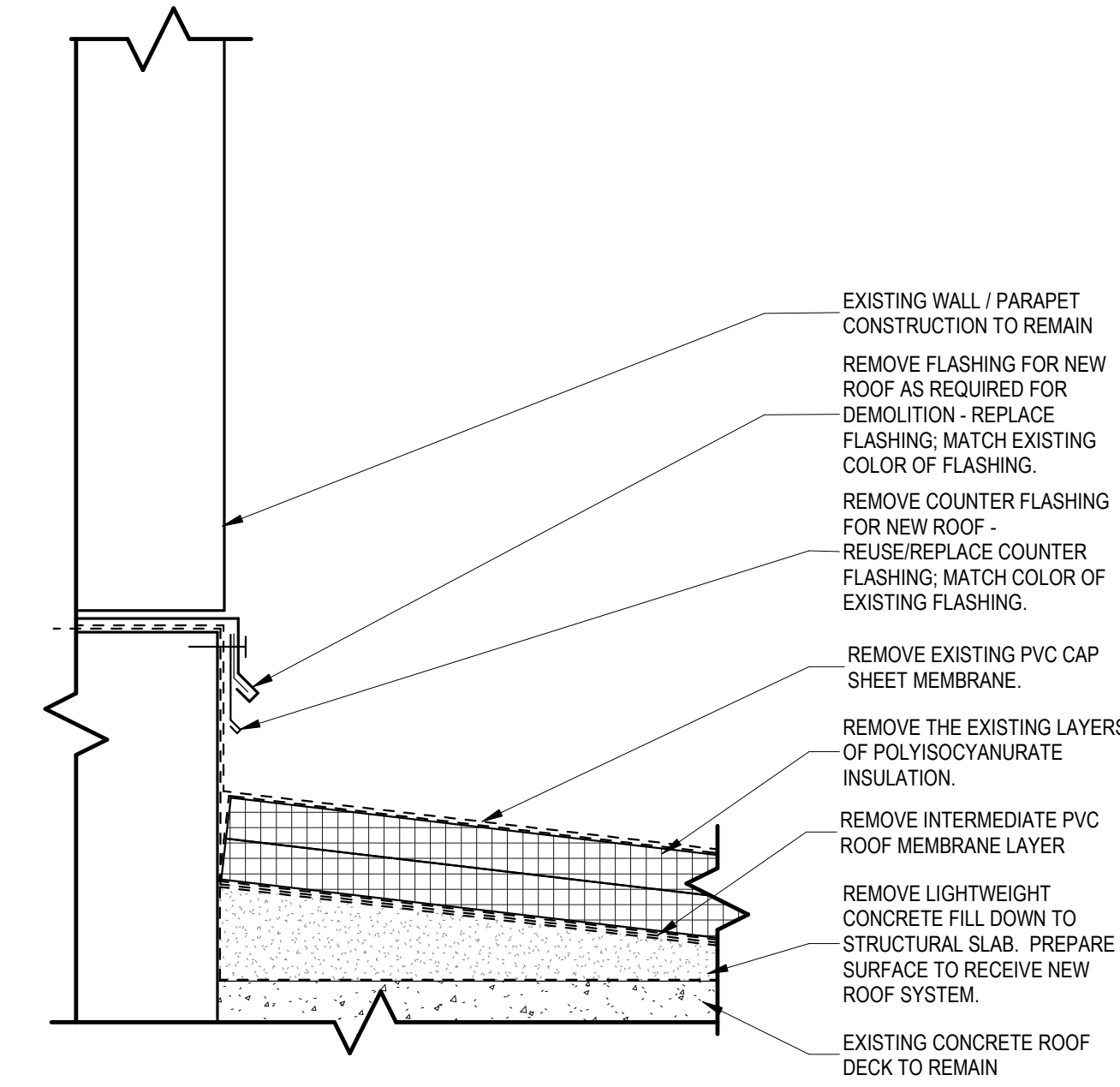
7 EXISTING ROOF 5 - TYPICAL DEMOLITION 3" = 1'-0"
