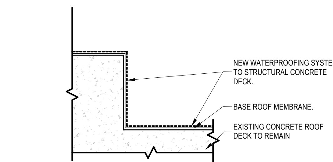
6 ROOF STEP UP WITHOUT PAVERS 1 1/2" = 1'-0"
