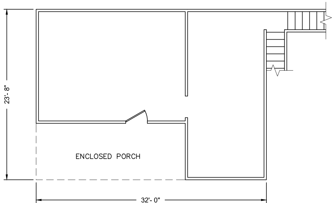
MAIN LEVEL FLOORPLAN
