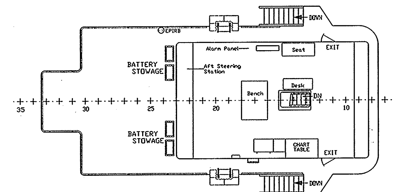
WHEELHOUSE
