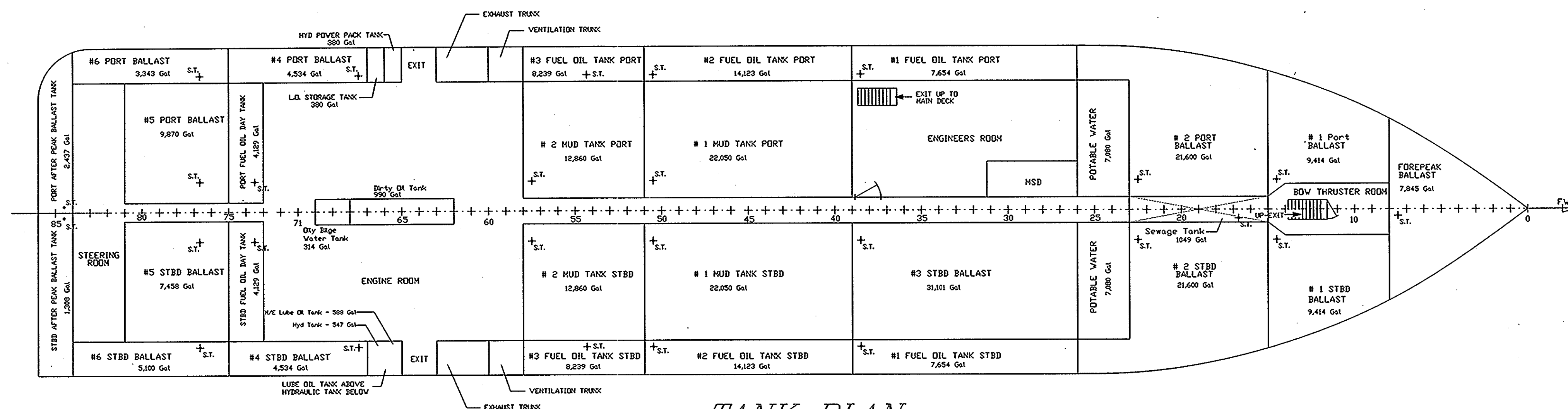
TANK PLAN
