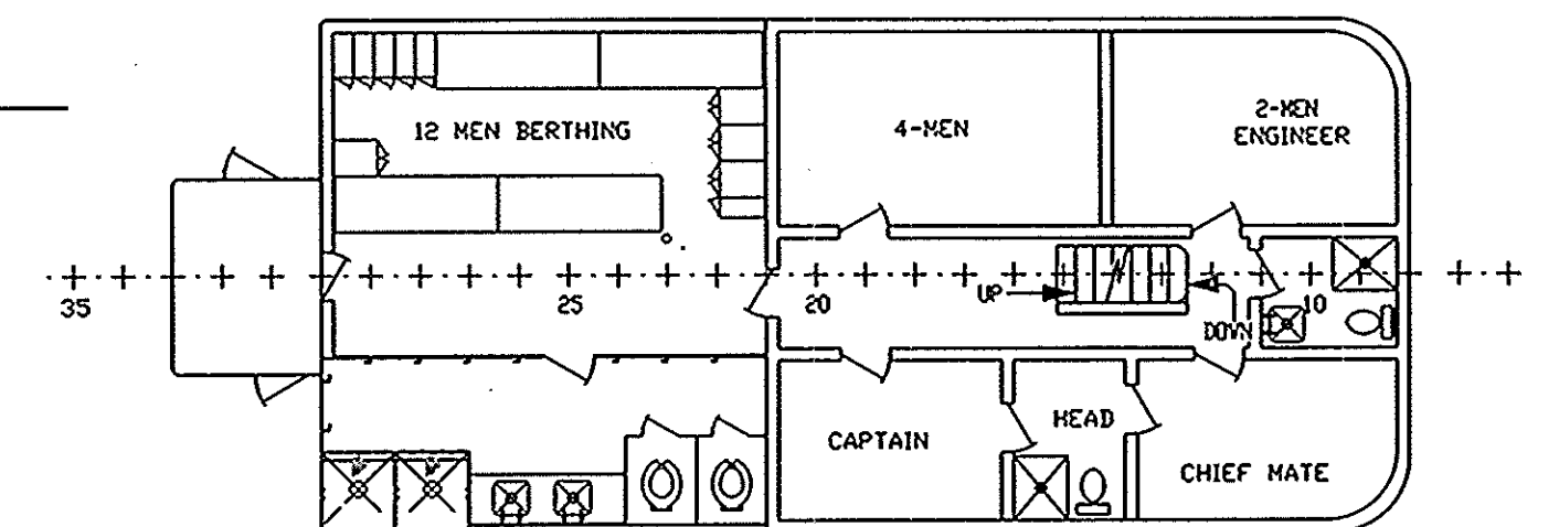
01 LEVEL
