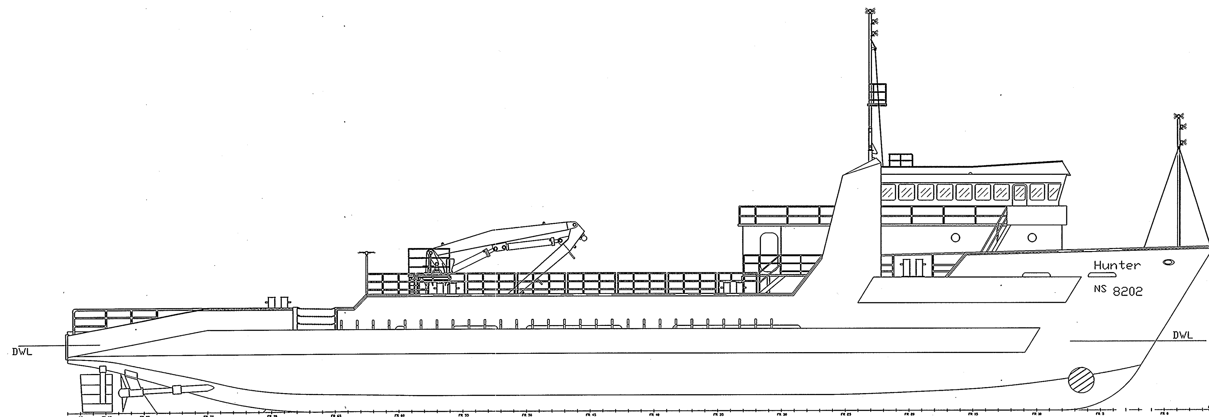
STBD PROFILE
