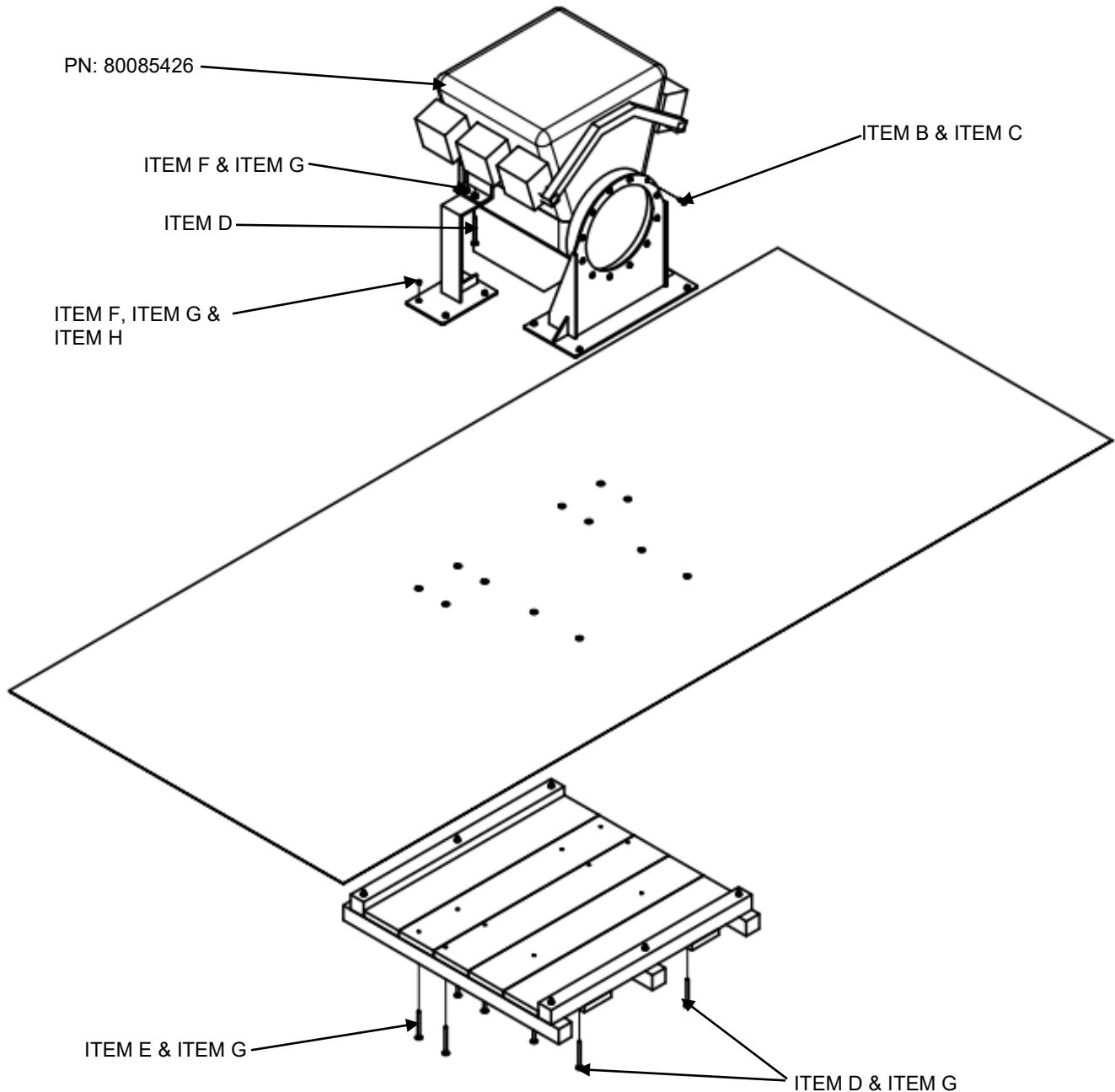
FIGURE 5 PART PLACEMENT ON CRATE BASE
