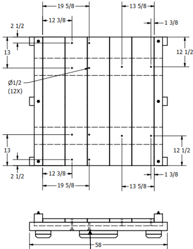
FIGURE 3 BASE SLEEPER BOARD AND HOLE LOCATIONS
