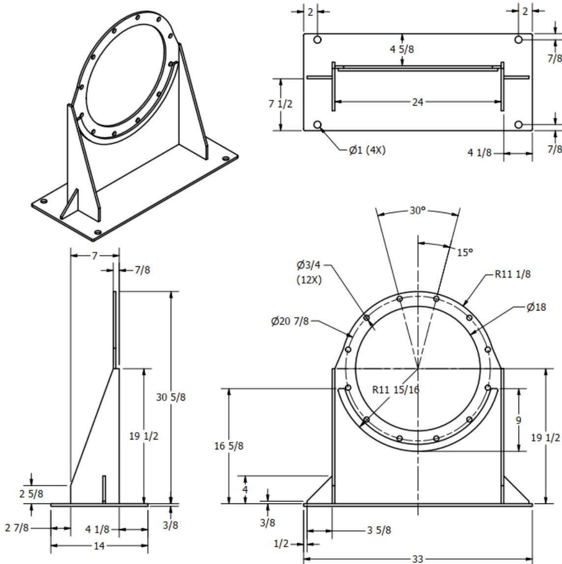
FIGURE 1 FRONT BRACKET VIEW (BRACKETS ARE TO BE CONSTRUCTED FROM 3/8" STEEL)
