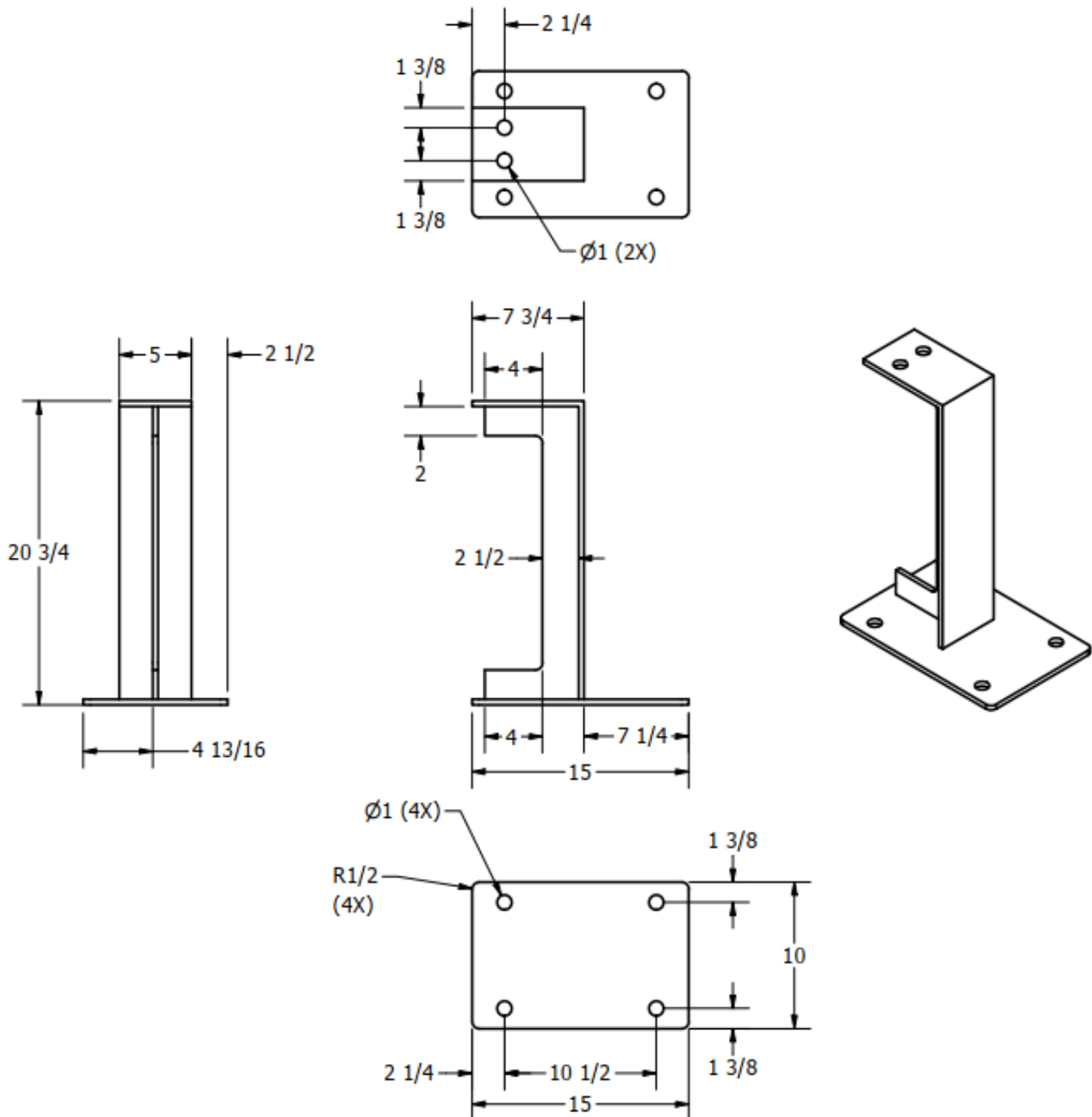
FIGURE 2 REAR BRACKET VIEW (BRACKETS TO BE CONSTRUCTED FROM 3/8" STEEL)
