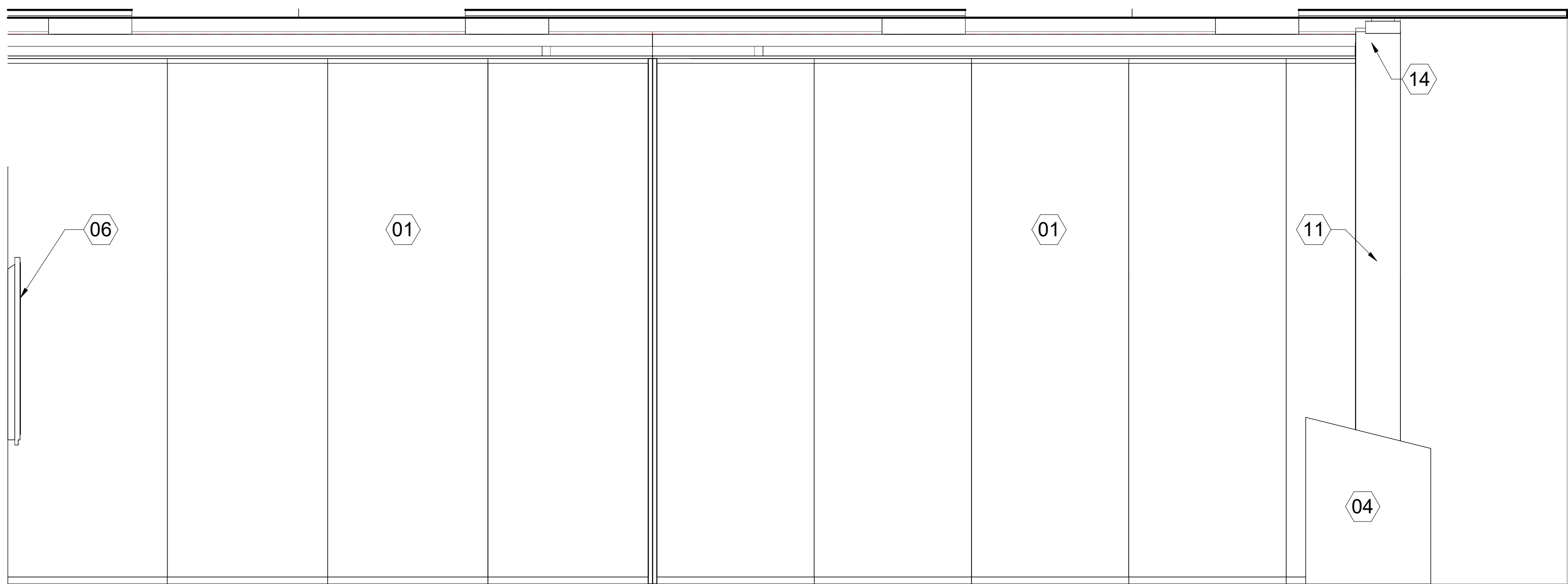
(F1) 1H122-EAST ELEVATION 1/2" = 1'-0"
