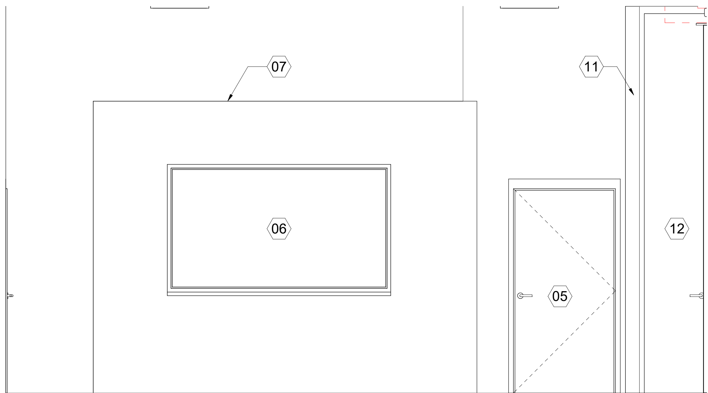
(F6) 1H122-NORTH ELEVATION 1/2" = 1'-0"
