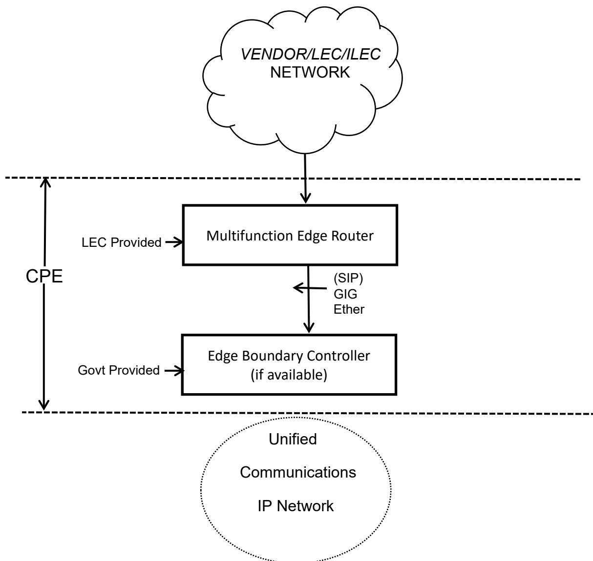
Diagram 2 UTILIZING SIP TRUNKING
