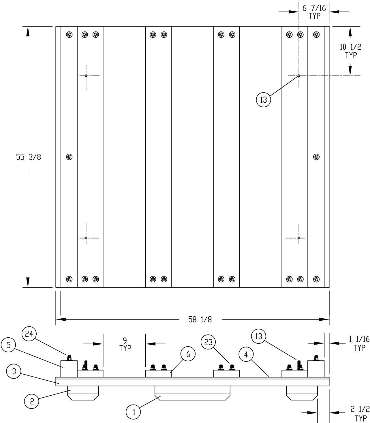
DETAIL NO. 2
