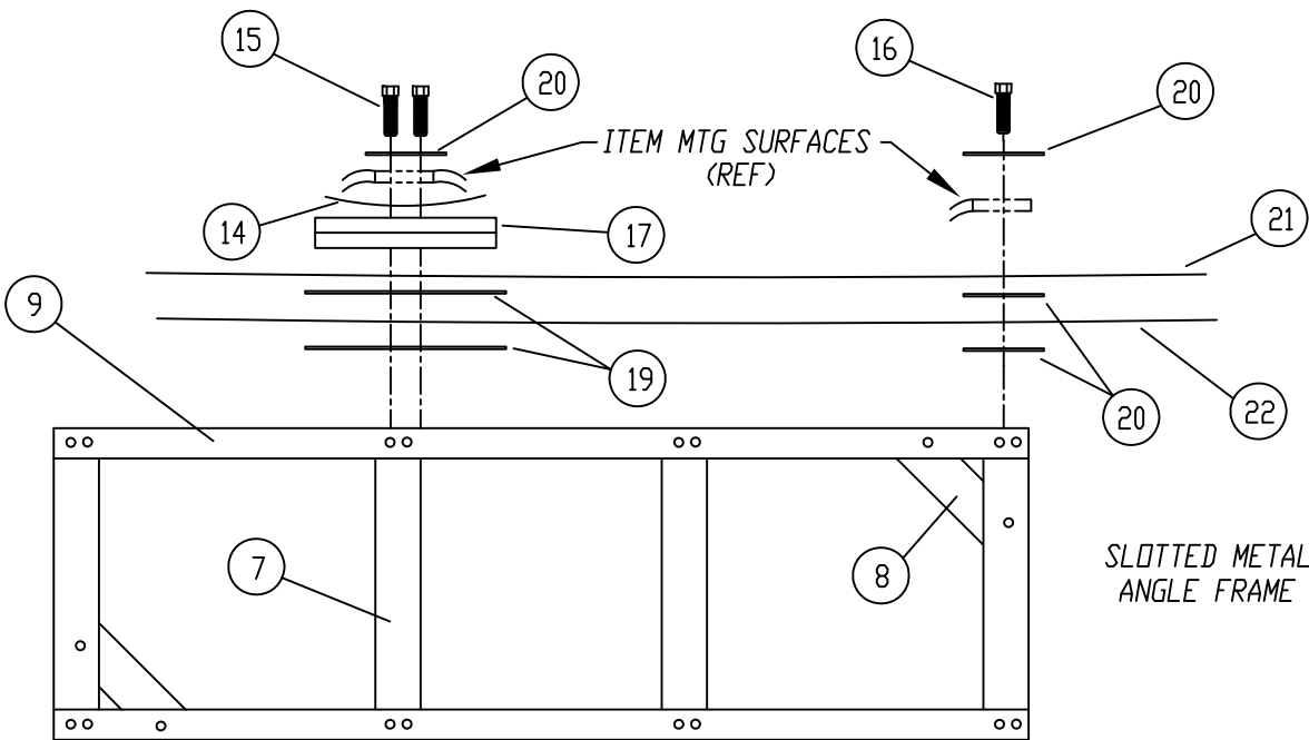
DETAIL NO. 3
