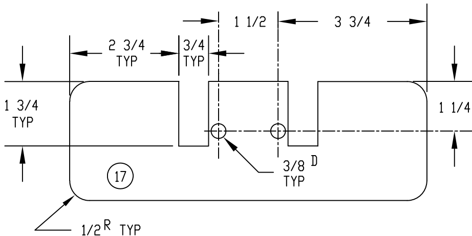
DETAIL NO. 4
