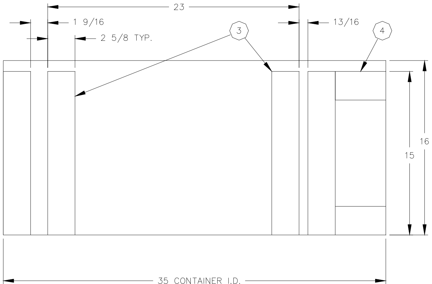
DETAIL "C"
