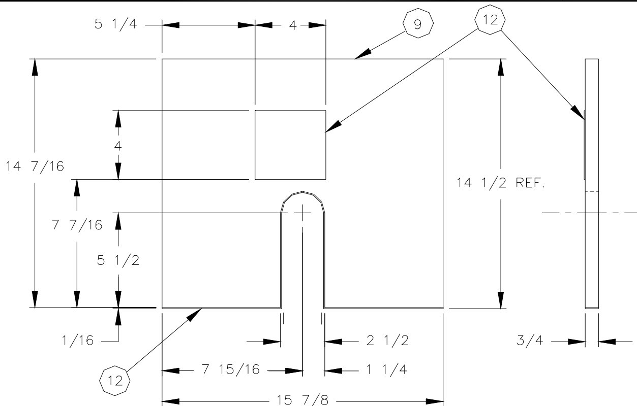
DETAIL "D"
