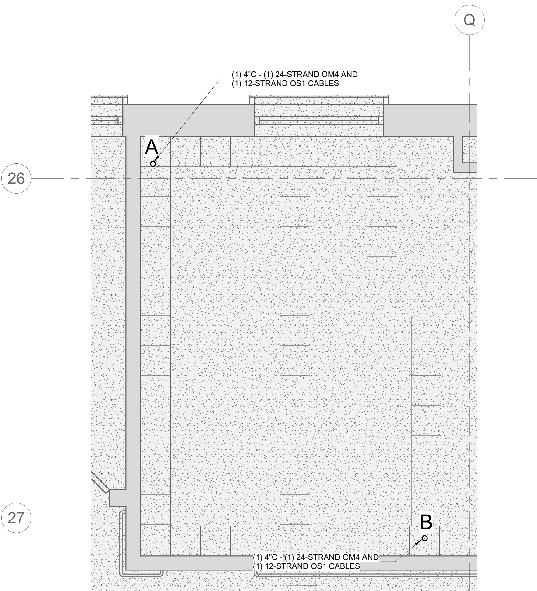
NORTH 4 1/2" = 1'-0" TELECOM ROOM PATHWAY TR #C506
