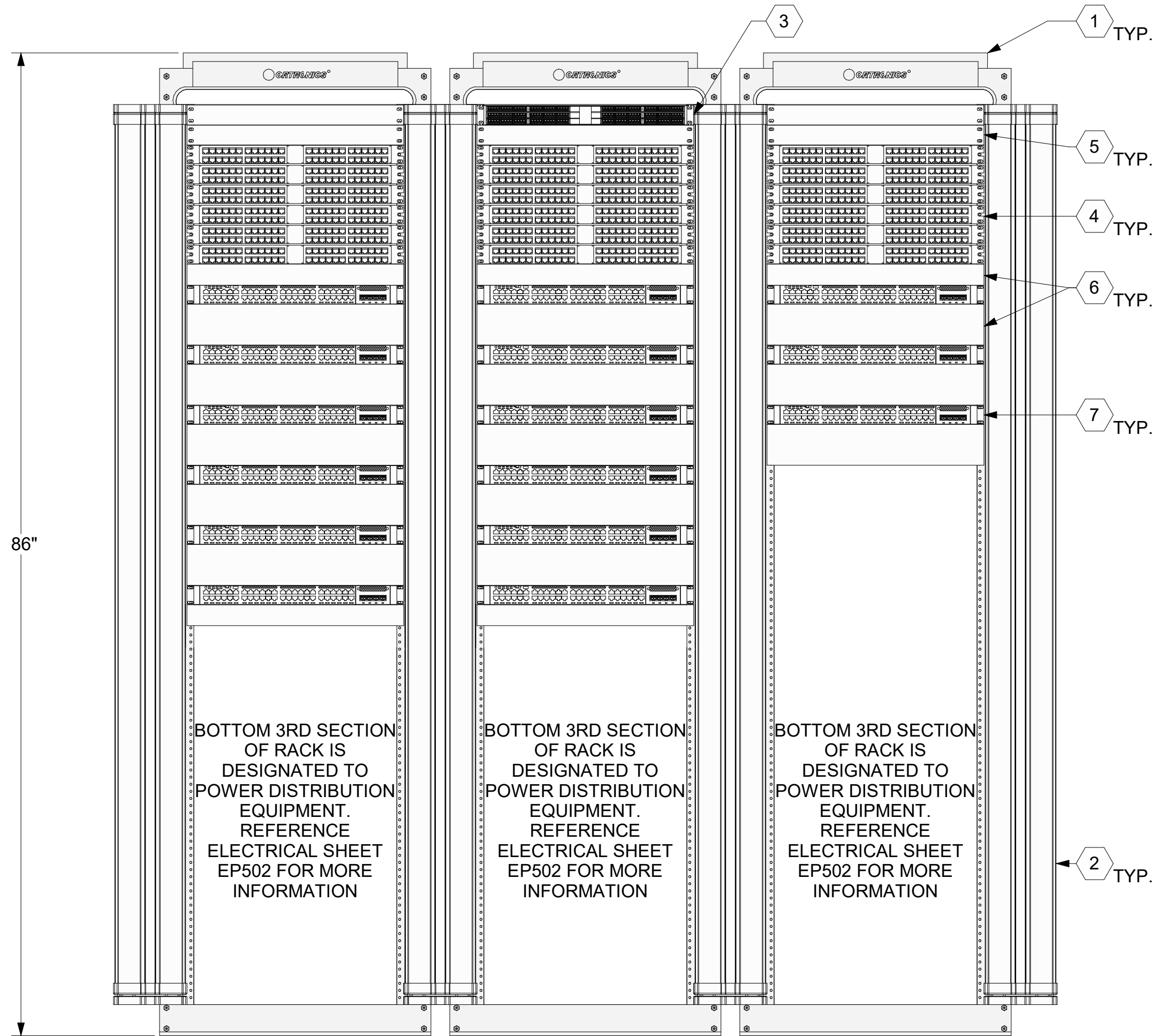
1 TR DATA RACK ELEVATION - THREE RACK 1" = 0'-9"
