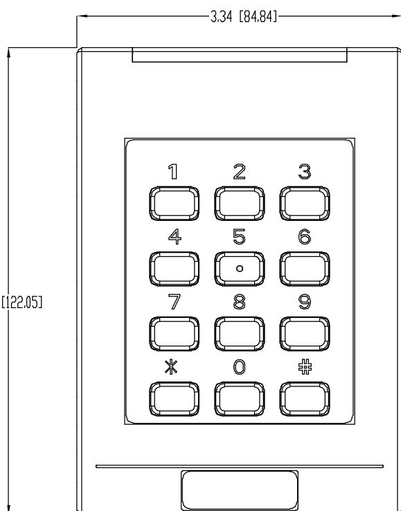
3 TYPICAL CONTACTLESS AUTHENTICATION AND PINPAD DEVICE NTS
