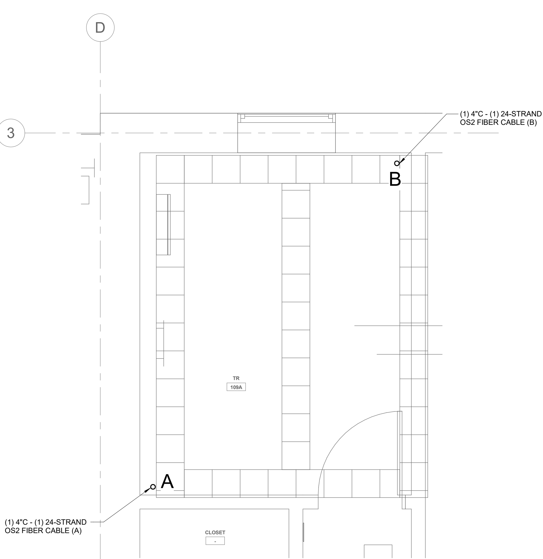
2 TELECOM ROOM PATHWAY TR #109A 1/2" = 1'-0"
