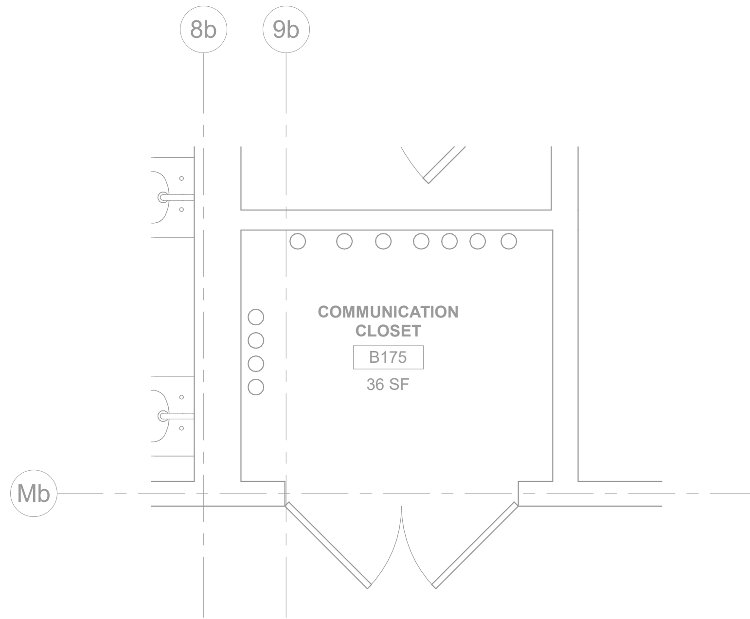
4 RM B175 - OVERHEAD PLAN 148TN101A 1/2" = 1'-0"
