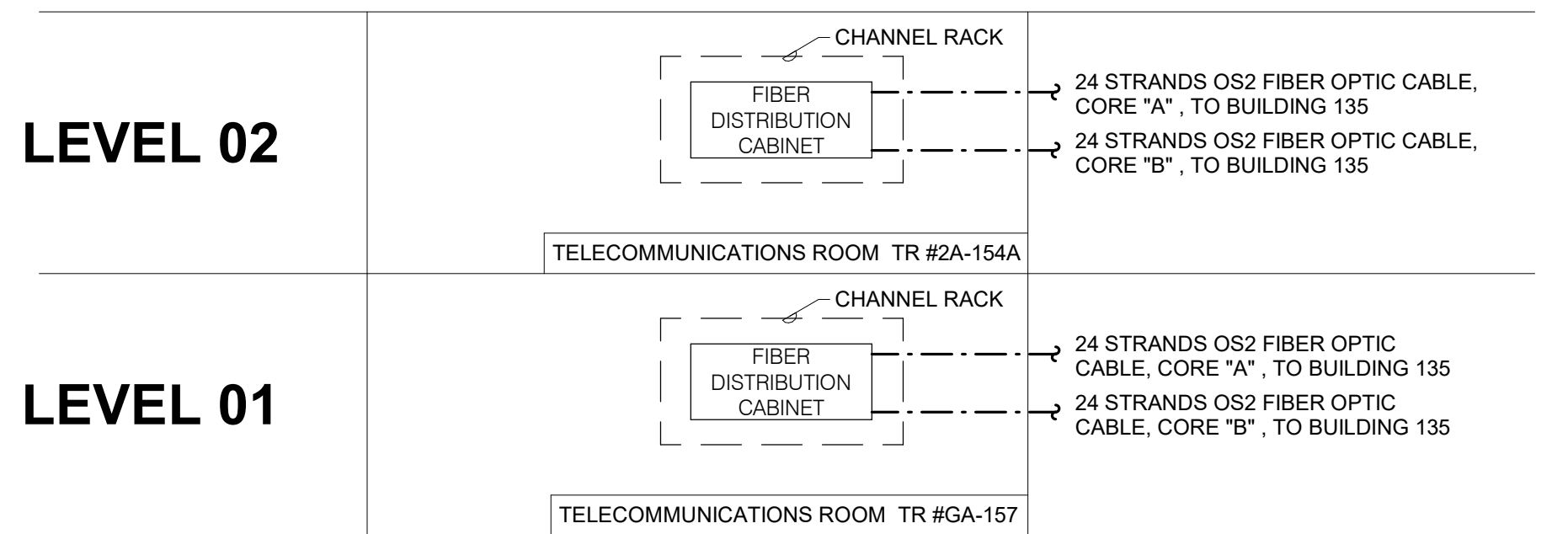
3 FIBER RISER DIAGRAM NO SCALE
