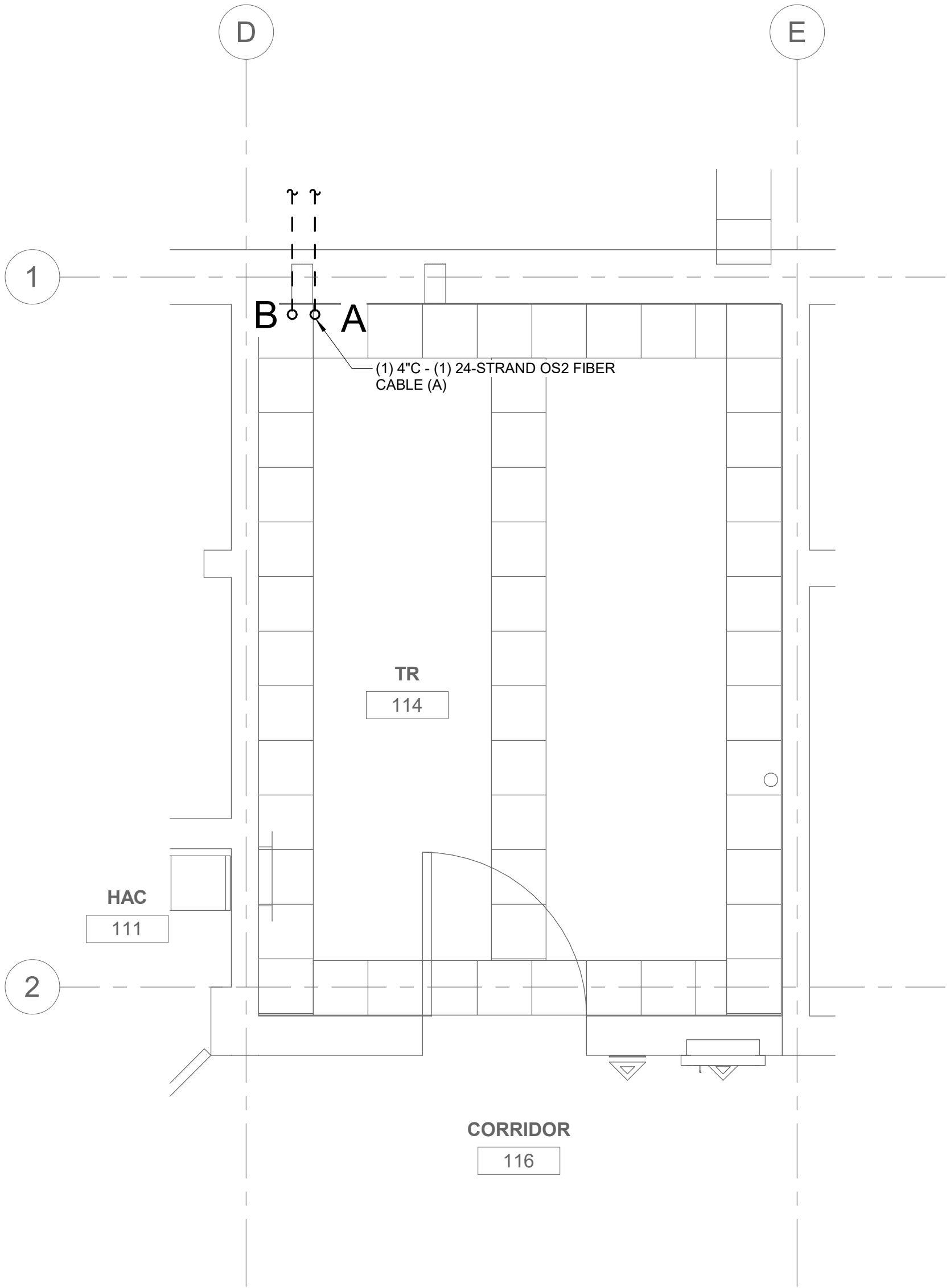
2 TELECOM ROOM PATHWAY TR #114 1/2" = 1'-0"
