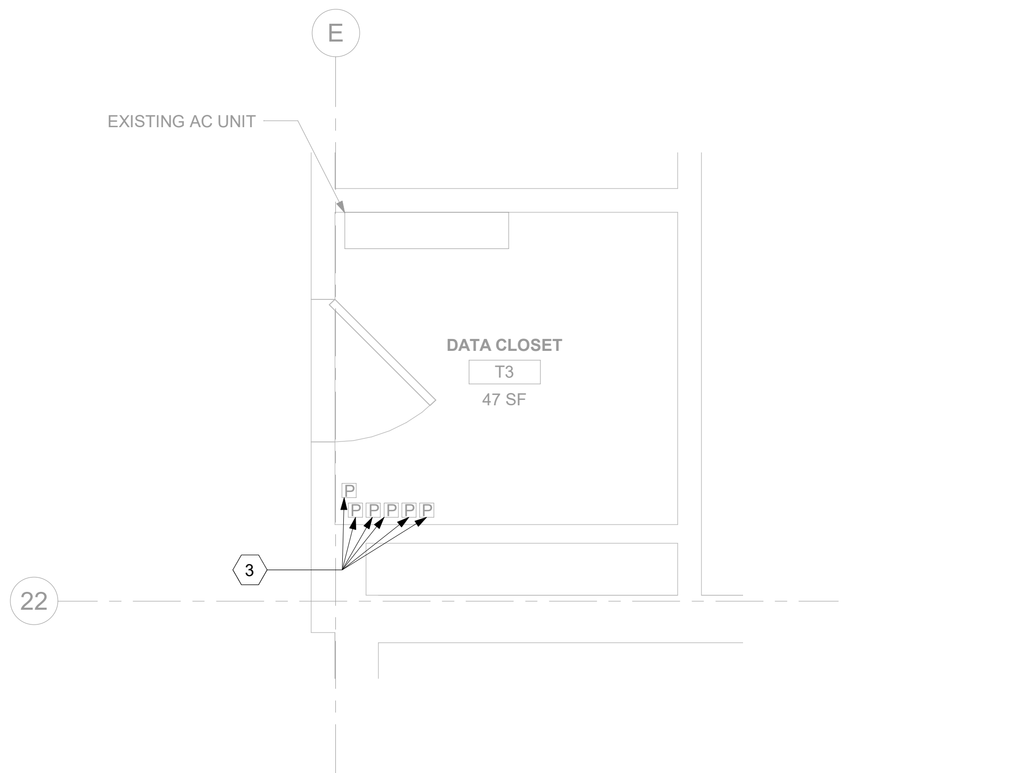
3 RM T3 - DEMOLITION OVERHEAD PLAN 146TN101A 1/2" = 1'-0"
