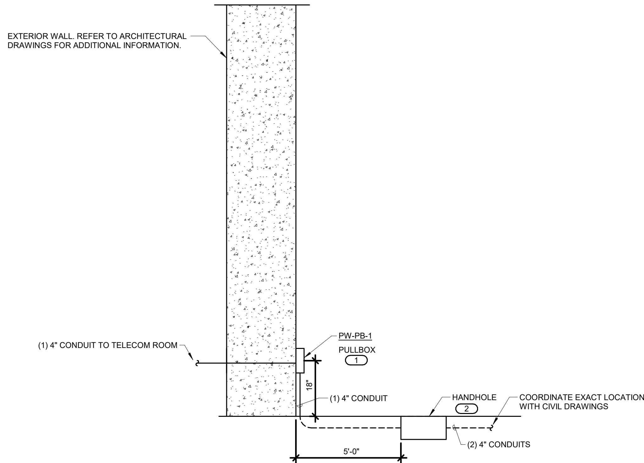
2 EXTERIOR PATHWAY DETAIL (LOW HEIGHT) NO SCALE NOTES: 1. REFER TO CIVIL DRAWINGS FOR EXACT LOCATION OF HANDHOLES. KEYNOTES: # 1. CONTRACTOR TO COORDINATE JUNCTION BOX ELEVATIONS. 2. REFER TO 2/T400 EXTERIOR HAND HOLE DETAIL FOR ADDITIONAL INFORMATION.
