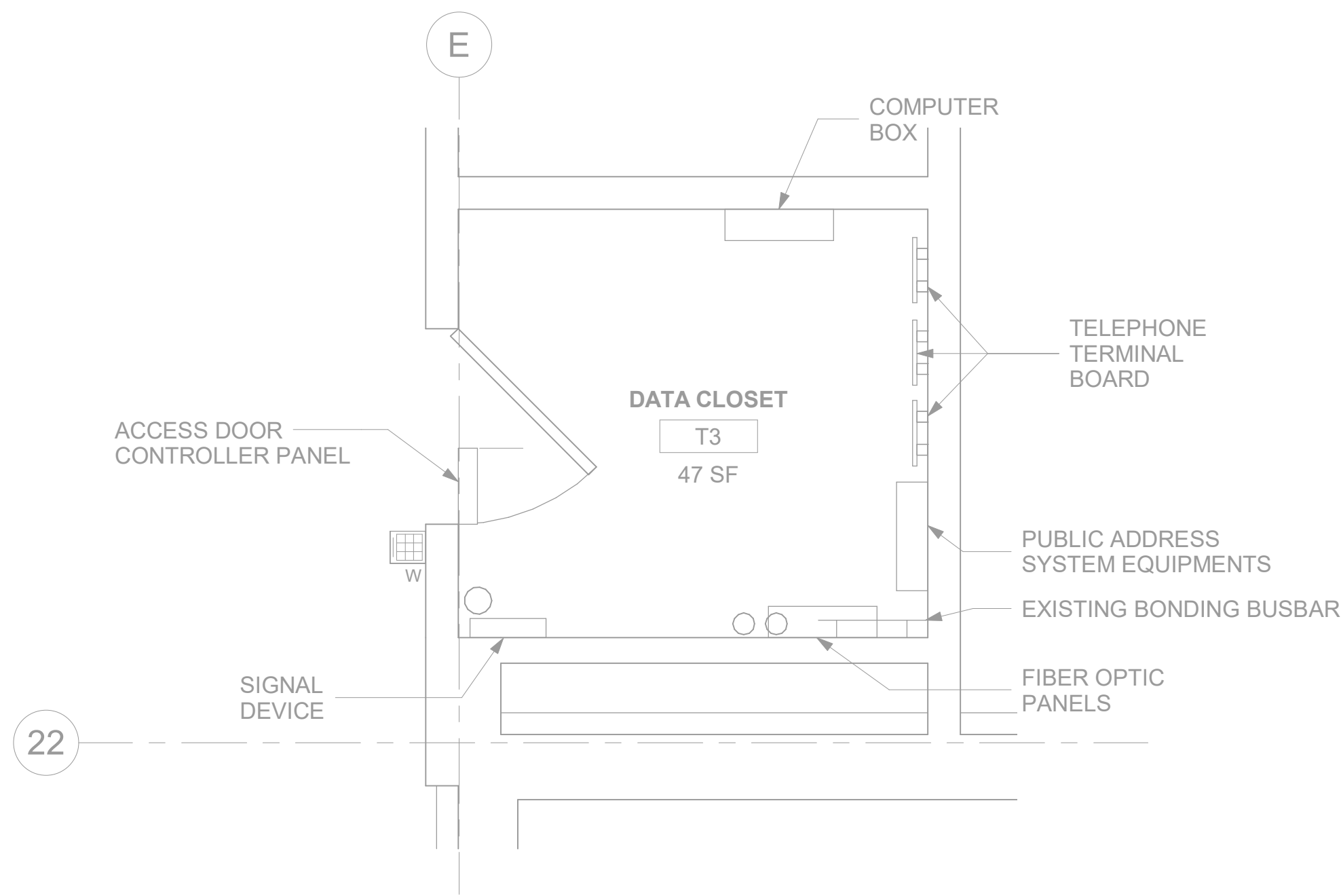
2 RM T3 - TELECOMMUNICATIONS PLAN 146TN101A 1/2" = 1'-0"
