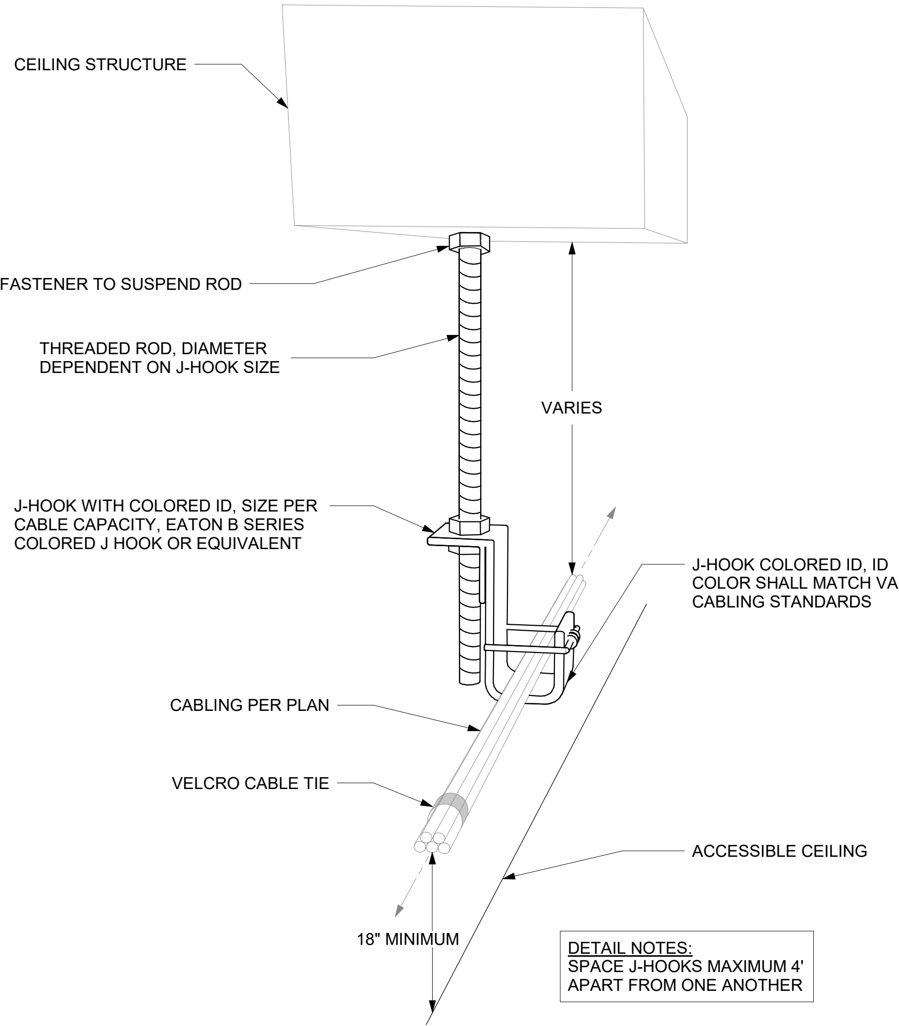
1 TYPICAL J-HOOK INSTALLATION DETAIL NTS
