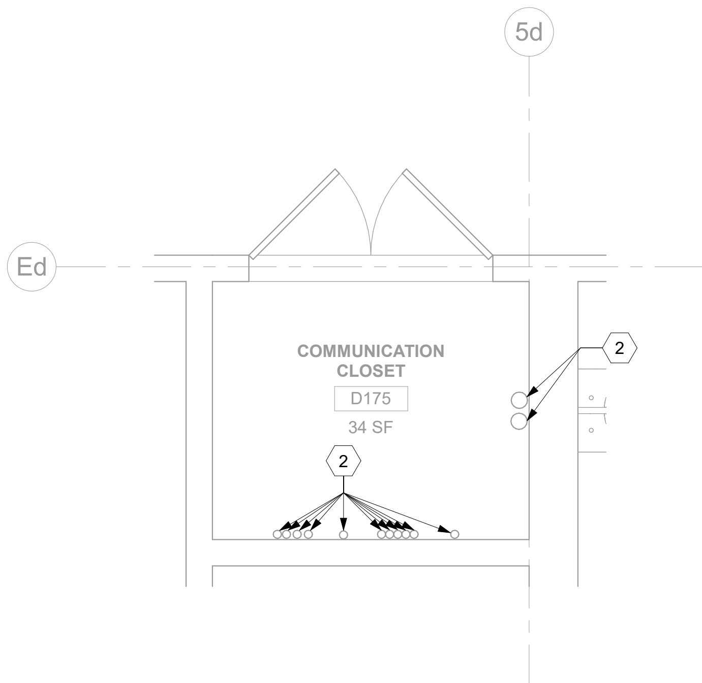
3 RM D175 - DEMOLITION OVERHEAD PLAN 148TN101A 1/2" = 1'-0"
