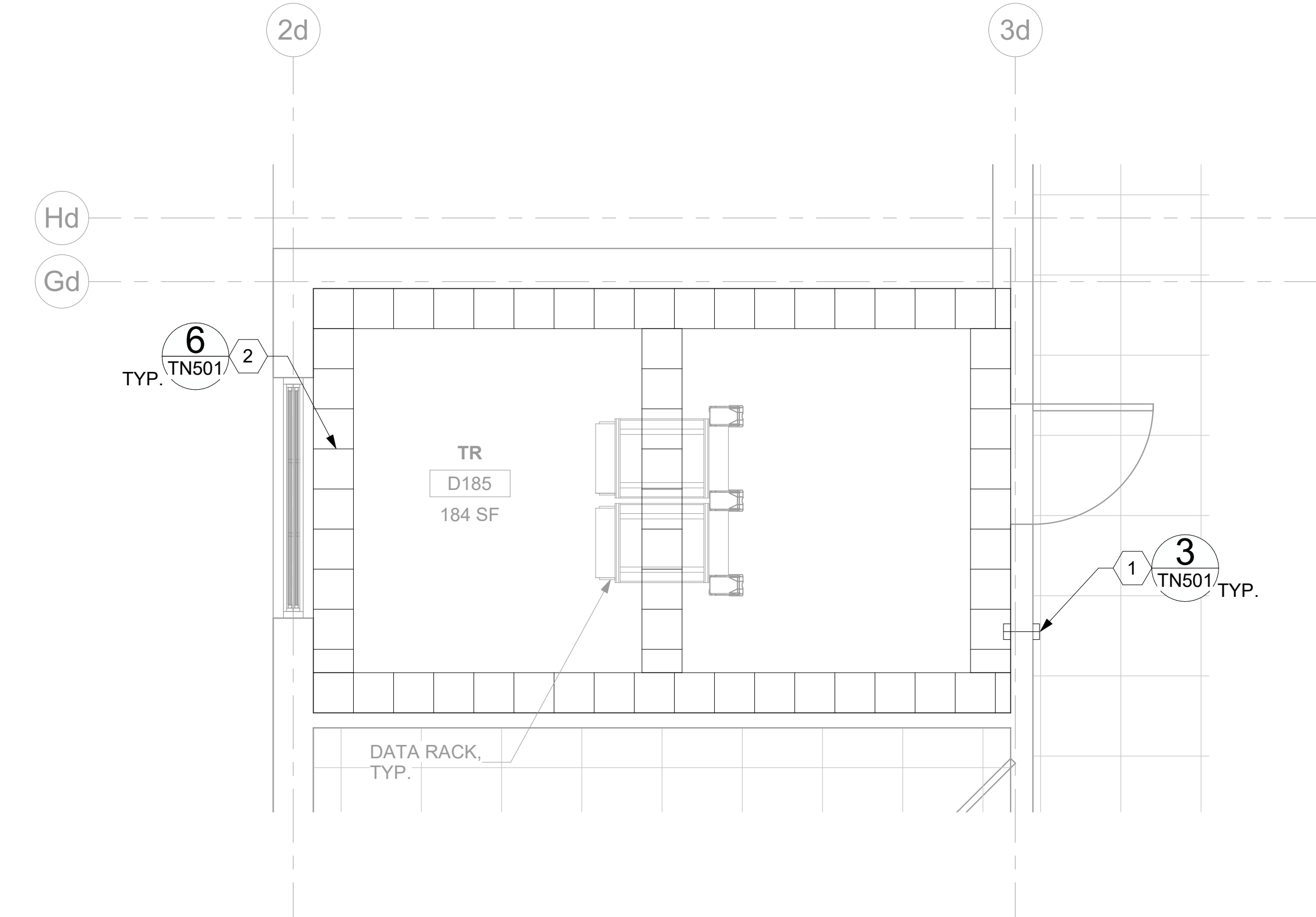
2 RM D185 - TELECOMMUNICATIONS PLAN
