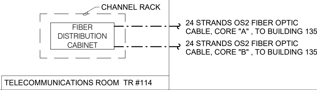
3 FIBER RISER DIAGRAM NO SCALE NOTES: 1. THIS RISER IS DIAGRAMMATIC AND MAY NOT SHOW ACTUAL ROUTING OR QUANTITIES OF MATERIALS SHOWN. THIS RISER IS SHOWN FOR CLARIFICATION OF CONNECTION(S), LOCATIONS AND CABLE TYPE. ALL INFORMATION OUTLETS ARE TYPICAL OF THE OUTLETS IN THE AREA SHOWN. REFER TO FLOOR PLANS FOR MORE SPECIFIC ROUTING INFORMATION. REFER TO SPECIFICATIONS FOR ADDITIONAL REQUIREMENTS. 2. REFER TO ELECTRICAL DRAWINGS FOR CHANNEL RACK AND FIBER OPTIC DISTRIBUTION CABINET SPECIFICATIONS
