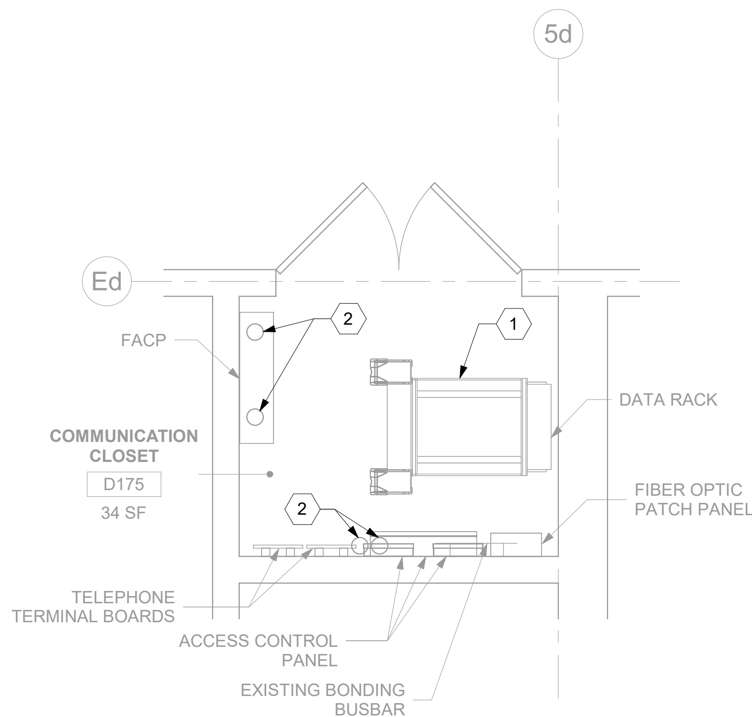
1 RM D175 - DEMOLITION FLOOR PLAN 148TN101A 1/2" = 1'-0"
