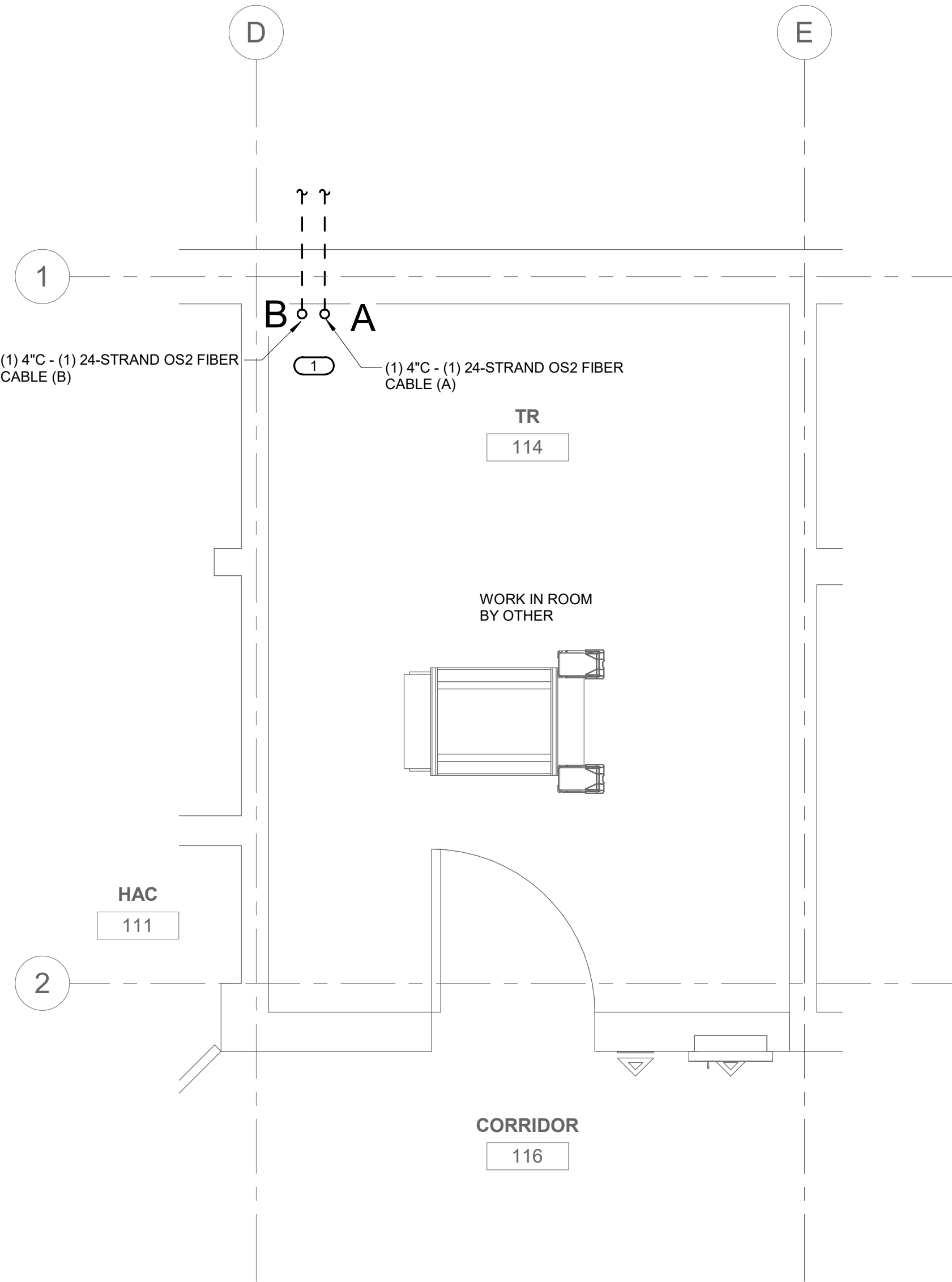
1 TELECOM ROOM ENLARGEMENT TR #114 1/2" = 1'-0" NOTES: 1. REFER TO ELECTRICAL DRAWINGS FOR ROOM LAYOUT AND RACK ELEVATIONS. 2. ROUTE OPTICAL FIBER CABLE TO OVERHEAD CABLE TRAY AND TERMINATE IN FIBER DISTRIBUTION CABINET. KEY NOTES: # 1. THROUGH WALL PENETRATION FOR BACKBONE CONDUIT. OPTICAL FIBER CABLE CONTINUES ON CABLE TRAY TO RACKS.
