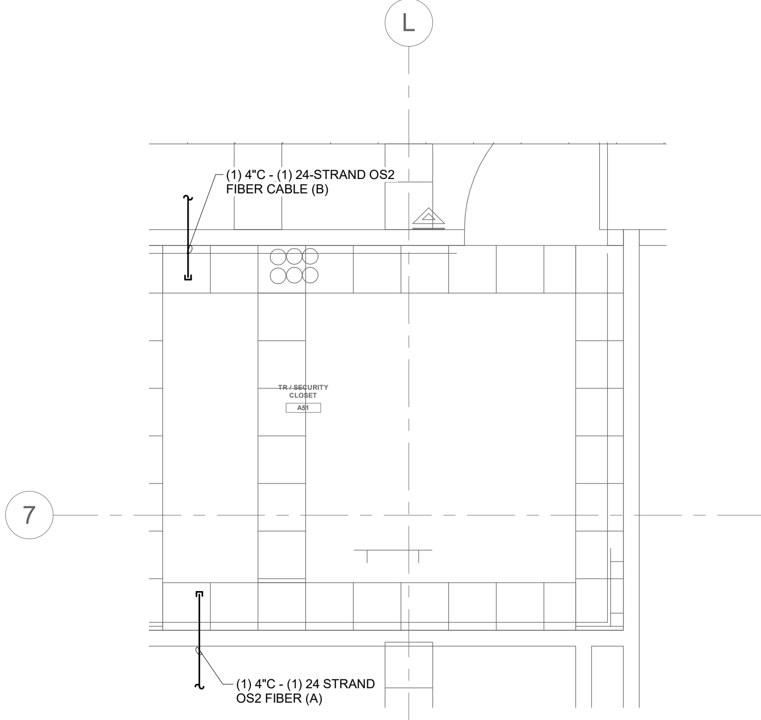
2 TELECOM ROOM PATHWAY TR #A51 1/2" = 1'-0"
