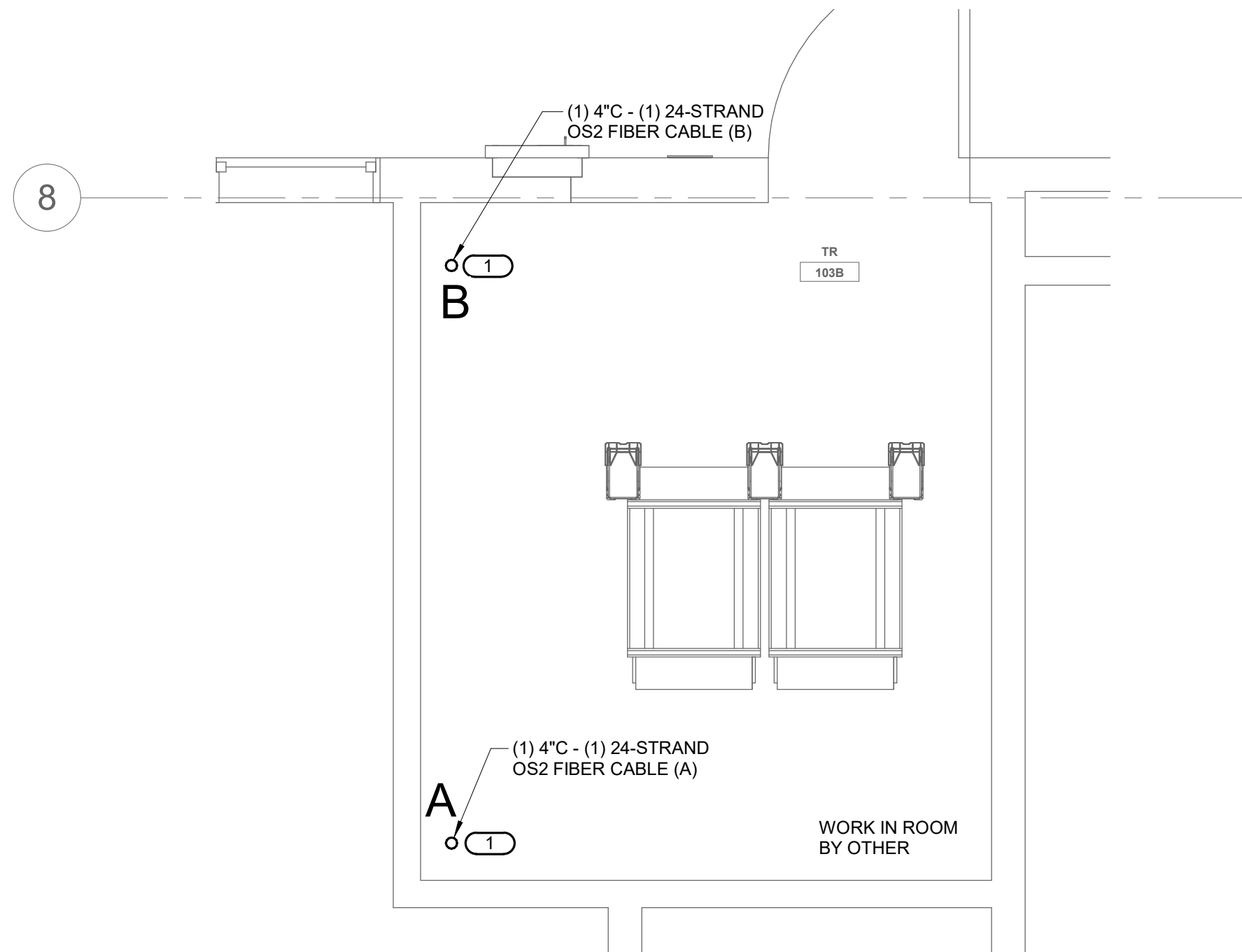
1 TELECOM ROOM ENLARGEMENT TR #103B 1/2" = 1'-0" NOTES: 1. REFER TO ELECTRICAL DRAWINGS FOR ROOM LAYOUT AND RACK ELEVATIONS. 2. ROUTE OPTICAL FIBER CABLE TO OVERHEAD CABLE TRAY AND TERMINATE IN FIBER DISTRIBUTION CABINET. KEY NOTES: (B) 1. THROUGH FLOOR PENETRATION FOR BACKBONE CONDUIT. OPTICAL FIBER CABLE CONTINUES ON CABLE TRAY TO RACKS.
