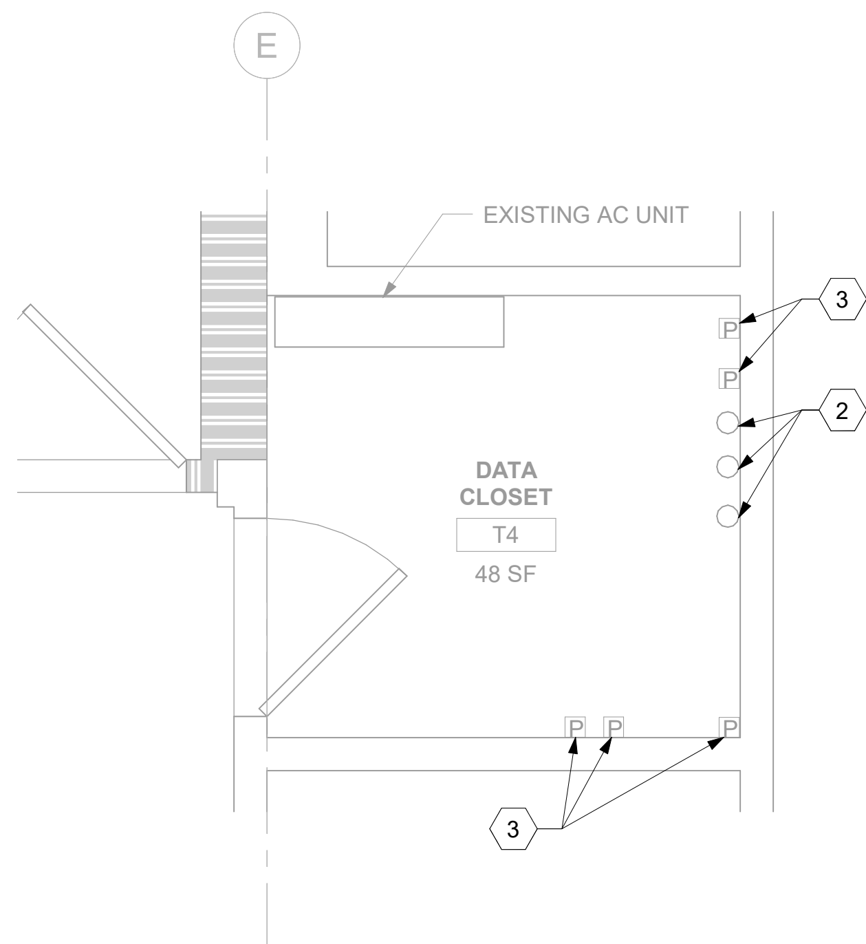
3 RM T4 - DEMOLITION OVERHEAD PLAN 146TN101A 1/2" = 1'-0"
