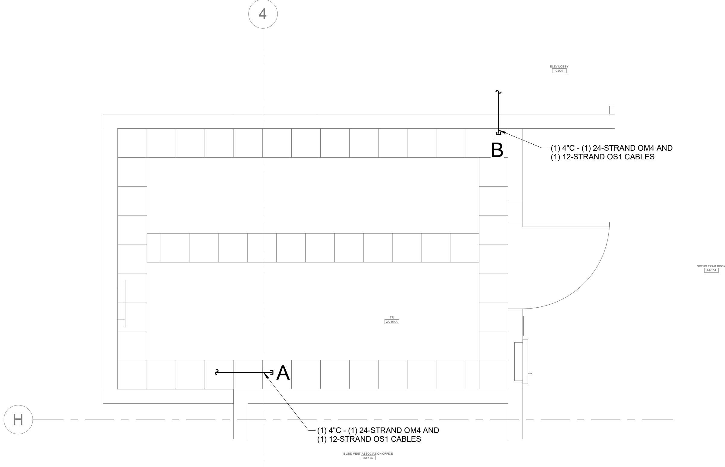
5 TELECOM ROOM PATHWAY TR #2A-154A 1/2" = 1'-0"
