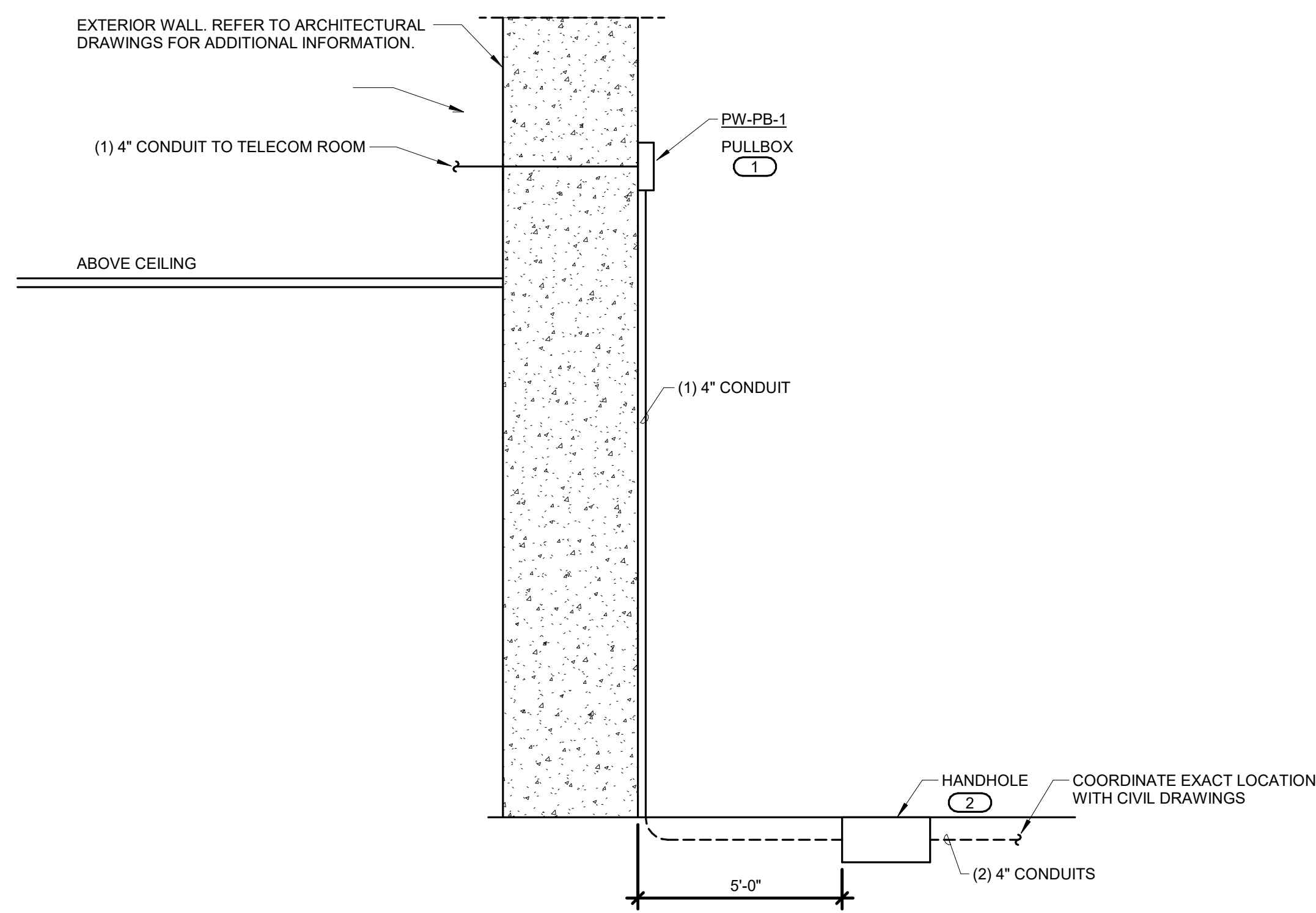
1 EXTERIOR PATHWAY DETAIL NO SCALE NOTES: 1. REFER TO CIVIL DRAWINGS FOR EXACT LOCATION OF HANDHOLES. KEYNOTES: # 1. CONTRACTOR SHALL FIELD VERIFY PULLBOX ELEVATION TO ROUTE CONDUITS INTO BUILDING ABOVE FINISHED CEILING. 2. REFER TO 2/T400 EXTERIOR HAND HOLE DETAIL FOR ADDITIONAL INFORMATION.
