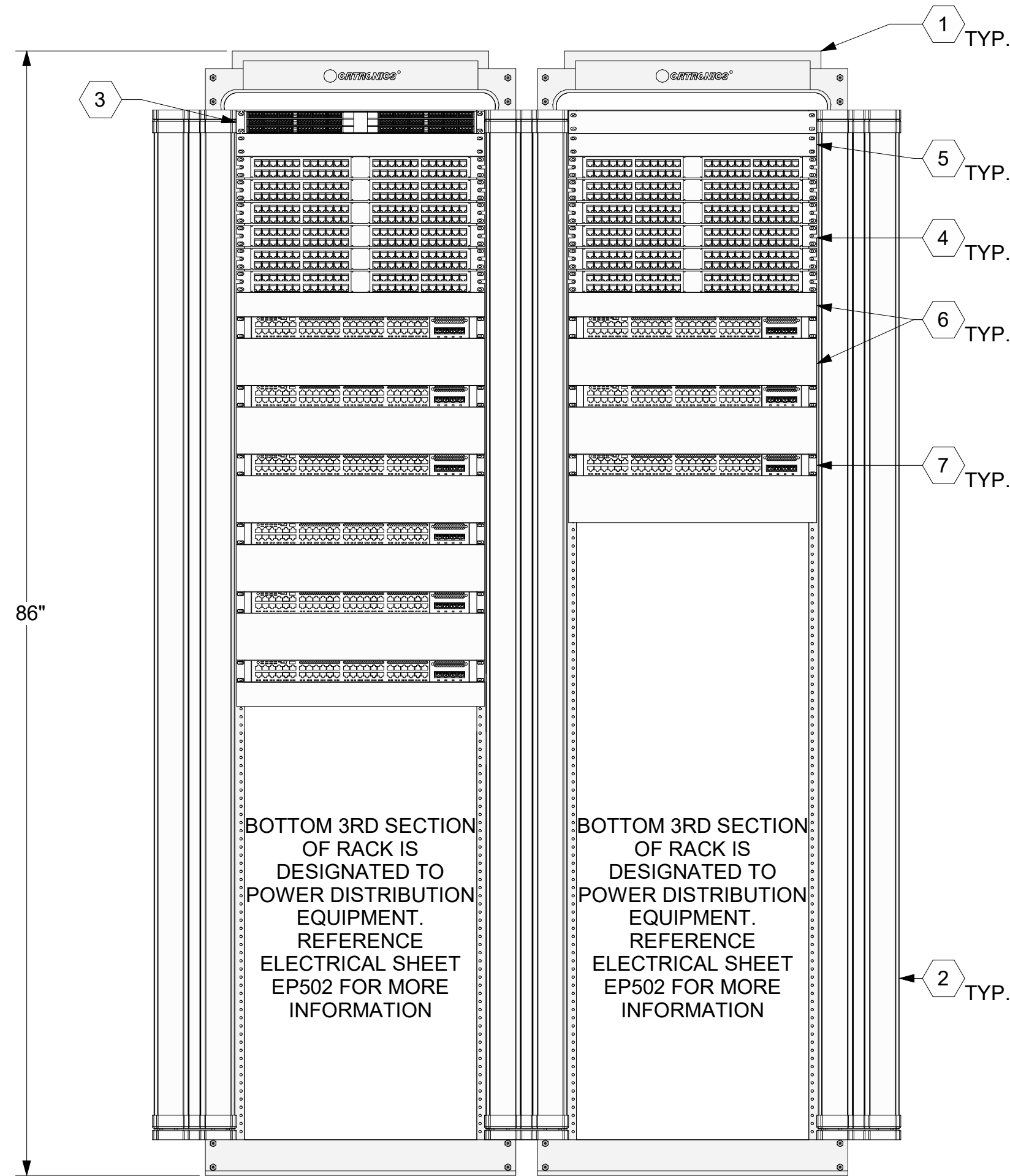
3 TR DATA RACK ELEVATION - TWO RACK 1" = 0'-9"
