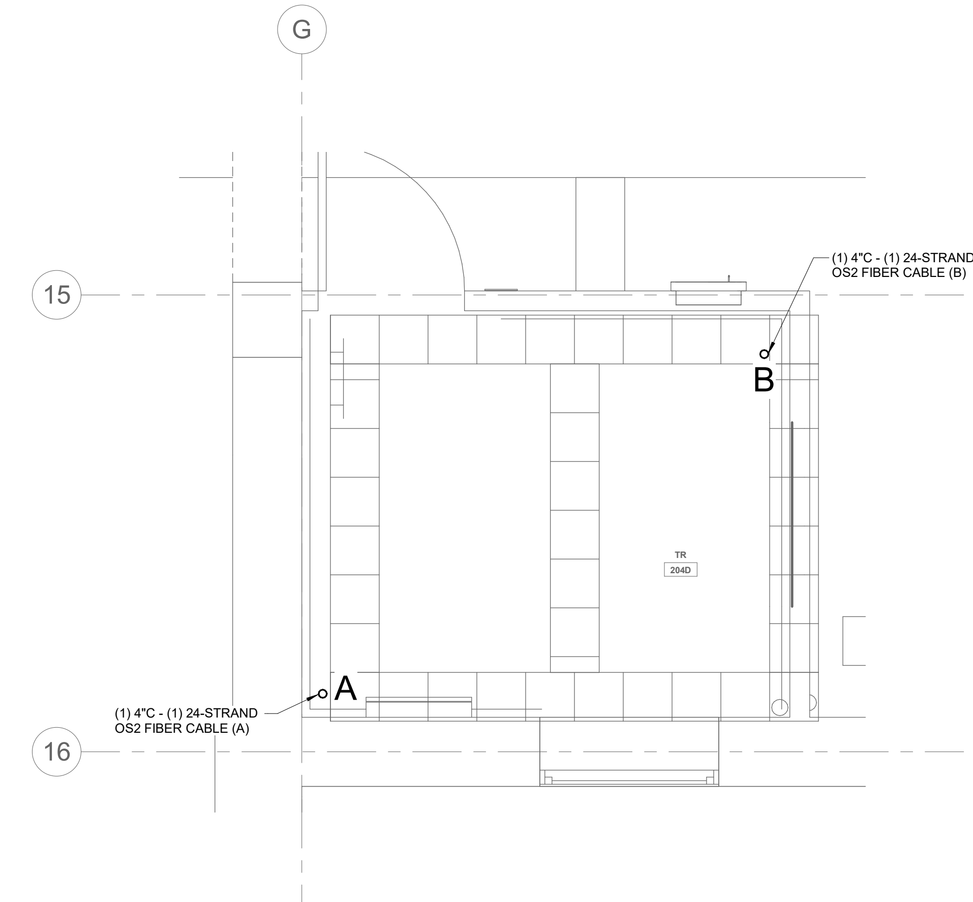
4 TELECOM ROOM PATHWAY TR #204D 1/2" = 1'-0"
