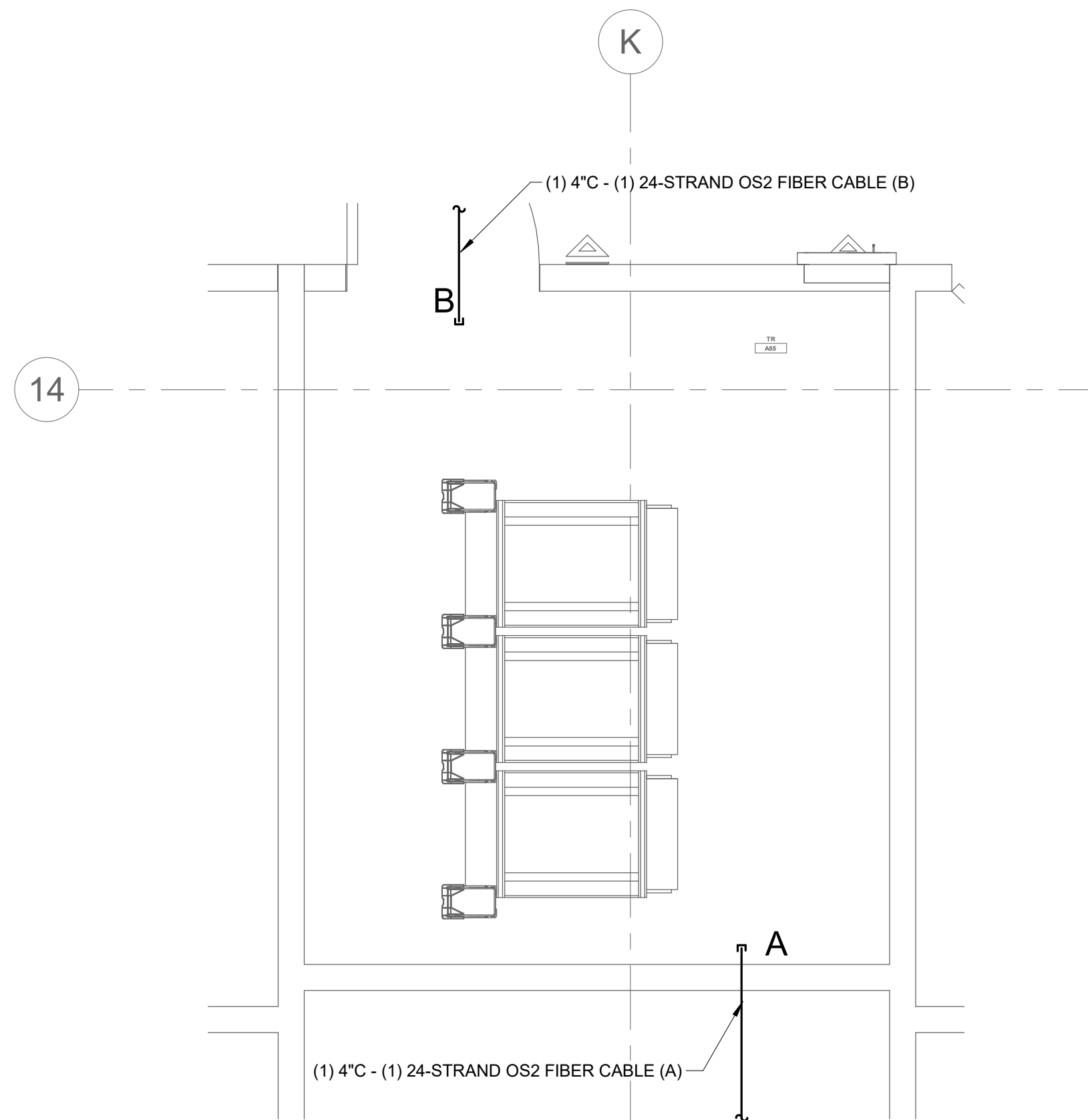
1 TELECOM ROOM ENLARGEMENT PLAN TR #A85 1/2" = 1'-0" NOTES: 1. REFER TO ELECTRICAL DRAWINGS FOR ROOM LAYOUT AND RACK ELEVATIONS. 2. ROUTE OPTICAL FIBER CABLE TO OVERHEAD CABLE TRAY AND TERMINATE IN FIBER DISTRIBUTION CABINET. KEYNOTES: ( # ) 1. THROUGH WALL PENETRATION FOR BACKBONE CONDUIT. OPTICAL FIBER CABLE CONTINUES ON CABLE TRAY TO RACKS.
