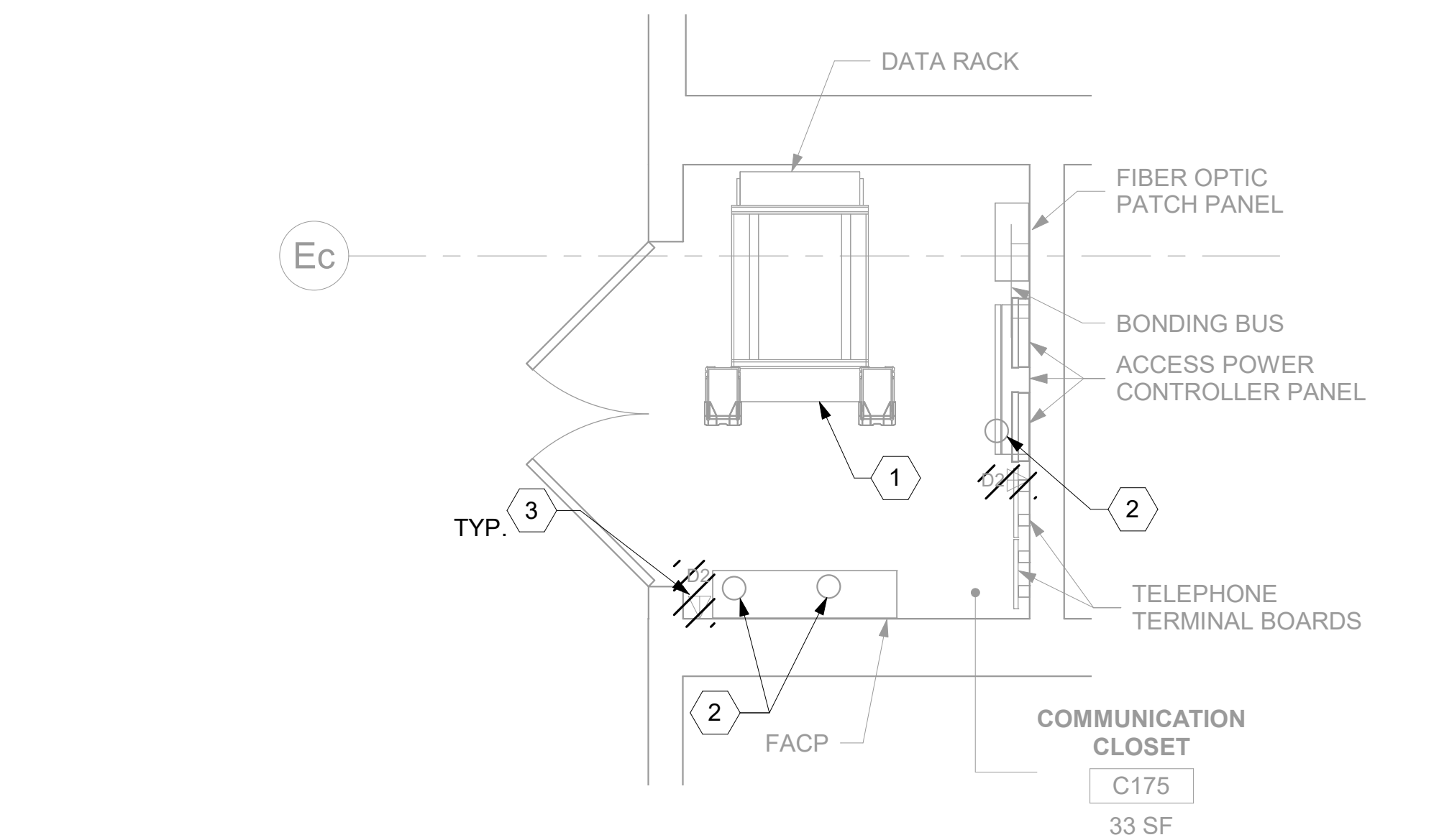
1 RM C175 - DEMOLITION FLOOR PLAN 148TN101A 1/2" = 1'-0"
