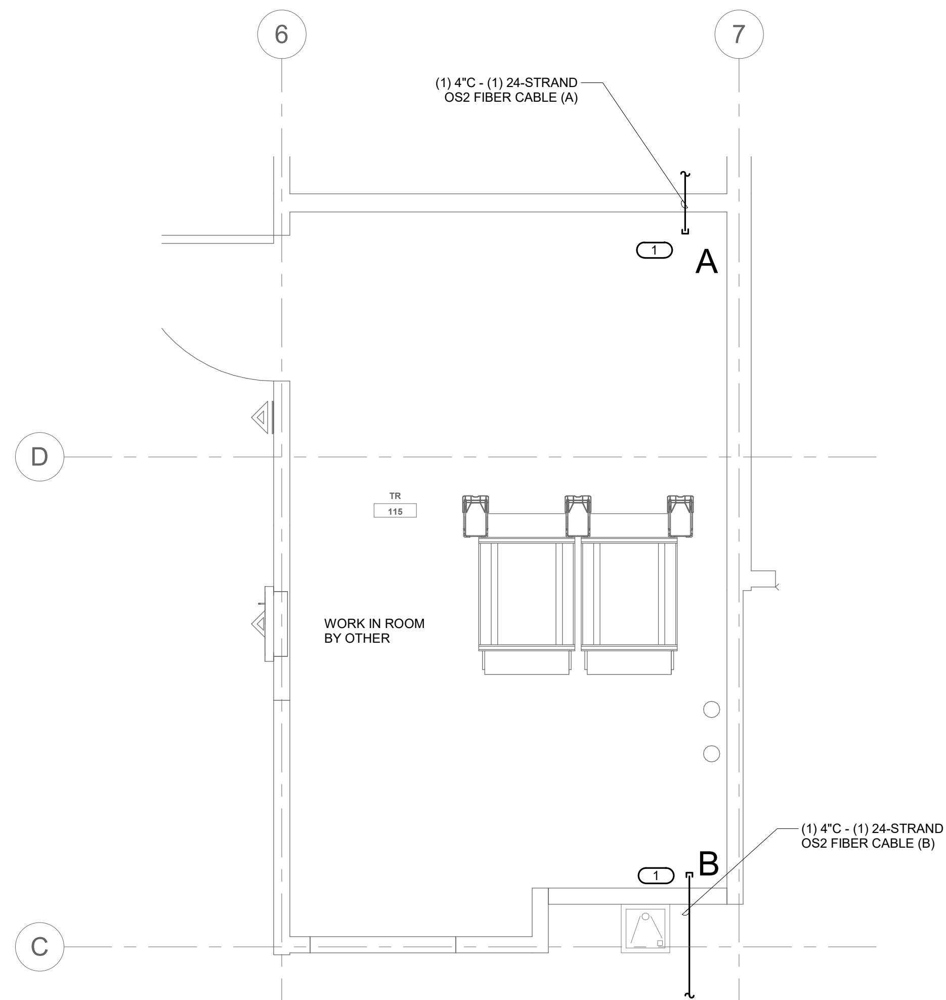
1 TELECOM ROOM ENLARGEMENT TR #115 1/2" = 1'-0" NOTES: 1. REFER TO ELECTRICAL DRAWINGS FOR ROOM LAYOUT AND RACK ELEVATIONS. 2. ROUTE OPTICAL FIBER CABLE TO OVERHEAD CABLE TRAY AND TERMINATE IN FIBER DISTRIBUTION CABINET. KEYNOTES: # 1. THROUGH WALL PENETRATION FOR BACKBONE CONDUIT. OPTICAL FIBER CABLE CONTINUES ON CABLE TRAY TO RACKS.
