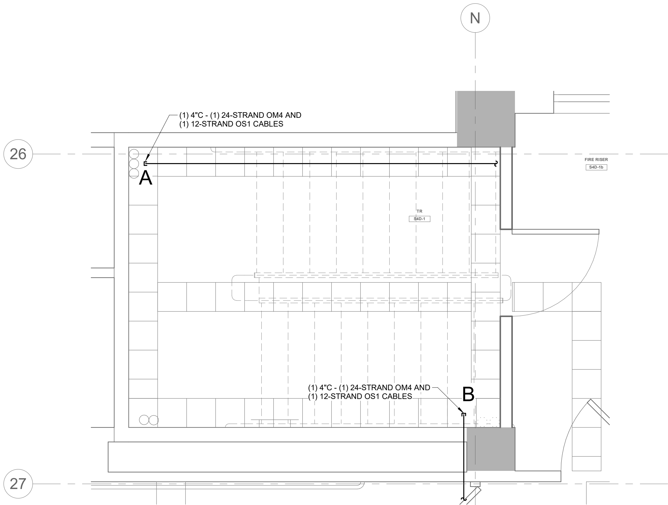
NORTH 2 1/2" = 1'-0" TELECOM ROOM PATHWAY TR #S4D-1
