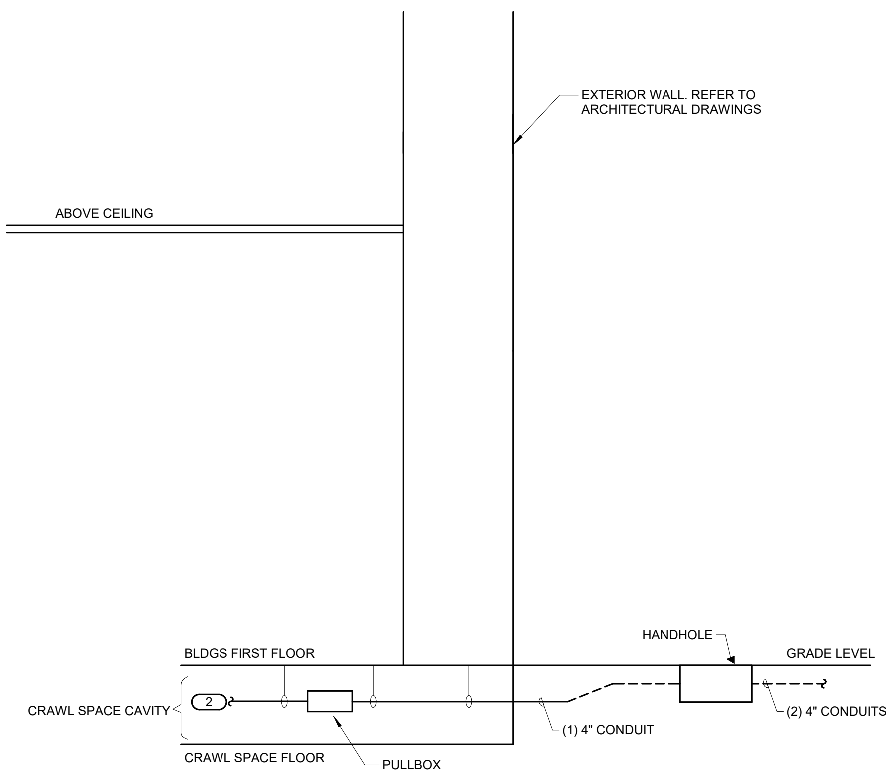
3 EXTERIOR PATHWAY DETAIL (CRAWL SPACE) NO SCALE KEYNOTES: 1. ROUTE CONDUITS THROUGH CRAWL SPACES SUSPENDED ABOVE FLOOR AND SUPPORTED BY BEAM CLAMPS, PIPE COLLARS AND SPACERS. 2. ROUTE CONDUIT THROUGH CRAWL SPACE TO CONDUIT STUB UP LOCATION. REFER TO INTERIOR FLOOR PLANS FOR STUB UP LOCATIONS.
