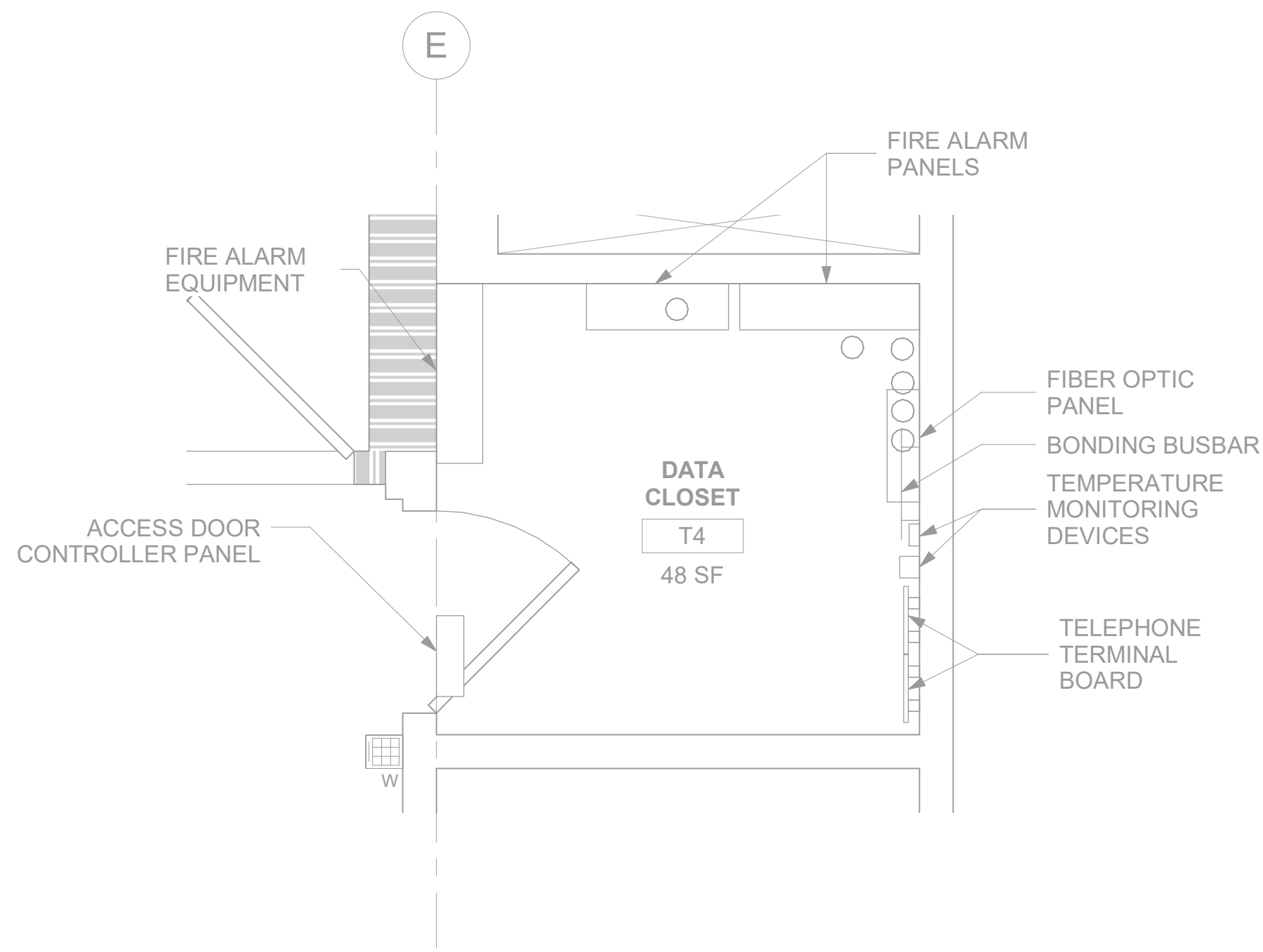
2 RM T4 - TELECOMMUNICATIONS PLAN 146TN101A 1/2" = 1'-0"
