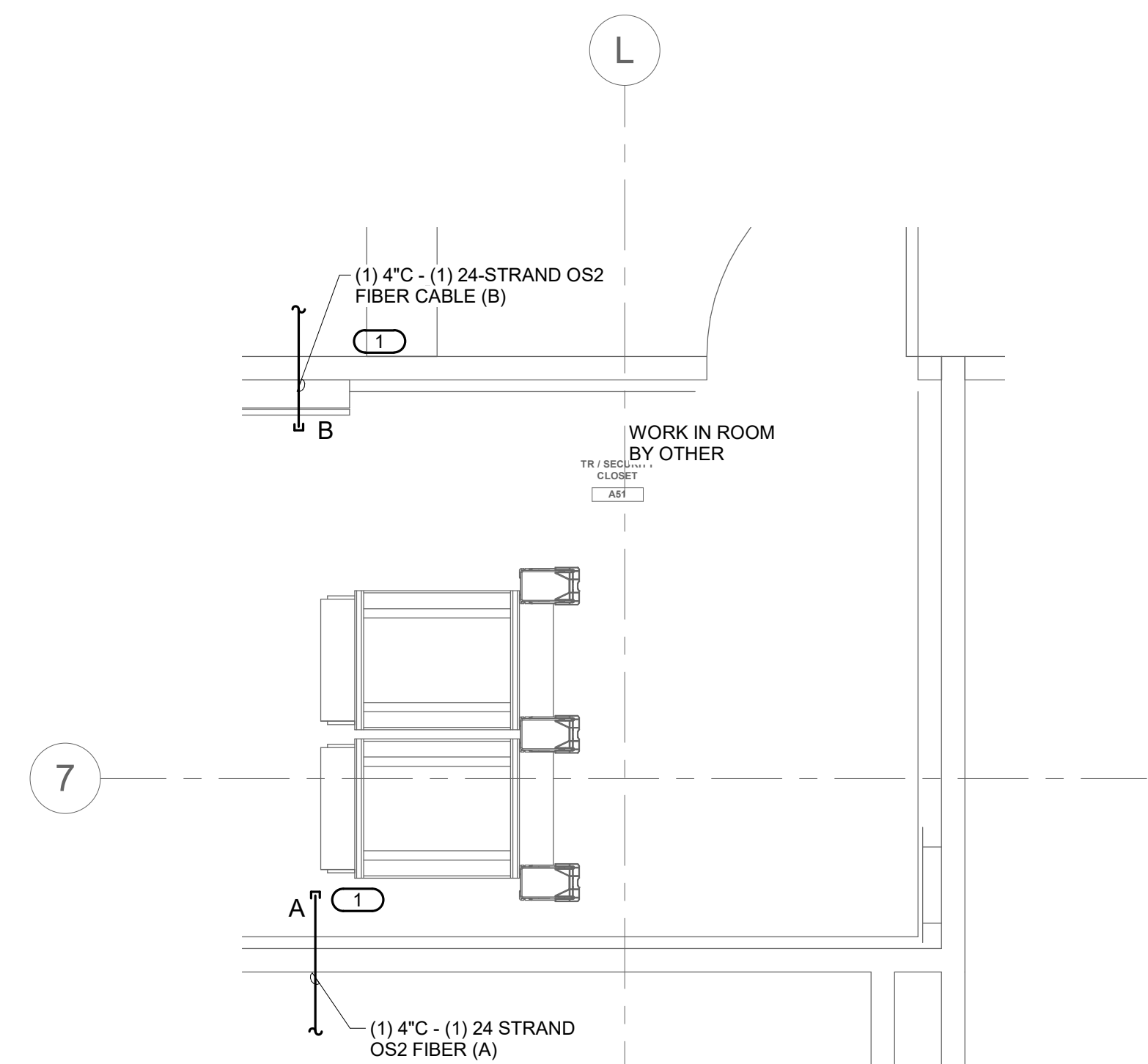
1 TELECOM ROOM ENLARGEMENT TR #A51 1/2" = 1'-0"
