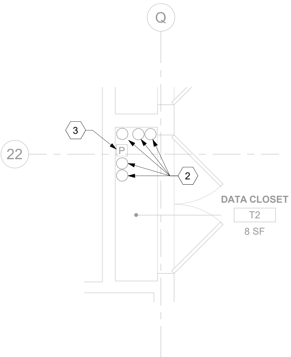
3 RM T2 - DEMOLITION OVERHEAD PLAN 146TN101A 1/2" = 1'-0"
