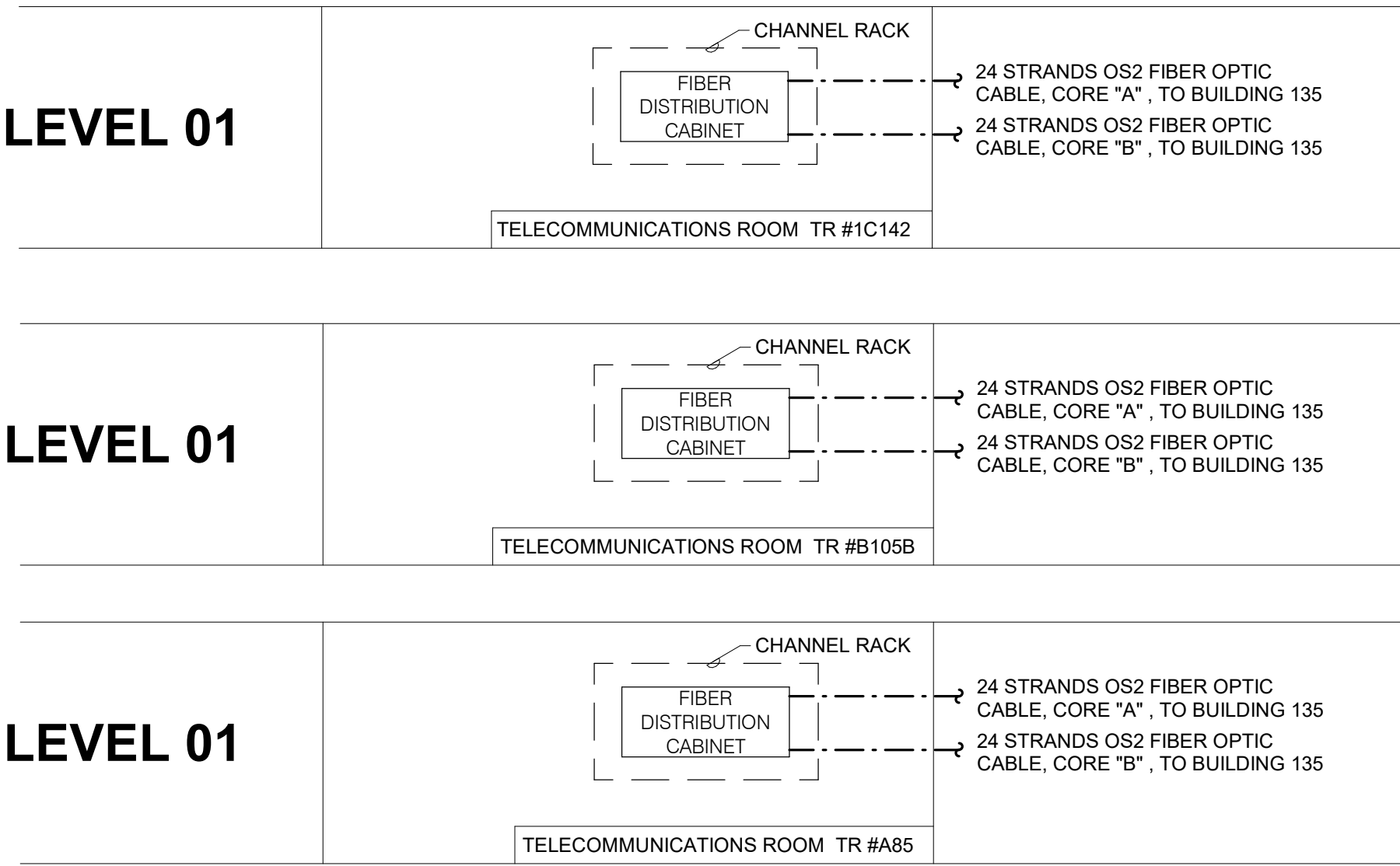
3 FIBER RISER DIAGRAM NO SCALE NOTES: 1. THIS RISER IS DIAGMATIC AND MAY NOT SHOW ACTUAL ROUTING OR QUANTITIES OF MATERIALS SHOWN. THIS RISER IS SHOWN FOR CLARIFICATION OF CONNECTIONS, LOCATIONS AND CABLE TYPE. ALL INFORMATION OUTLETS ARE TYPICAL OF THE OUTLETS IN THE AREA SHOWN. REFER TO FLOOR PLANS FOR MORE SPECIFIC ROUTING INFORMATION. REFER TO REQUIREMENTS. 2. REFER TO ELECTRICAL DRAWINGS FOR CHANNEL RACK AND FIBER OPTIC DISTRIBUTION CABINET SPECIFICATIONS
