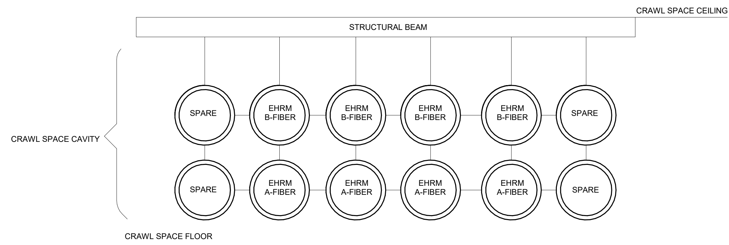
4 EXTERIOR PATHWAY DETAIL (BLDG 146 CRAWL SPACE SECTION) NO SCALE NOTES: 1. ROUTE CONDUITS THROUGH CRAWL SPACES SUSPENDED ABOVE FLOOR AND SUPPORTED BY BEAM CLAMPS, PIPE COLLARS AND SPACERS. 2. IN BLDG 146 CRAWL SPACE, ROUTE CONDUIT IN A (2) x (6) CONDUIT STACK. ADJUST CONDUIT ARRANGEMENT TO (1) x (12) OR (3) x (4) CONDUIT STACK AS REQUIRED TO ROUTE THROUGH CRAWL SPACE.
