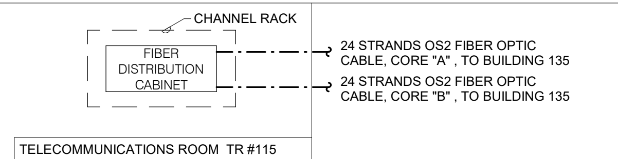
3 FIBER RISER DIAGRAM NO SCALE NOTES: 1. THIS RISER IS DIAGRAMMATIC AND MAY NOT SHOW ACTUAL ROUTING OR QUANTITIES OF MATERIALS SHOWN. THIS RISER IS SHOWN FOR CLARIFICATION OF CONNECTION(S), LOCATIONS AND CABLE TYPE. ALL INFORMATION OUTLETS ARE TYPICAL OF THE OUTLETS IN THE AREA SHOWN. REFER TO FLOOR PLANS FOR MORE SPECIFIC ROUTING INFORMATION. REFER TO SPECIFICATIONS FOR ADDITIONAL REQUIREMENTS. 2. REFER TO ELECTRICAL DRAWINGS FOR CHANNEL RACK AND FIBER OPTIC DISTRIBUTION CABINET SPECIFICATIONS
