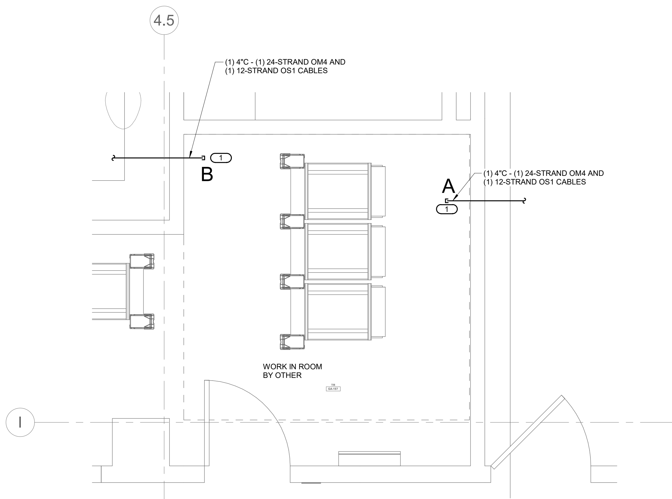
1 TELECOM ROOM ENLARGEMENT TR #GA-157 1/2" = 1'-0"
