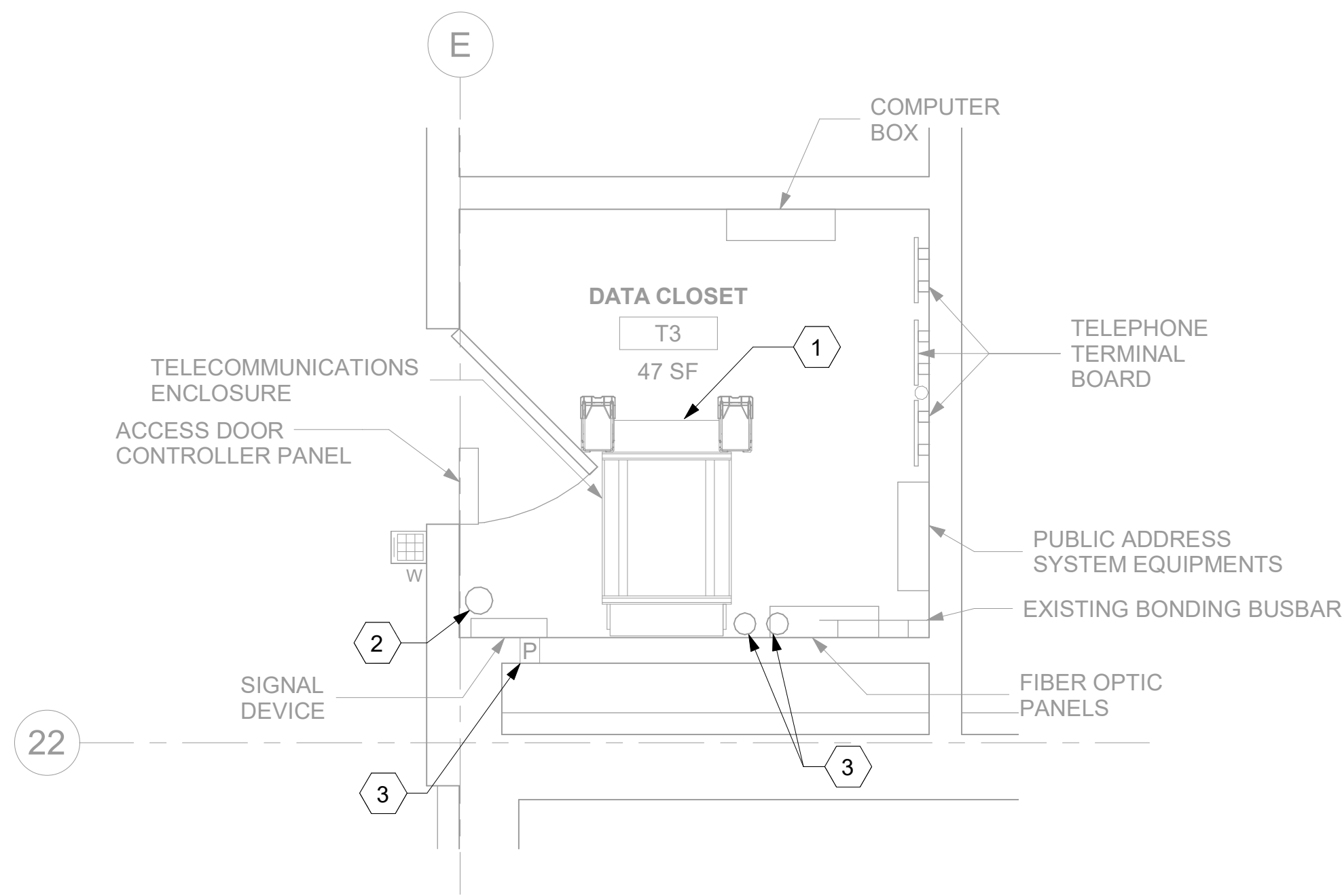
1 RM T3 - DEMOLITION FLOOR PLAN 146TN101A 1/2" = 1'-0"
