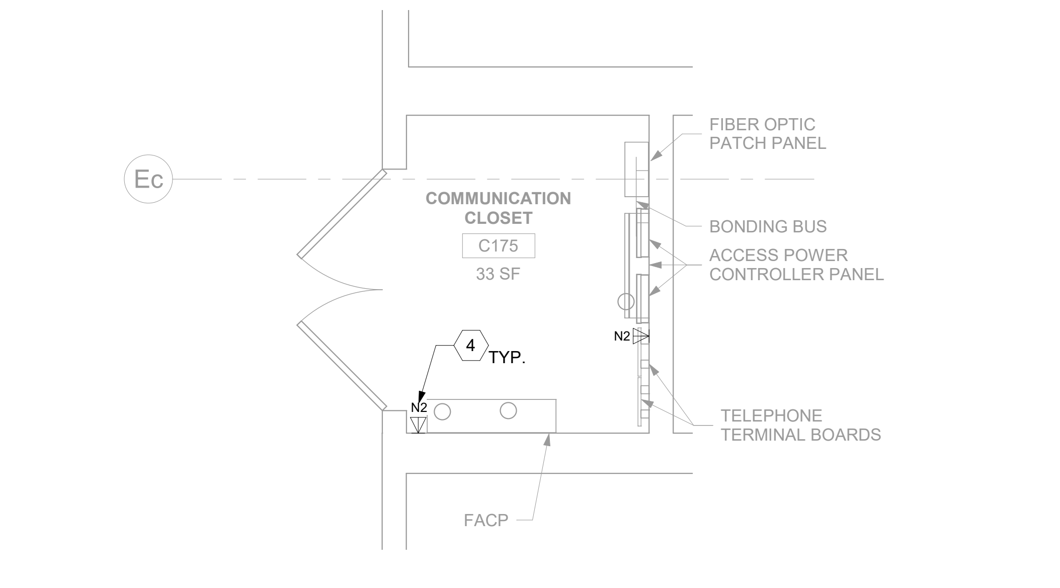
2 RM C175 - TELECOMMUNICATIONS PLAN 148TN101A 1/2" = 1'-0"
