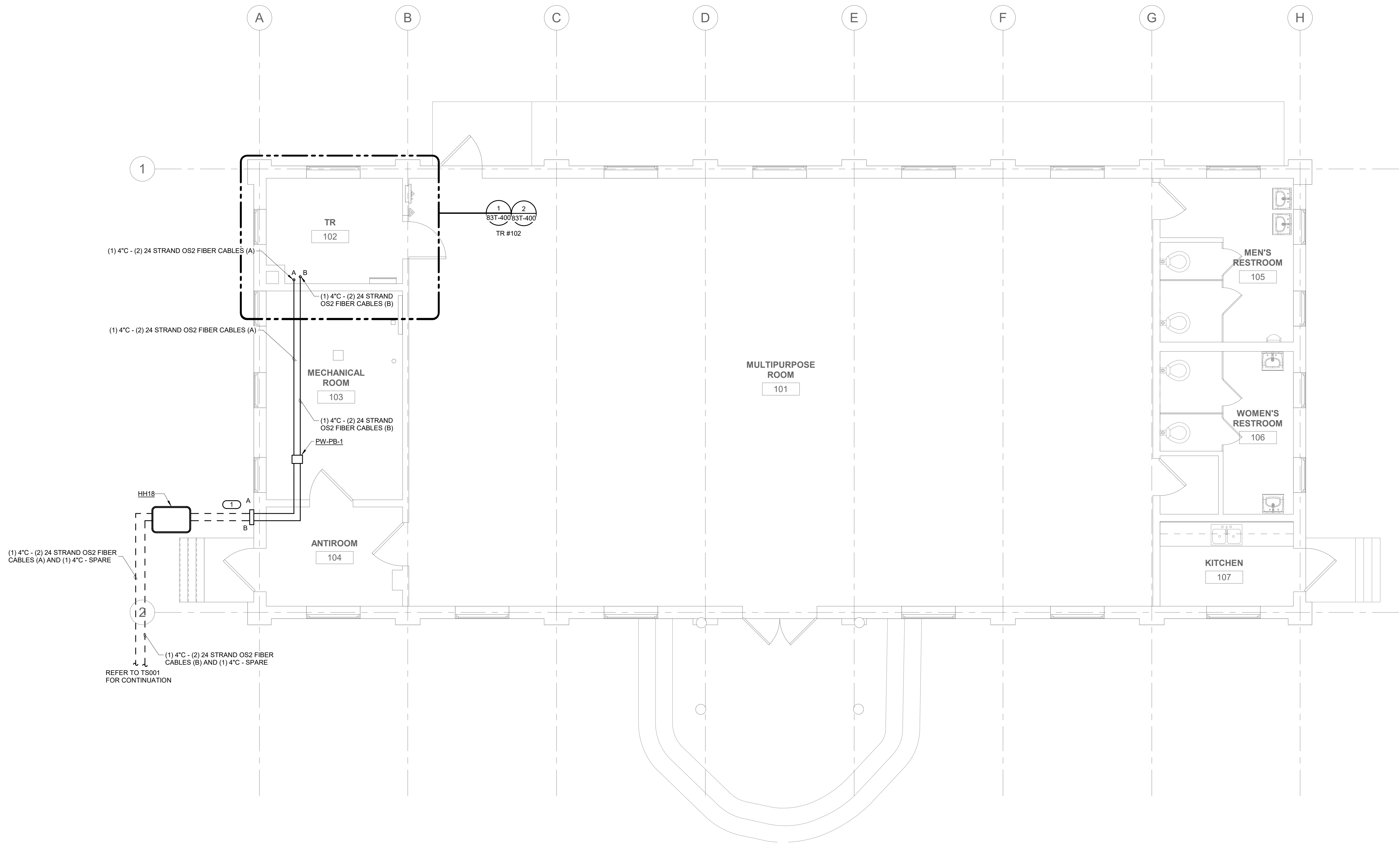
1 LEVEL 01 PLAN - TECHNOLOGY 1/4" = 1'-0"
