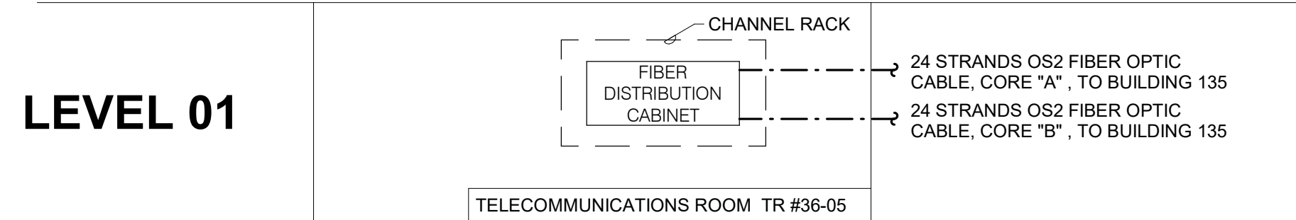
3 FIBER RISER DIAGRAM NO SCALE NOTES: 1. THIS RISER IS DIAGRAMMATIC AND MAY NOT SHOW ACTUAL ROUTING OR QUANTITIES OF MATERIALS SHOWN. THIS RISER IS SHOWN FOR CLARIFICATION OF CONNECTION(S), LOCATIONS AND CABLE TYPE. ALL INFORMATION OUTLETS ARE TYPICAL OF THE OUTLETS IN THE AREA SHOWN. REFER TO FLOOR PLANS FOR MORE SPECIFIC ROUTING INFORMATION. REFER TO SPECIFICATIONS FOR ADDITIONAL REQUIREMENTS. 2. REFER TO ELECTRICAL DRAWINGS FOR CHANNEL RACK AND FIBER OPTIC DISTRIBUTION CABINET SPECIFICATIONS
