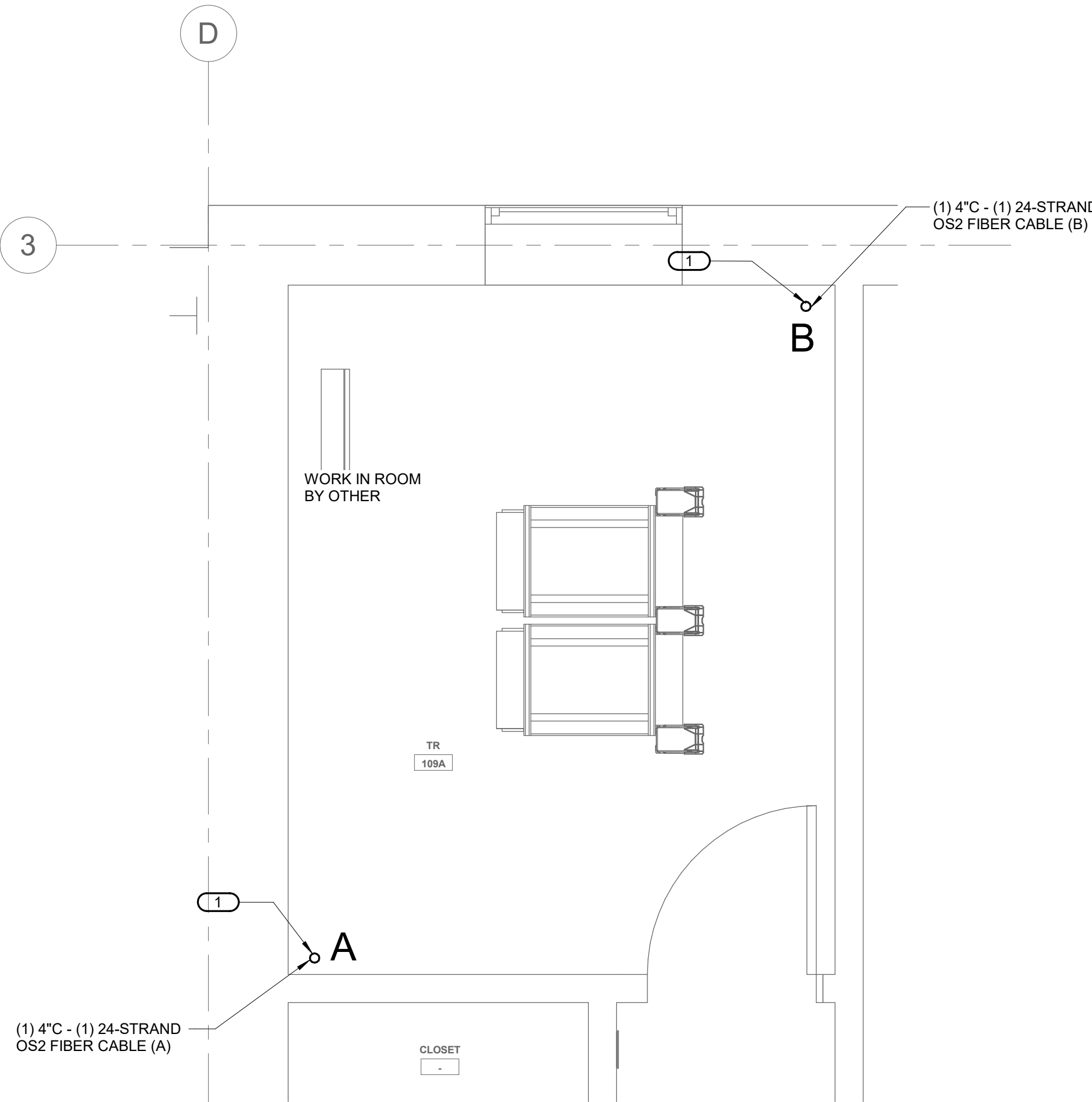
1 TELECOM ROOM ENLARGEMENT TR #109A 1/2" = 1'-0"
