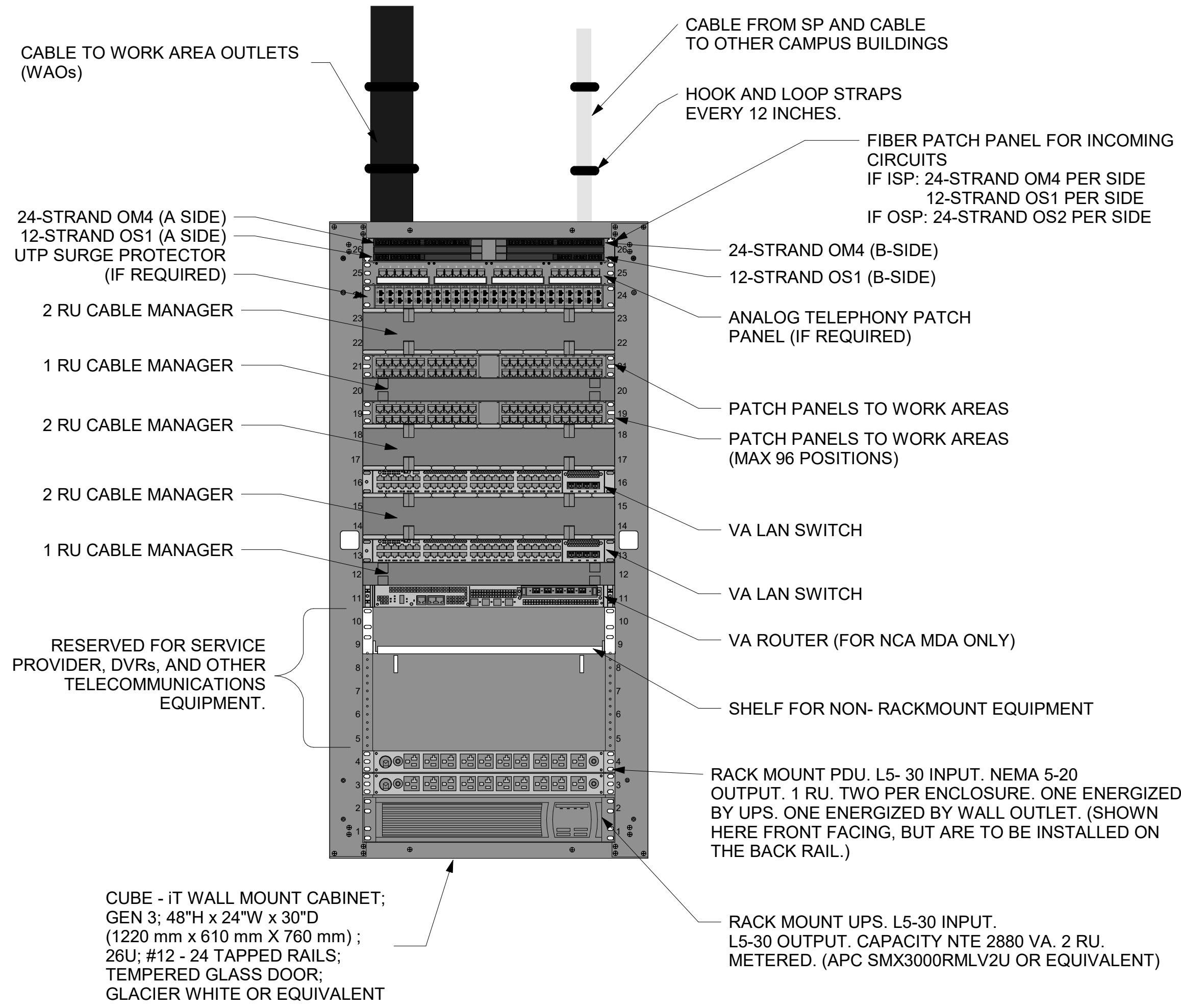
2 TELECOMMUNICATIONS ENCLOSURE ELEVATION DETAIL NTS
