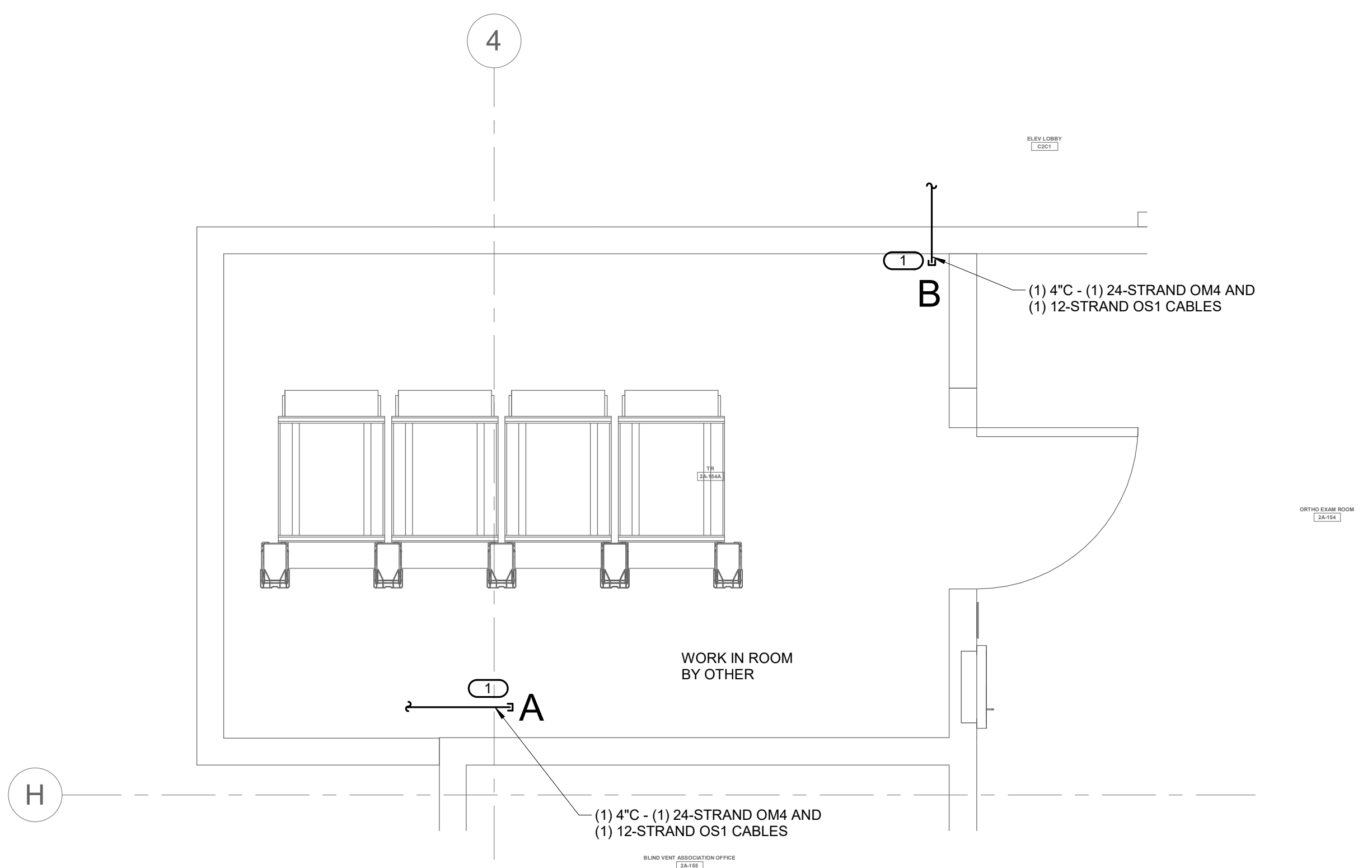
4 TELECOM ROOM ENLARGEMENT TR #2A-154A 1/2" = 1'-0"
