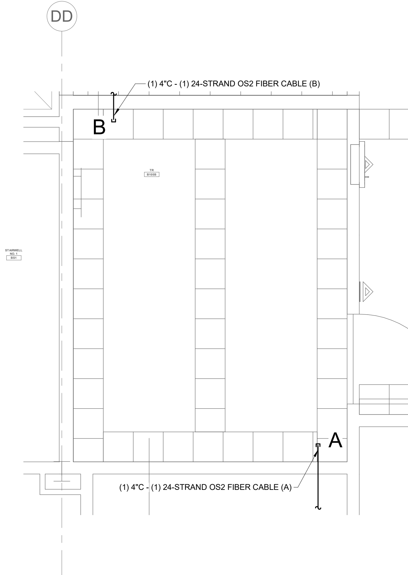
4 TELECOM ROOM PATHWAY PLAN - TR #B105B 1/2" = 1'-0"
