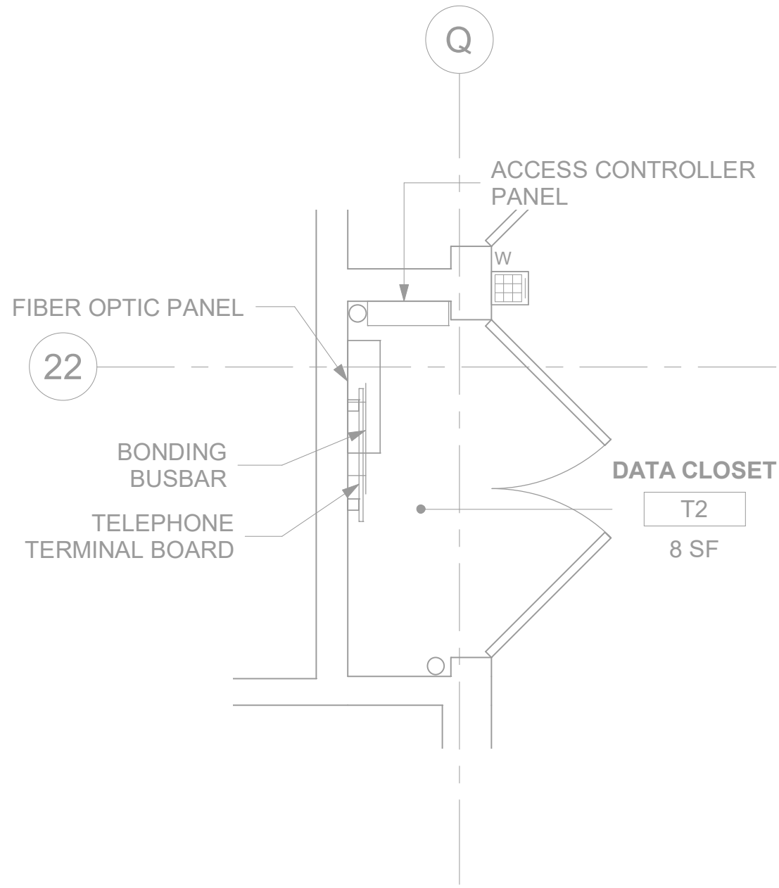
2 RM T2 - TELECOMMUNICATIONS PLAN 146TN101A 1/2" = 1'-0"
