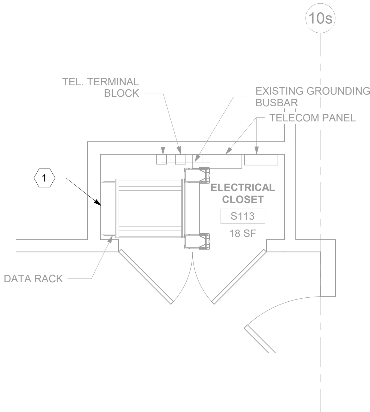
1 RM S113 - DEMOLITION FLOOR PLAN 148TN101A 1/2" = 1'-0"
