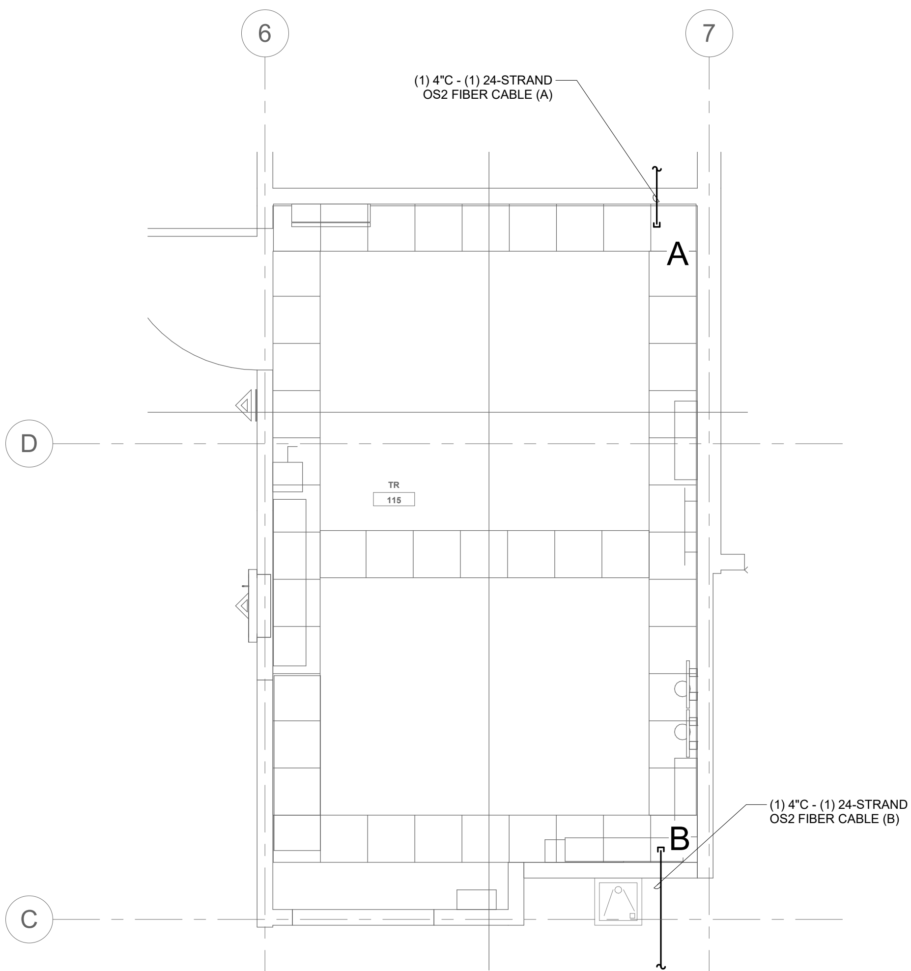
2 TELECOM ROOM PATHWAY TR #115 1/2" = 1'-0"
