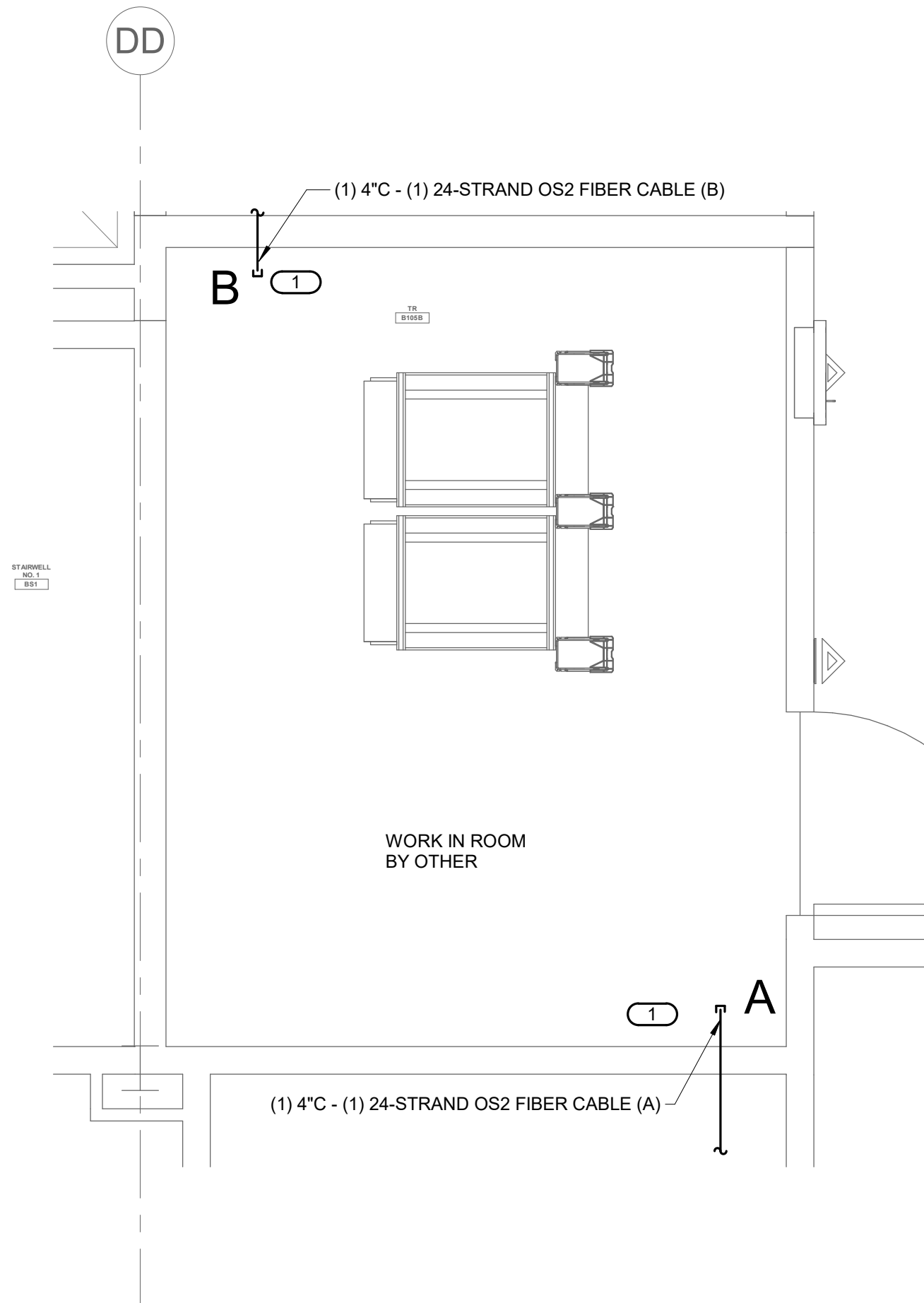
3 TELECOM ROOM ENLARGEMENT PLAN - TR #B105B 1/2" = 1'-0" NOTES: 1. REFER TO ELECTRICAL DRAWINGS FOR ROOM LAYOUT AND RACK ELEVATIONS. 2. ROUTE OPTICAL FIBER CABLE TO OVERHEAD CABLE TRAY AND TERMINATE IN FIBER DISTRIBUTION CABINET. KEYNOTES: ( # ) 1. THROUGH WALL PENETRATION FOR BACKBONE CONDUIT. OPTICAL FIBER CABLE CONTINUES ON CABLE TRAY TO RACKS.
