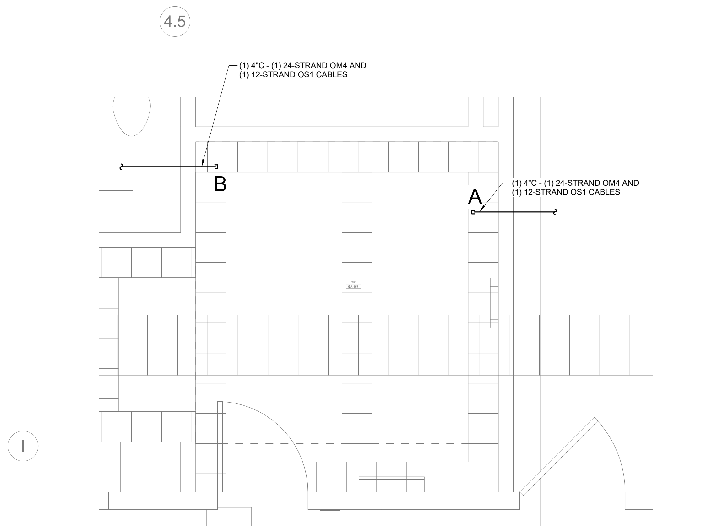
2 TELECOM ROOM PATHWAY TR #GA-157 1/2" = 1'-0"
