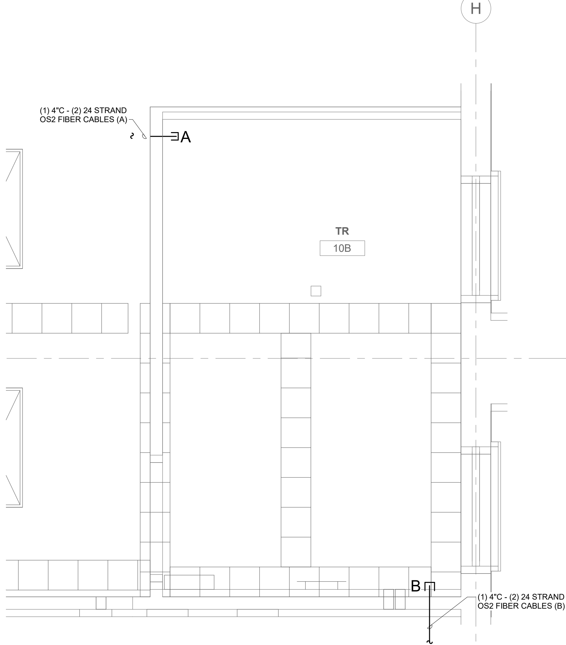
NORTH 2 1/2" = 1'-0" TELECOM ROOM PATHWAY TR #10B
