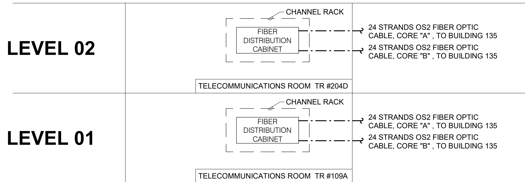
5 FIBER RISER DIAGRAM NO SCALE
