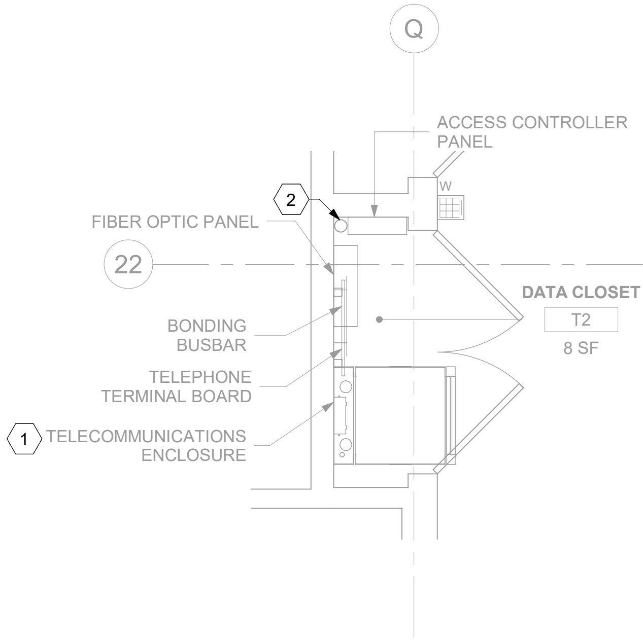
1 RM T2 - DEMOLITION FLOOR PLAN 146TN101A 1/2" = 1'-0"
