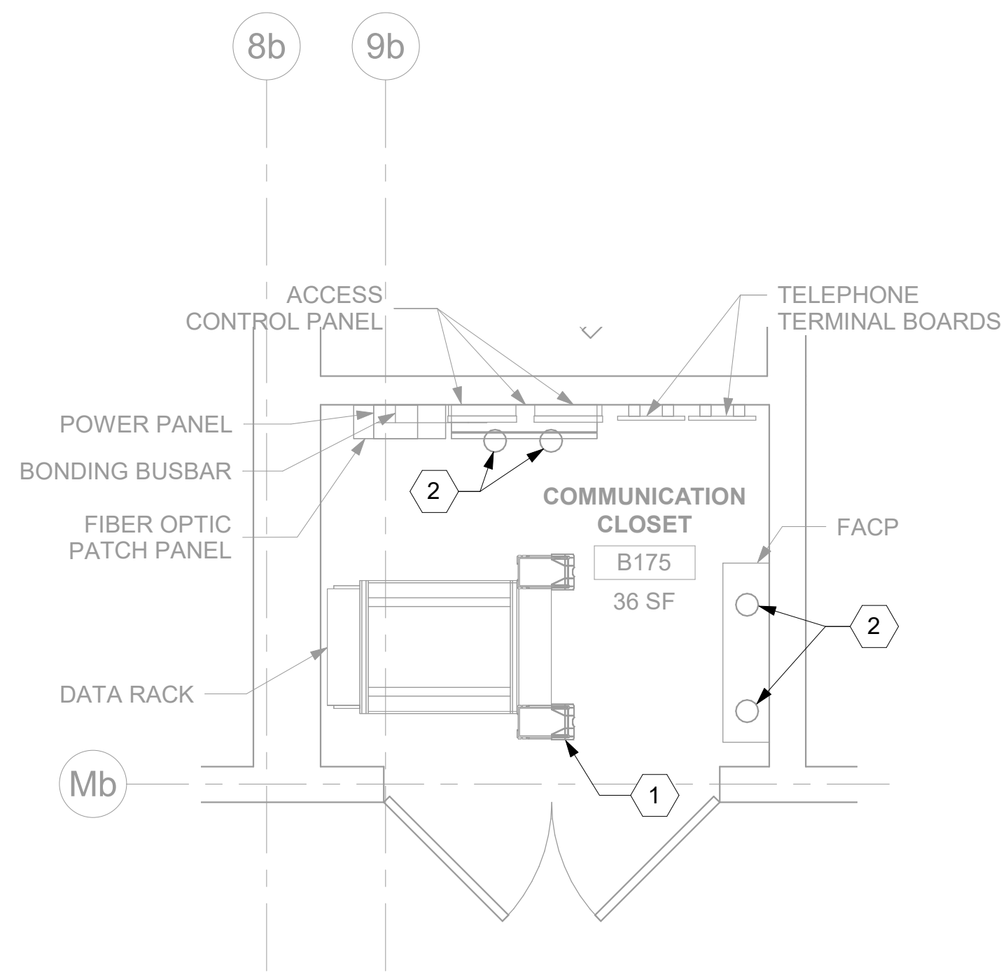
1 RM B175 - DEMOLITION FLOOR PLAN 148TN101B 1/2" = 1'-0"
