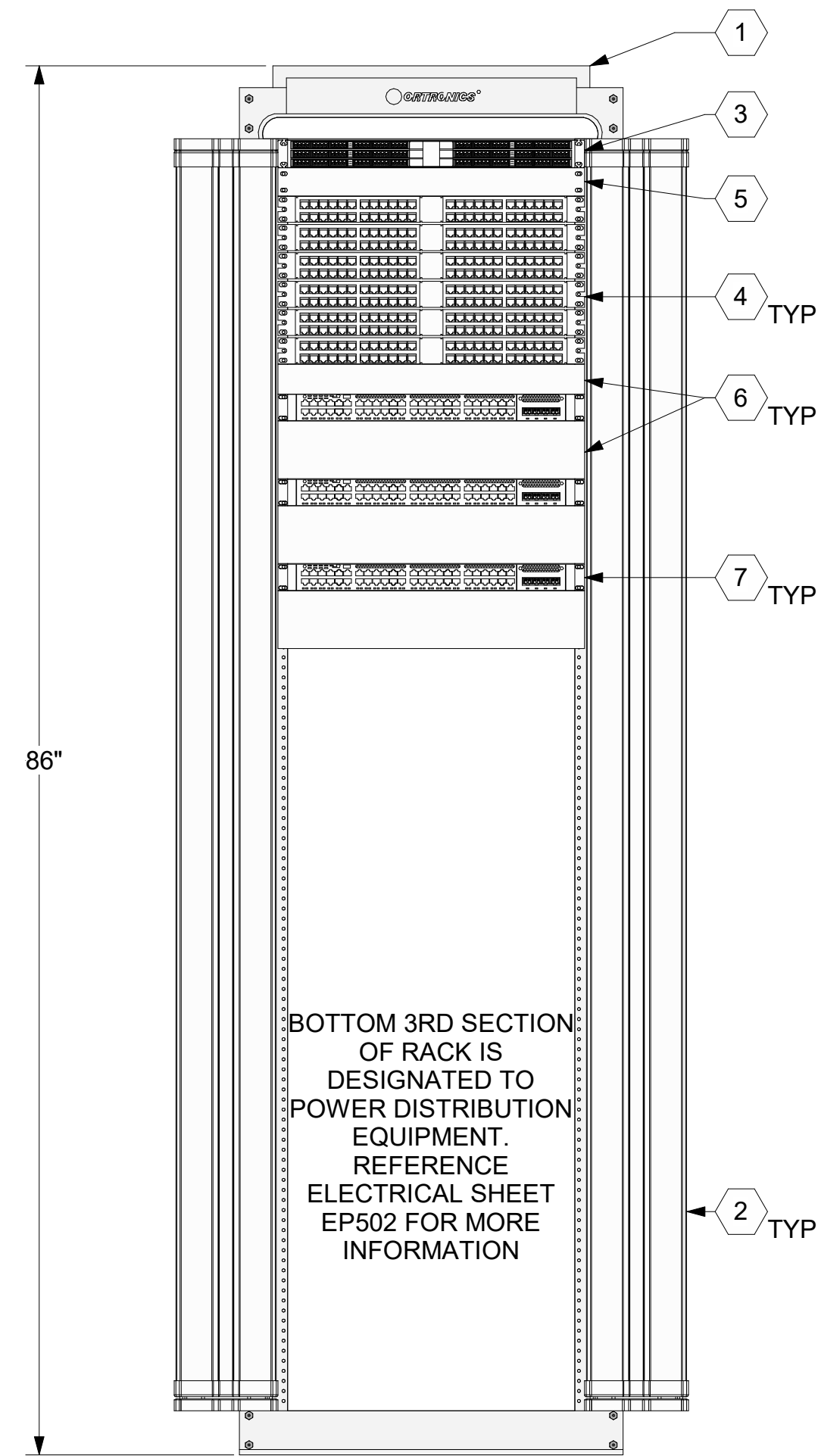
4 TR DATA RACK ELEVATION - SINGLE RACK 1" = 0'-9"
