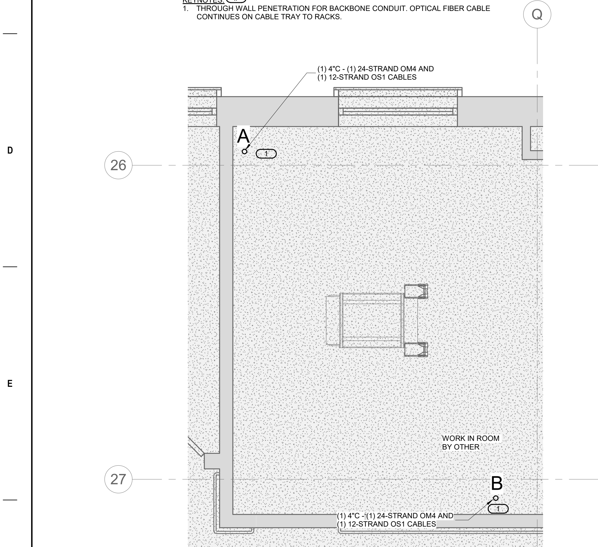
NORTH 3 1/2" = 1'-0" TELECOM ROOM ENLARGEMENT TR #C506 NOTES: 1. REFER TO ELECTRICAL DRAWINGS FOR ROOM LAYOUT AND RACK ELEVATIONS. 2. ROUTE OPTICAL FIBER CABLE TO OVERHEAD CABLE TRAY AND TERMINATE IN FIBER DISTRIBUTION CABINET. KEYNOTES: # 1. THROUGH WALL PENETRATION FOR BACKBONE CONDUIT. OPTICAL FIBER CABLE CONTINUES ON CABLE TRAY TO RACKS.
