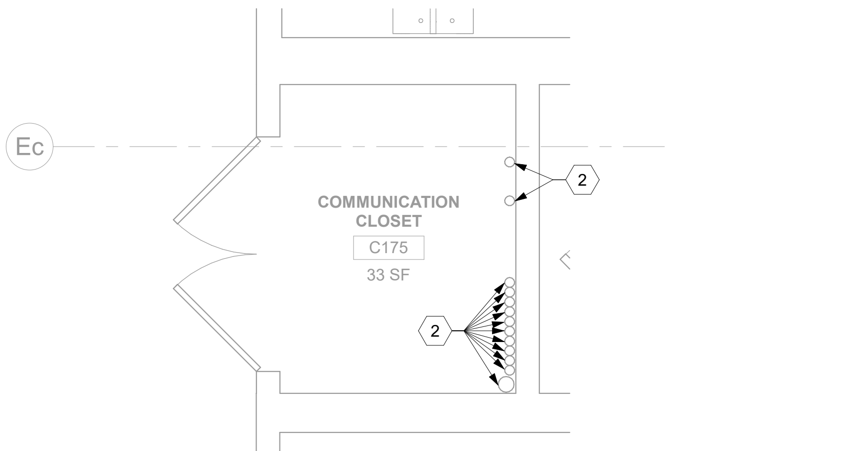
3 RM C175 - DEMOLITION OVERHEAD PLAN 148TN101A 1/2" = 1'-0"
