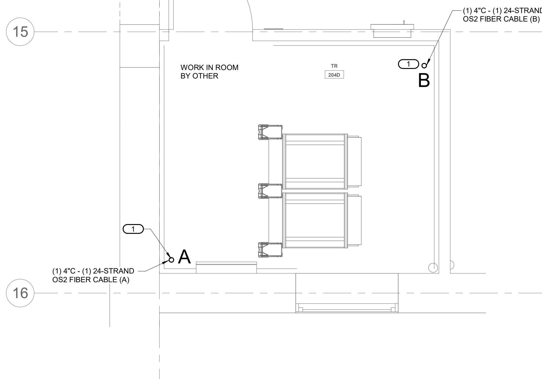
3 TELECOM ROOM ENLARGEMENT TR #204D 1/2" = 1'-0"
