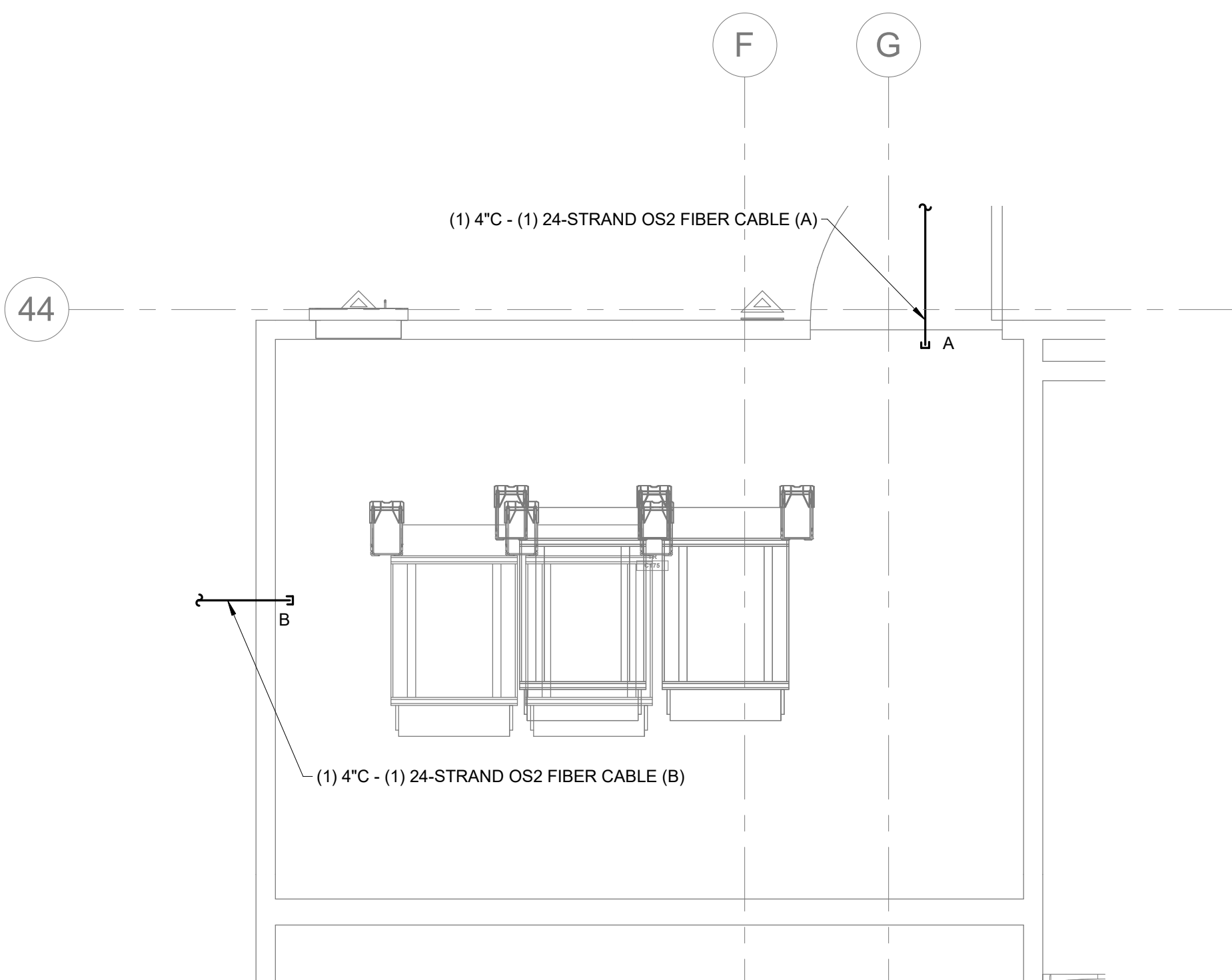
4 TELECOM ROOM ENLARGEMENT PLAN TR #C175 1/2" = 1'-0" NOTES: 1. REFER TO ELECTRICAL DRAWINGS FOR ROOM LAYOUT AND RACK ELEVATIONS. 2. ROUTE OPTICAL FIBER CABLE TO OVERHEAD CABLE TRAY AND TERMINATE IN FIBER DISTRIBUTION CABINET. KEYNOTES: C # 1. THROUGH WALL PENETRATION FOR BACKBONE CONDUIT. OPTICAL FIBER CABLE CONTINUES ON CABLE TRAY TO RACKS.
