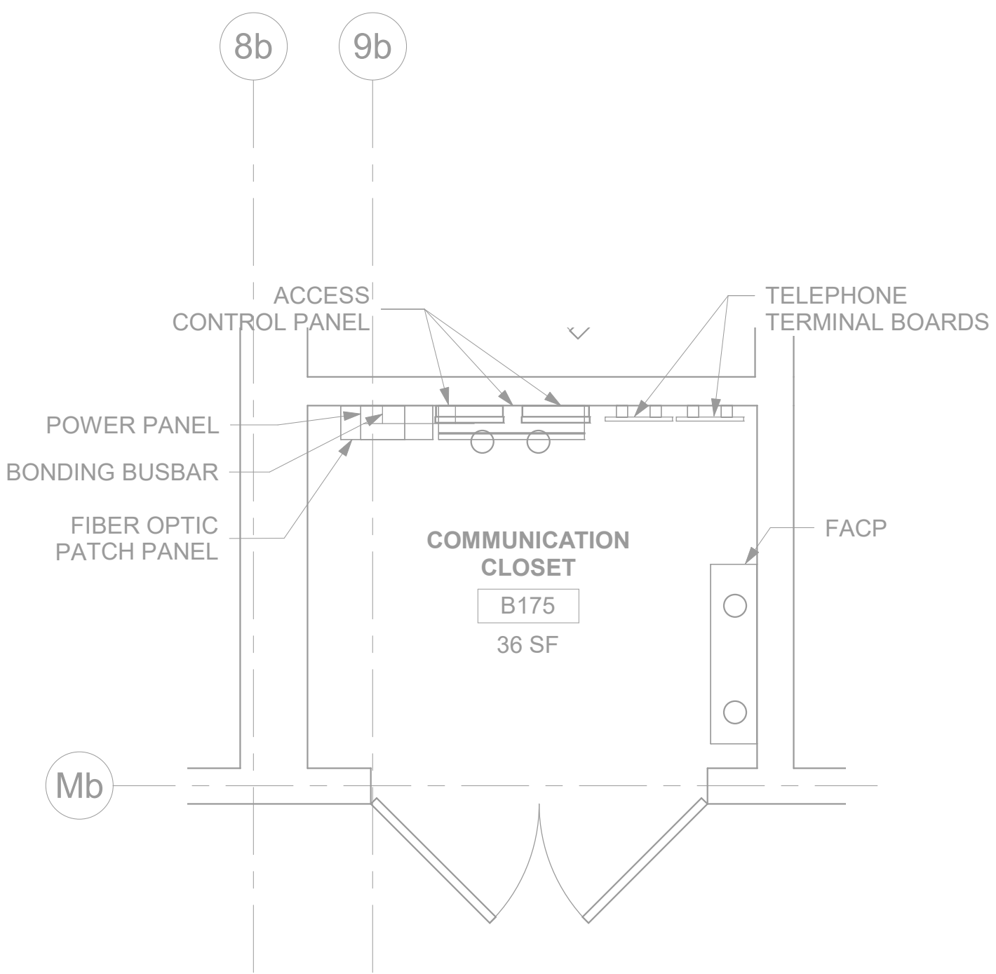
2 RM B175 - TELECOMMUNICATIONS PLAN 148TN101B 1/2" = 1'-0"
