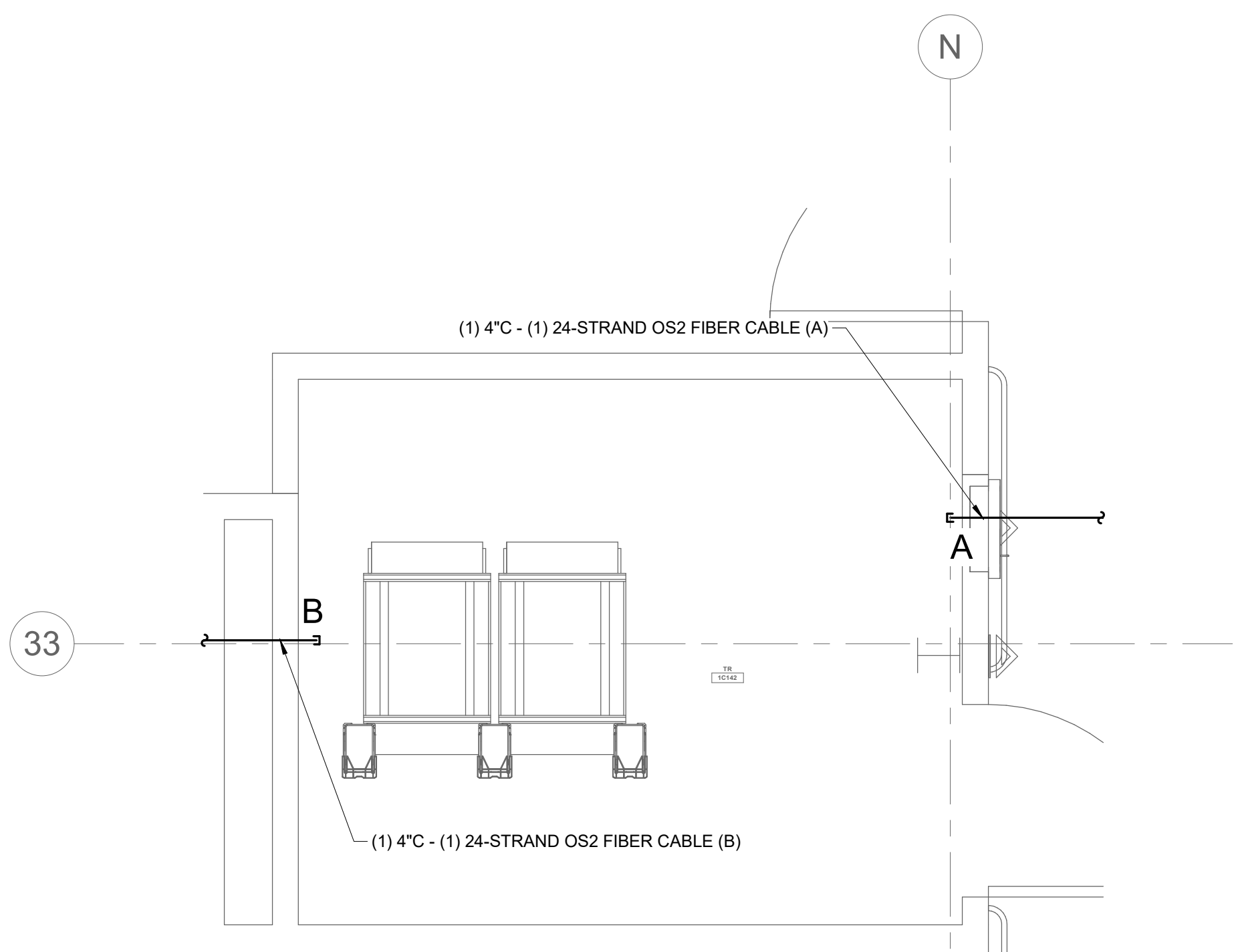
1 TELECOM ROOM ENLARGEMENT PLAN TR #1C142 1/2" = 1'-0" NOTES: 1. REFER TO ELECTRICAL DRAWINGS FOR ROOM LAYOUT AND RACK ELEVATIONS. 2. ROUTE OPTICAL FIBER CABLE TO OVERHEAD CABLE TRAY AND TERMINATE IN FIBER DISTRIBUTION CABINET. KEYNOTES: C # 1. THROUGH WALL PENETRATION FOR BACKBONE CONDUIT. OPTICAL FIBER CABLE CONTINUES ON CABLE TRAY TO RACKS.
