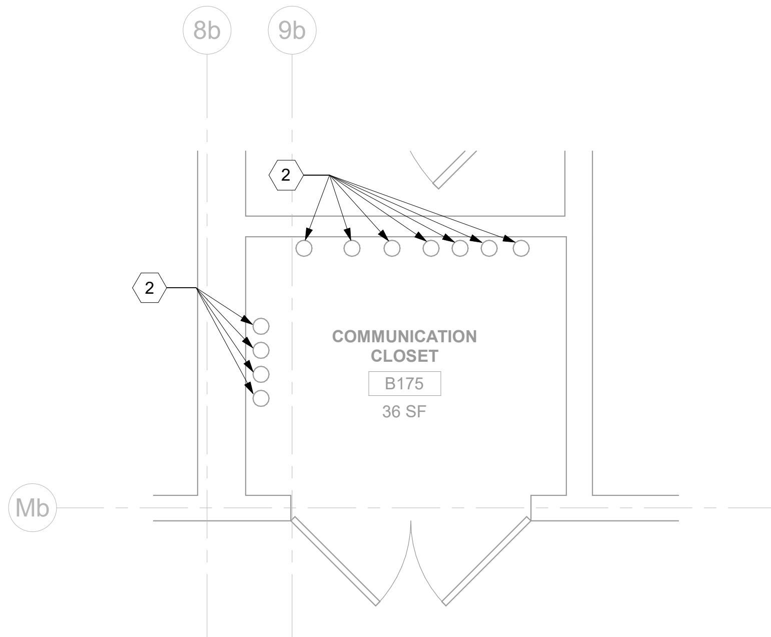
3 RM B175 - DEMOLITION OVERHEAD PLAN 148TN101A 1/2" = 1'-0"
