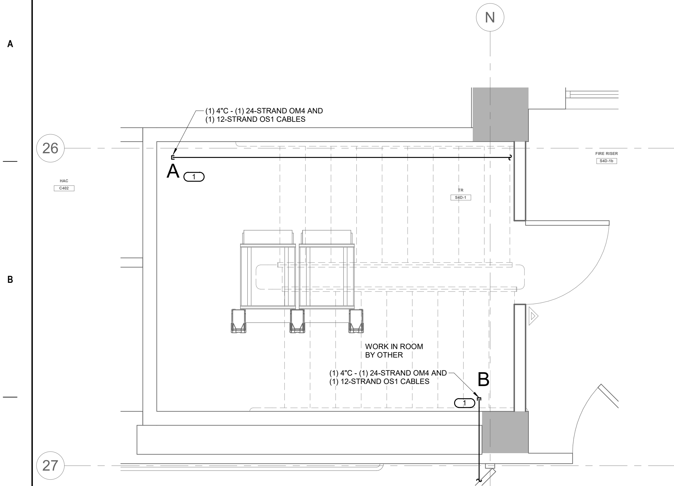
NORTH 1 1/2" = 1'-0" TELECOM ENLARGEMENT TR #S4D-1 NOTES: 1. REFER TO ELECTRICAL DRAWINGS FOR ROOM LAYOUT AND RACK ELEVATIONS. 2. ROUTE OPTICAL FIBER CABLE TO OVERHEAD CABLE TRAY AND TERMINATE IN FIBER DISTRIBUTION CABINET. KEYNOTES: # 1. THROUGH WALL PENETRATION FOR BACKBONE CONDUIT. OPTICAL FIBER CABLE CONTINUES ON CABLE TRAY TO RACKS.
