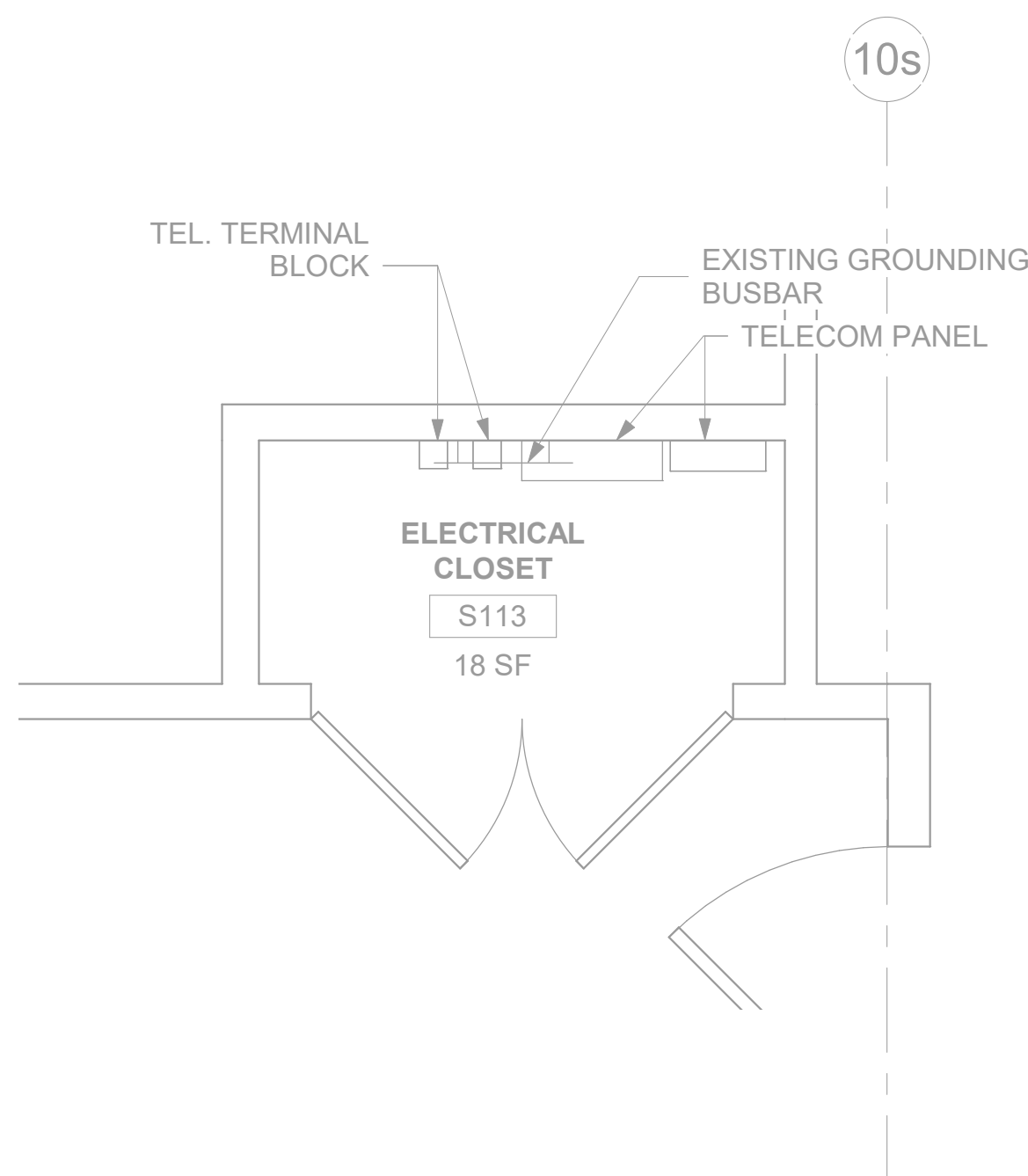
2 RM S113 - TELECOMMUNICATIONS PLAN 148TN101A 1/2" = 1'-0"
