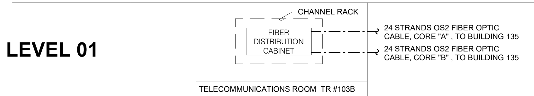
3 FIBER RISER DIAGRAM NO SCALE NOTES: 1. THIS RISER IS DIAGRAMMATIC AND MAY NOT SHOW ACTUAL ROUTING OR QUANTITIES OF MATERIALS SHOWN. THIS RISER IS SHOWN FOR CLARIFICATION OF CONNECTION(S), LOCATIONS AND CABLE TYPE. ALL INFORMATION OUTLETS ARE TYPICAL OF THE OUTLETS IN THE AREA SHOWN. REFER TO FLOOR PLANS FOR MORE SPECIFIC ROUTING INFORMATION. REFER TO SPECIFICATIONS FOR ADDITIONAL REQUIREMENTS. 2. REFER TO ELECTRICAL DRAWINGS FOR CHANNEL RACK AND FIBER OPTIC DISTRIBUTION CABINET SPECIFICATIONS
