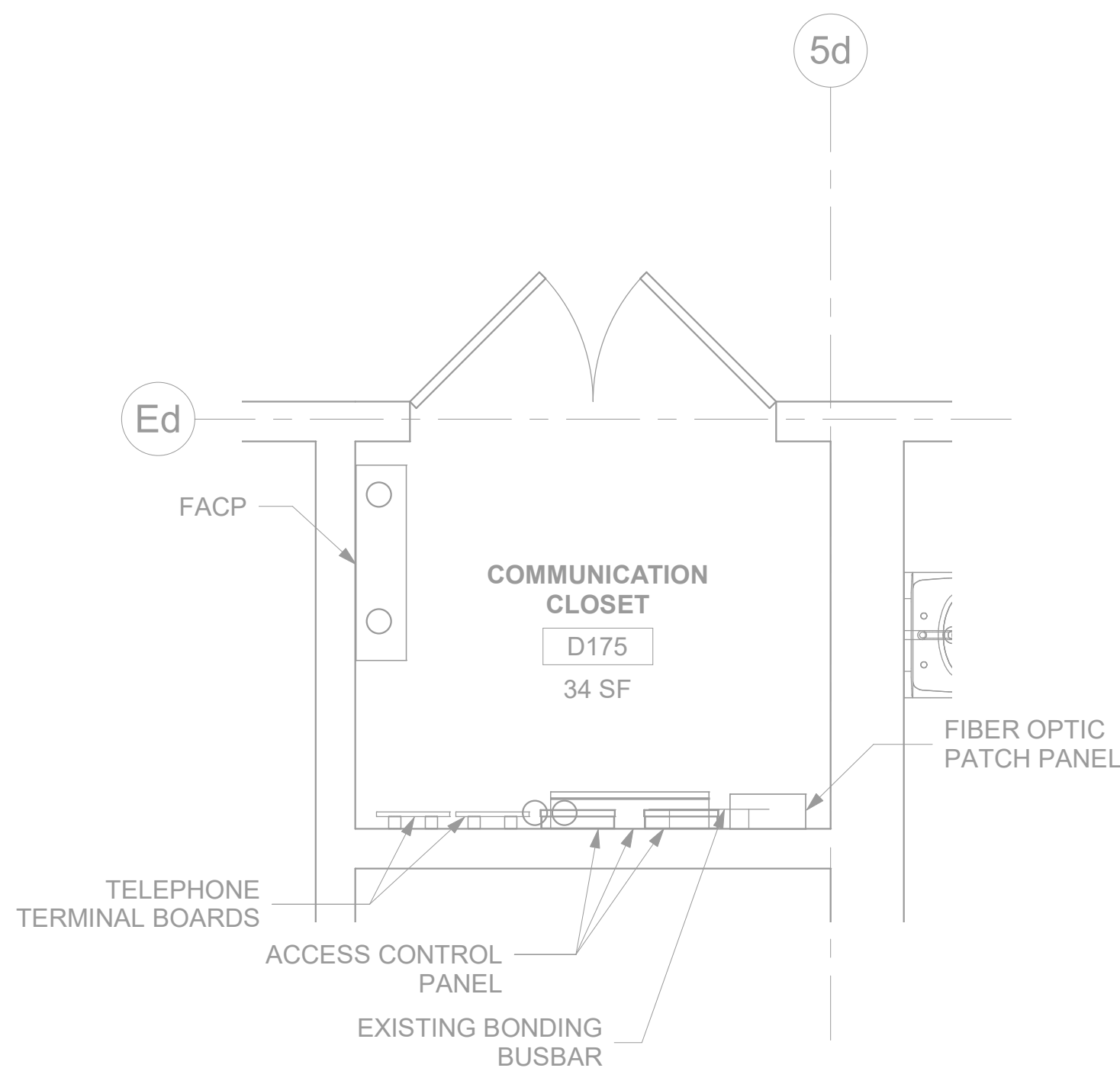
2 RM D175 - TELECOMMUNICATIONS PLAN 148TN101A 1/2" = 1'-0"
