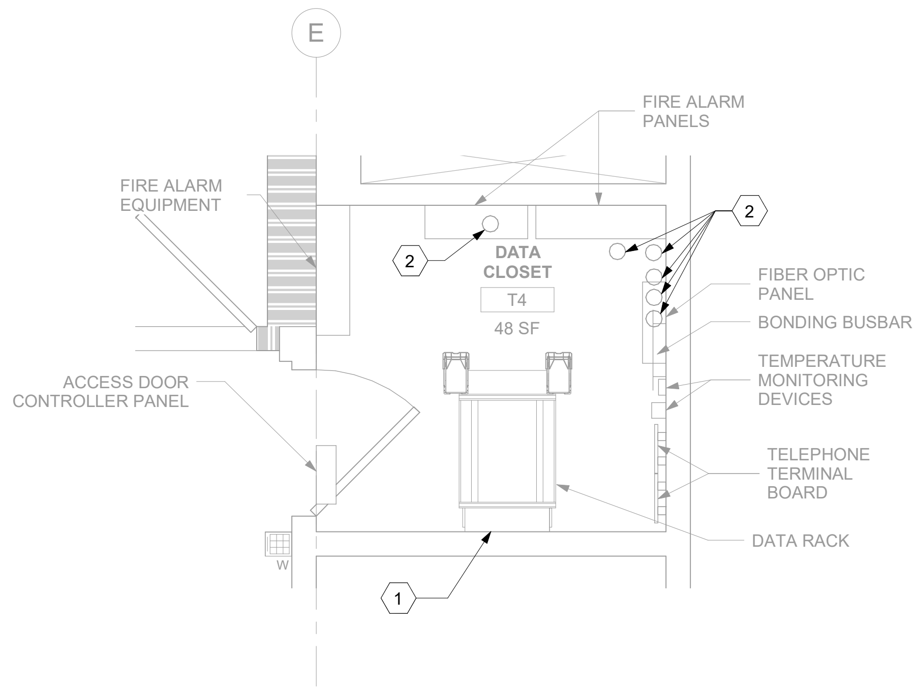
1 RM T4 - DEMOLITION FLOOR PLAN 146TN101A 1/2" = 1'-0"
