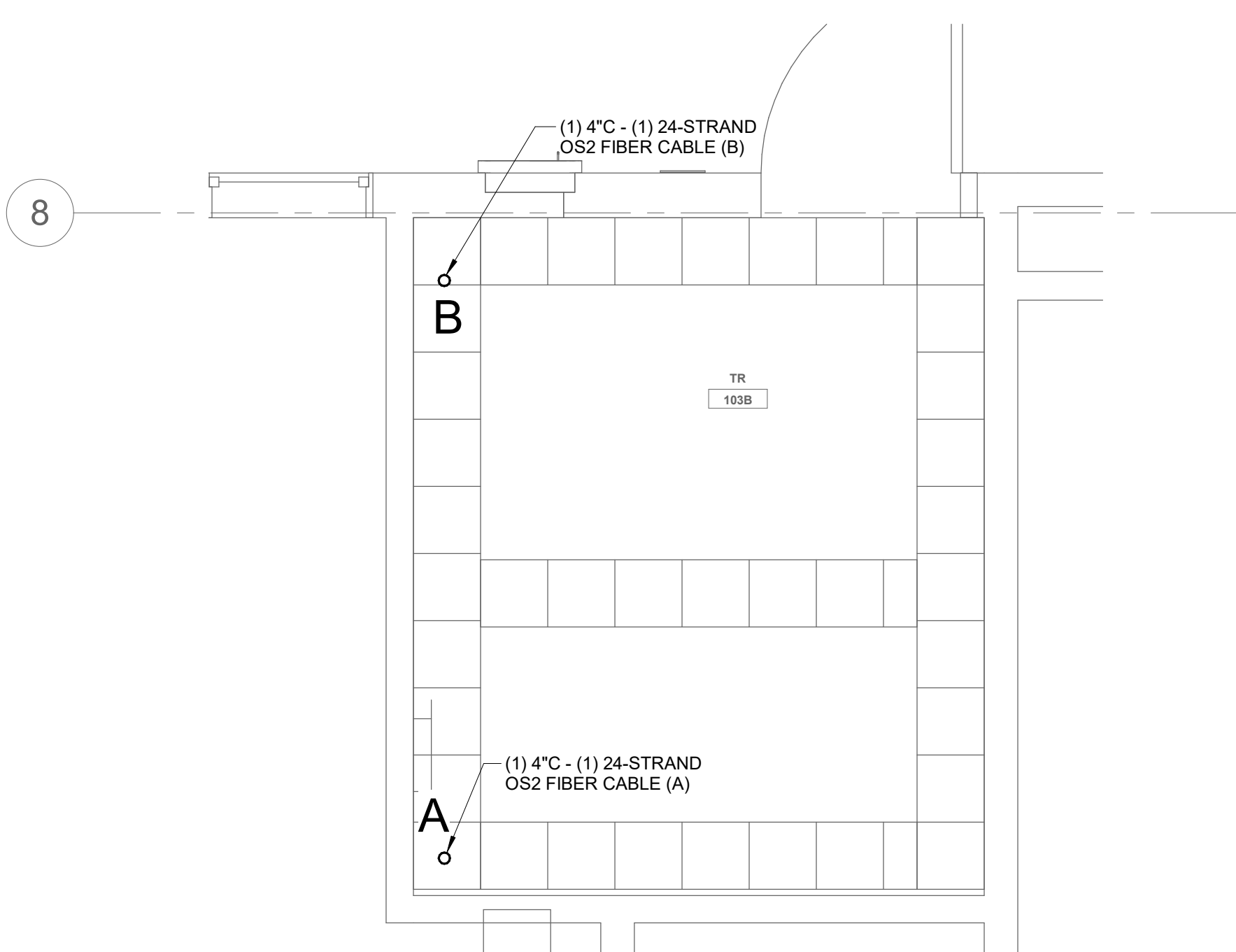
2 TELECOM ROOM PATHWAY TR #103B 1/2" = 1'-0"
