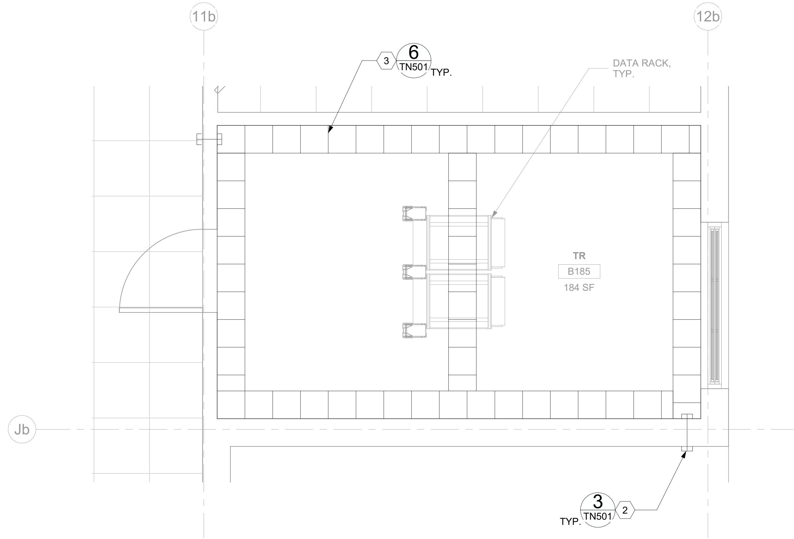
2 RM B185 - TELECOMMUNICATIONS PLAN 148TN101A 1/2" = 1'-0"
