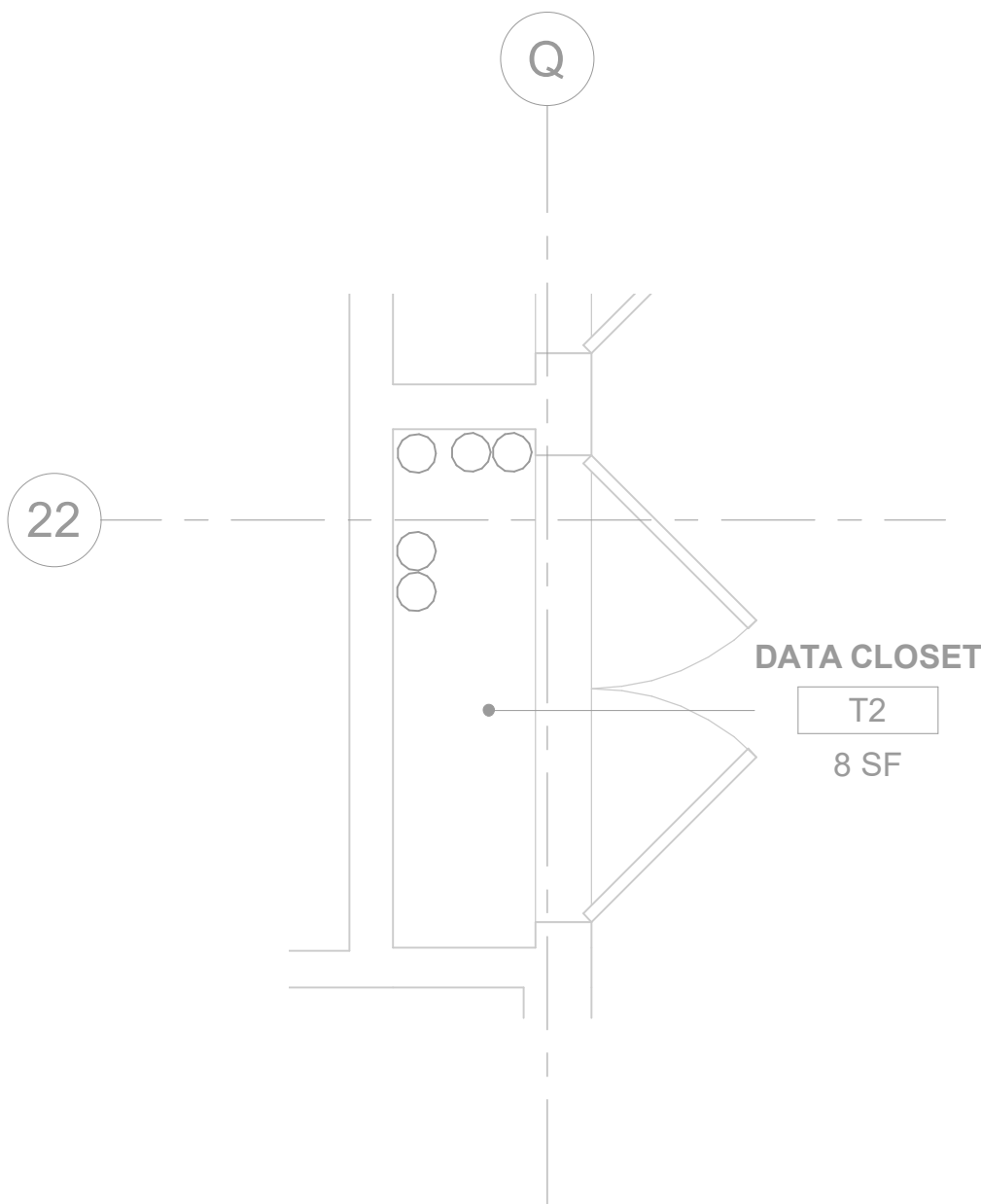
4 RM T2 - OVERHEAD PLAN 146TN101A 1/2" = 1'-0"
