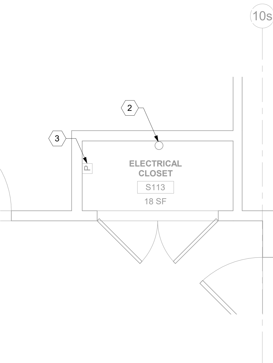
3 RM S113 - DEMOLITION OVERHEAD PLAN 148TN101A 1/2" = 1'-0"
