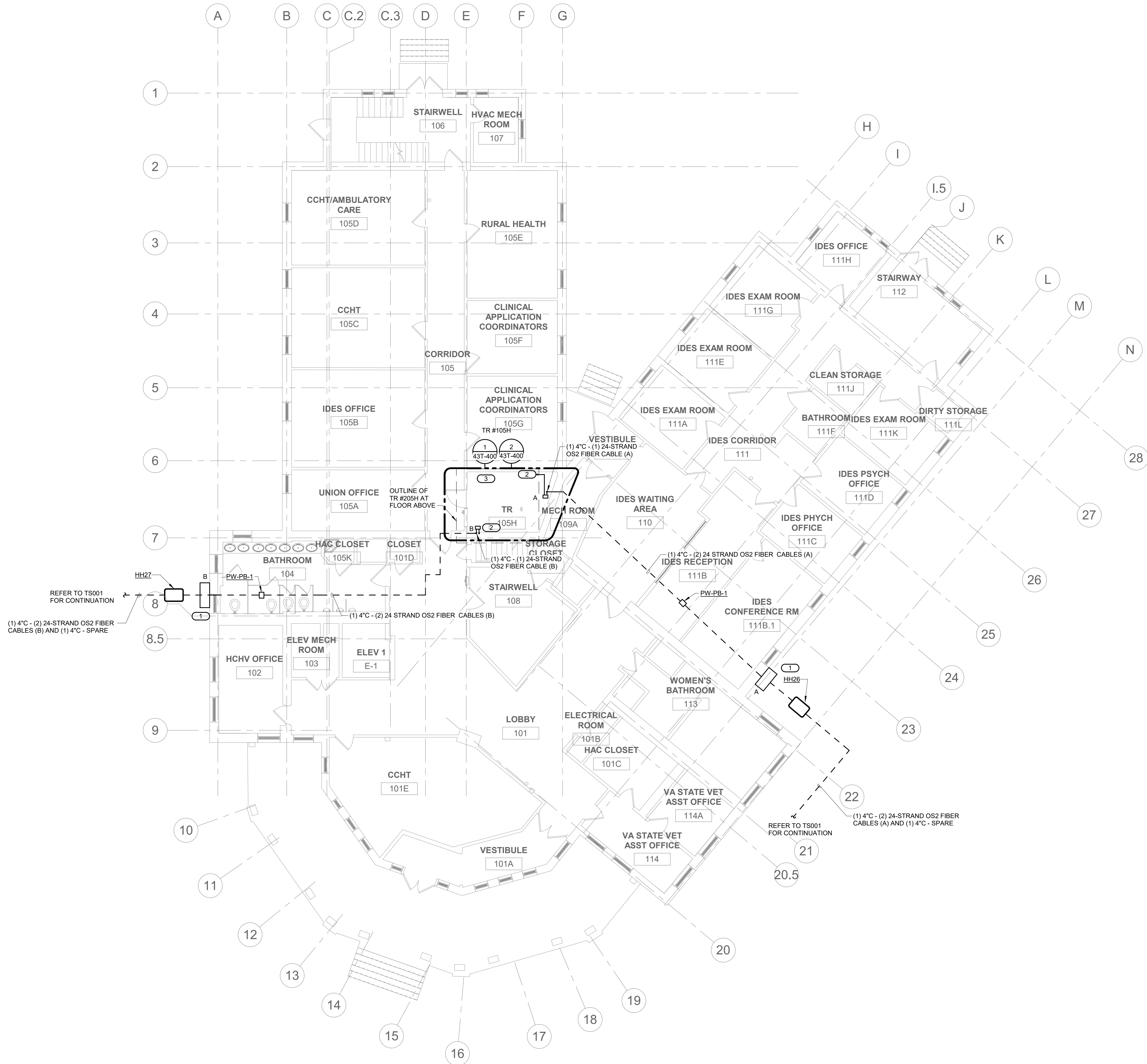
1 LEVEL 01 PLAN - TECHNOLOGY 1/8" = 1'-0"
