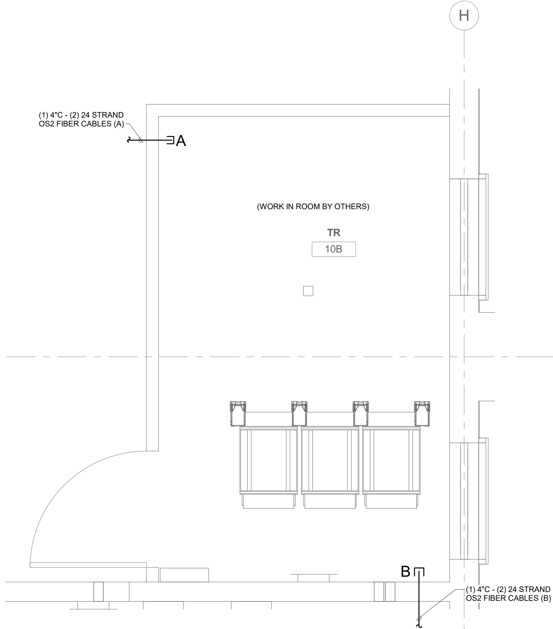
NORTH 1 1/2" = 1'-0" TELECOM ROOM ENLARGEMENT TR #10B KEY NOTES: C # 1. ROUTE CONDUITS UP TO CEILING HEIGHT AND STUB AND BUSH ABOVE CABLE TRAY. CONTINUE ROUTE OF CORE A OPTICAL FIBER CABLES ON CABLE TRAY, THRU PATHWAYS AND INTO MCR #25.
