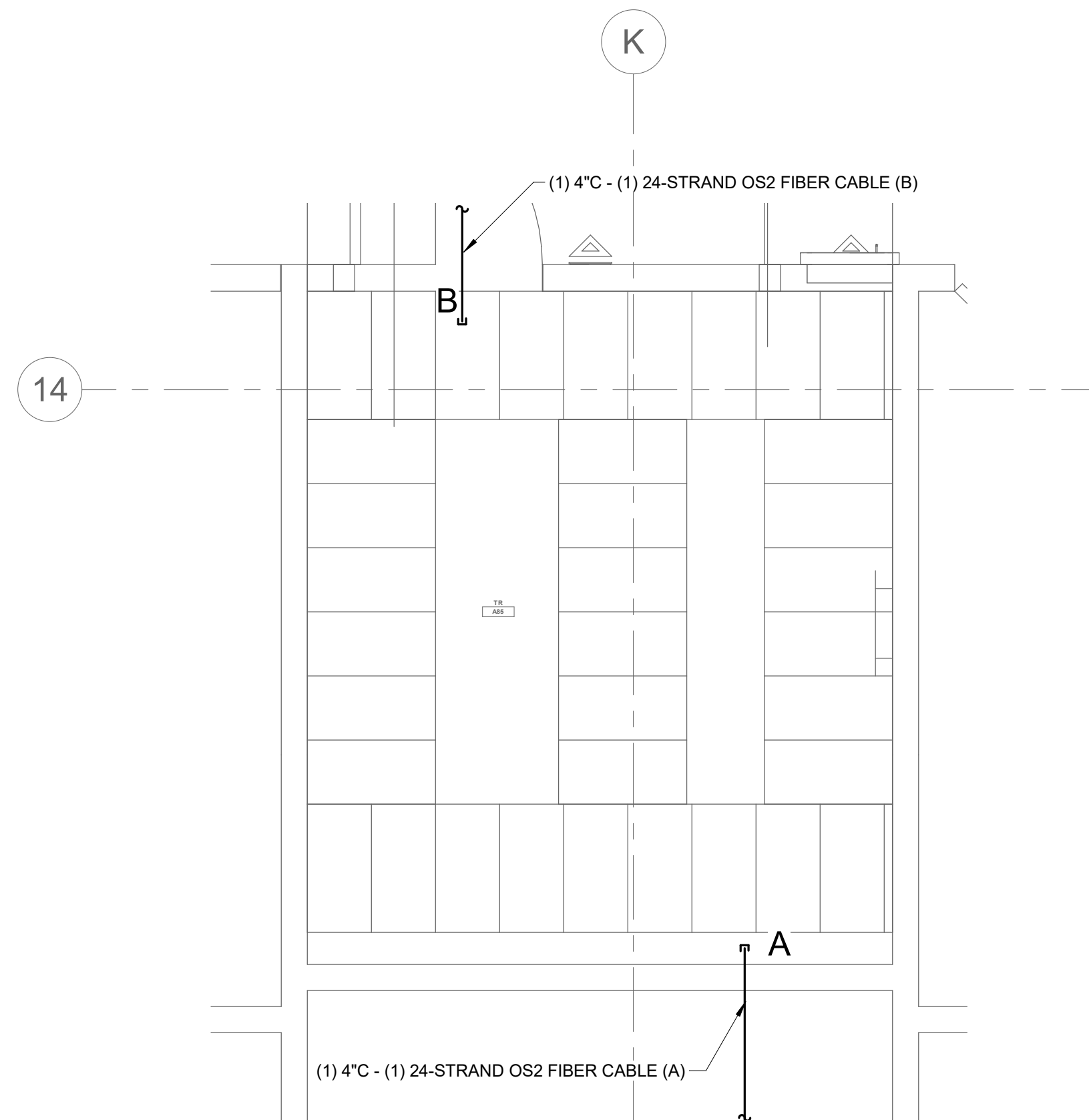
2 TELECOM ROOM PATHWAY PLAN TR #A85 1/2" = 1'-0"
