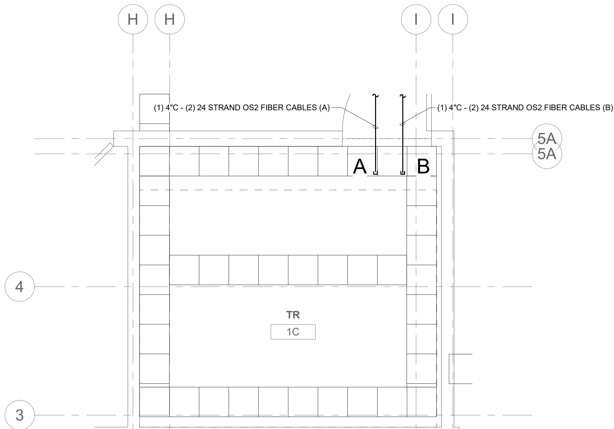
2 TELECOM ROOM PATHWAY TR #36-05 1/2" = 1'-0"
