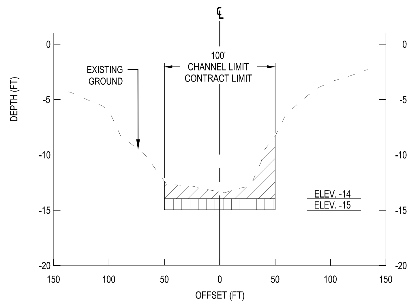
4 TYPICAL SECTION - CAPE MAY HARBOR - STA -10+249 TO -8+234 AS SHOWN
