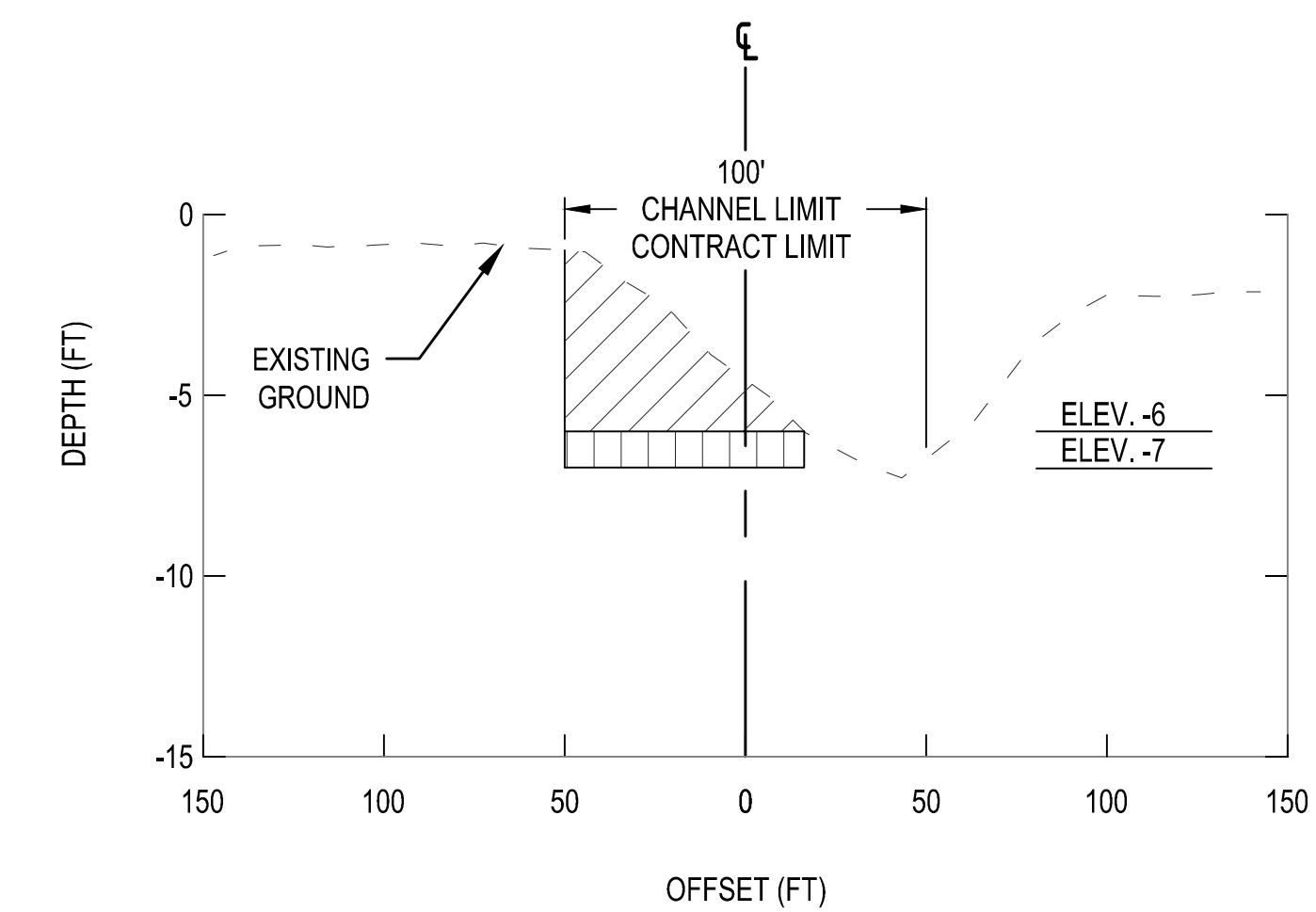
9 TYPICAL SECTION - NJIWW - MARKER 152 TO 163 AS SHOWN
