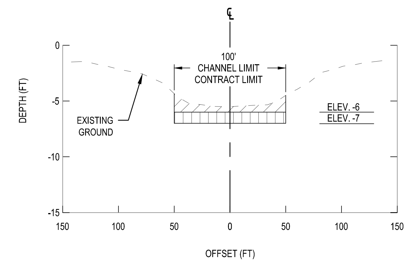
3 OPTION 1 - TYPICAL SECTION - NJIWW - MARKER 276 TO 282 AS SHOWN
