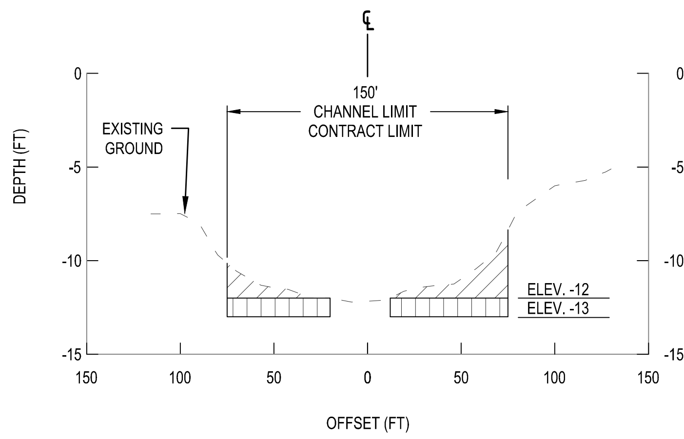
1 TYPICAL SECTION - CAPE MAY FERRY - STA -12+52 TO -4+00 AS SHOWN
