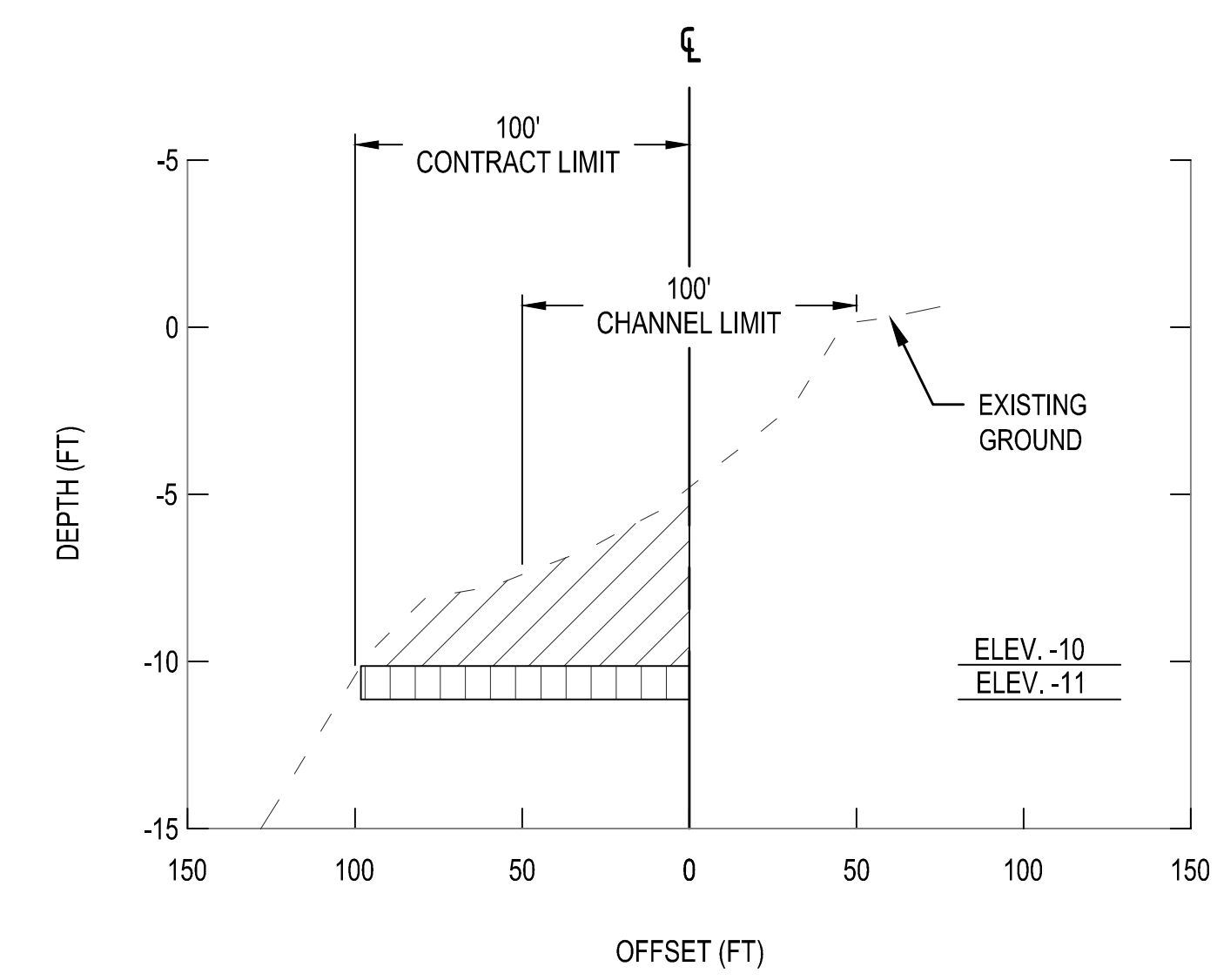
3 TYPICAL SECTION - CAPE MAY FERRY - STA 11+00 TO 17+37 AS SHOWN
