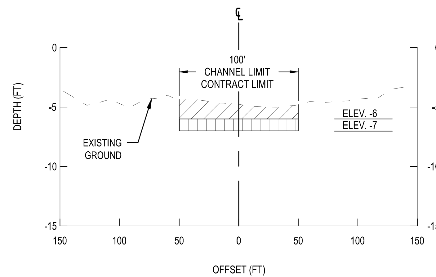
8 TYPICAL SECTION - NJIWW - MARKER 206 TO 209 AS SHOWN
