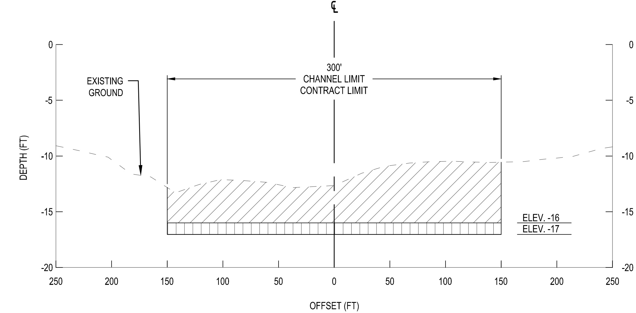
6 TYPICAL SECTION - CAPE MAY HARBOR - STA -6+700 TO -2+000 AS SHOWN
