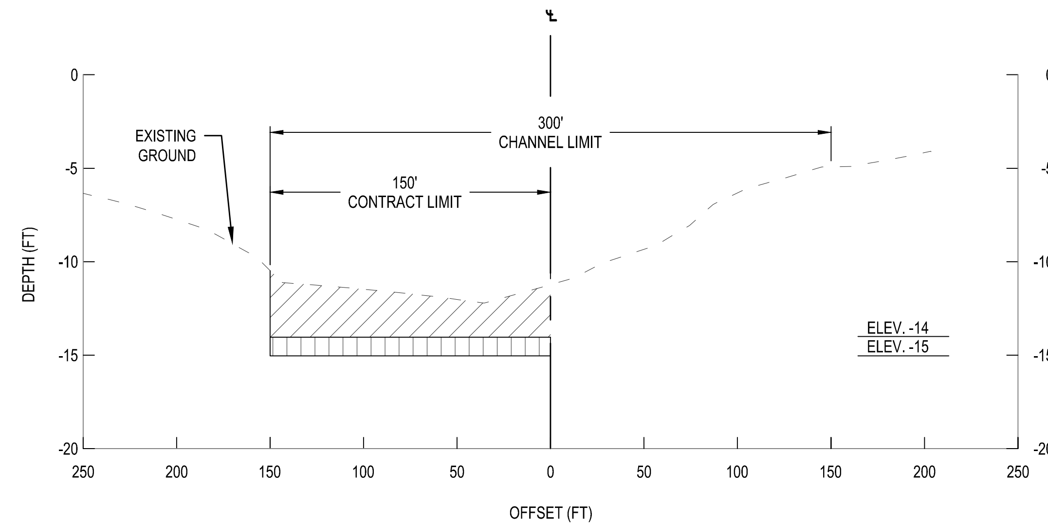
5 TYPICAL SECTION - CAPE MAY HARBOR - STA -8+234 TO -6+700 AS SHOWN
