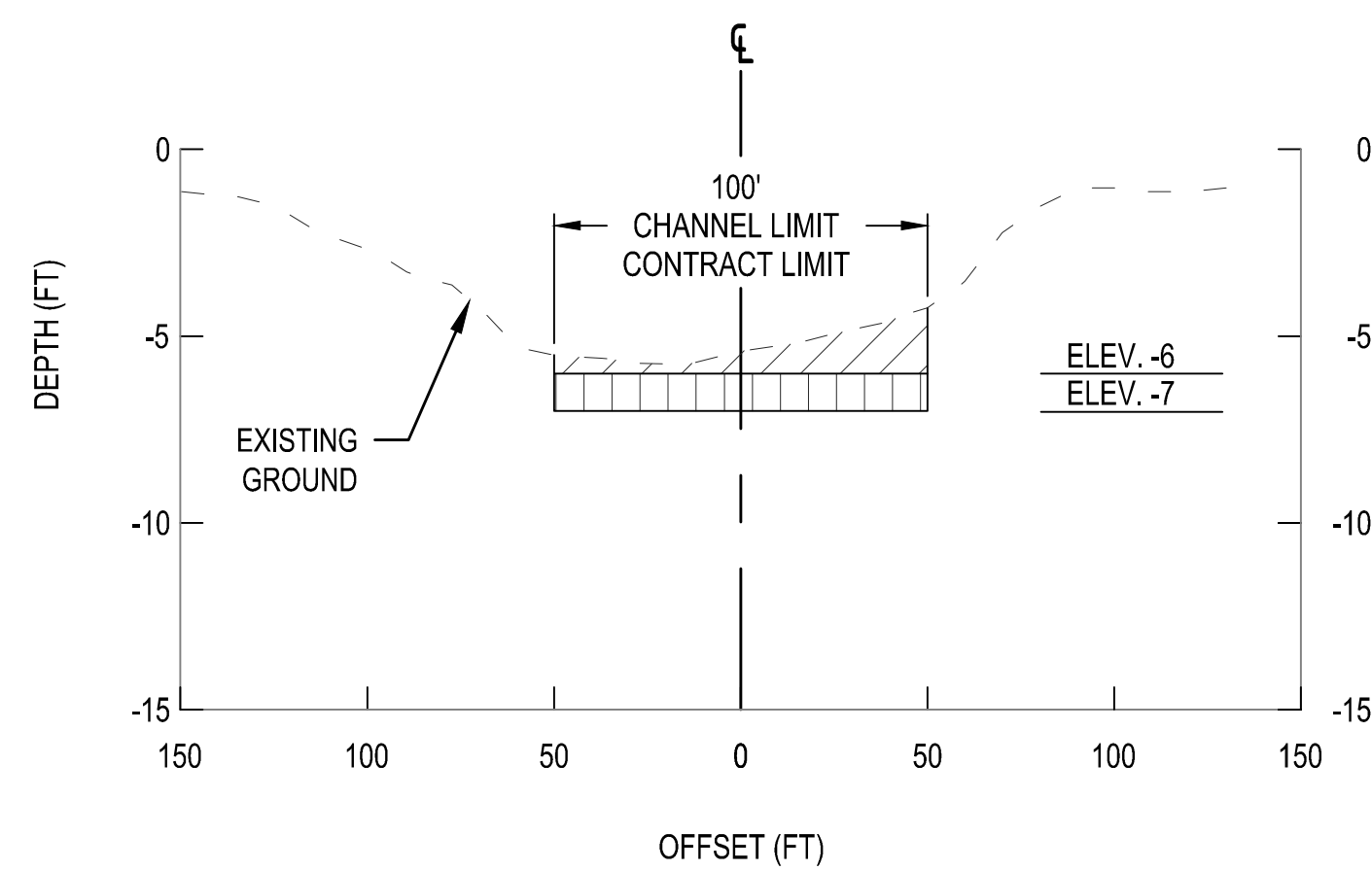
7 TYPICAL SECTION - NJIWW - MARKER 385 TO 400 AS SHOWN
