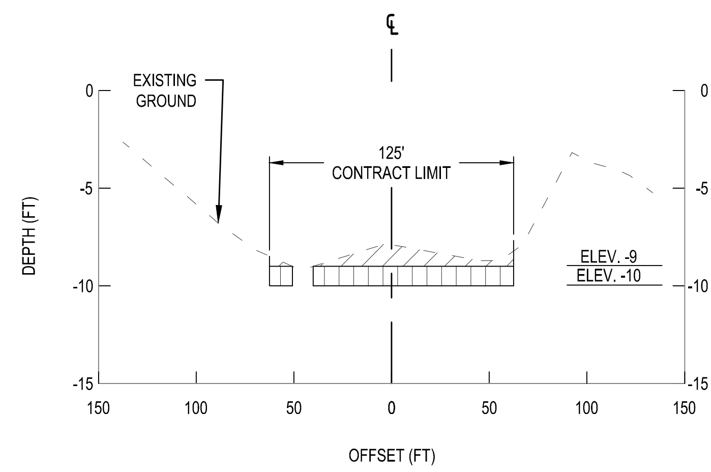
2 TYPICAL SECTION - OYSTER CREEK - MARKER 37 TO 42 AS SHOWN
