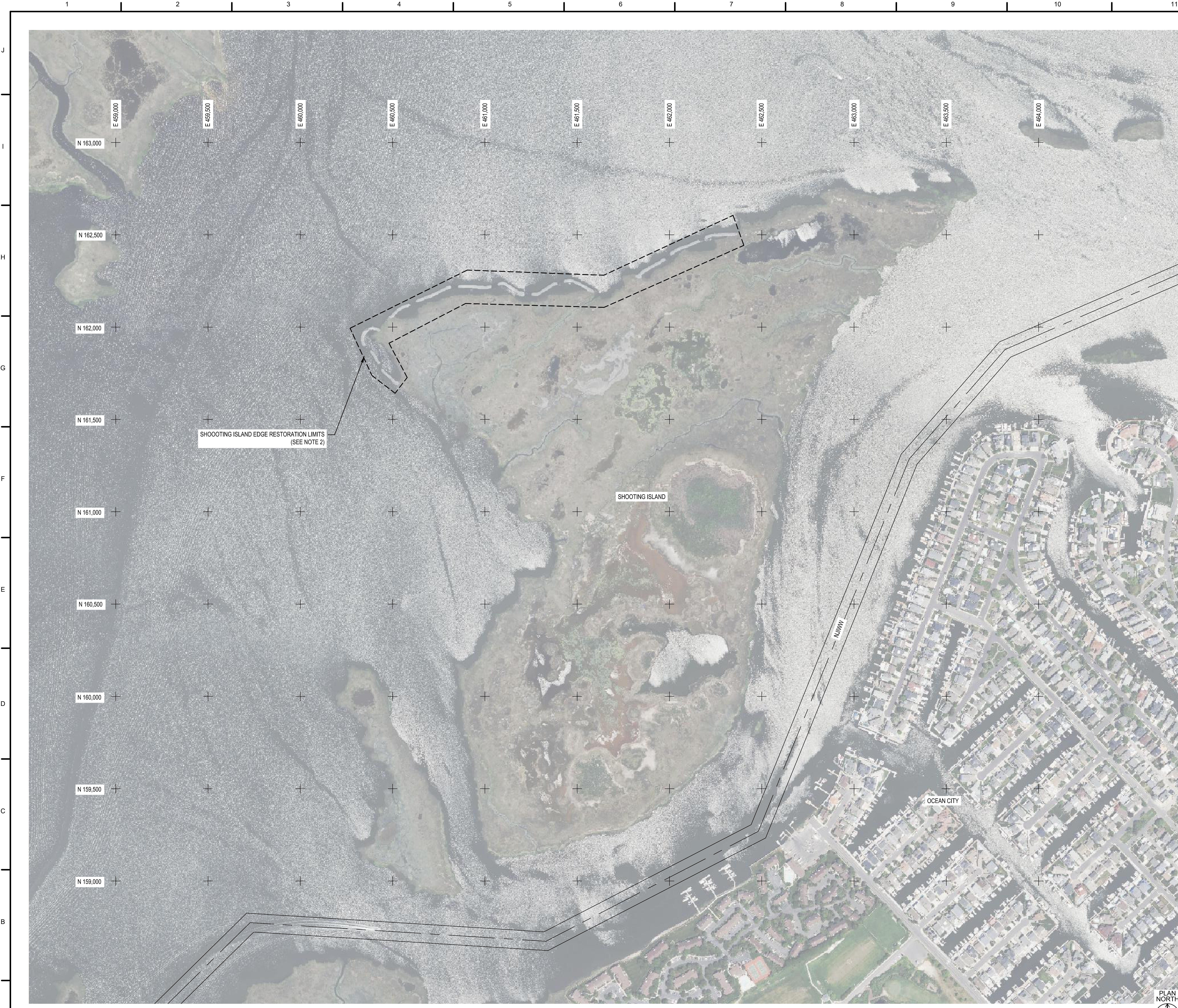
1 PLAN - SHOOTING ISLAND BENEFICIAL USE AREA SCALE: 1" = 200'-0"
