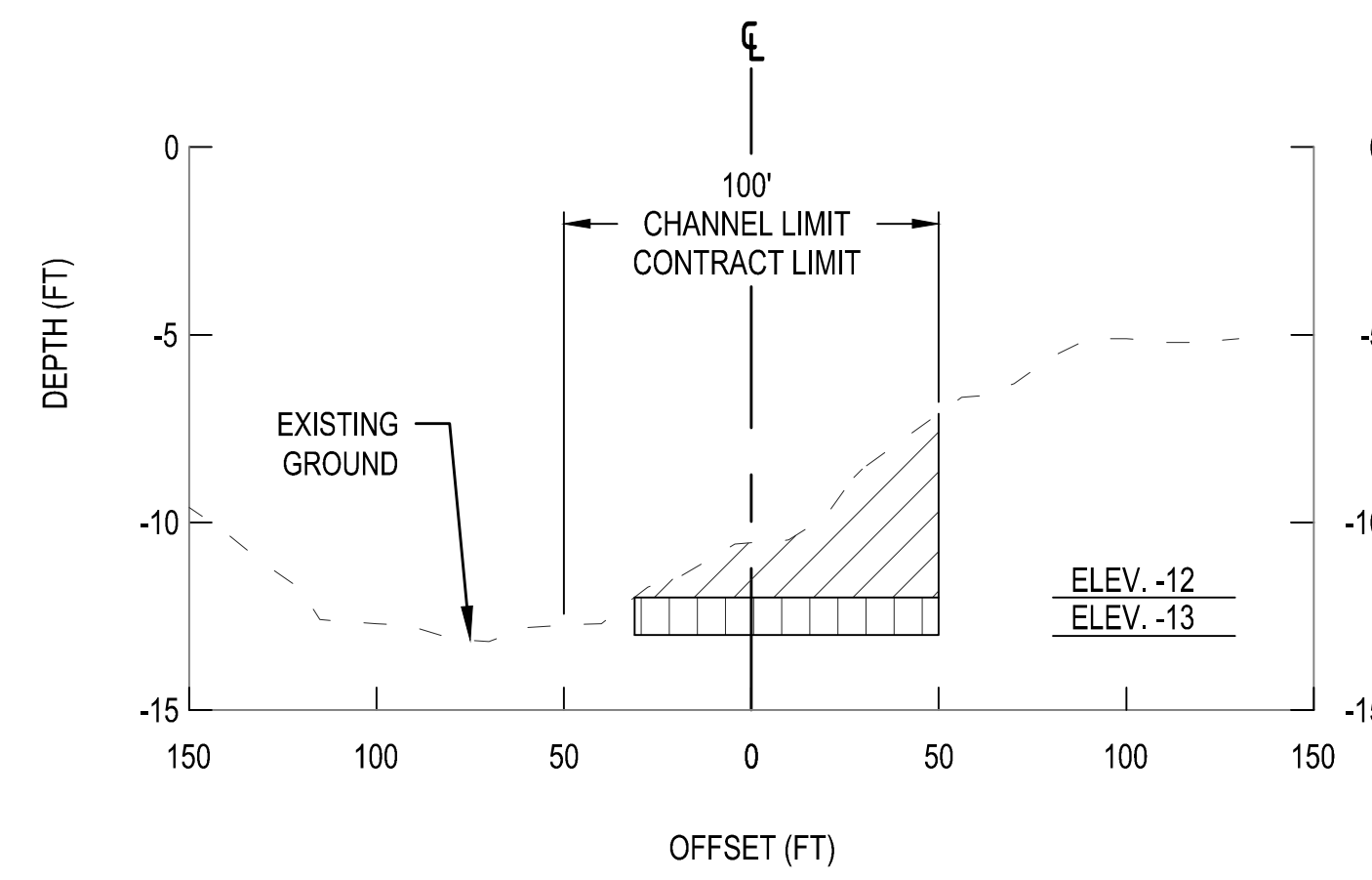
2 TYPICAL SECTION - CAPE MAY FERRY - STA 0+00 TO 11+00 AS SHOWN
