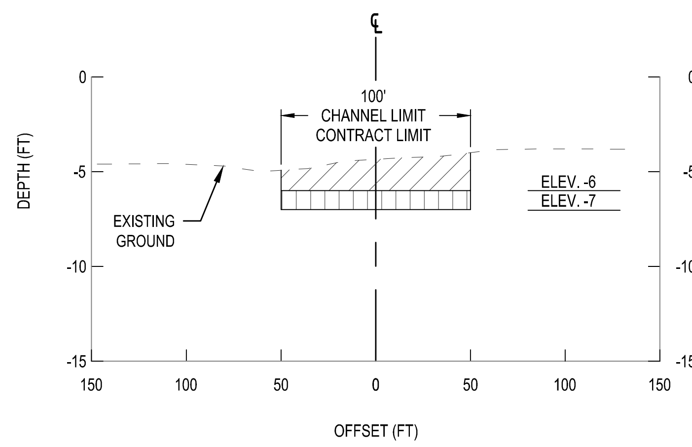
1 TYPICAL SECTION - NJIWW - MARKER 135 TO 145 AS SHOWN
