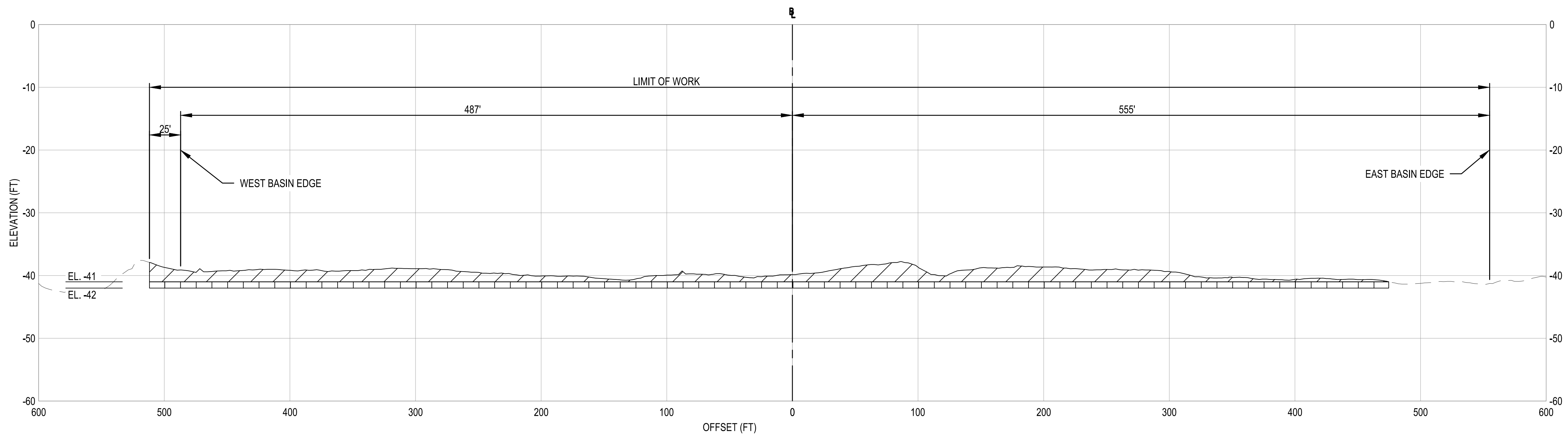
A1 CROSS SECTION - FAIRLESS TURNING BASIN (STA. 0+350) SCALE IN FEET
