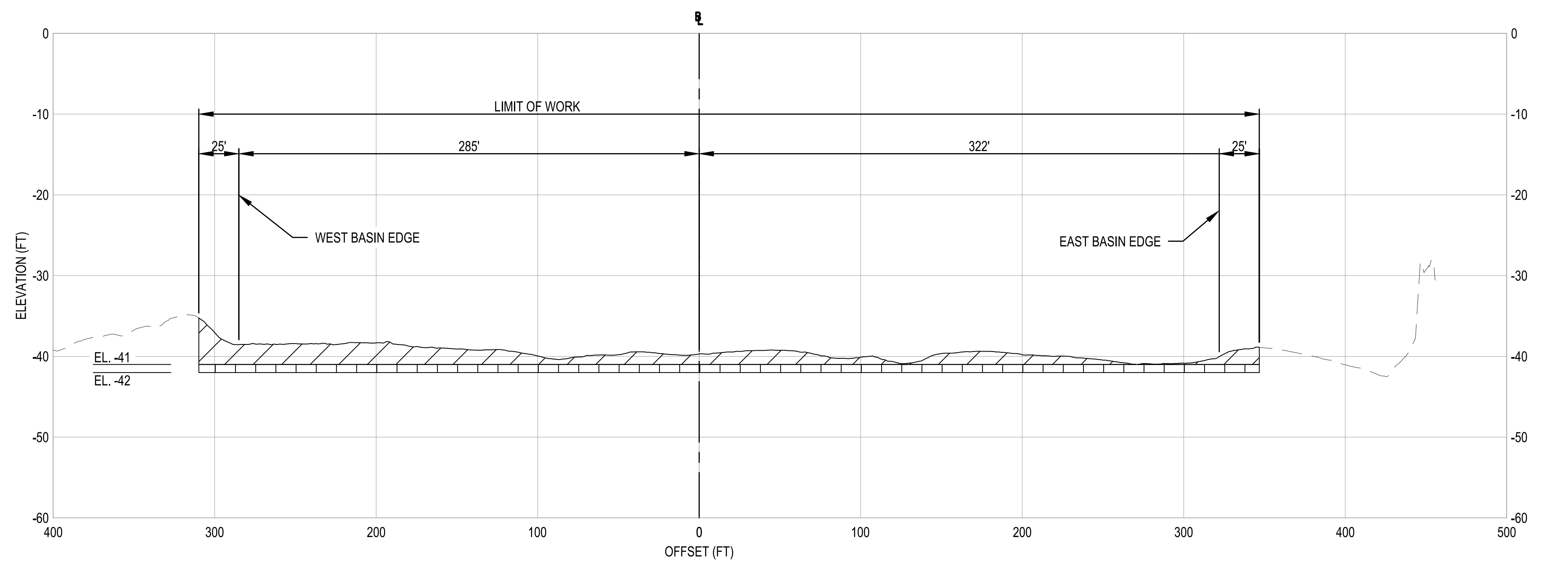
G4 CROSS SECTION - FAIRLESS TURNING BASIN (STA. 0+750) SCALE IN FEET
