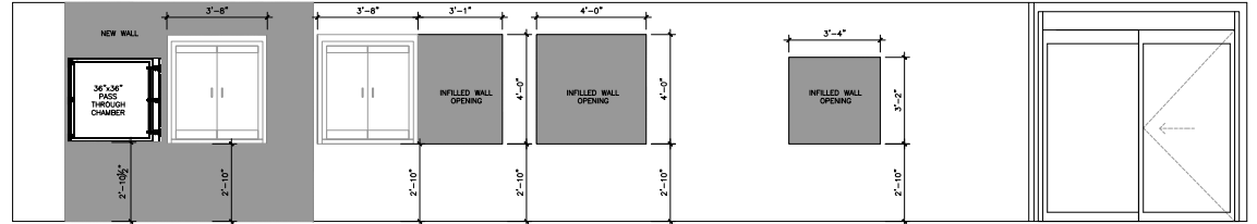
3 PREP/PACKAGE/INSPECT ROOM-SG87 INTERIOR ELEVATION -E SCALE: 1/2"=1'-0"
