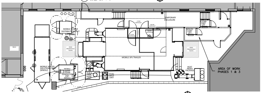
2 TEMPORARY MOBILE SPS SITE PHASING PLAN SCALE: 1/8"=1'-0"
