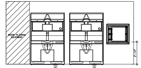
4 SCOPE DECON-SG86A - INTERIOR ELEVATION -E SCALE: 1/2"=1'-0"
