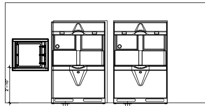
5 SCOPE PROCESSING-SG96- INTERIOR ELEVATION -W SCALE: 1/2"=1'-0"
