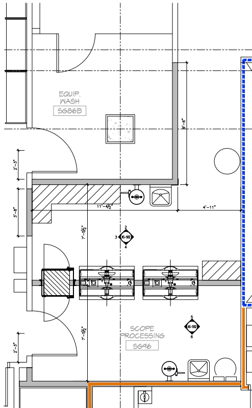
1 ENLARGED SCOPE PROCESSING SG96, PORTION OF EQUIPMENT WASH SG86B & PORTION OF SCOPE DECON-SG86A PLANS SCALE: 1/2"=1'-0"
