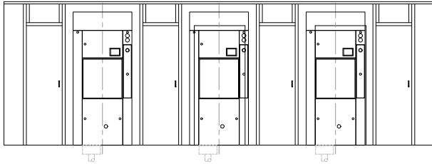
3 PREP/PACKAGE/INSPECT ROOM-SG87 INTERIOR ELEVATION -S SCALE: 1/2"=1'-0"
