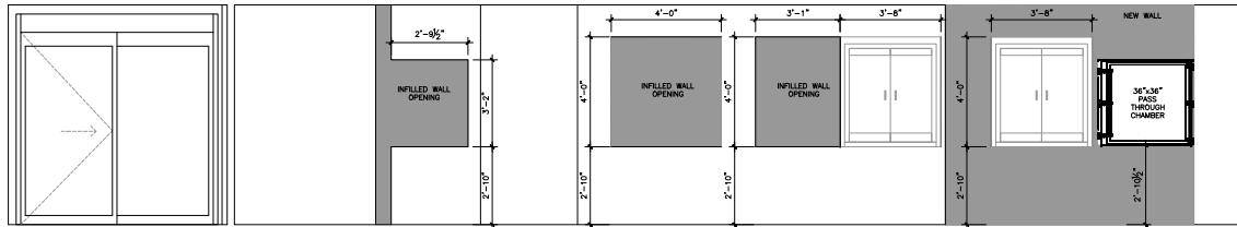
4 MAIN DECON ROOM-SG86 INTERIOR ELEVATION -W SCALE: 1/2"=1'-0"
