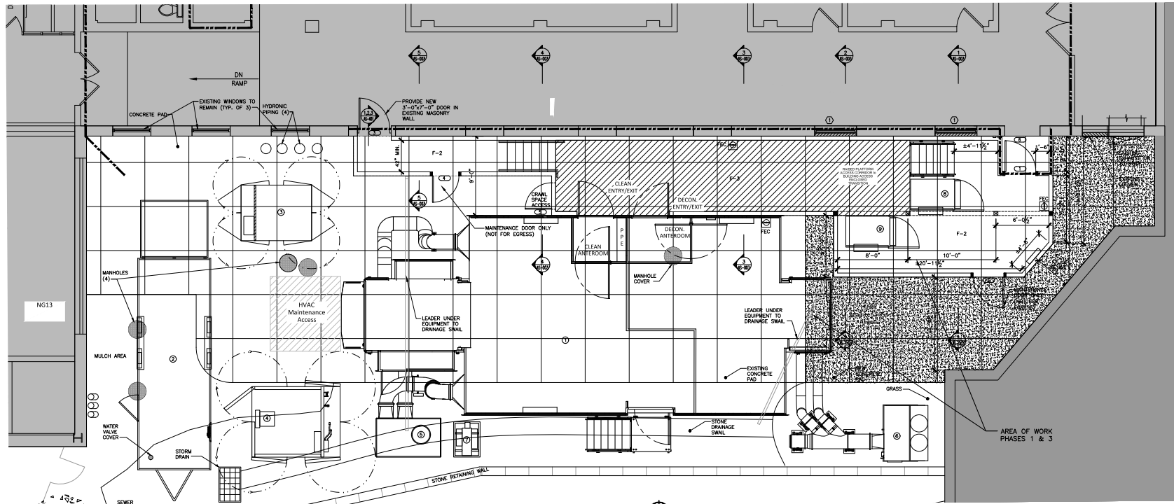
1 SITE PLAN SCALE: 1/4"=1'-0"
