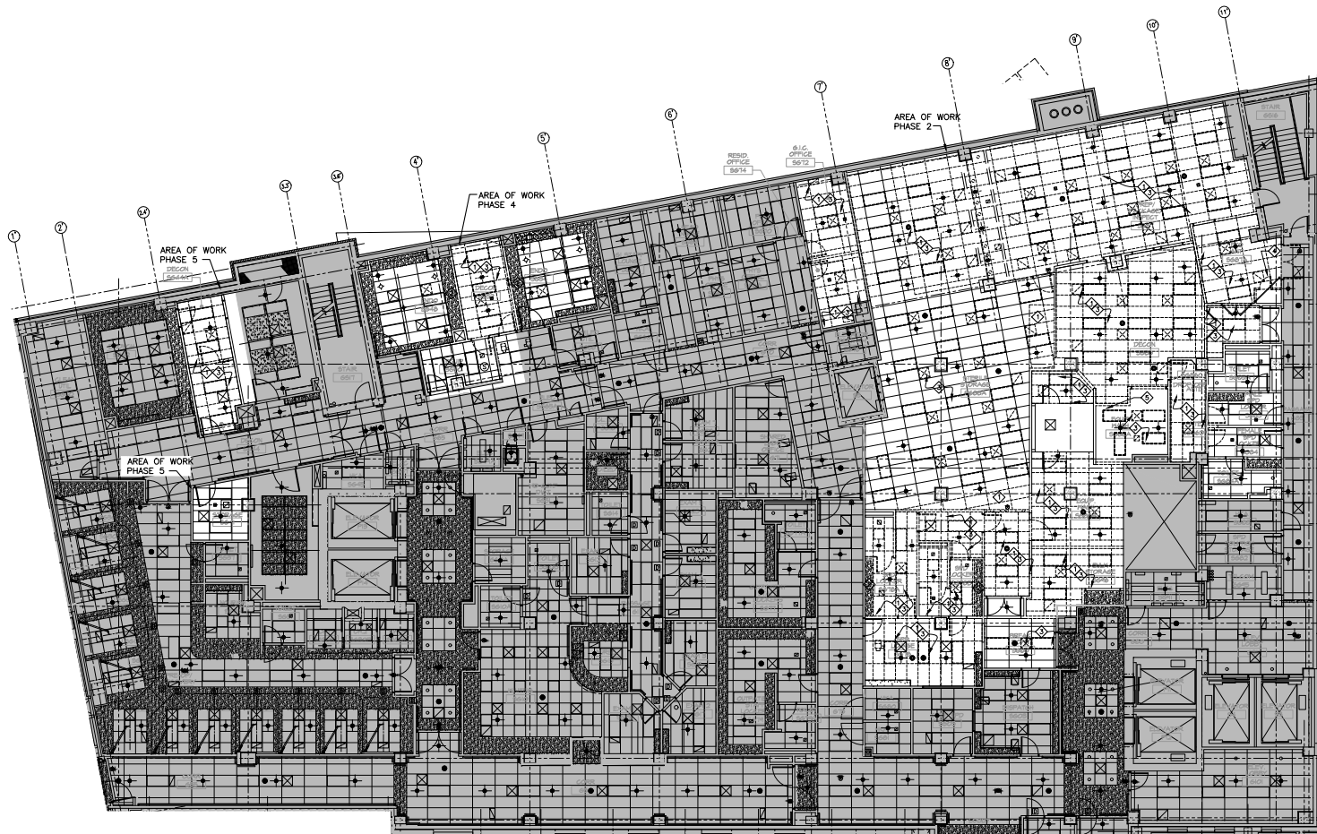
1 ARCHITECTURAL: DEMOLITION GROUND FLOOR REFLECTIVE CEILING PLAN SCALE: 1/8"=1'-0"
