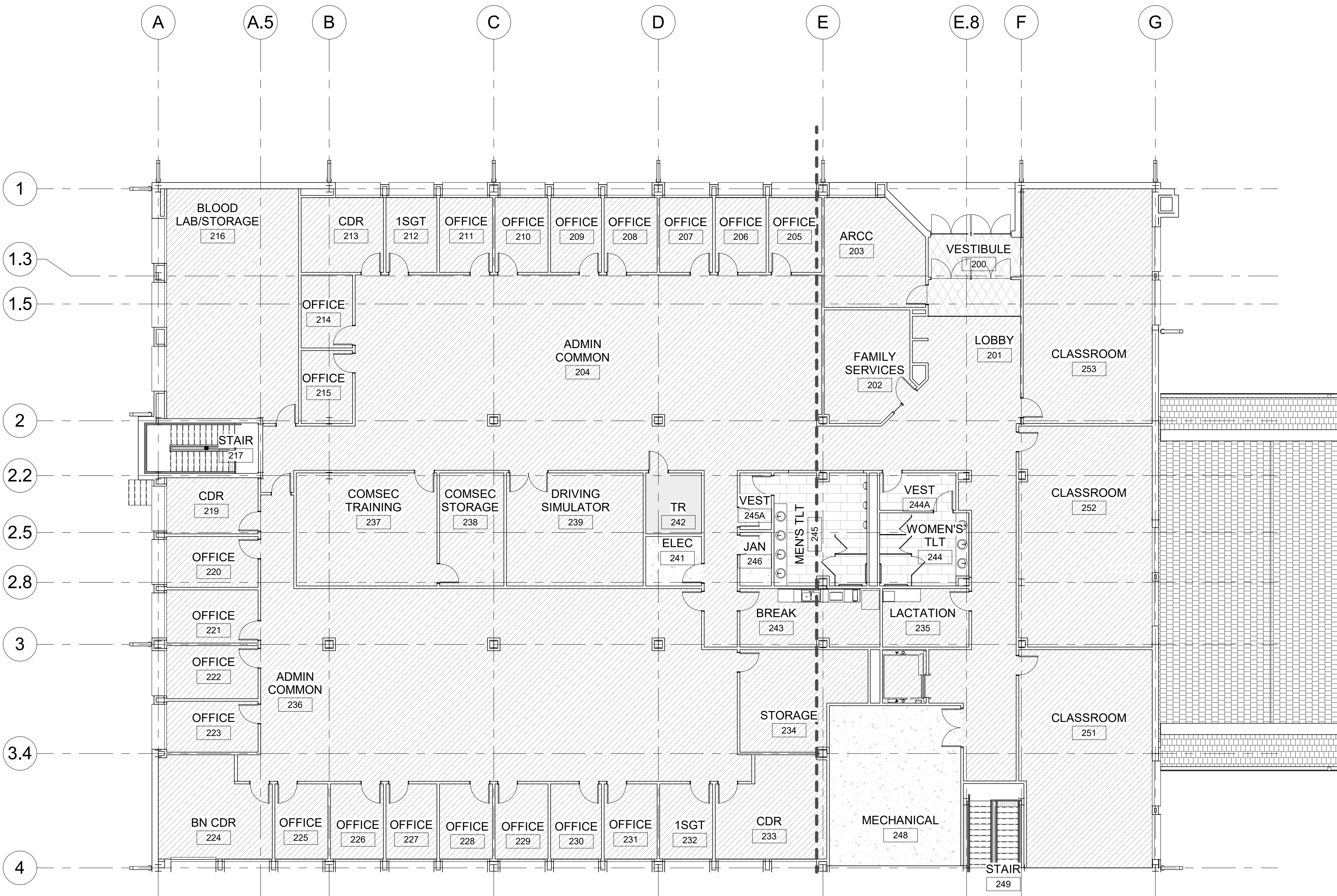
(A1) PROPOSED OVERALL FINISH PLAN - FLOOR 02 SCALE 3/32" = 1'-0"
