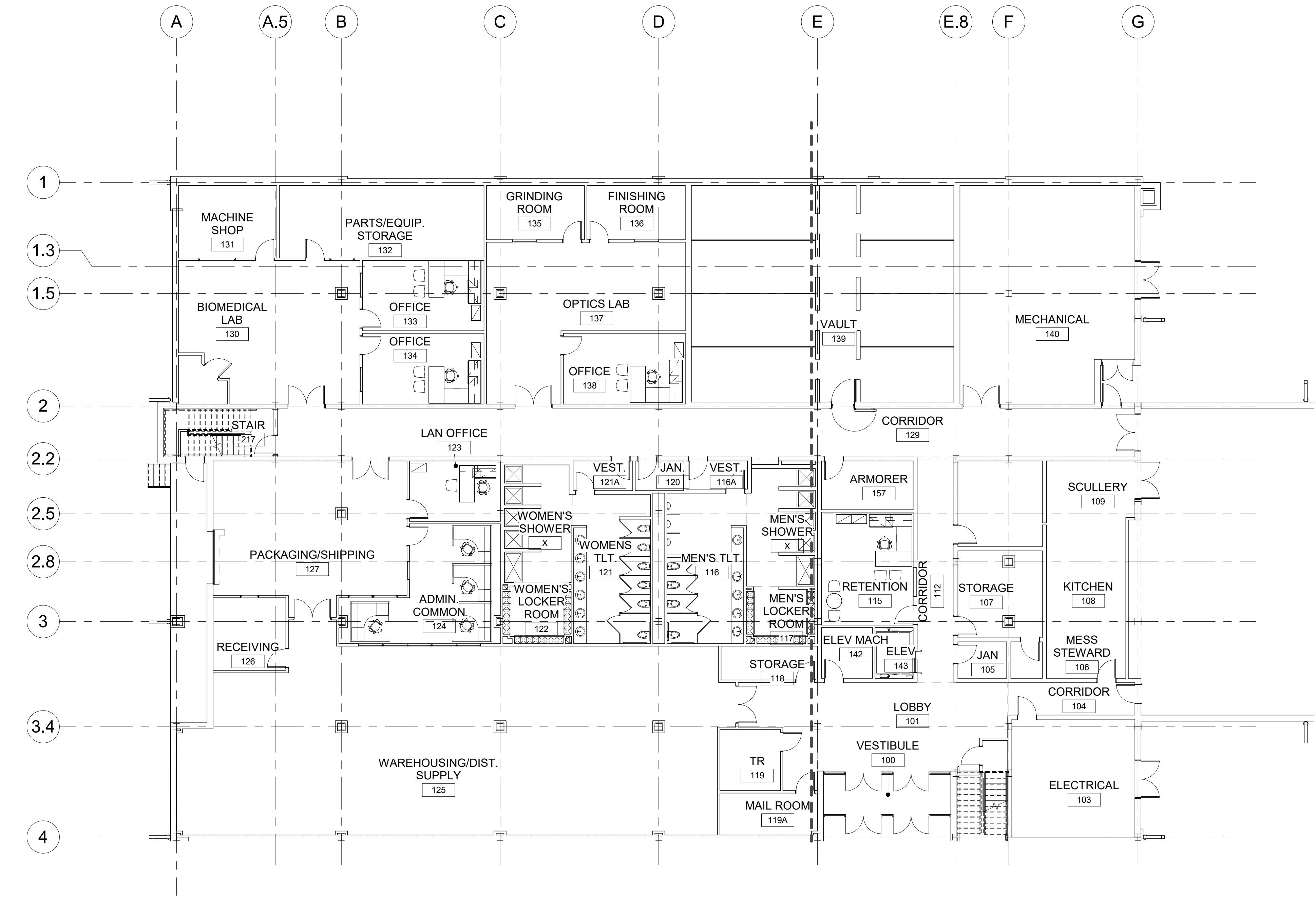
(A1) PROPOSED OVERALL FURNITURE PLAN - FLOOR 01 SCALE 3/32" = 1'-0"
