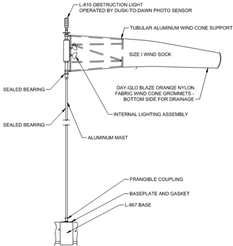
SUPPLEMENTAL WIND CONE - TYPE L-806 NTS
