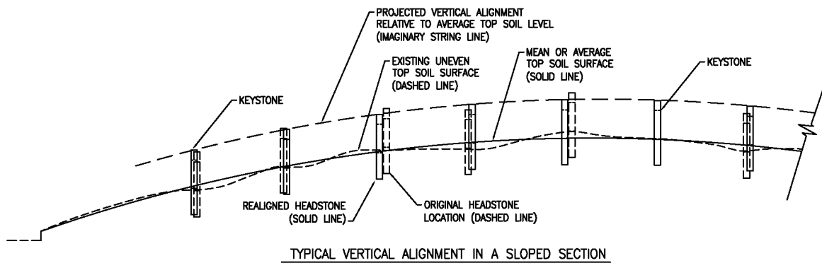
FIGURE 3 ELEVATION VIEW OF BURIAL SECTION REALIGNMENT
