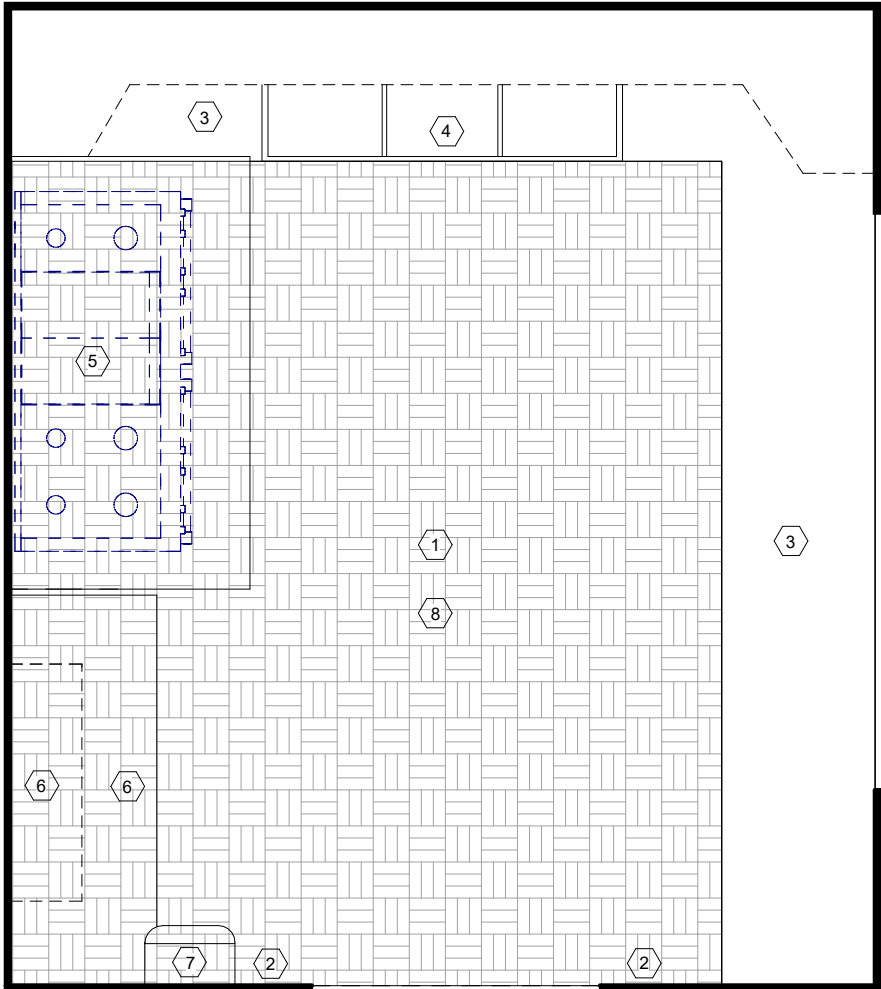
2 KITCHEN DEMOLITION PLAN 3/8" = 1'-0"
