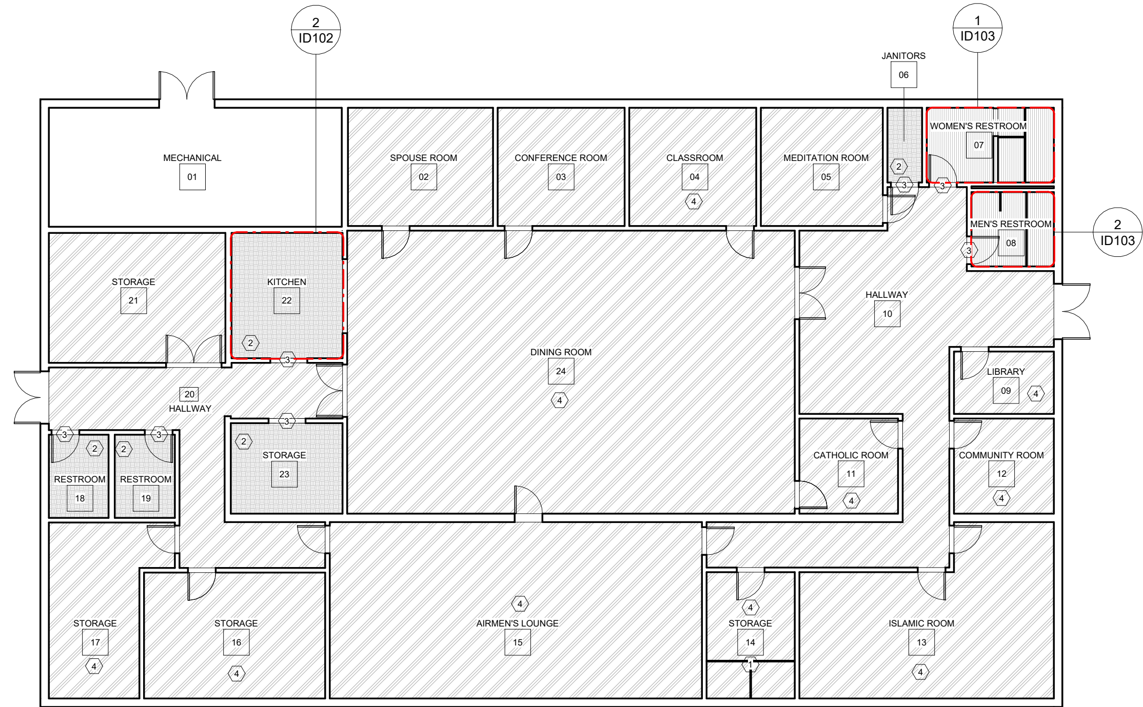
1 DEMOLITION PLAN 3/32" = 1'-0"
