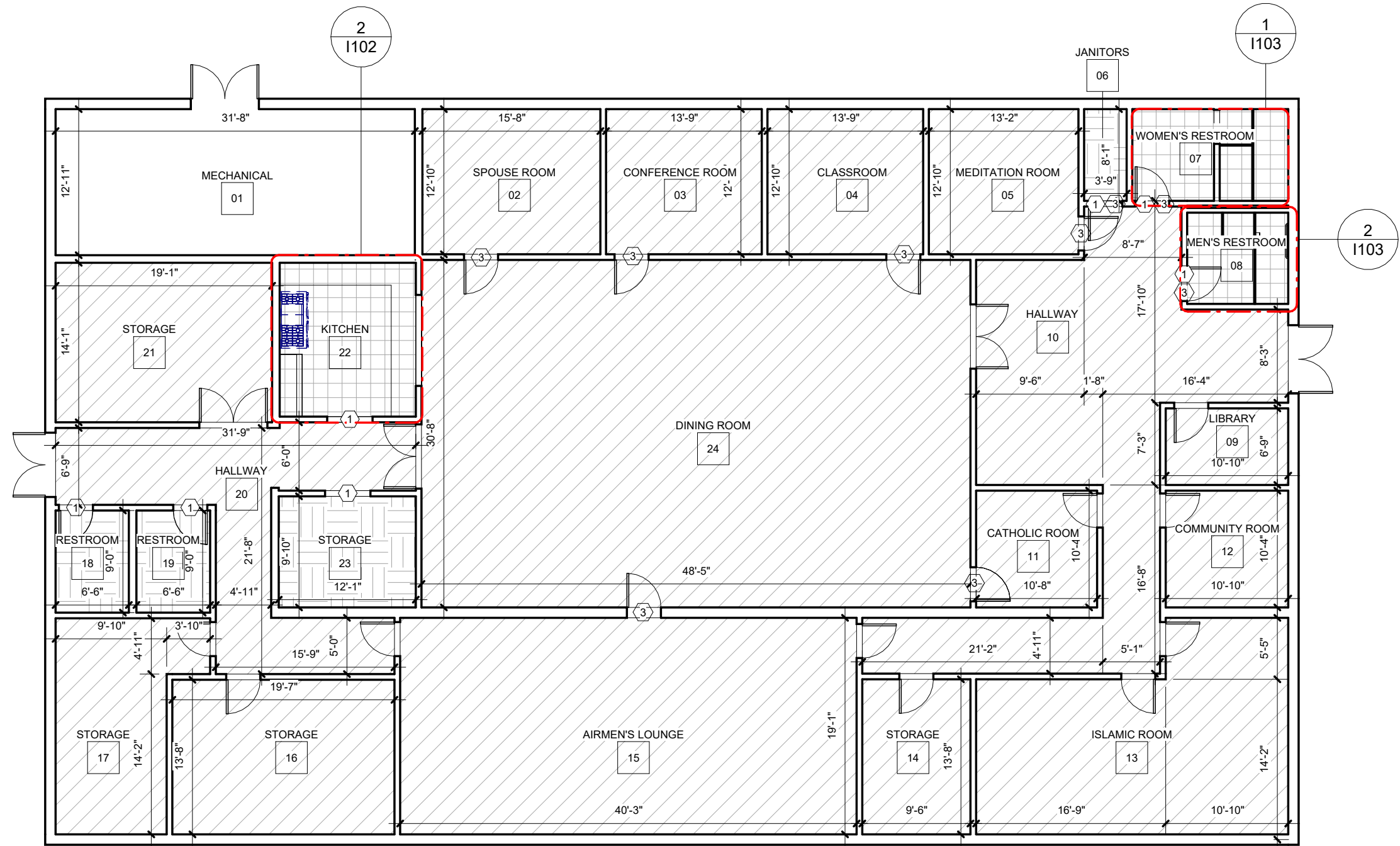
1 FINISH PLAN 3/32" = 1'-0"
