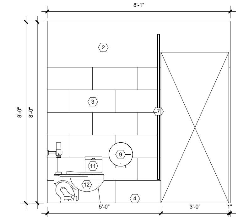
3 NORTH WOMEN'S RESTROOM ELEVATION 3/8" = 1'-0"
