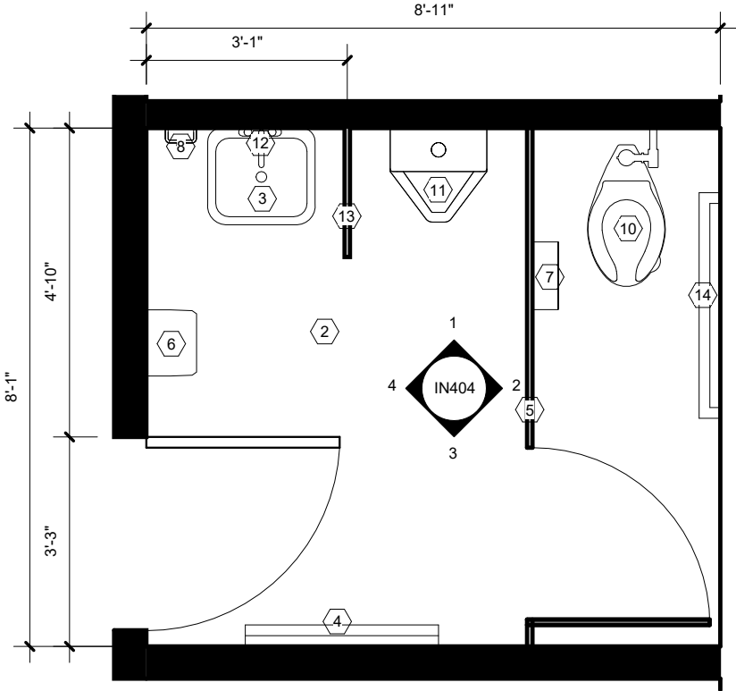
2 MEN'S RESTROOM FINISH PLAN 3/8" = 1'-0"
