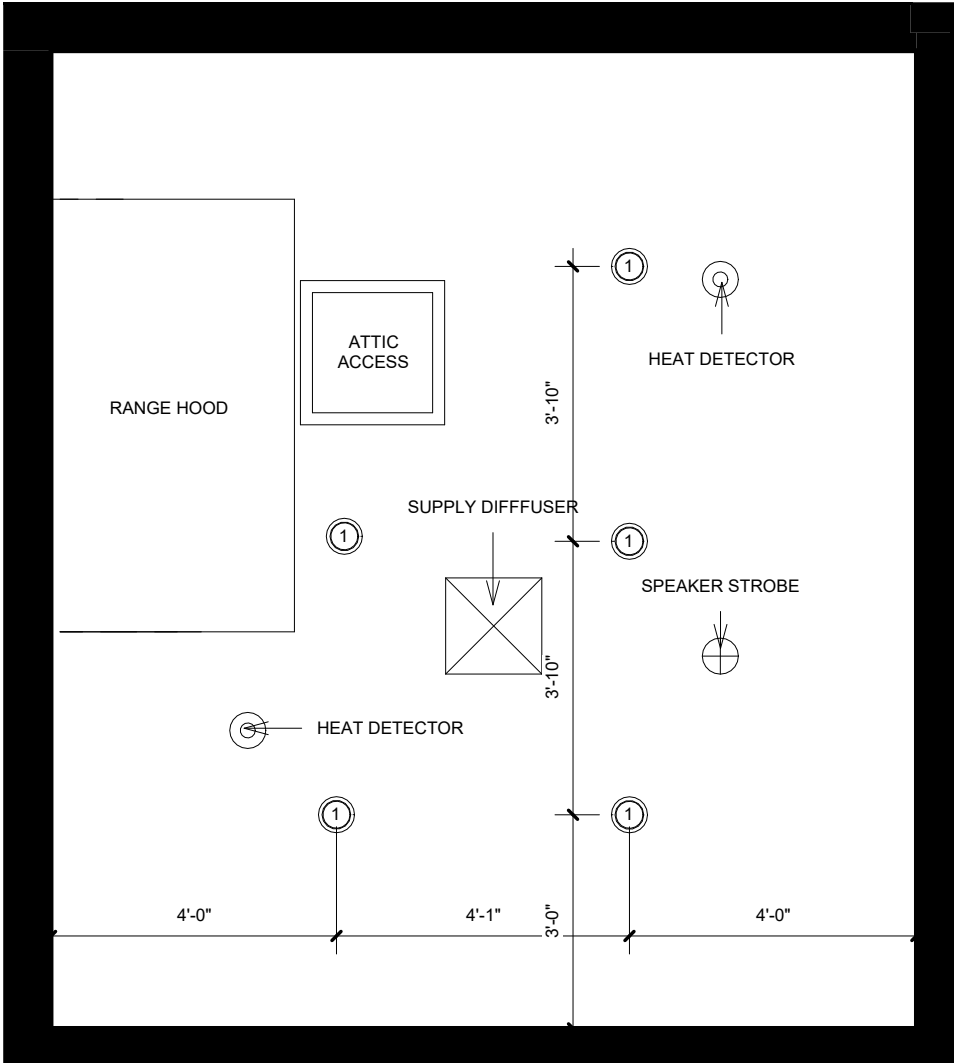
1 KITCHEN REFLECTED CEILING PLAN 3/8" = 1'-0"
