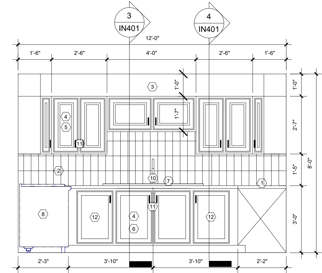
2 EAST KITCHEN ELEVATION 3/8" = 1'-0"
