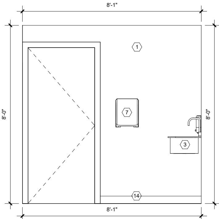
4 NORTH MEN'S RESTROOM ELEVATION 3/8" = 1'-0"
