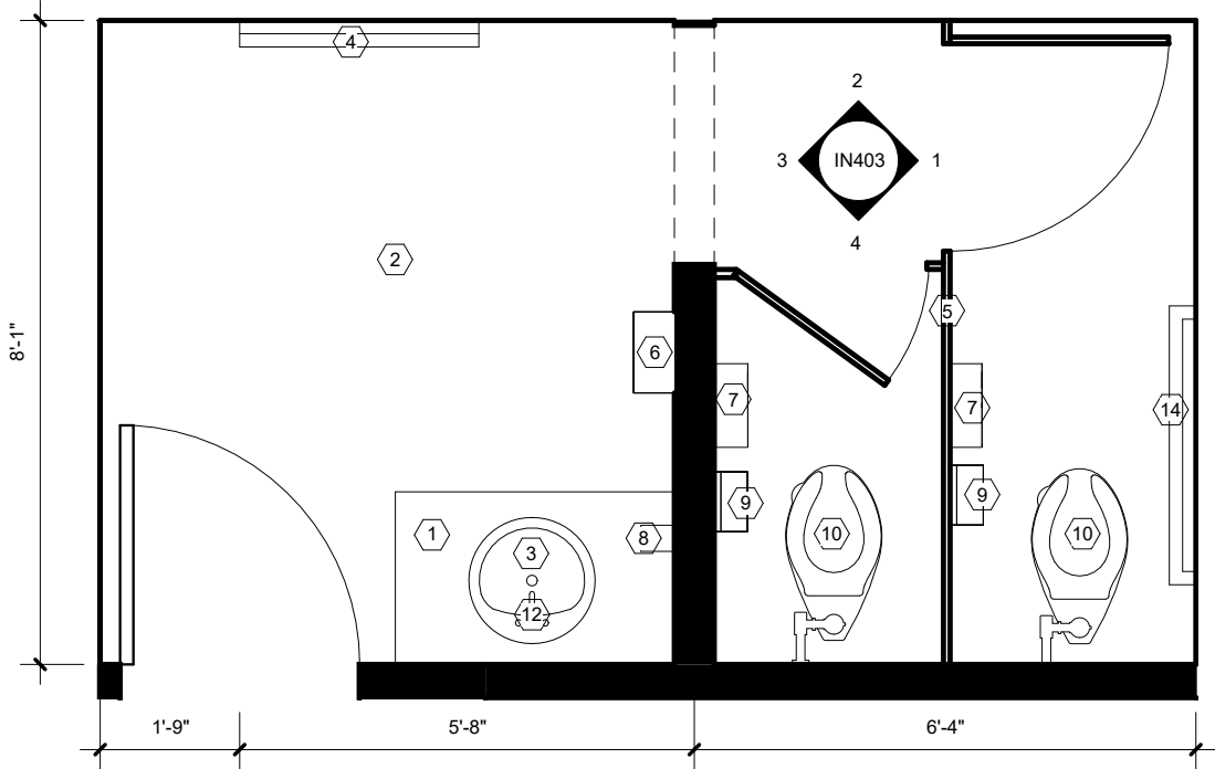
1 WOMEN'S RESTROOM FINISH PLAN 3/8" = 1'-0"
