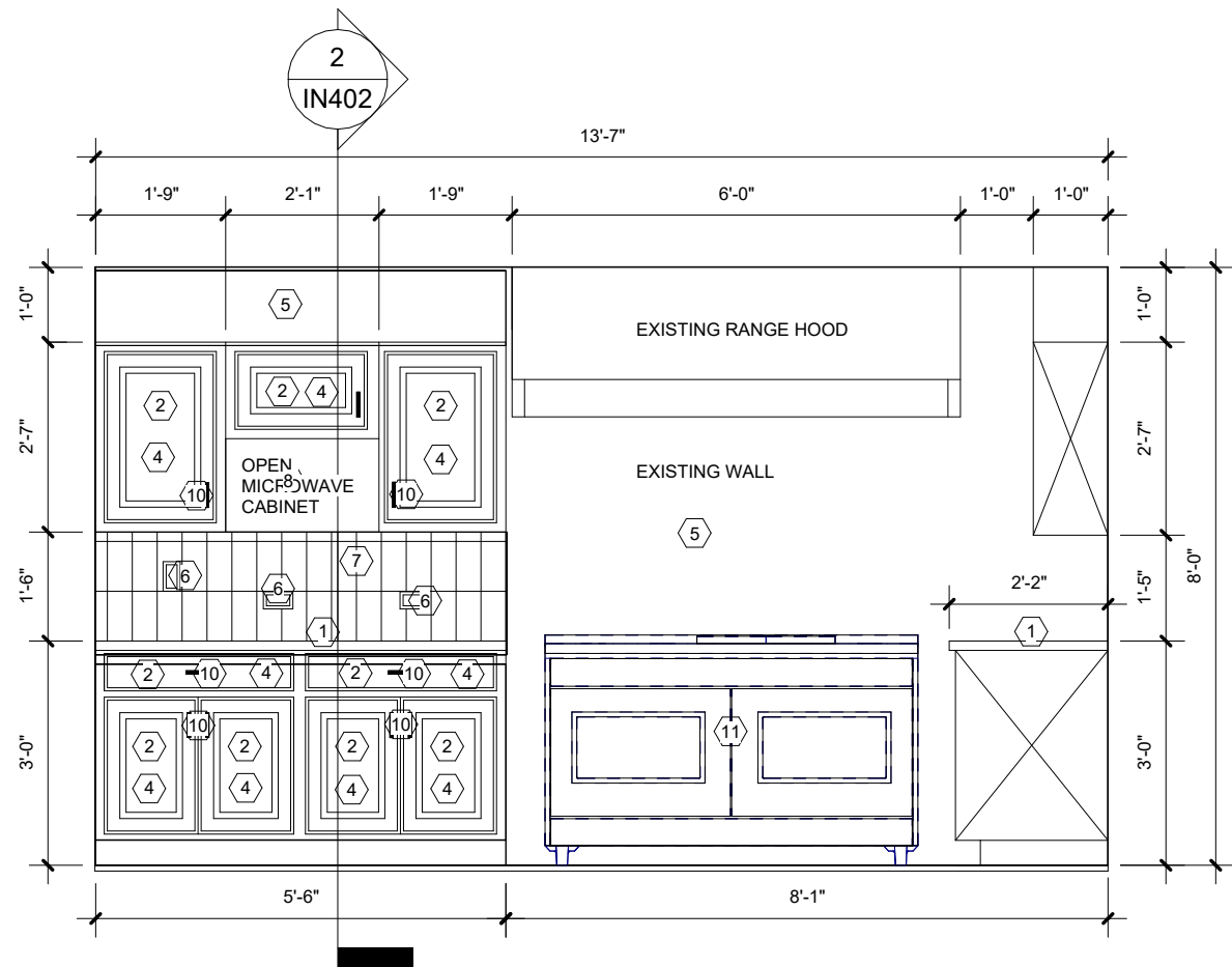
1 NORTH KITCHEN ELEVATION 3/8" = 1'-0"
