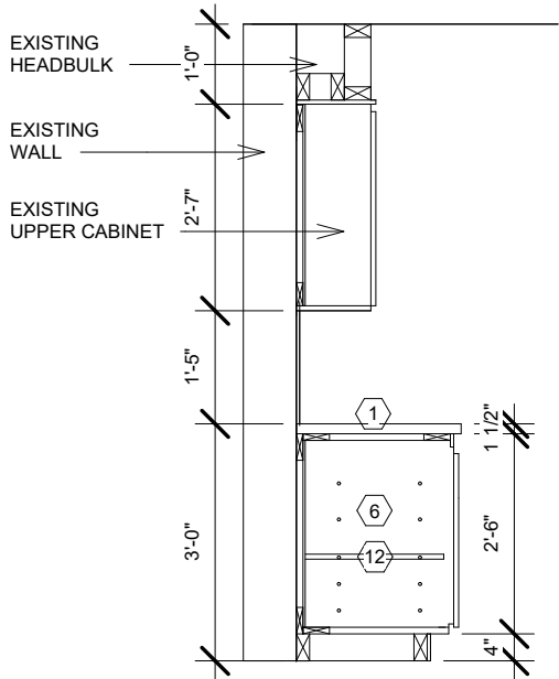
4 KITCHEN BASE CABINET SECTION VIEW 3/8" = 1'-0"
