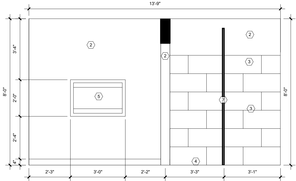
2 EAST WOMEN'S RESTROOM ELEVATION 3/8" = 1'-0"
