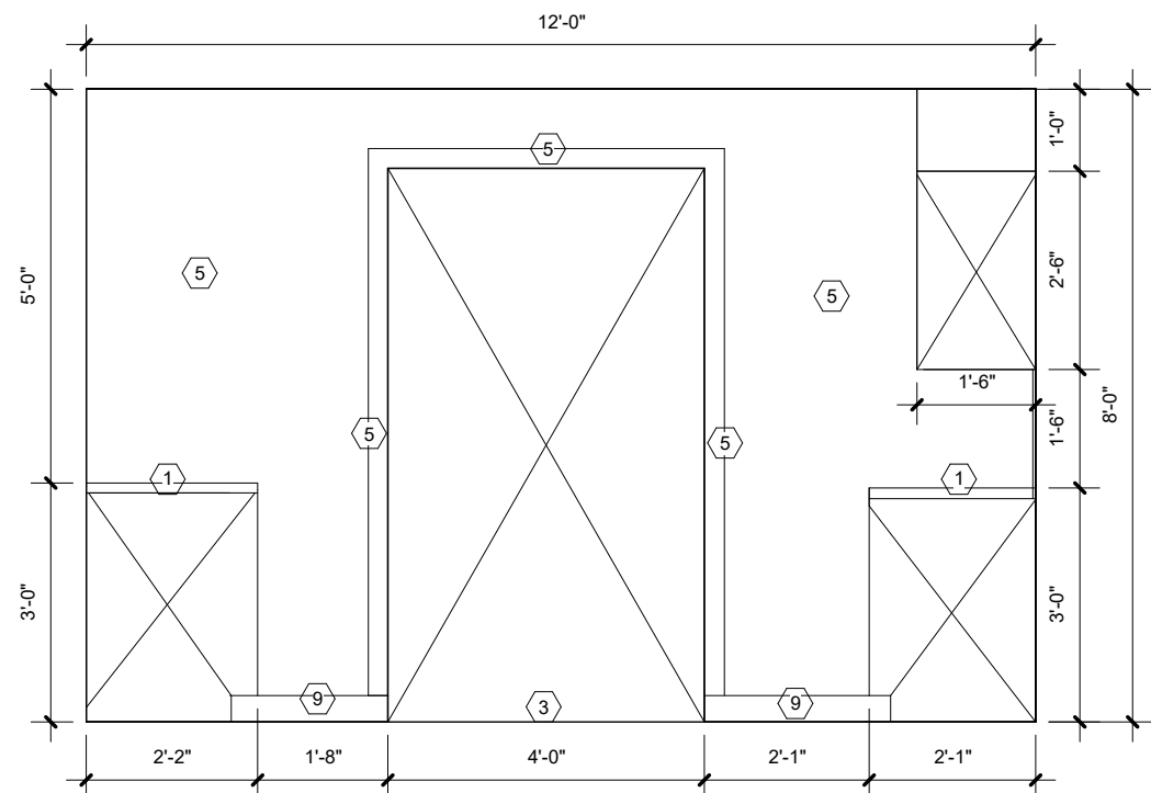
3 WEST KITCHEN ELEVATION 3/8" = 1'-0"
