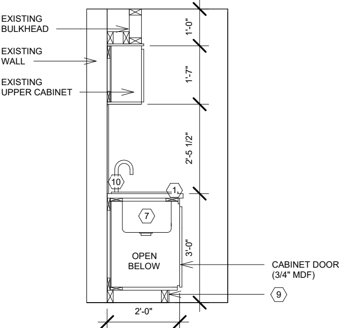
3 KITCHEN SINK SECTION VIEW 3/8" = 1'-0"
