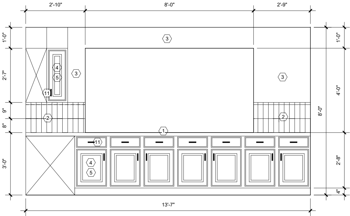
1 SOUTH KITCHEN ELEVATION 3/8" = 1'-0"
