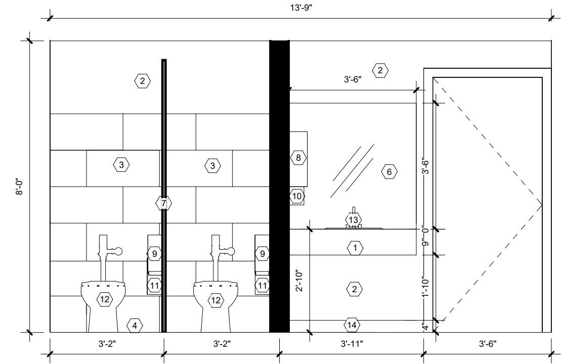
4 WEST WOMEN'S RESTROOM ELEVATION 3/8" = 1'-0"
