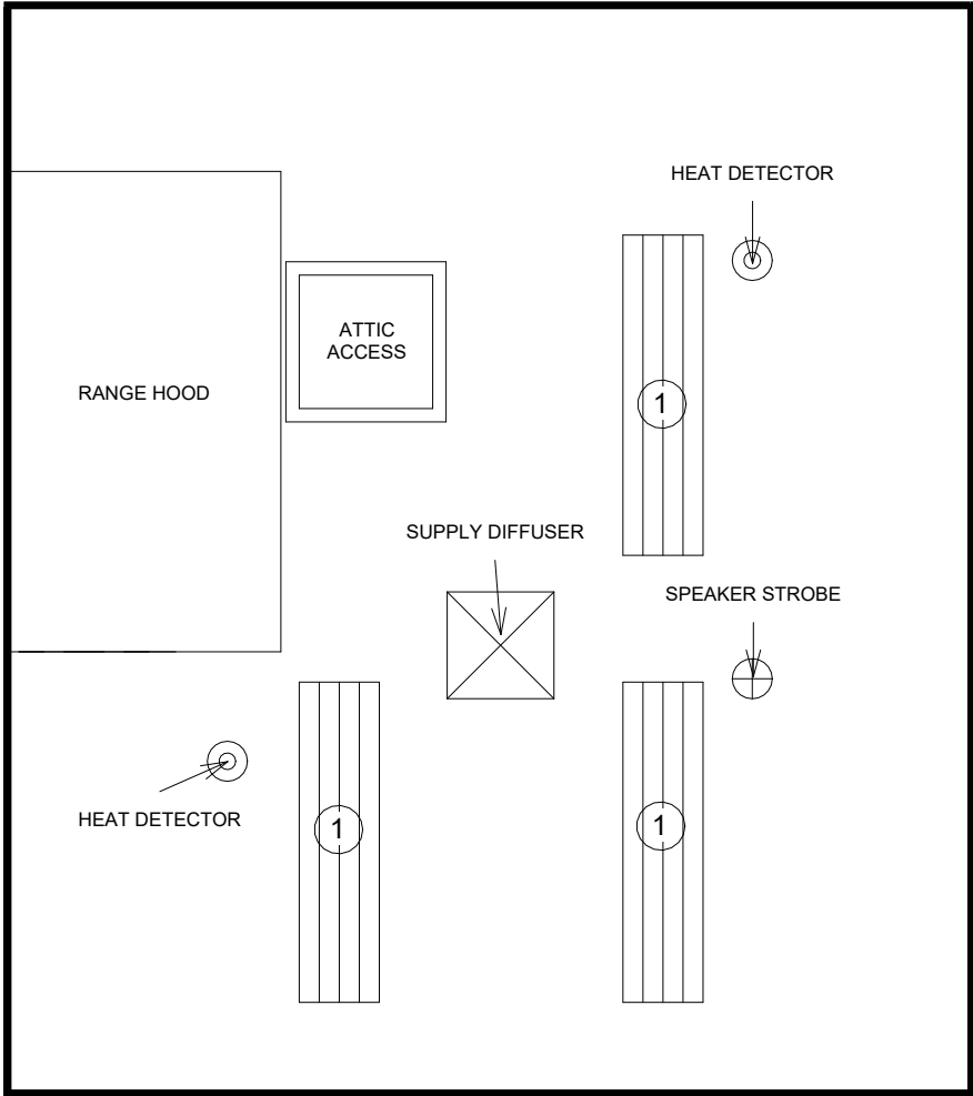
1 KITCHEN DEMOLITION RCP 3/8" = 1'-0"
