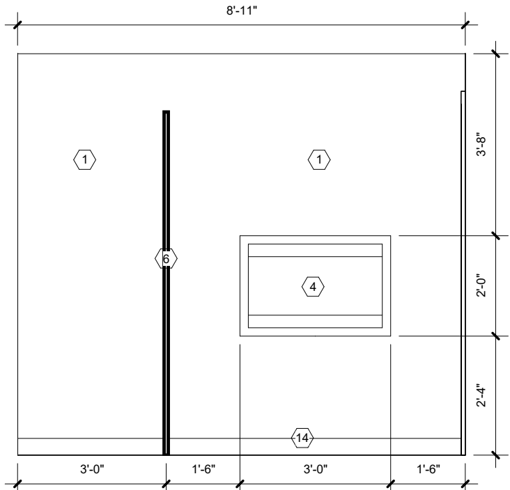
3 WEST MEN'S RESTROOM ELEVATION 3/8" = 1'-0"
