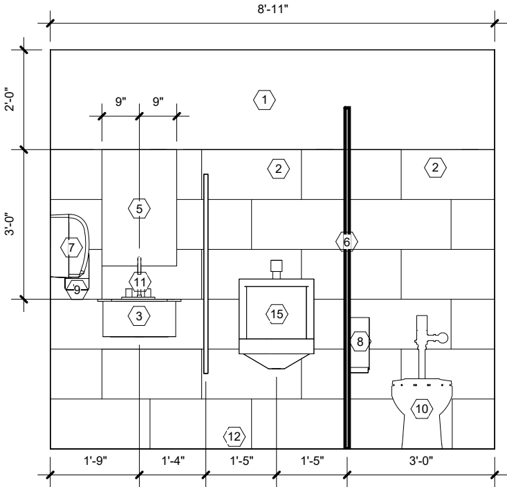
1 EAST MEN'S RESTROOM ELEVATION 3/8" = 1'-0"
