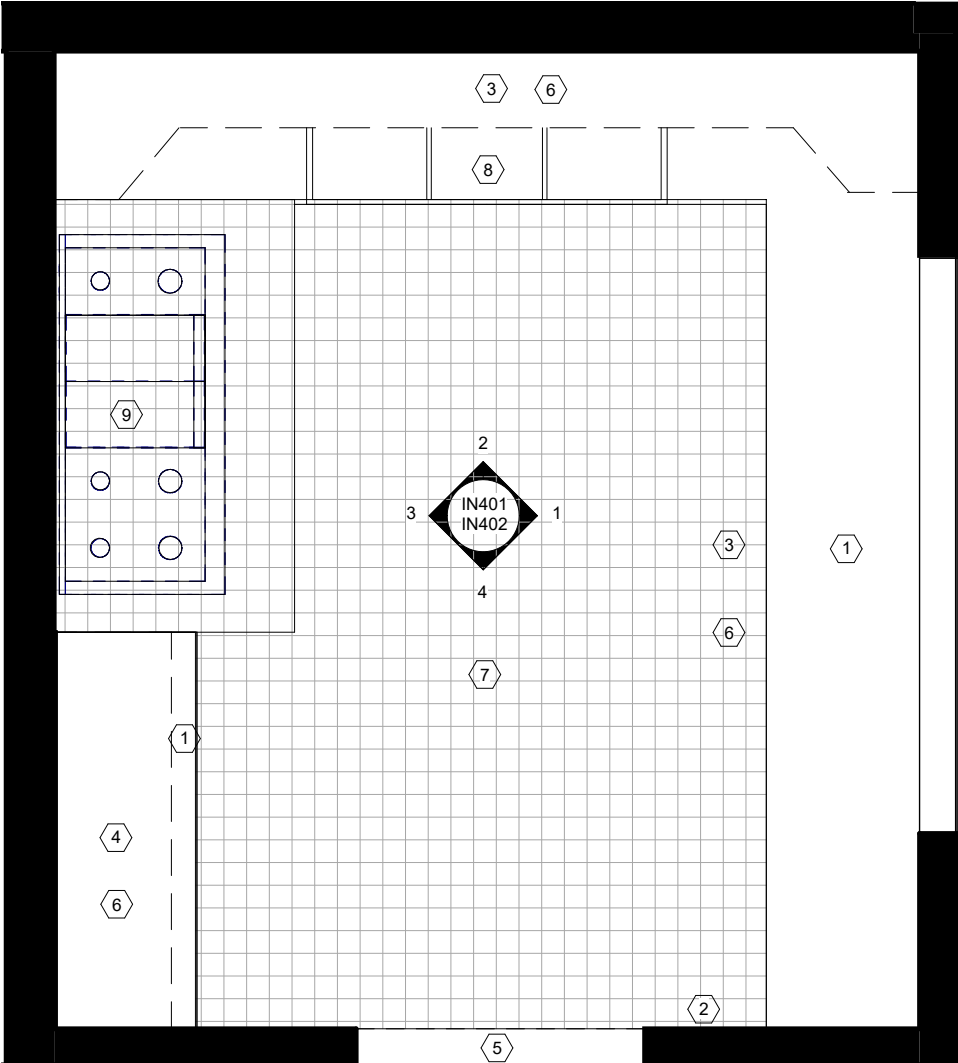
2 KITCHEN FINISH PLAN 3/8" = 1'-0"
