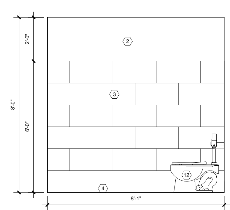
1 SOUTH WOMEN'S RESTROOM ELEVATION 3/8" = 1'-0"
