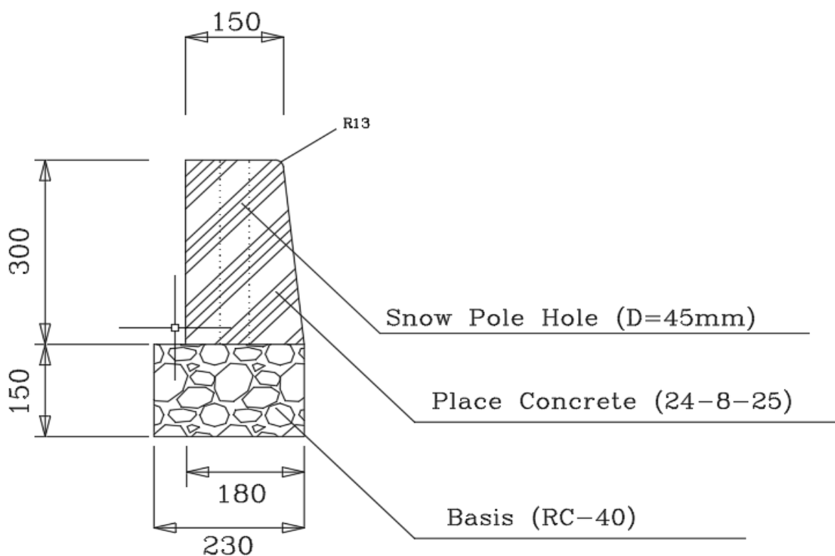
CAST-IN PLACE CONCRETE CURB 150 MM (BARRIER)
