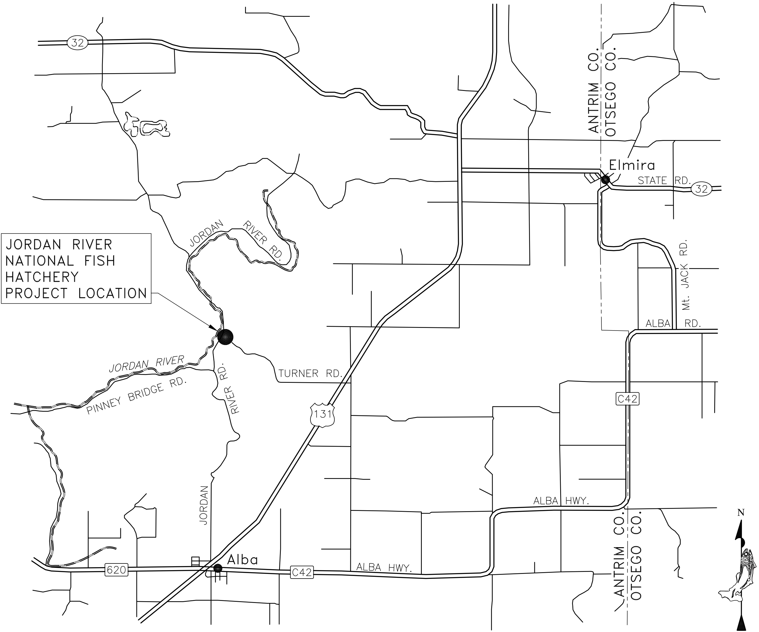
LOCATION MAP NO SCALE
