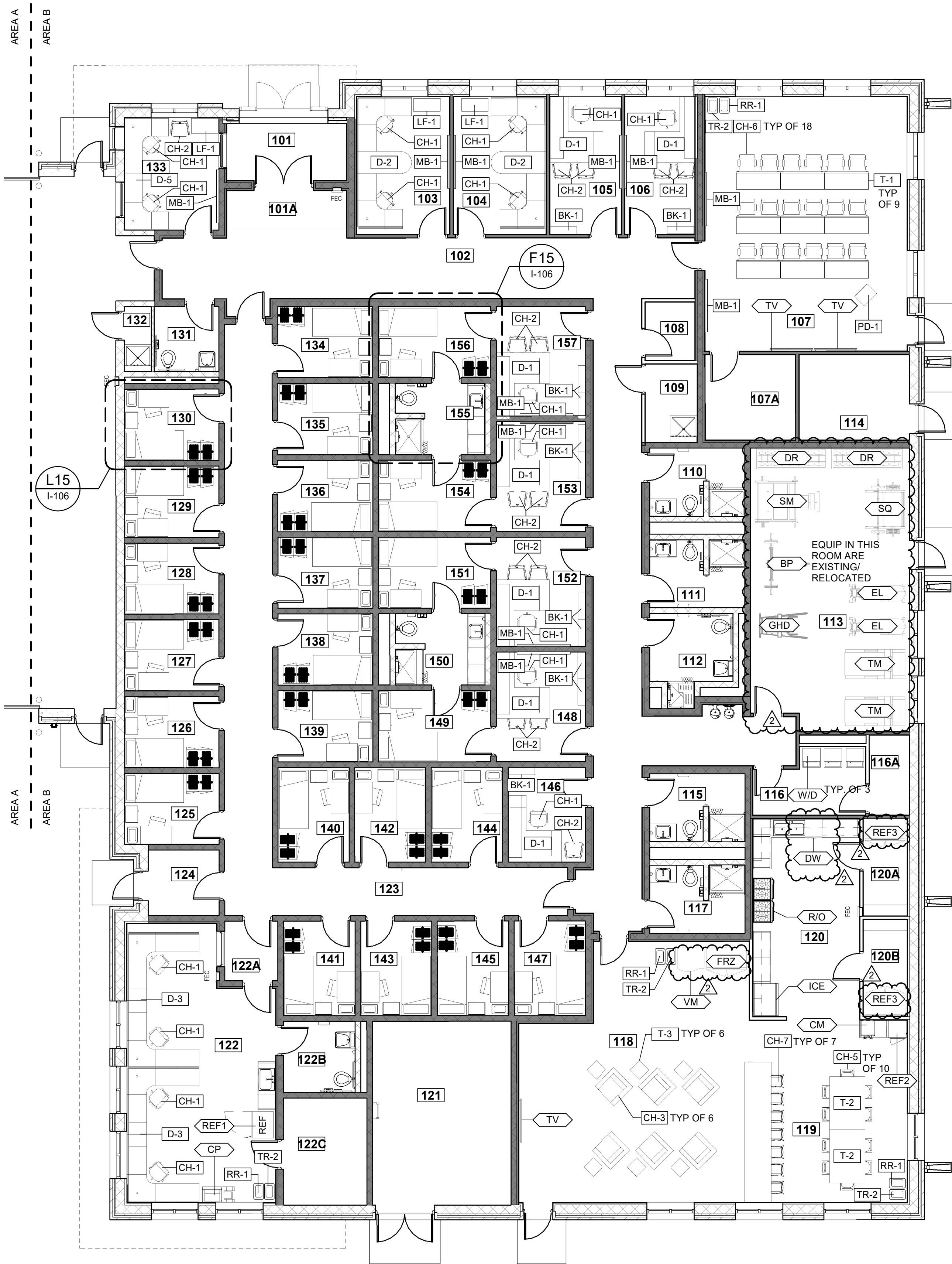
FURNITURE FLOOR PLAN - AREA B SCALE: 1/8" = 1'-0"
