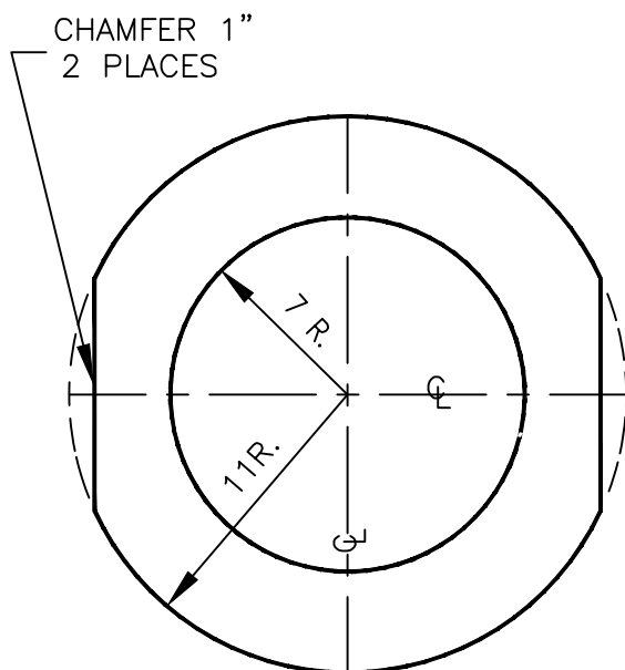
TOP PAD (CUT-OUT) ⑥
