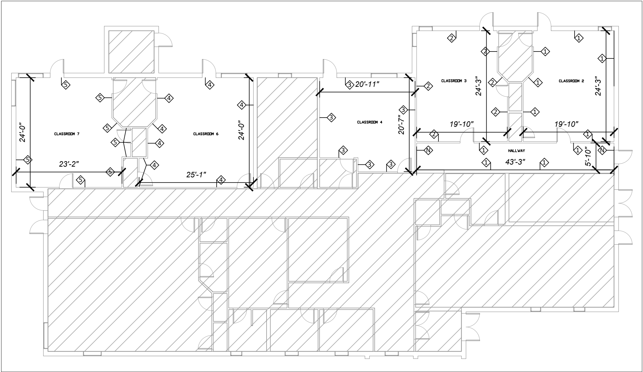
1 PHASING PLAN 5/64" = 1'-0"
