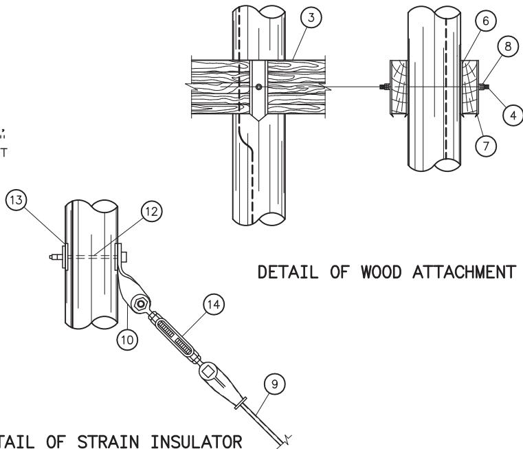
DETAIL OF STRAIN INSULATOR ATTACHMENT TO POLE
