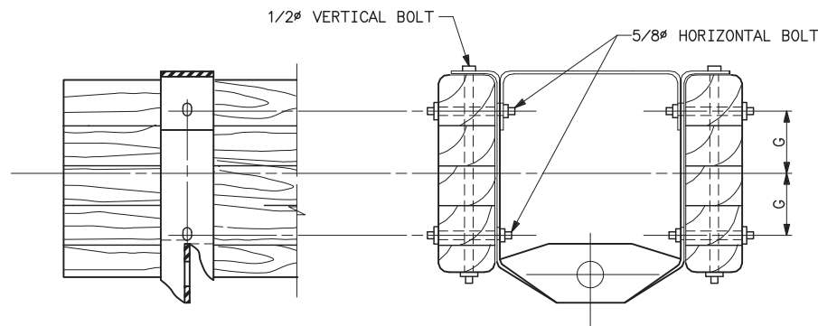
DETAIL OF FIXED SPACER FITTING (STANDARD DESIGN PART NO. 40.49-40.68)
