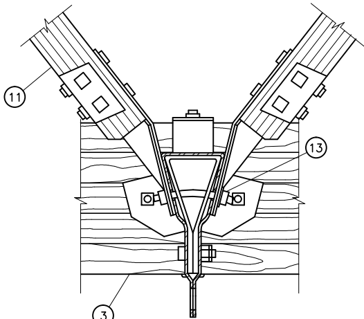
DETAIL OF CENTER PHASE FITTING ATTACHMENTS
