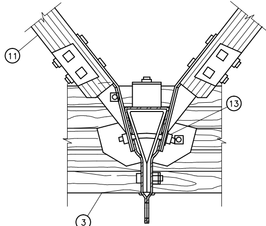
DETAIL OF CENTER PHASE FITTING ATTACHMENTS
