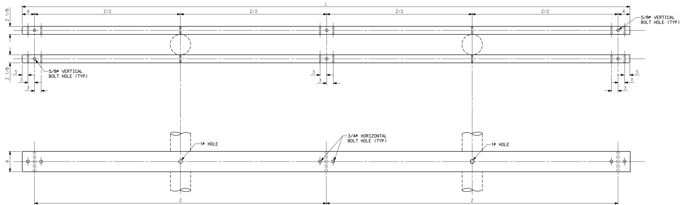
CROSSARM DRILLING DETAILS
