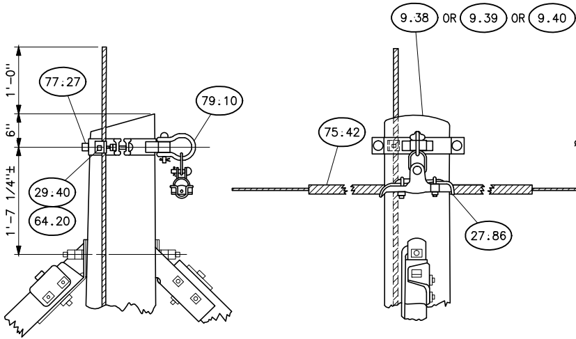
SUSPENSION
