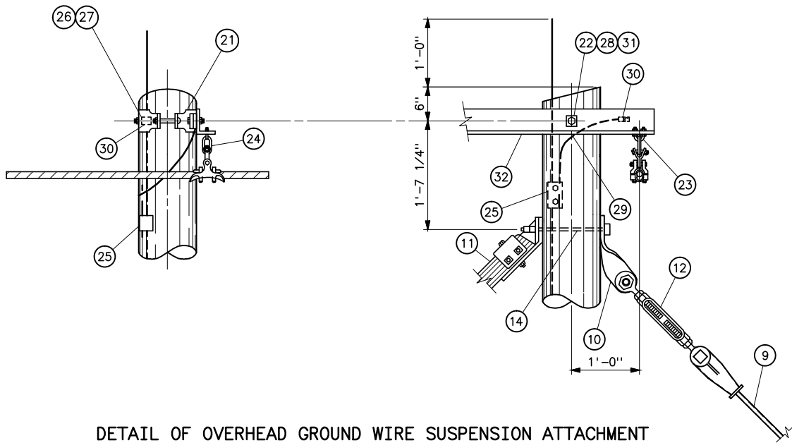
DETAIL OF OVERHEAD GROUND WIRE SUSPENSION ATTACHMENT AND BRACE ATTACHMENTS TO POLE
