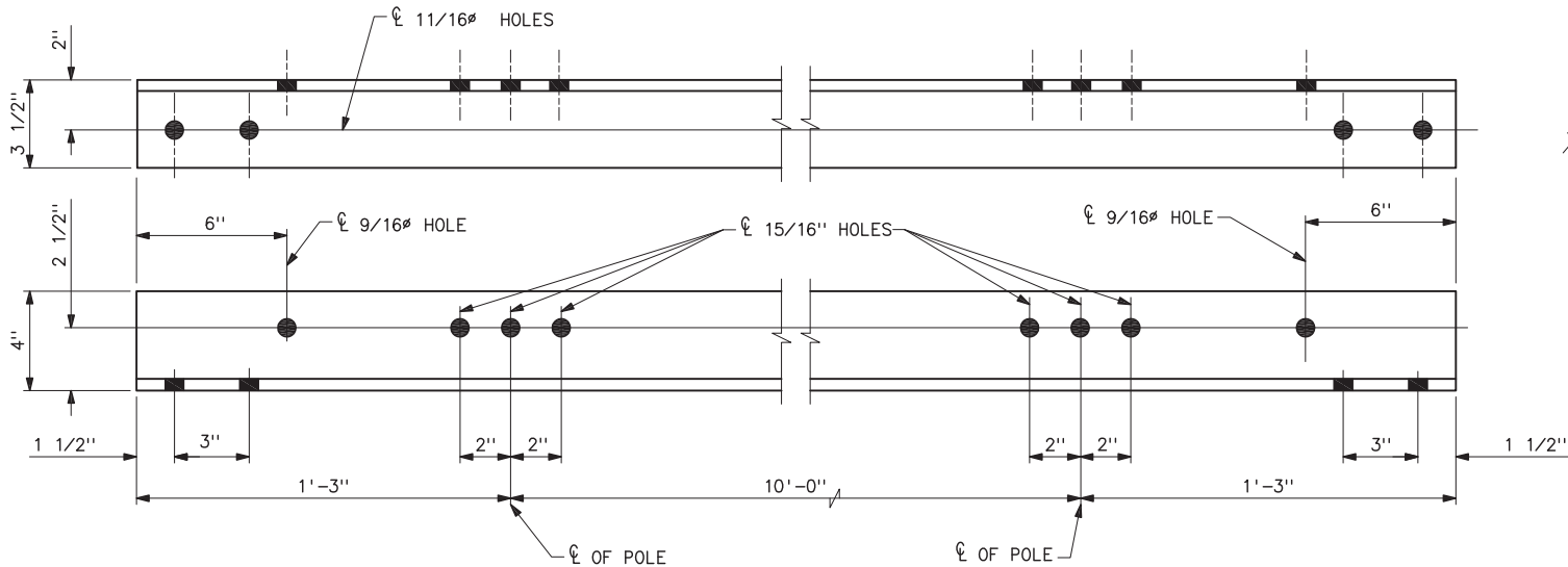
STEEL ANGLE (32)
