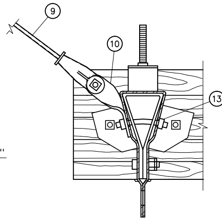
DETAIL OF END PHASE FITTING ASSEMBLY
