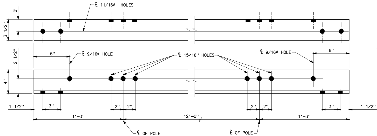
STEEL ANGLE (32)
