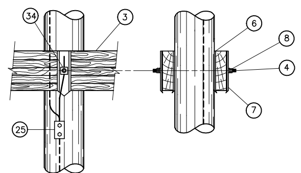
DETAIL OF WOOD CROSSARM ATTACHMENT TO POLE
