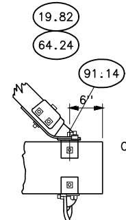
DETAIL OF PHASE FITTING ASSEMBLY
