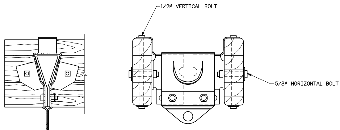
DETAIL OF ADJUSTABLE SPACER FITTING
