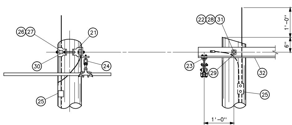
DETAIL OF OVERHEAD GROUND WIRE SUSPENSION ATTACHMENT
