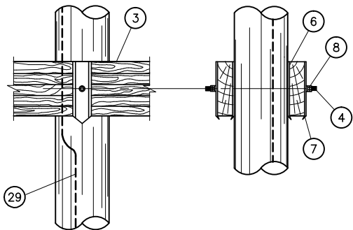
DETAIL OF WOOD ATTACHMENT
