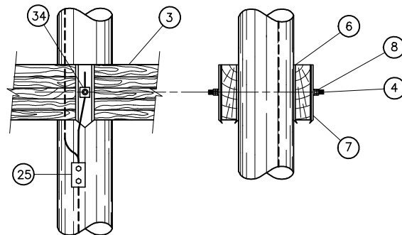
DETAIL OF WOOD CROSSARM ATTACHMENT TO POLE
