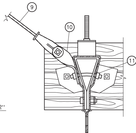
DETAIL OF PHASE FITTING ASSEMBLY
