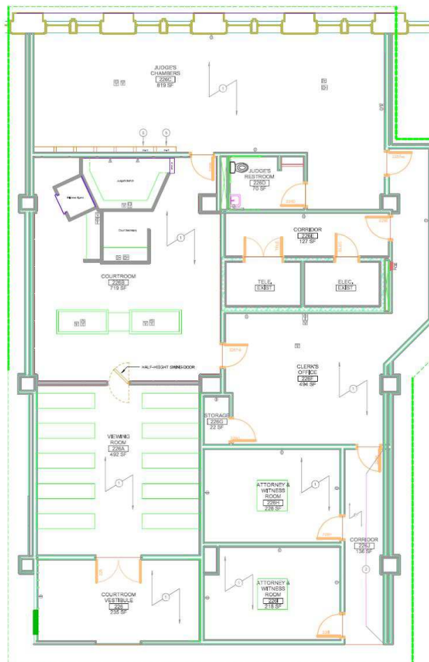
COURTROOM - FLOOR PLAN
