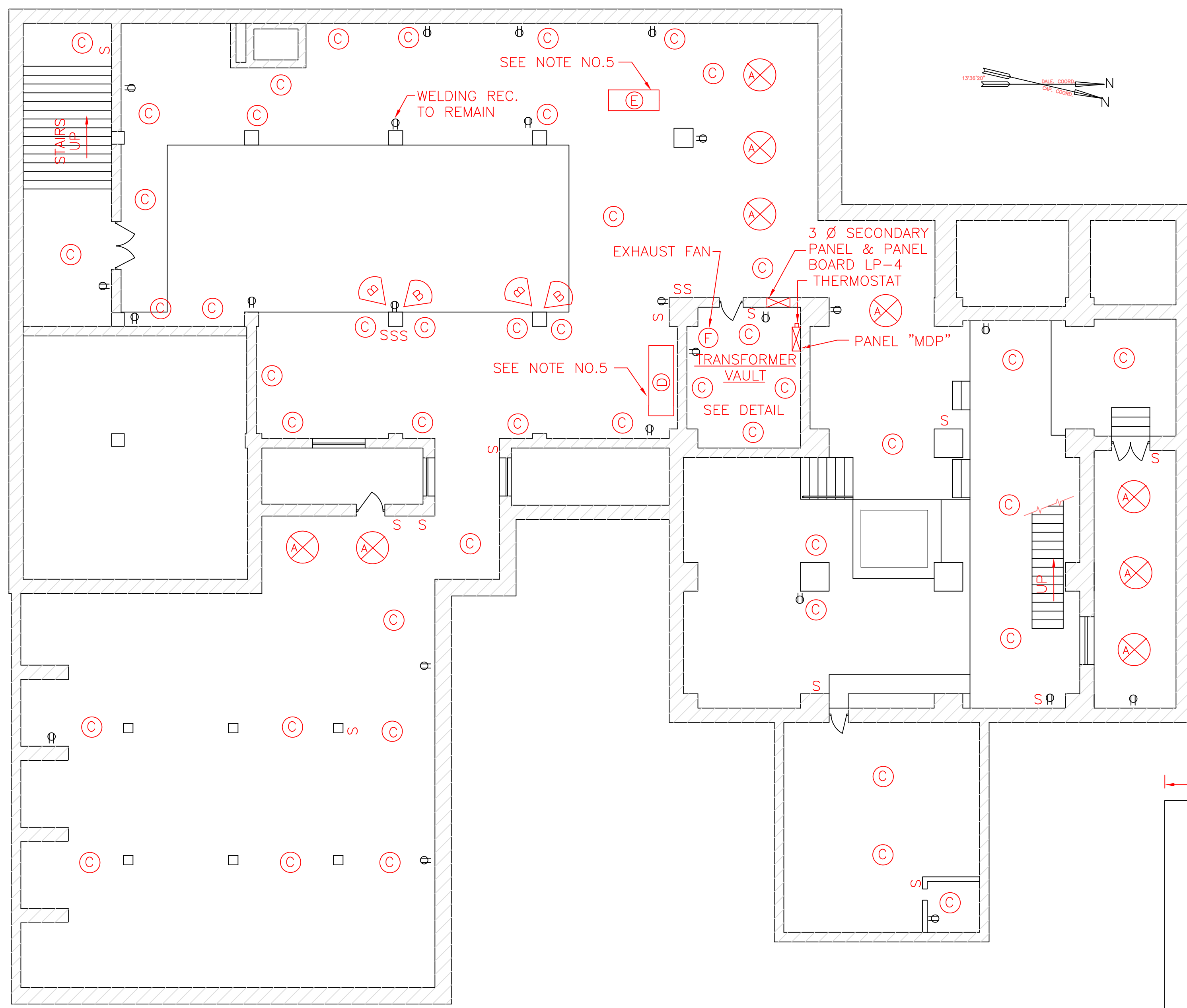
DEMOLITION/REMOVAL BASEMENT PLAN SCALE: 1/8" = 1'-0"
