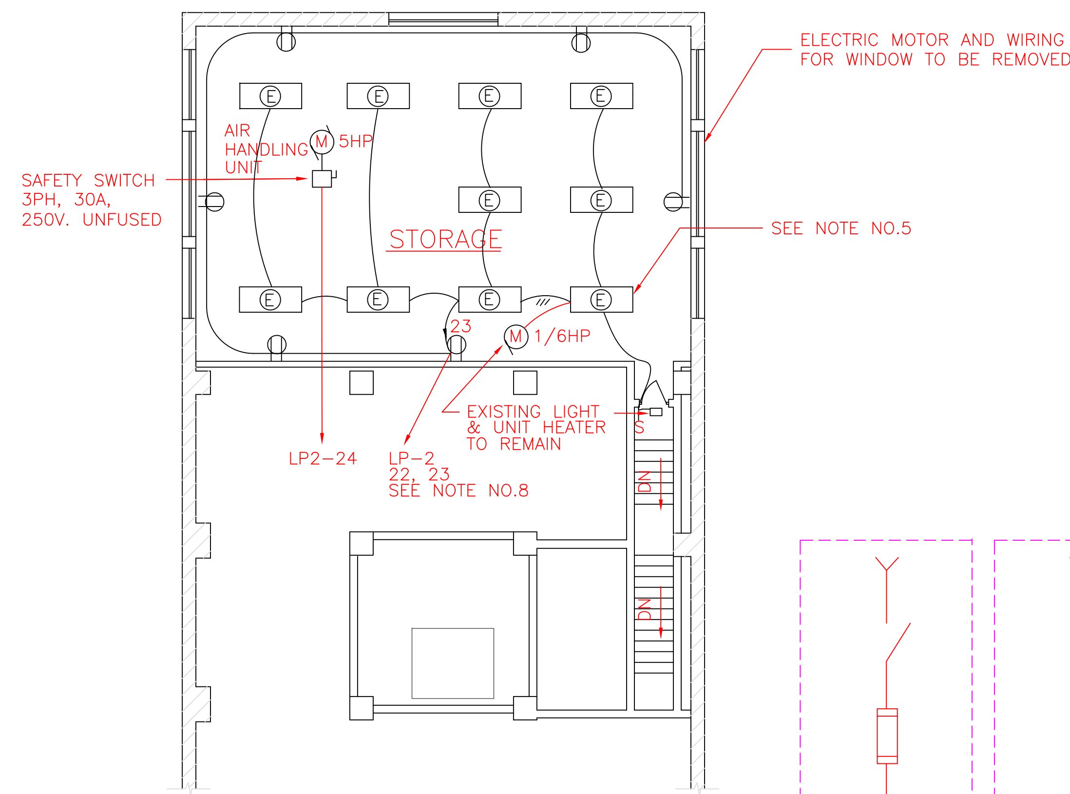
DEMOLITION/REMOVAL THIRD FLOOR PLAN SCALE: 1/8" = 1'-0"
