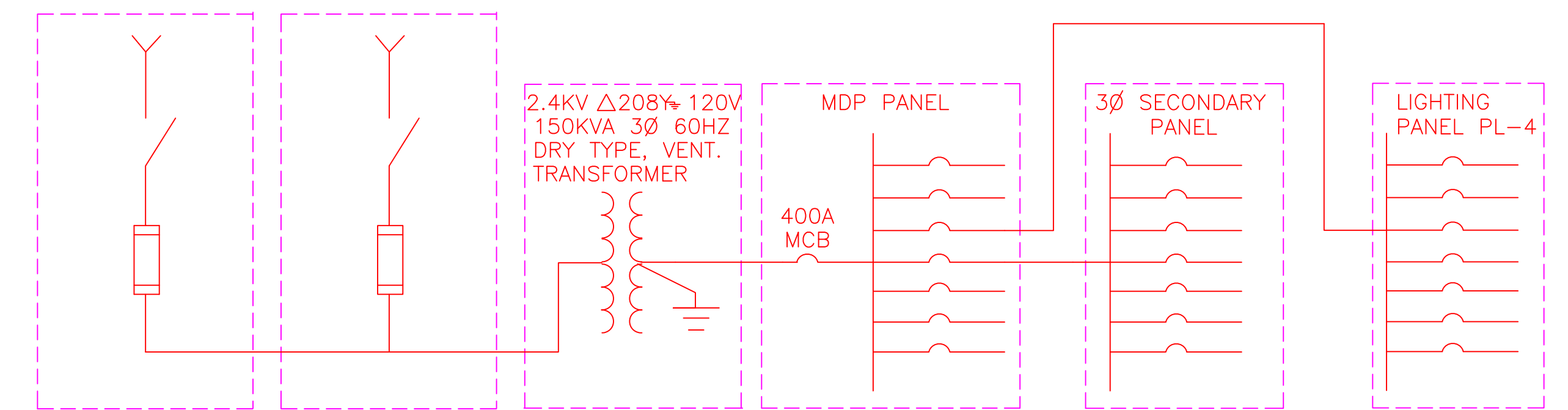
ONE-LINE DIAGRAM
