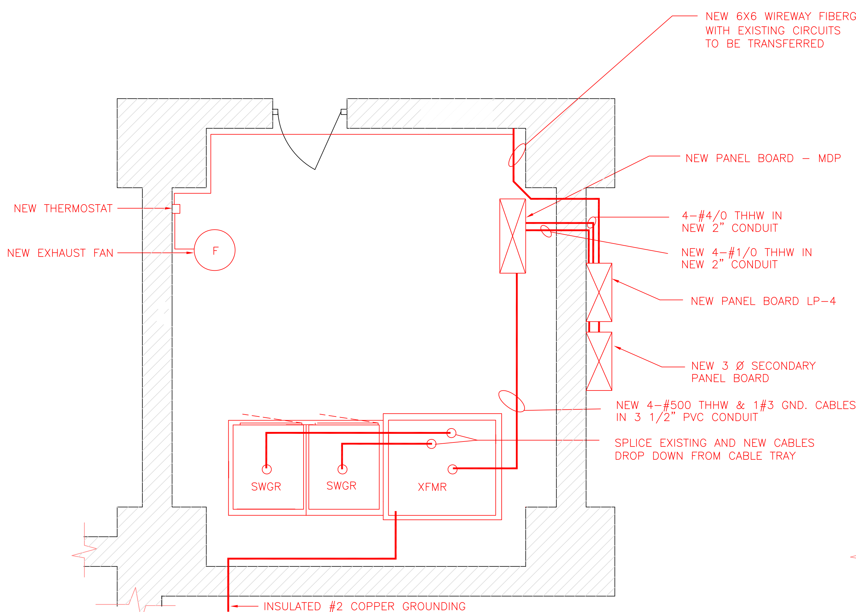
NEW TRANSFORMER AND DISCONNECT SWITCH DETAIL N. T. S. SK-4
