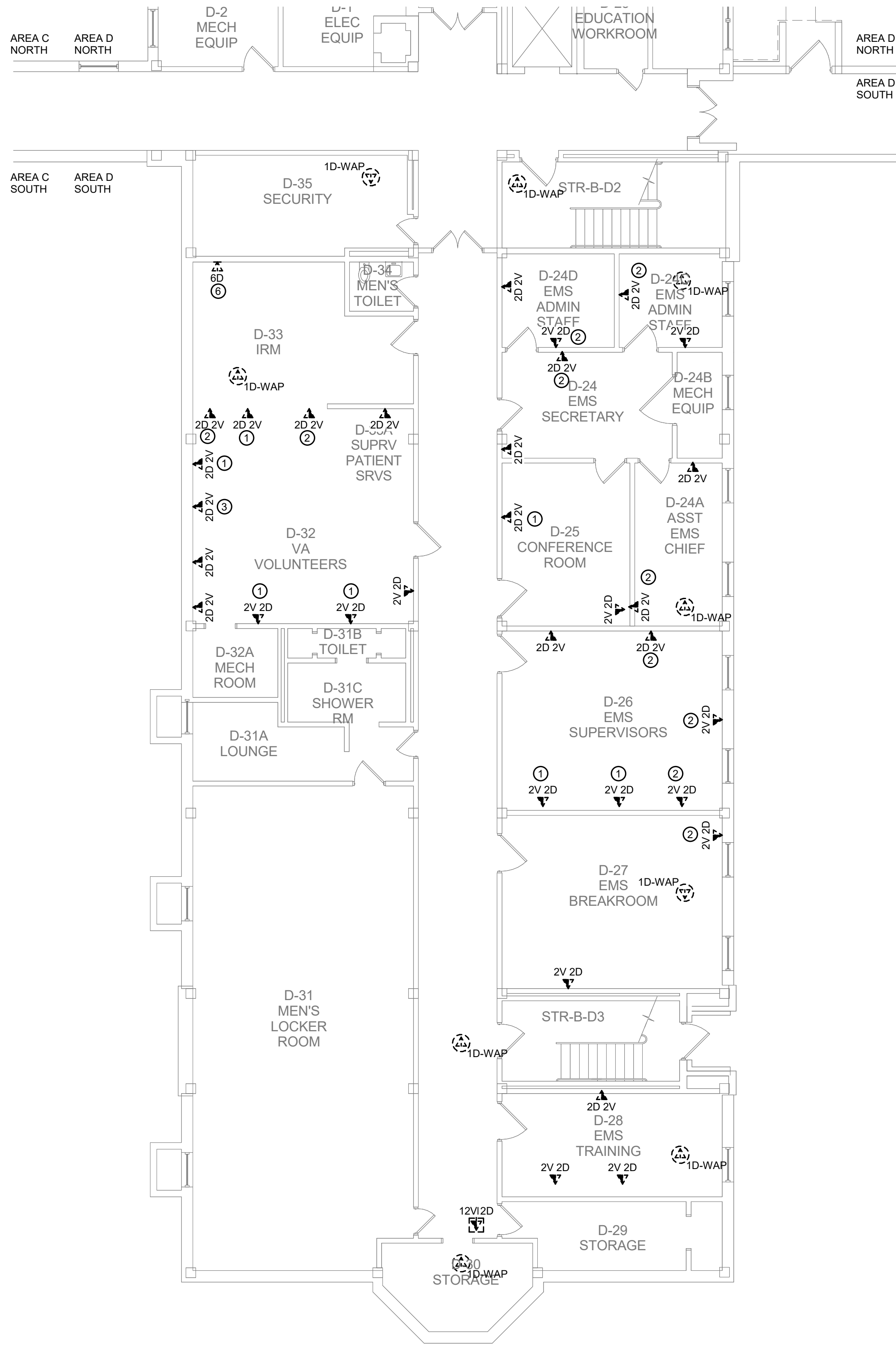
1 BUILDING 70 BASEMENT DEMOLITION PLAN - TECHNOLOGY - AREA D SOUTH 1/8" = 1'-0"
