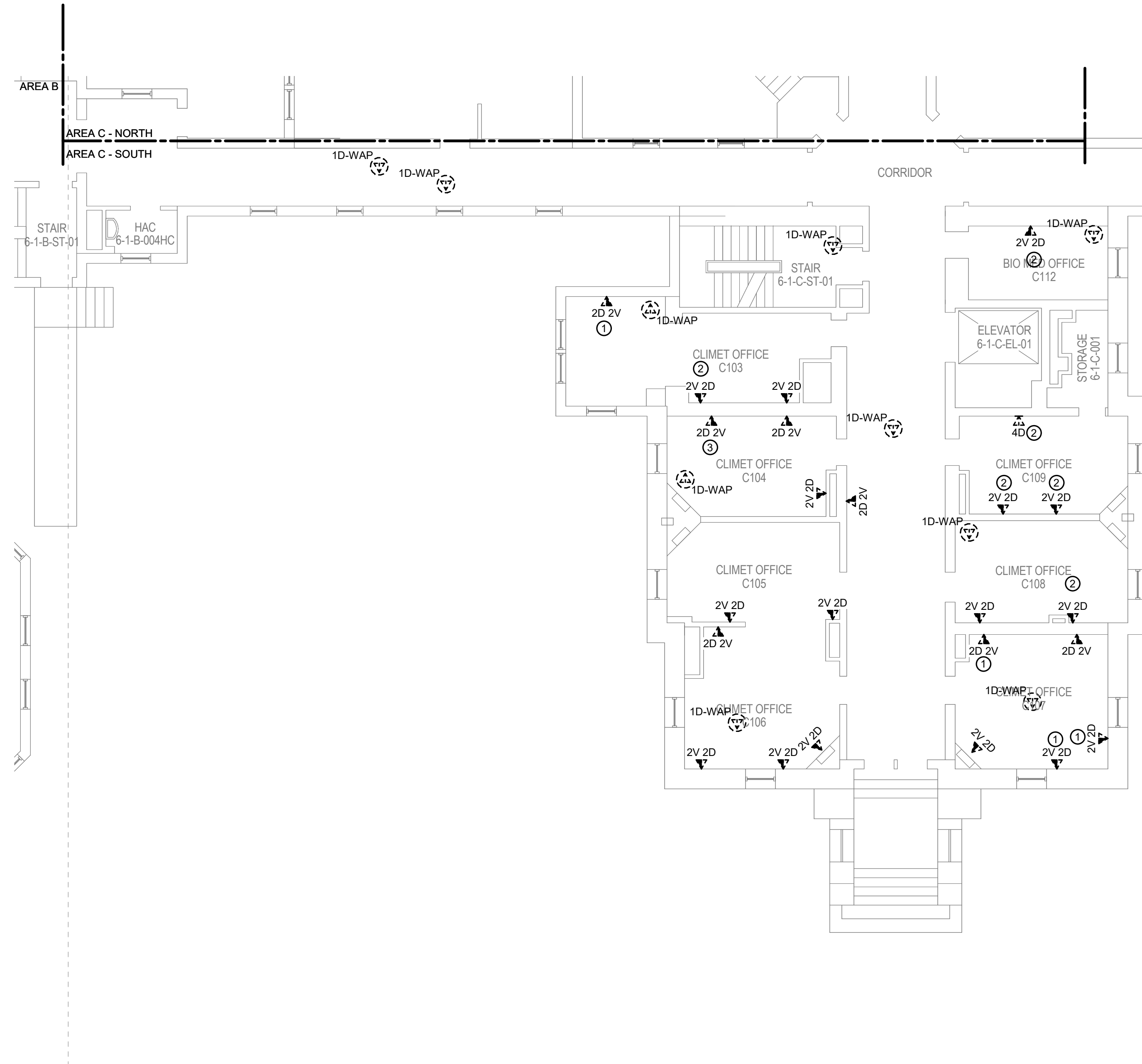
2 BUILDING 06 FIRST FLOOR DEMOLITION PLAN - TECHNOLOGY - AREA C SOUTH 1/8" = 1'-0"
