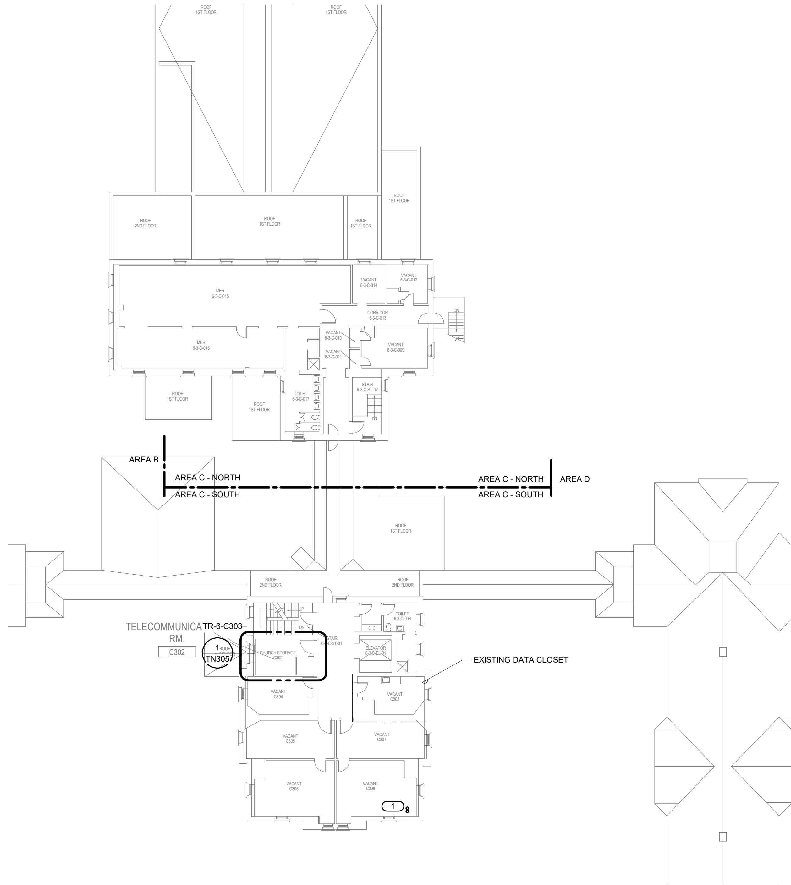
1 BUILDING 06 THIRD FLOOR OVERALL PLAN - TECHNOLOGY 1/16" = 1'-0"
