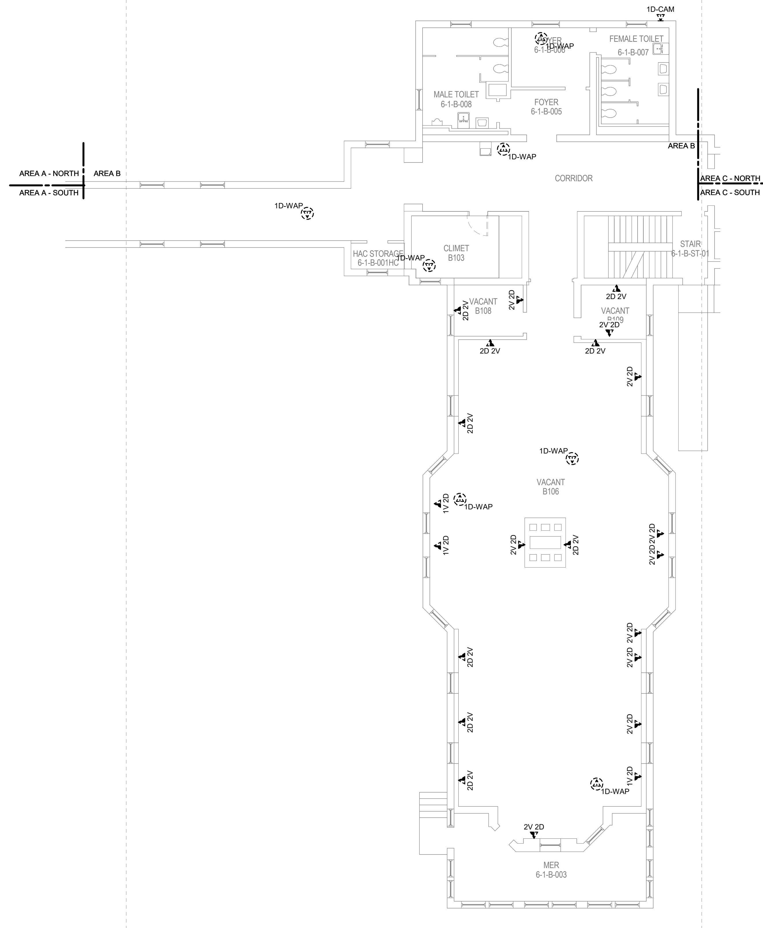
1 BUILDING 06 FIRST FLOOR DEMOLITION PLAN - TECHNOLOGY - AREA B 1/8" = 1'-0"
