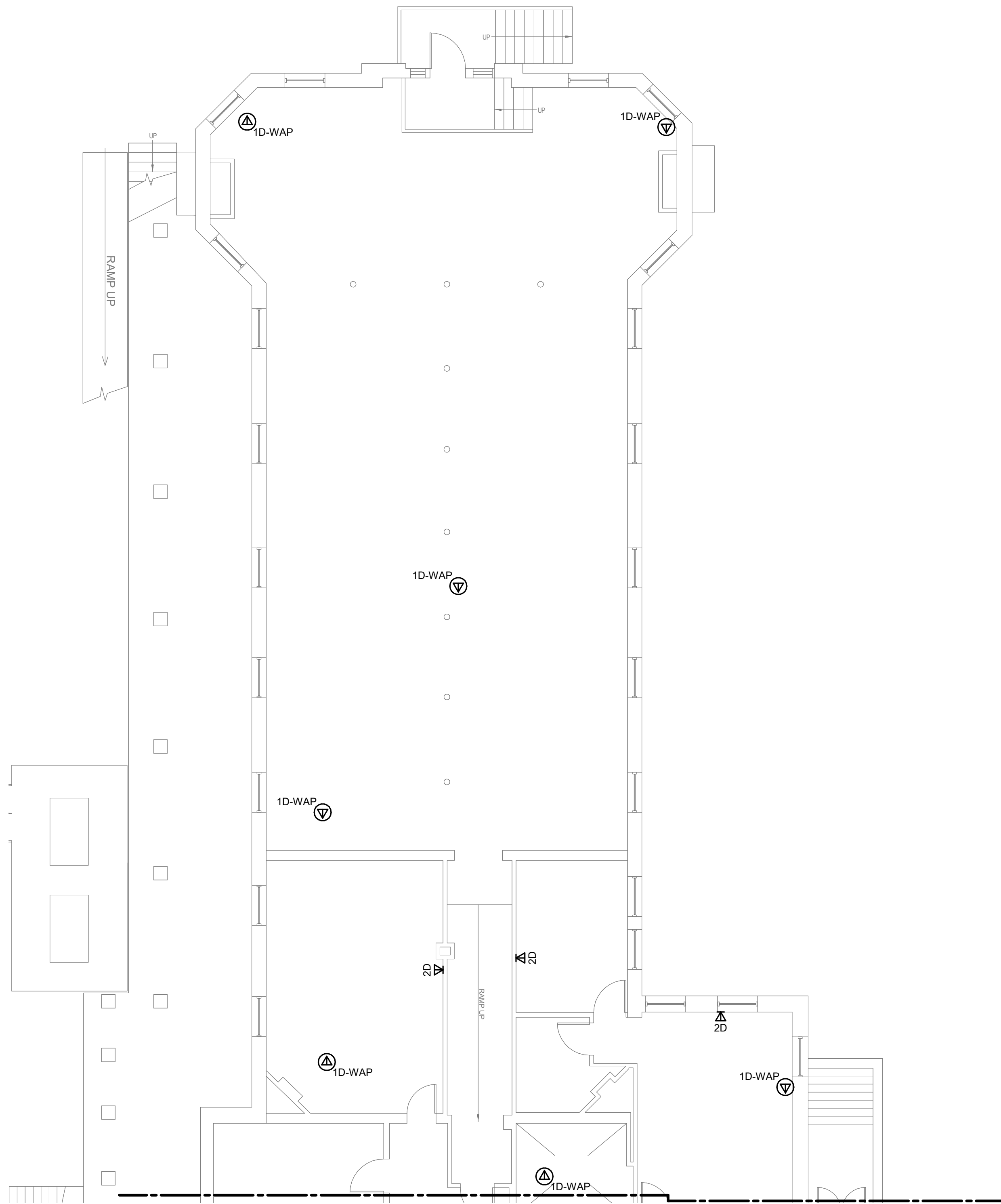
1 BUILDING 06 BASEMENT FLOOR PLAN - AREA A NORTH 1/8" = 1'-0"
