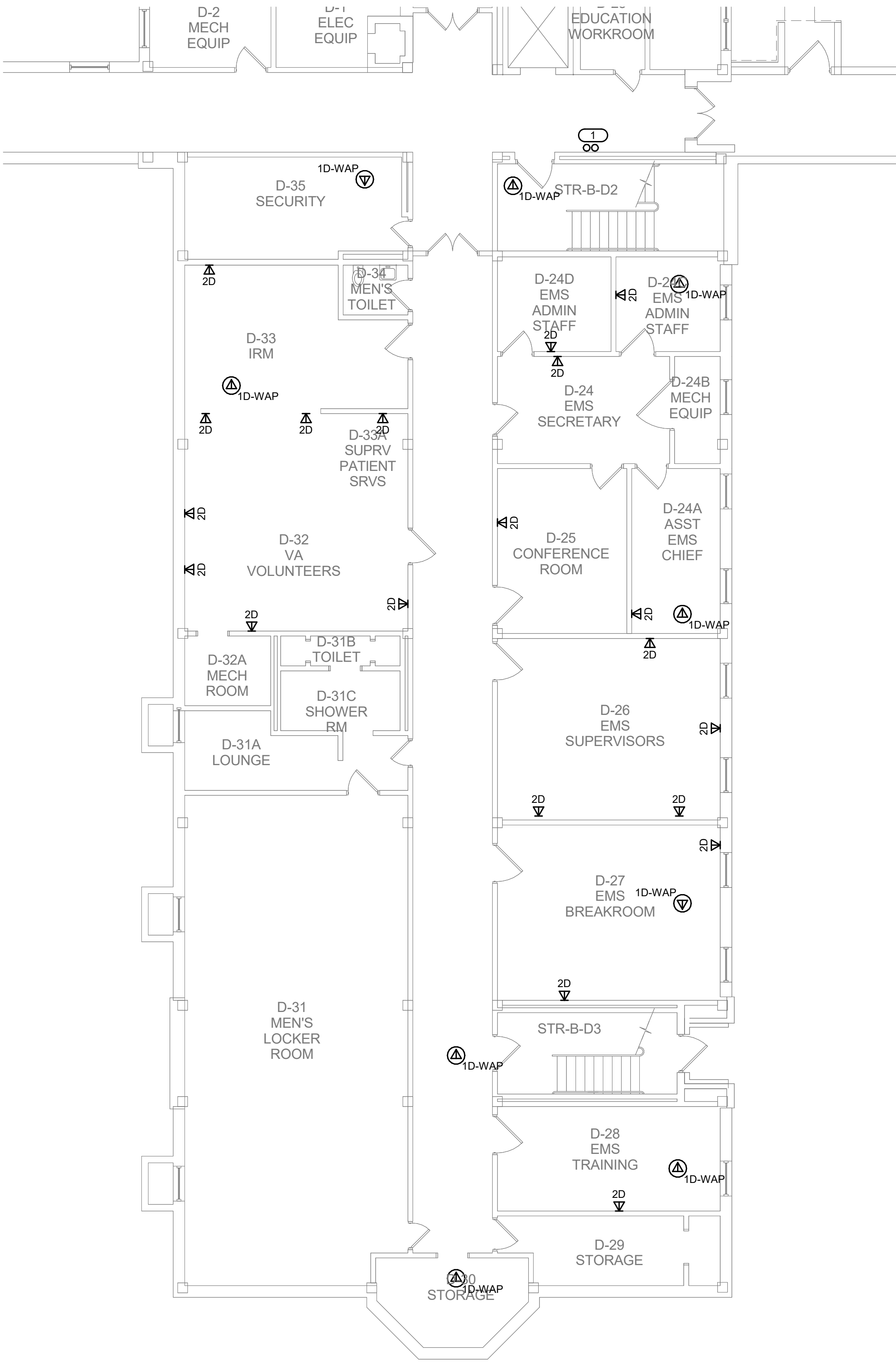
1 BUILDING 70 BASEMENT PLAN - TECHNOLOGY - AREA D SOUTH 1/8" = 1'-0"
