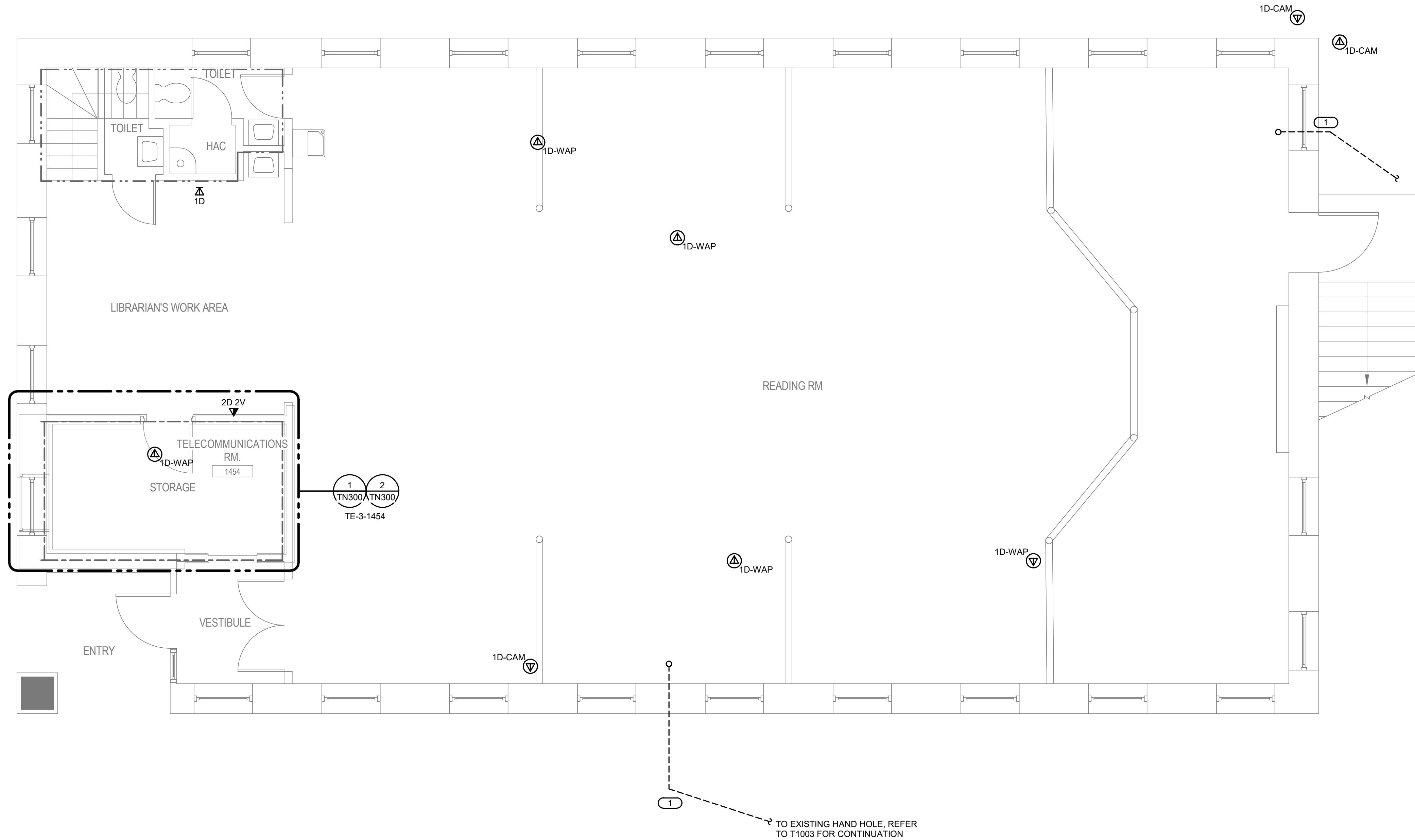
1 BUILDING 03 FIRST FLOOR PLAN - TECHNOLOGY 1/4" = 1'-0"
