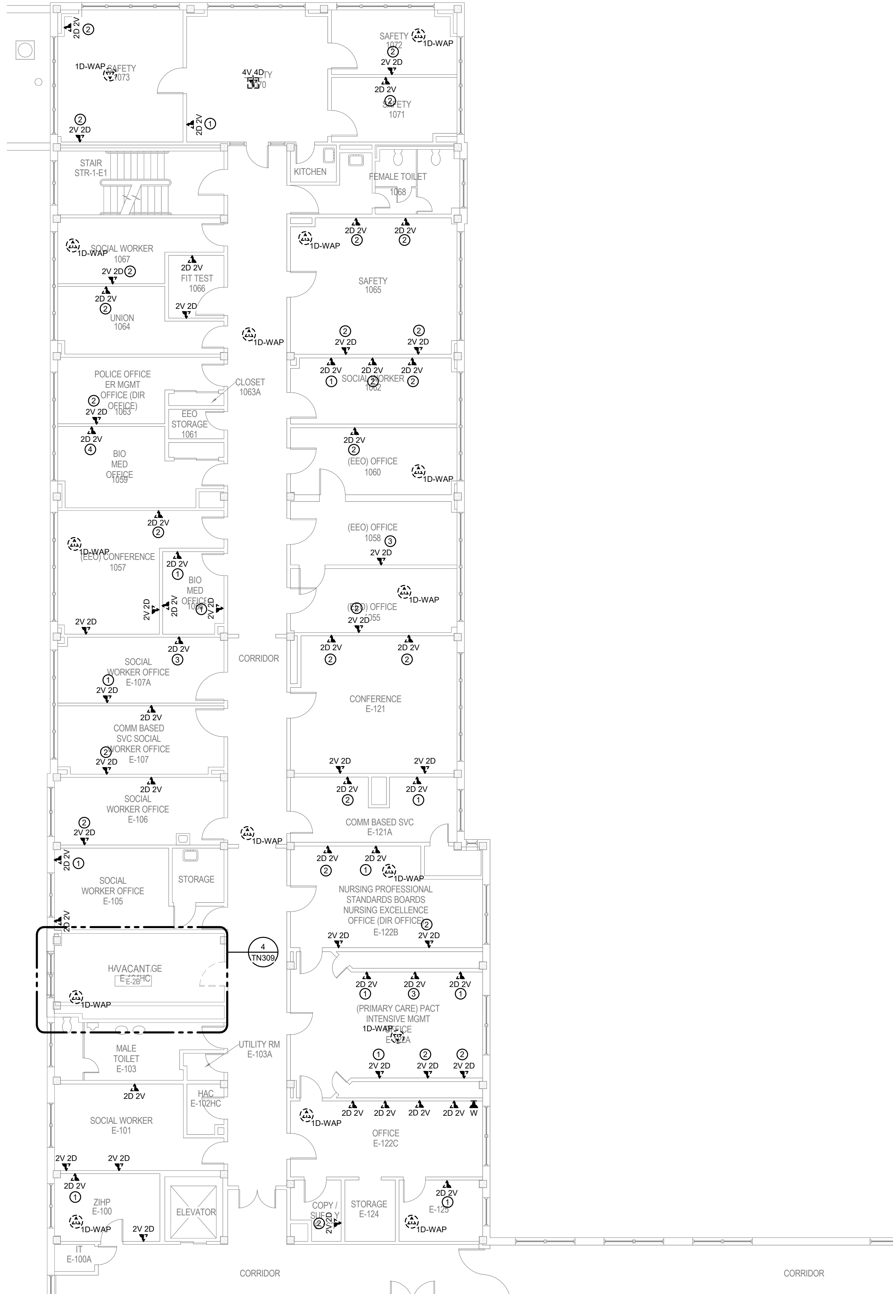
1 BUILDING 70 FIRST FLOOR DEMOLITION PLAN - TECHNOLOGY - AREA E NORTH 1/8" = 1'-0"
