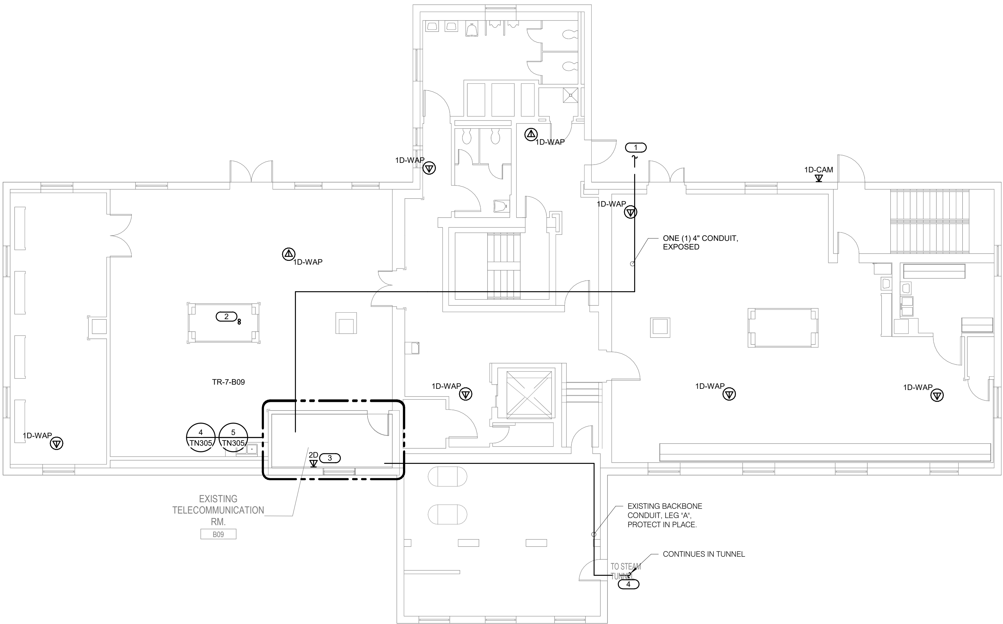
1 BUILDING 07 BASEMENT PLAN - TECHNOLOGY 1/8" = 1'-0"
