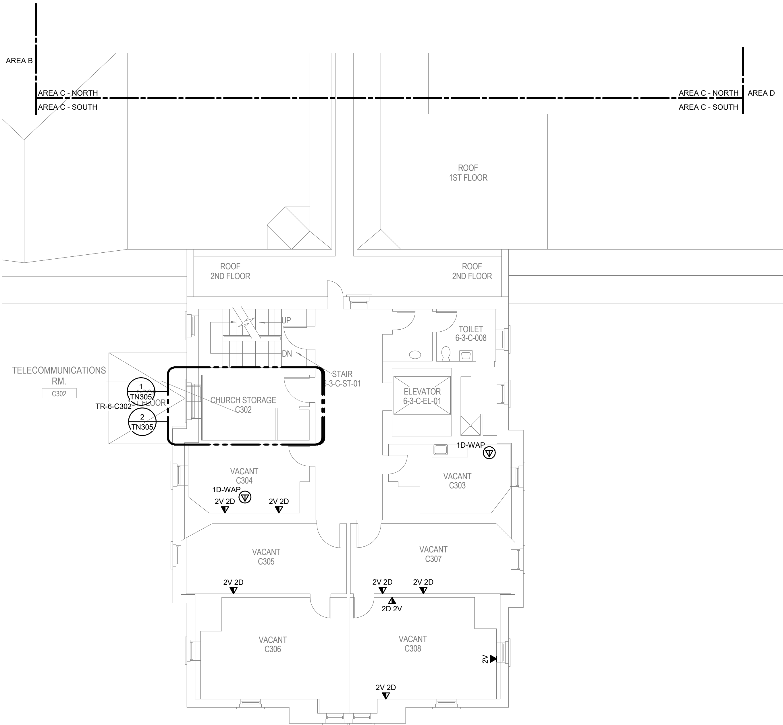
1 BUILDING 06 THIRD FLOOR PLAN - TECHNOLOGY - AREA C NORTH 1/8" = 1'-0"
