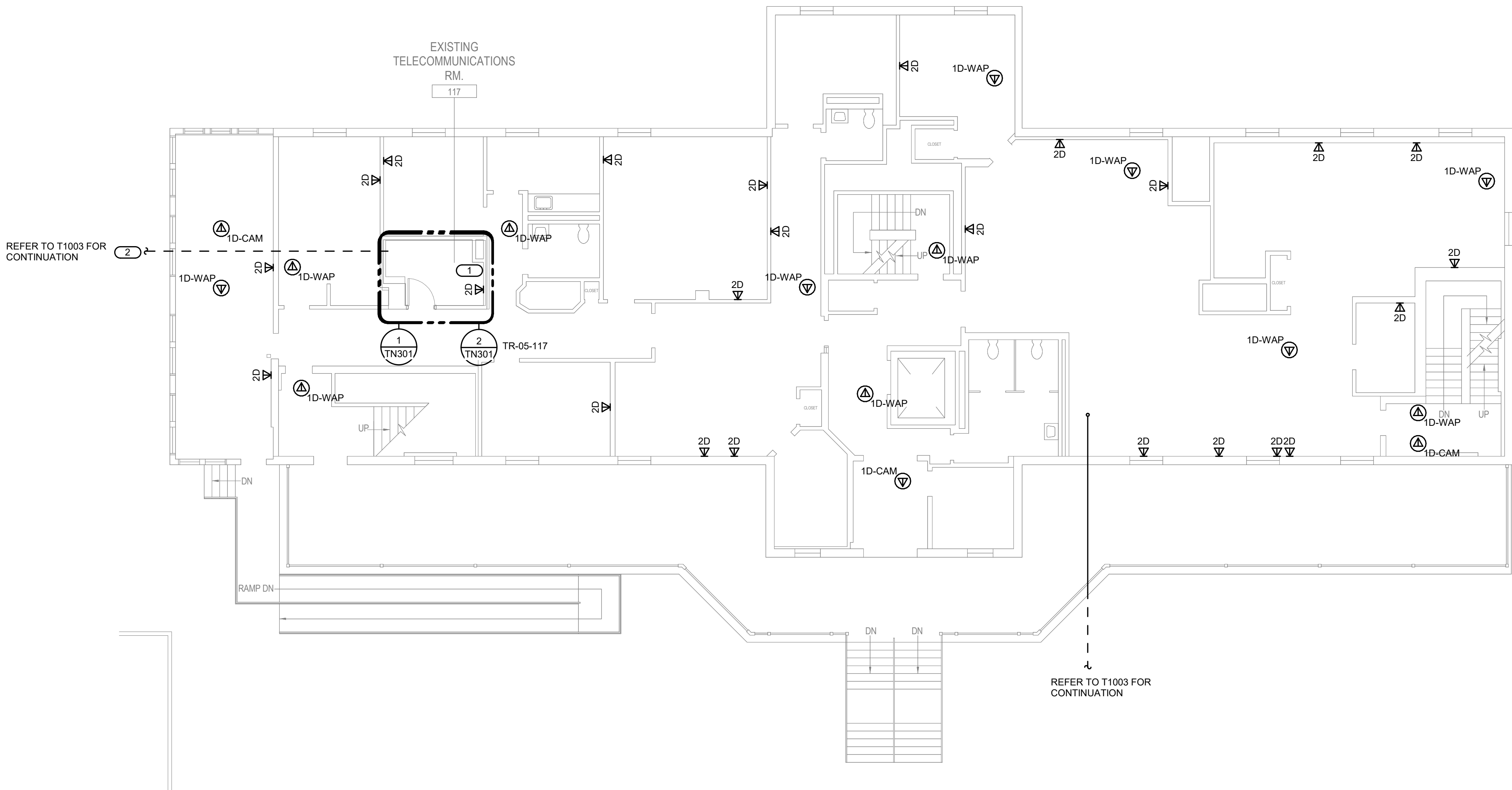
1 BUILDING 05 FIRST FLOOR PLAN - TECHNOLOGY 1/8" = 1'-0"
