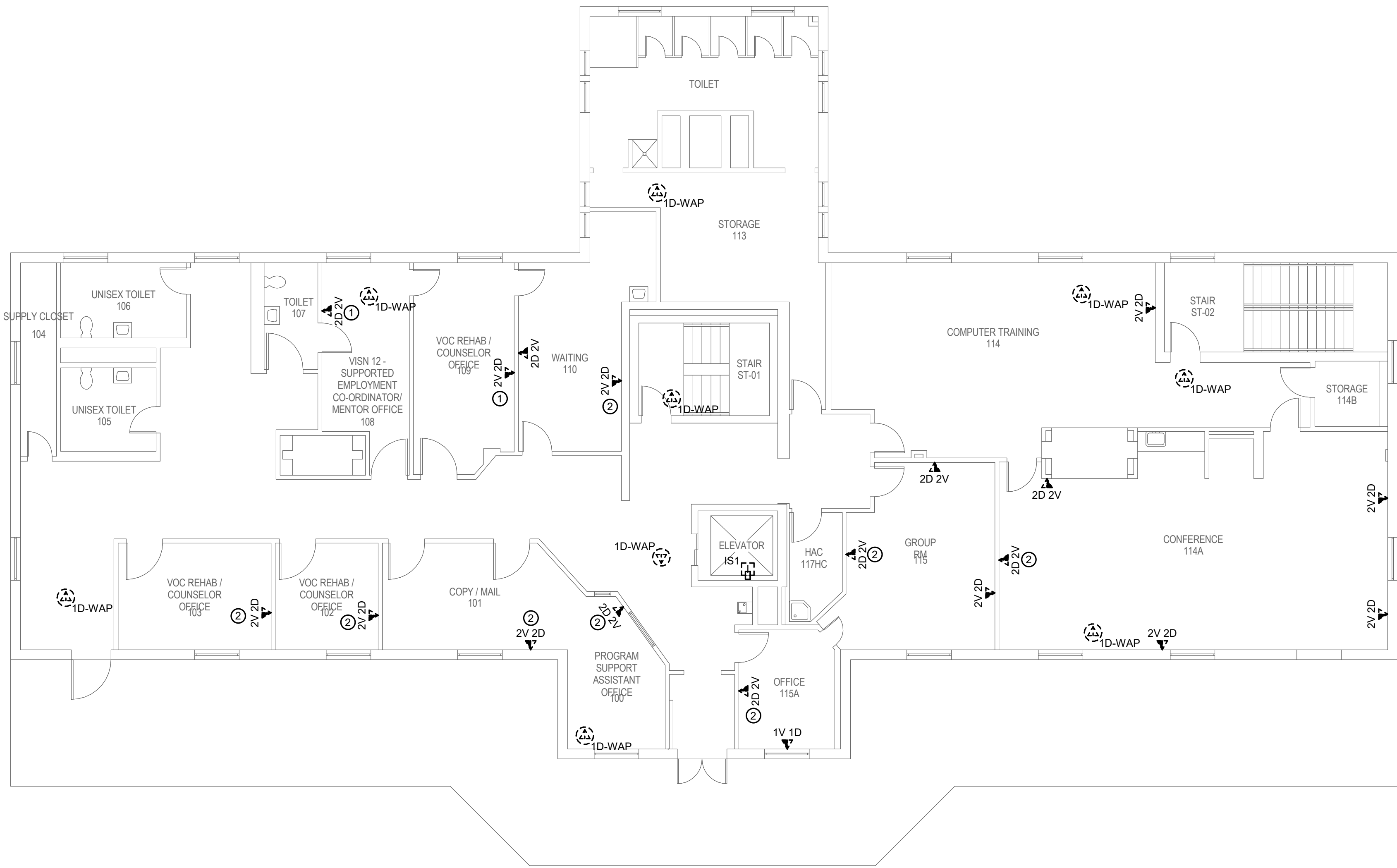
1 BUILDING 07 FIRST FLOOR DEMOLITION PLAN - TECHNOLOGY 1/8" = 1'-0"
