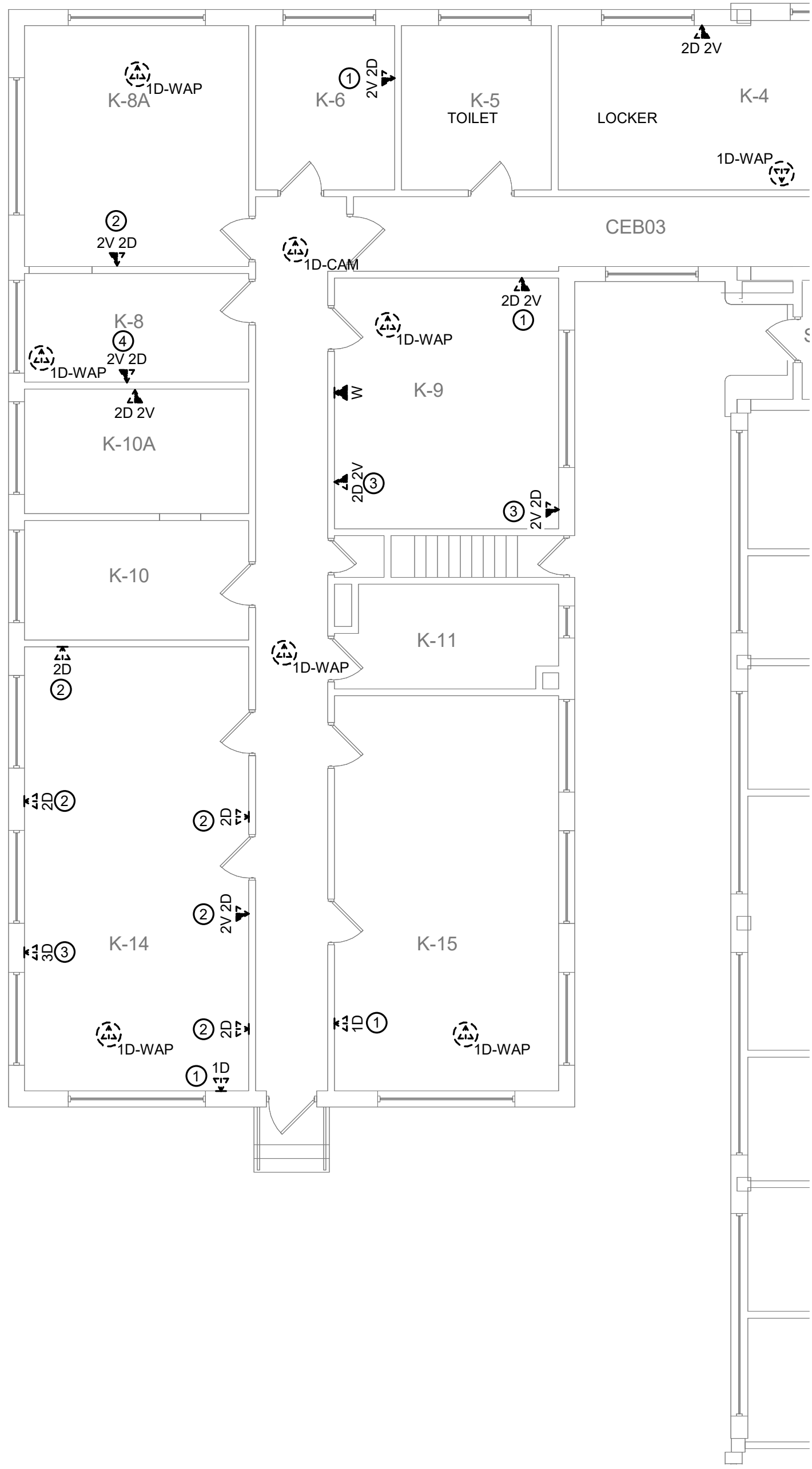
1 BUILDING 70 BASEMENT DEMOLITION PLAN - TECHNOLOGY - AREA K 1/8" = 1'-0"
