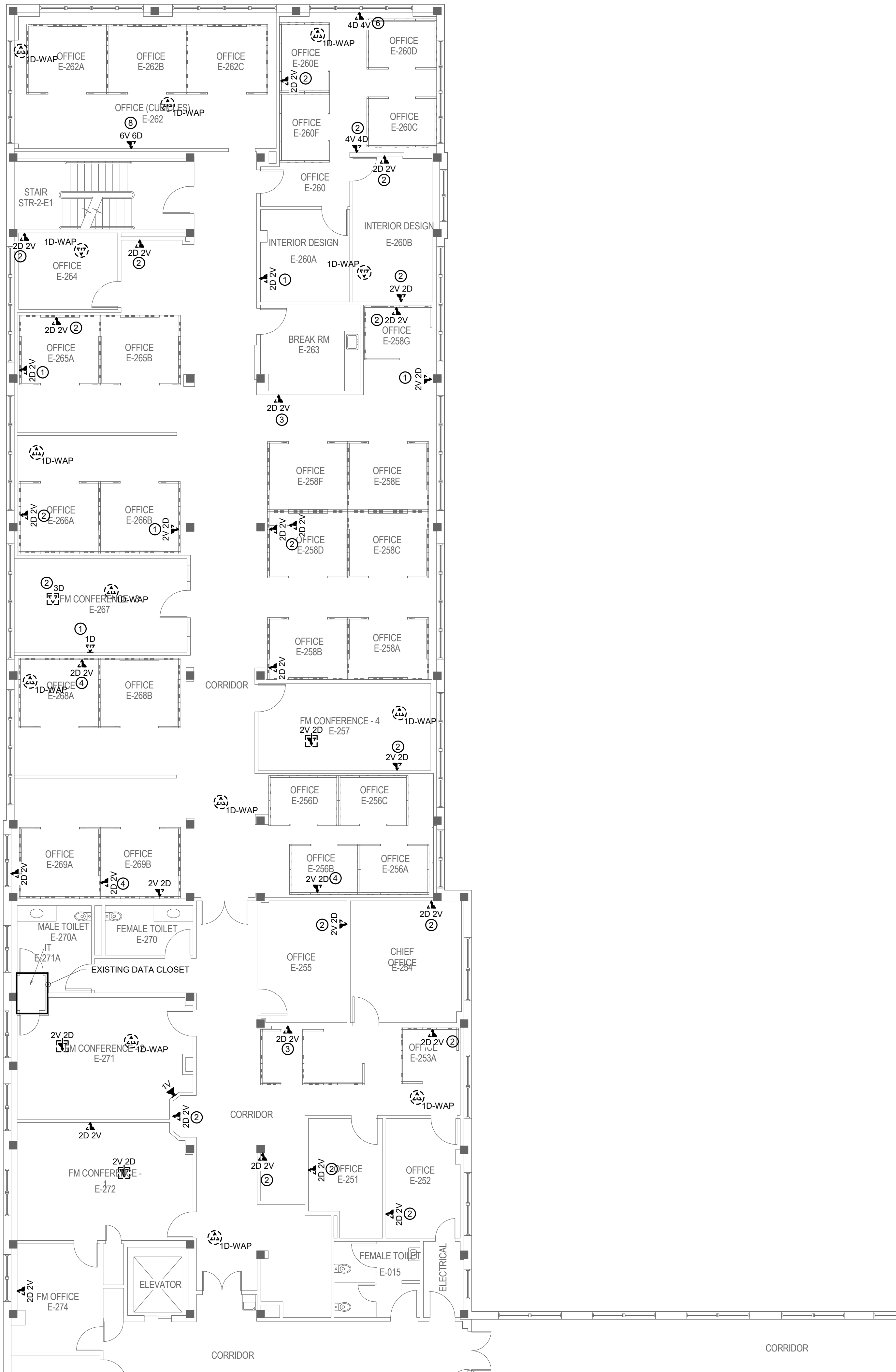
1 BUILDING 70 SECOND FLOOR DEMOLITION PLAN - TECHNOLOGY - AREA E NORTH 1/8" = 1'-0"
