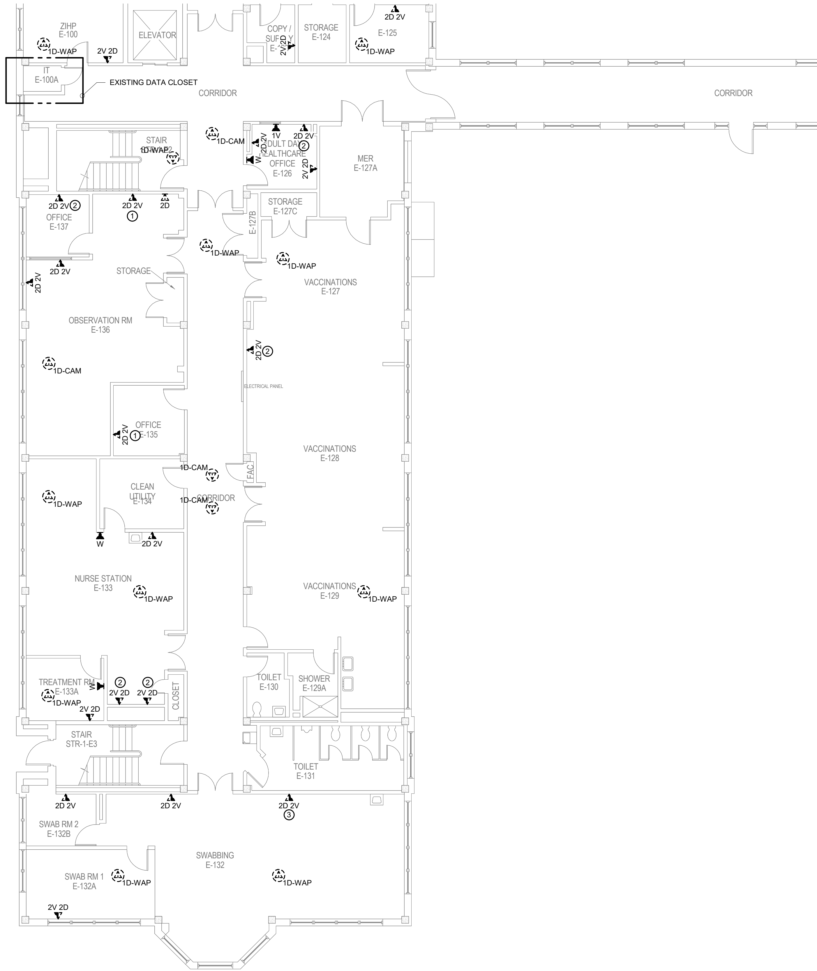
1 BUILDING 70 FIRST FLOOR DEMOLITION PLAN - TECHNOLOGY - AREA E SOUTH 1/8" = 1'-0"
