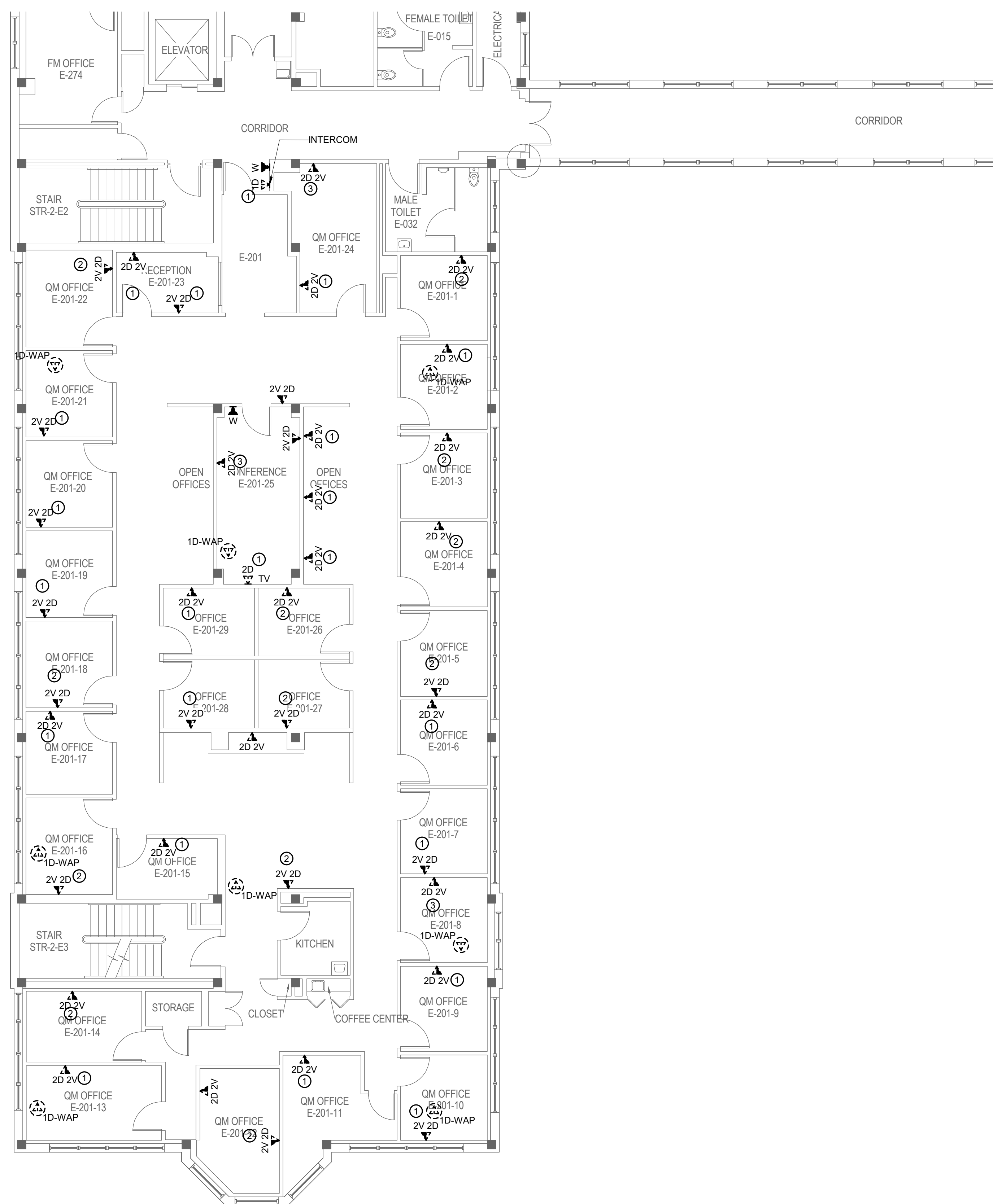
1 BUILDING 70 SECOND FLOOR DEMOLITION PLAN - TECHNOLOGY - AREA E SOUTH 1/8" = 1'-0"
