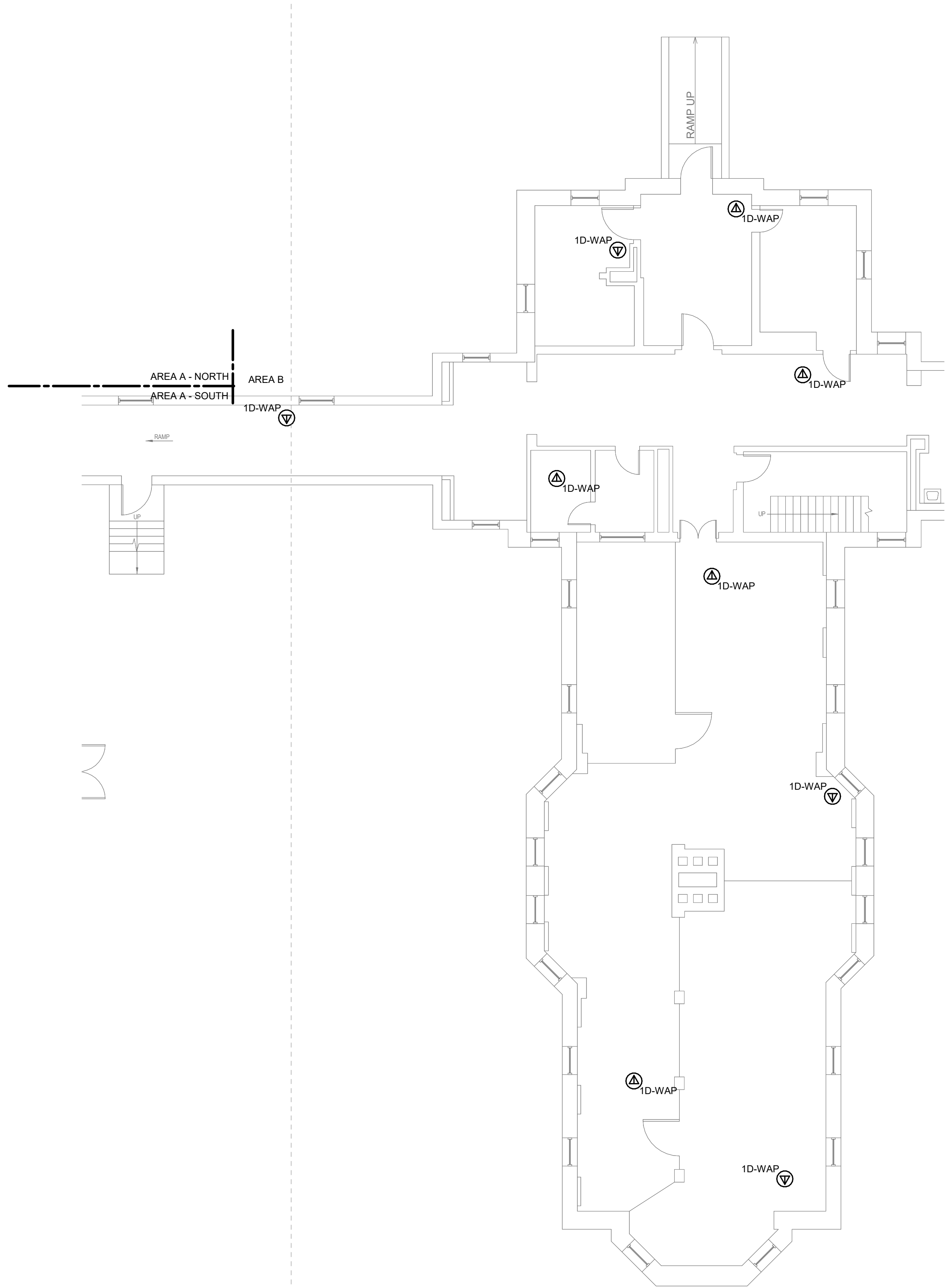
1 BUILDING 06 BASEMENT FLOOR PLAN - AREA B 1/8" = 1'-0"
