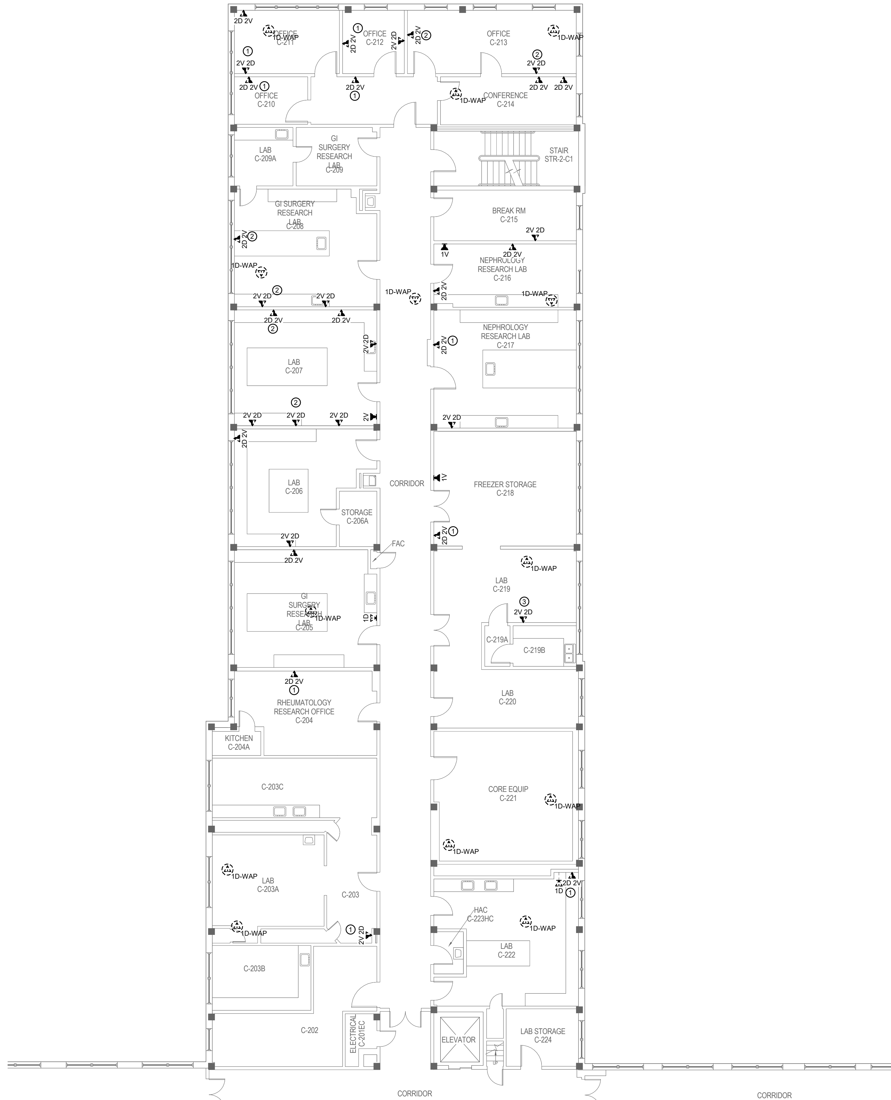
1 BUILDING 70 SECOND FLOOR DEMOLITION PLAN - TECHNOLOGY - AREA C NORTH 1/8" = 1'-0"
