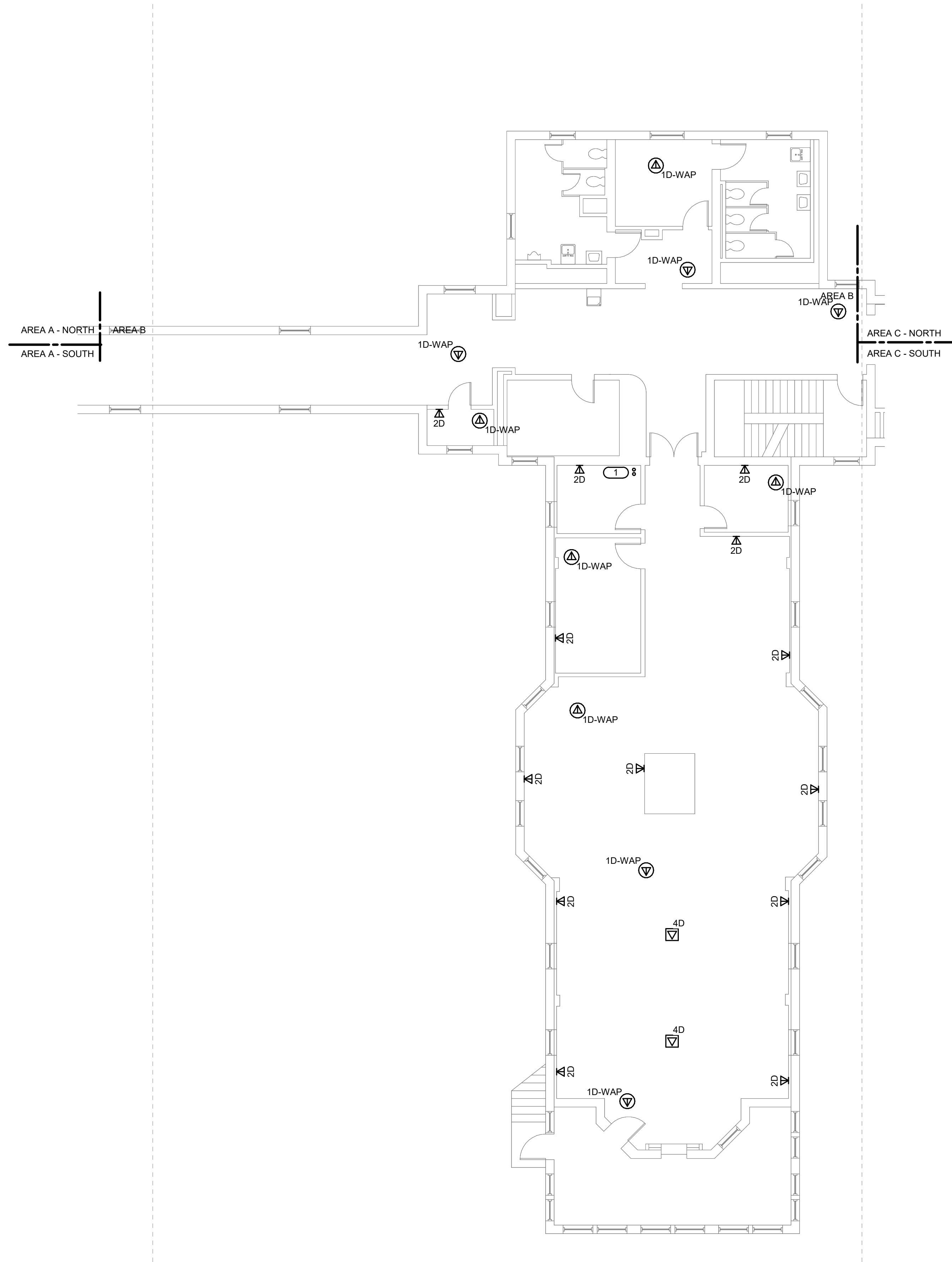
1 BUILDING 06 SECOND FLOOR PLAN - TECHNOLOGY - AREA B 1/8" = 1'-0"
