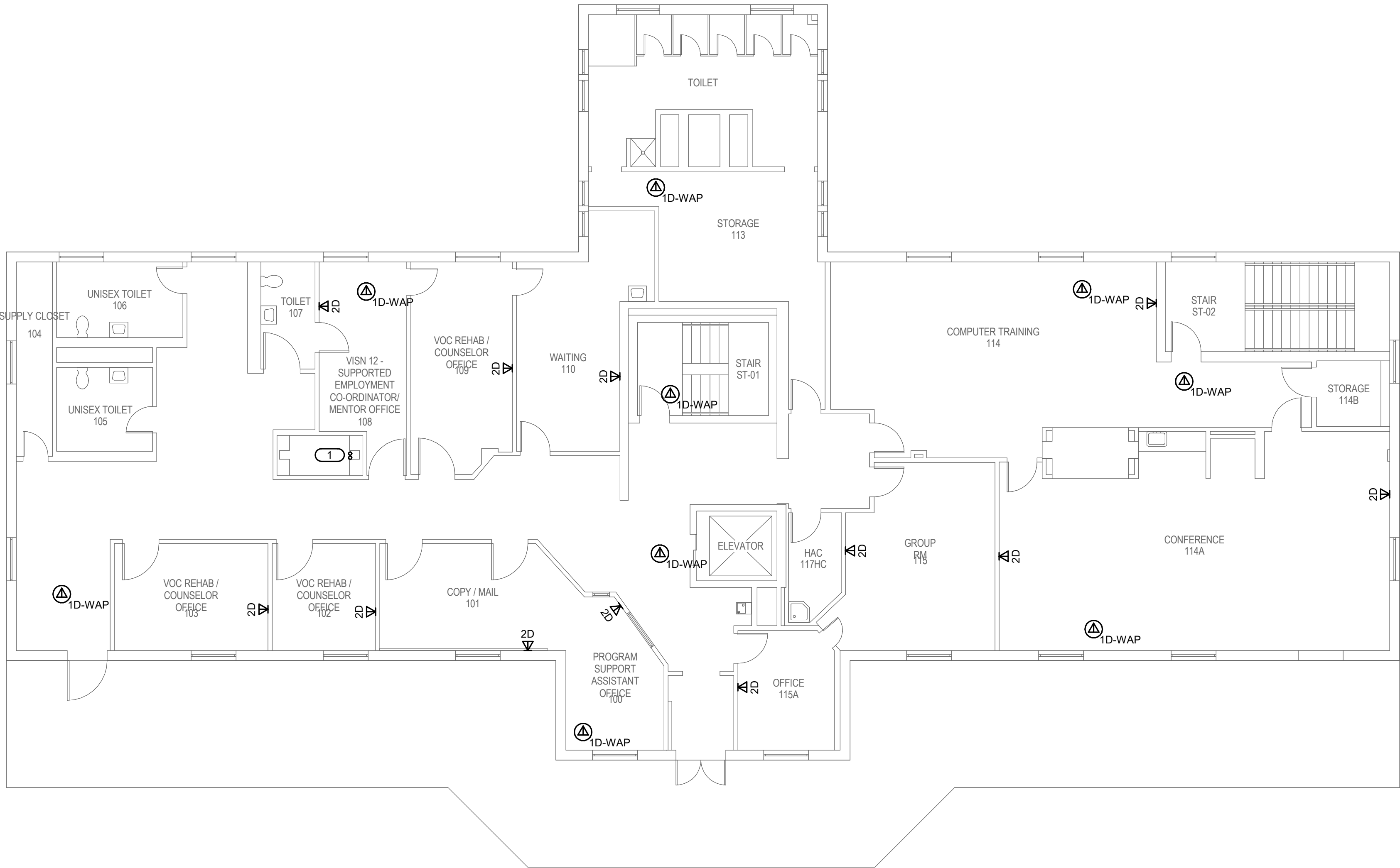
1 BUILDING 07 FIRST FLOOR PLAN - TECHNOLOGY 1/8" = 1'-0"
