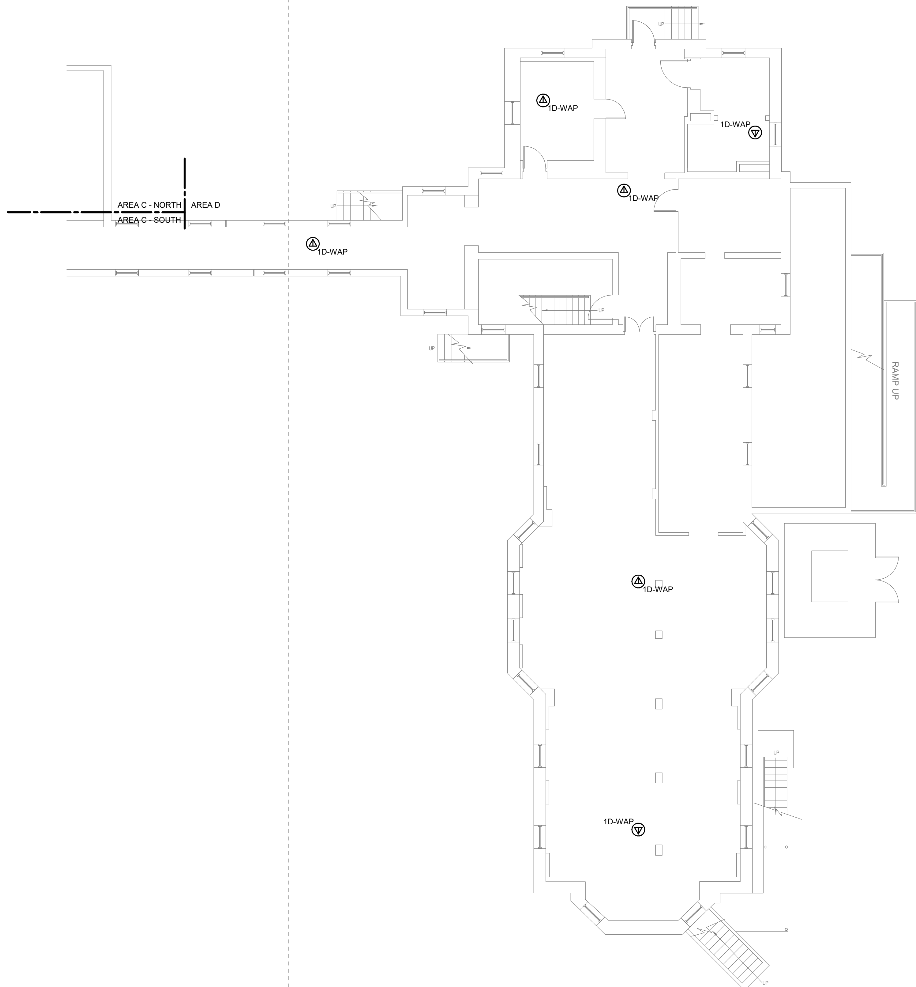
1 BUILDING 06 BASEMENT FLOOR PLAN - AREA D 1/8" = 1'-0"
