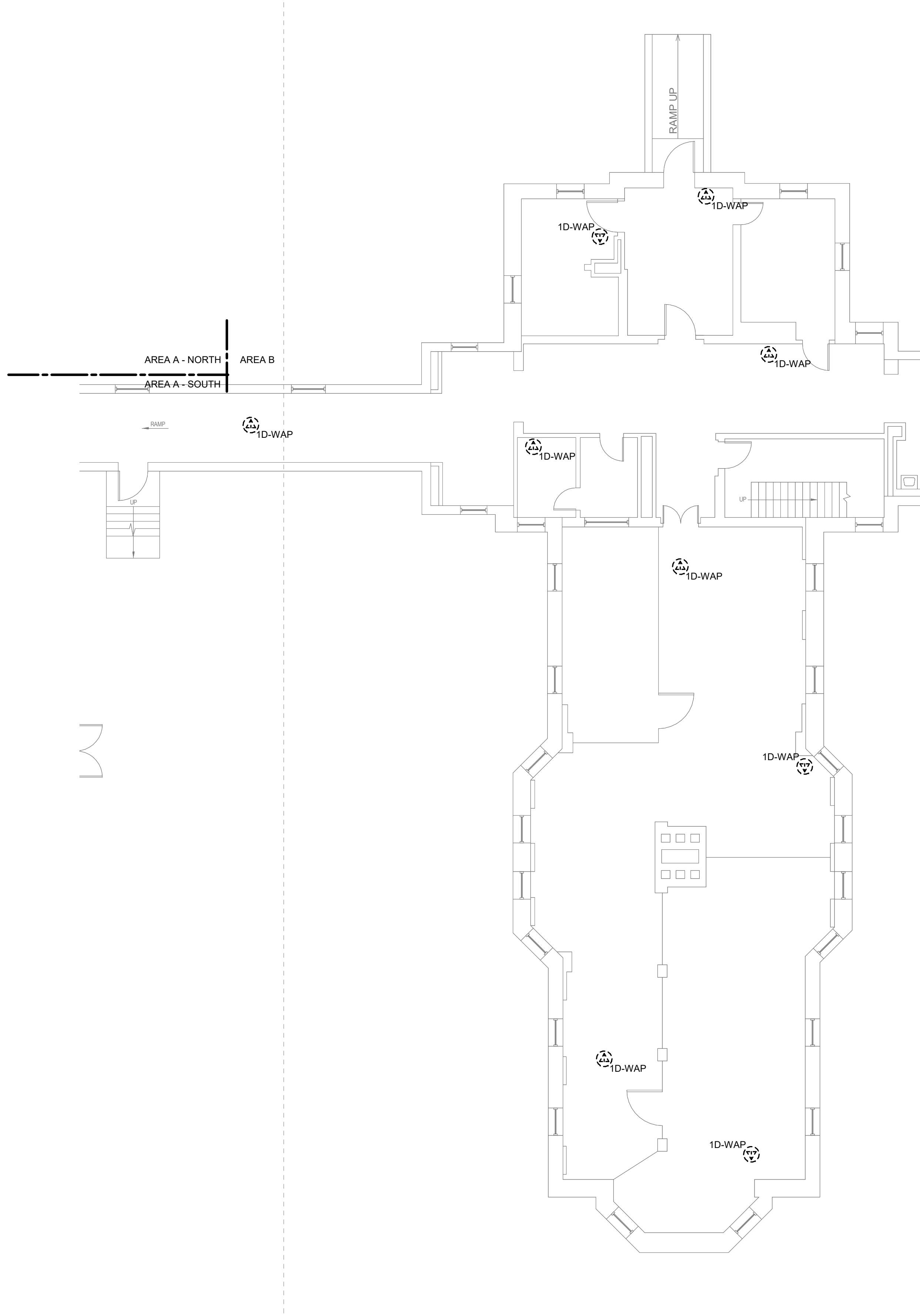
1 BUILDING 06 BASEMENT FLOOR DEMOLITION PLAN - TECHNOLOGY - AREA B 1/8" = 1'-0"
