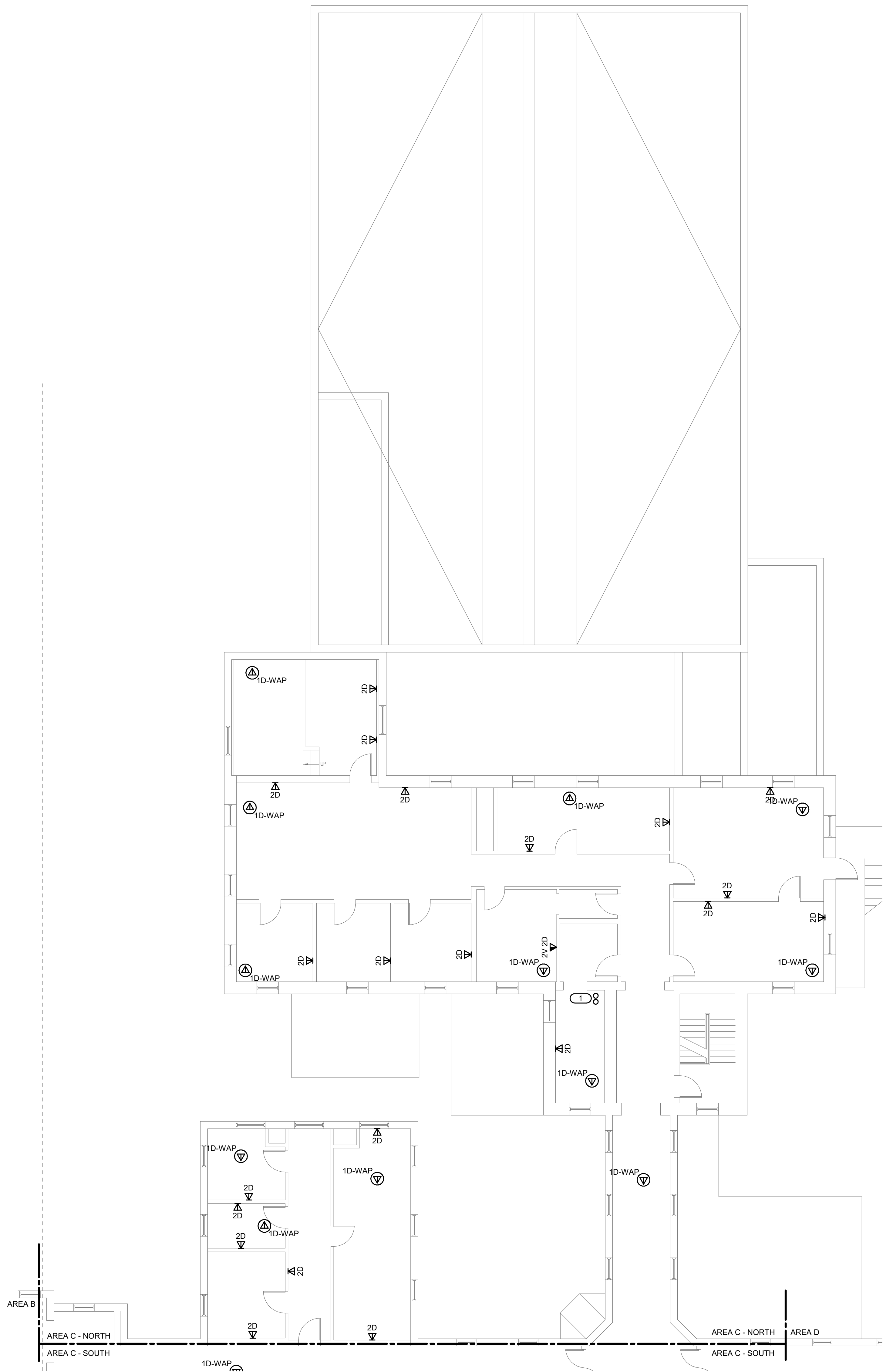
1 BUILDING 06 SECOND FLOOR PLAN - TECHNOLOGY - AREA C NORTH 1/8" = 1'-0"
