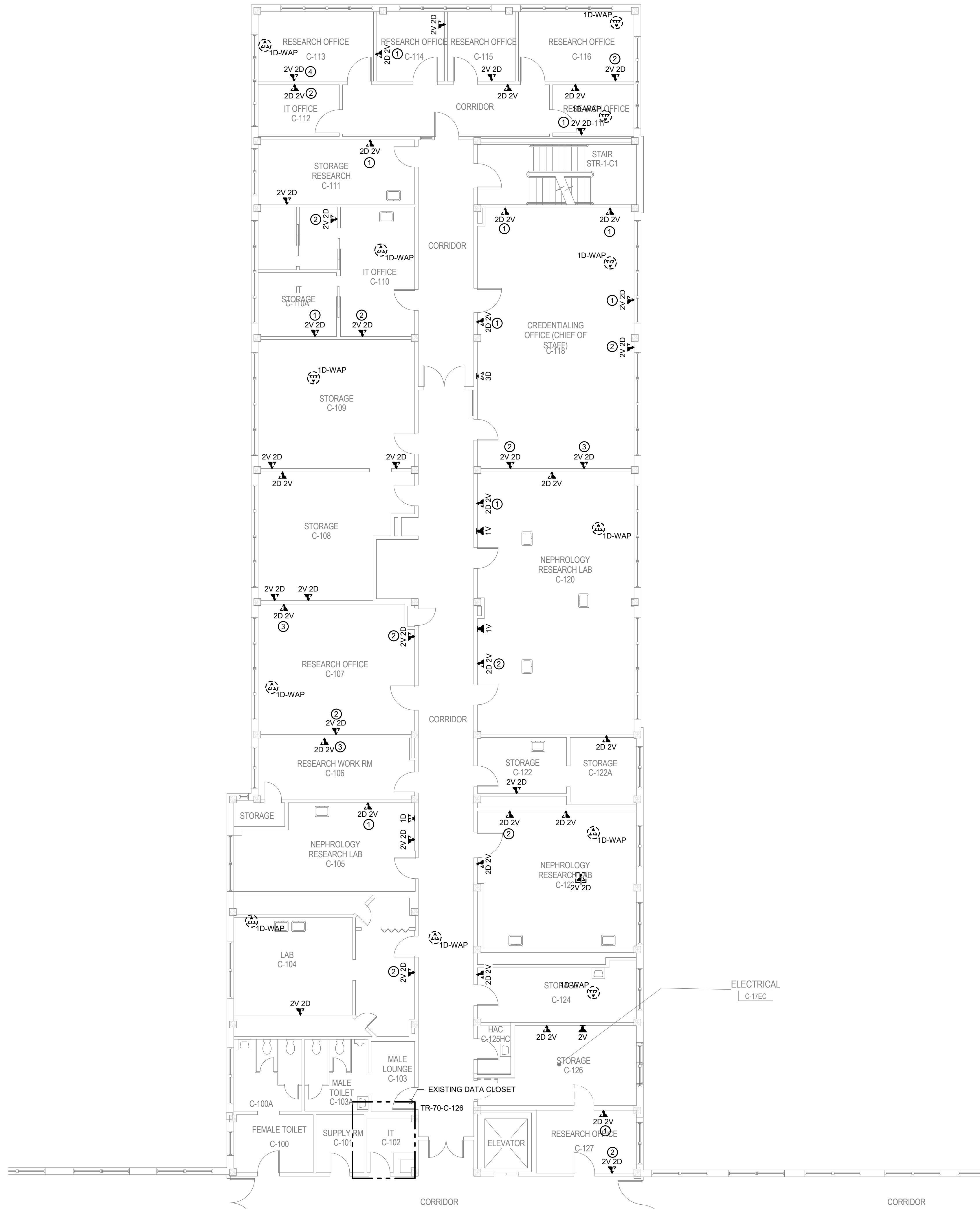
1 BUILDING 70 FIRST FLOOR DEMOLITION PLAN - TECHNOLOGY - AREA C NORTH 1/8" = 1'-0"
